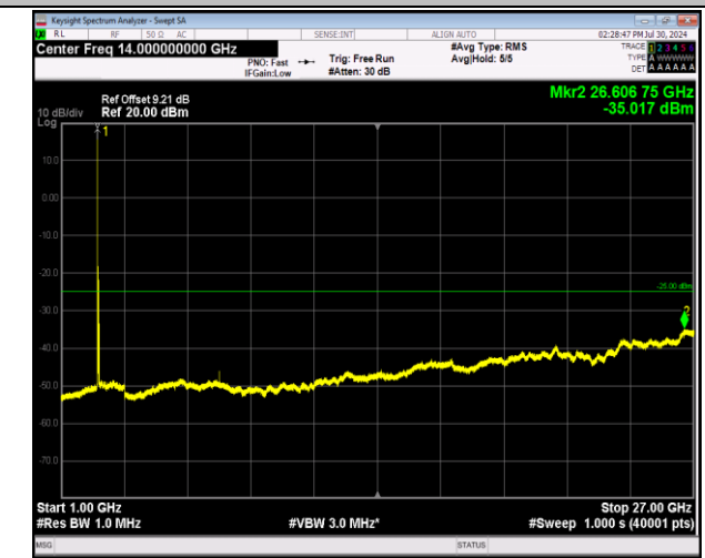
7-7-20MHz-20MHz-64QAM-64QAM-20850-21048-1RB#0-0RB#0-1000~27000MHz-PASS
