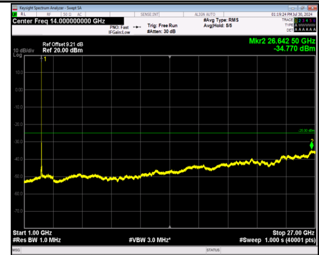
7-7-10MHz-20MHz-64QAM-64QAM-21206-21350-1RB#49- ORB#0-1000~27000MHz-PASS
