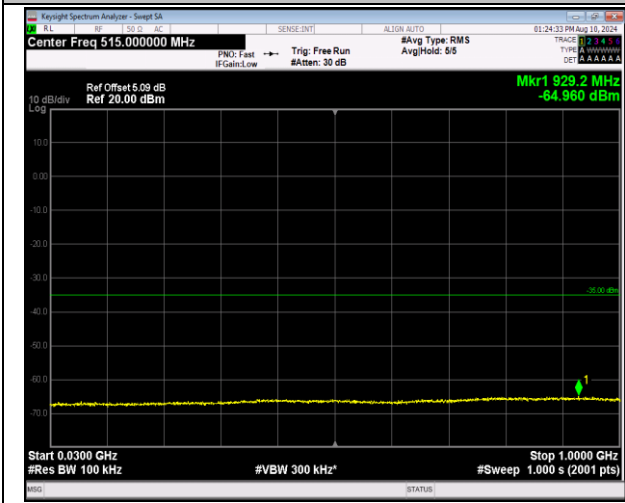
7-7-20MHz-10MHz-QPSK-QPSK-21051-21195-1RB#99-0 RB#0-30~1000MHz-PASS
