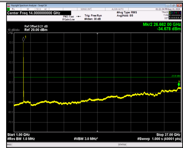
7-7-20MHz-10MHz-16QAM-16QAM-20850-20994-1RB#0-1 RB#49-1000~27000MHz-PASS
