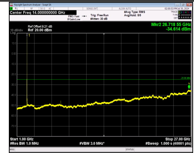
7-7-20MHz-10MHz-64QAM-64QAM-20850-20994-1RB#99- ORB#0-1000~27000MHz-PASS
