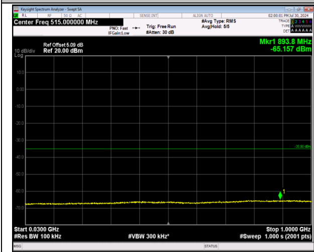
7-7-20MHz-10MHz-64QAM-64QAM-20850-20994-1RB#0 -0RB#0-30~1000MHz-PASS
