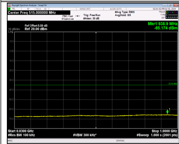
7-7-20MHz-10MHz-64QAM-64QAM-20850-20994-100RB #0-50RB#0-30~1000MHz-PASS
