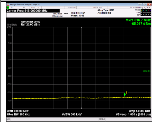
7-7-20MHz-10MHz-16QAM-16QAM-21051-21195-1RB#0 -1RB#49-30~1000MHz-PASS
