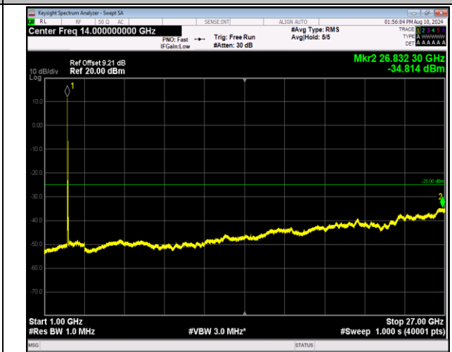
7-7-20MHz-20MHz-16QAM-16QAM-20850-21048-1RB#0-1 RB#99-1000~27000MHz-PASS
