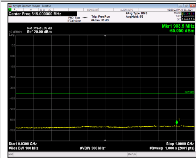
7-7-20MHz-20MHz-64QAM-64QAM-20850-21048-100RB #0-100RB#0-30~1000MHz-PASS
