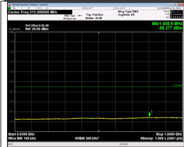
7-7-10MHz-20MHz-64QAM-64QAM-21206-21350-1RB#4 9-0RB#0-30~1000MHz-PASS
