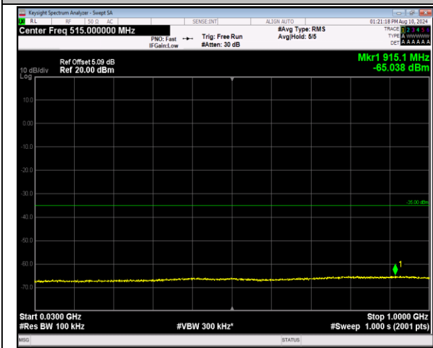
7-7-20MHz-10MHz-16QAM-16QAM-20850-20994-1RB#0 -1RB#49-30~1000MHz-PASS
