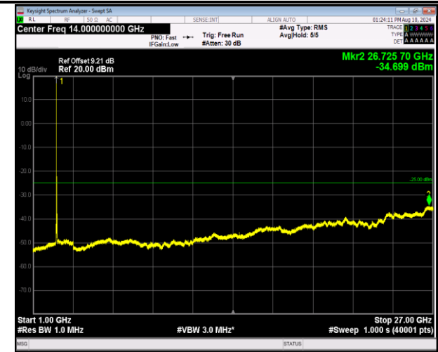
7-7-20MHz-10MHz-16QAM-16QAM-21051-21195-1RB#0-0 RB#0-1000~27000MHz-PASS
