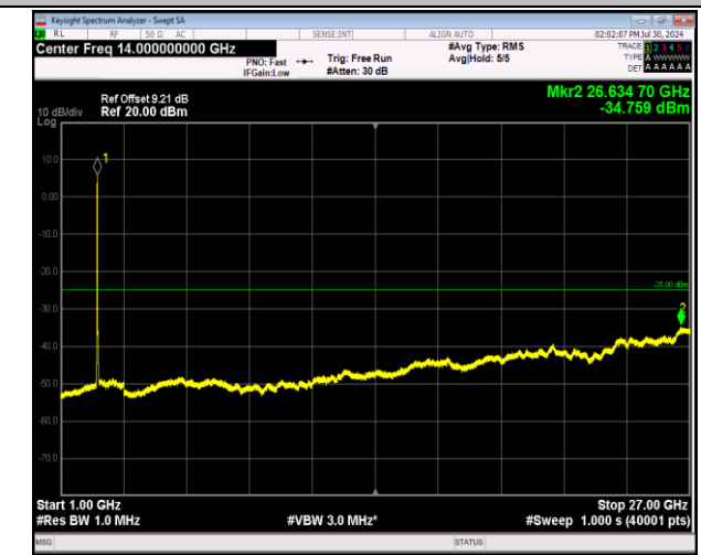
7-7-20MHz-10MHz-64QAM-64QAM-20850-20994-100RB#0 -50RB#0-1000~27000MHz-PASS
