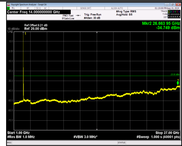
7-7-20MHz-10MHz-16QAM-16QAM-20850-20994-1RB#0-0 RB#0-1000~27000MHz-PASS
