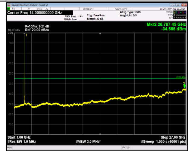
7-7-20MHz-10MHz-16QAM-16QAM-20850-20994-1RB#99- ORB#0-1000~27000MHz-PASS
