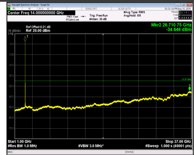
7-7-20MHz-10MHz-QPSK-QPSK-21251-21395-1RB#0-1RB #49-1000~27000MHz-PASS
