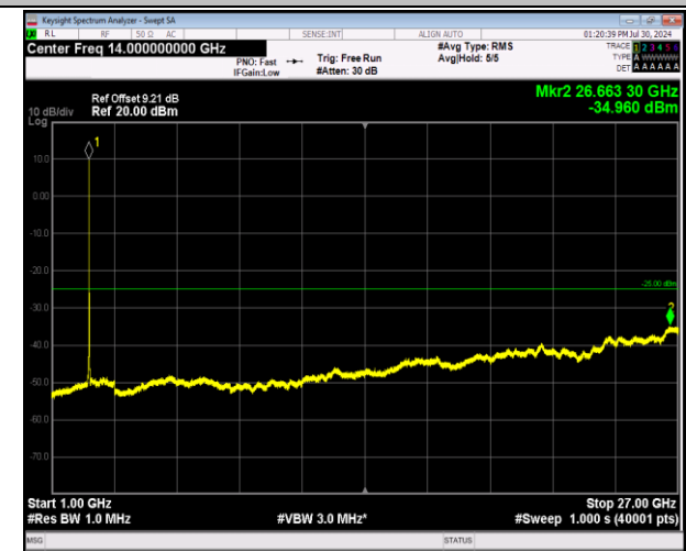
7-7-10MHz-20MHz-64QAM-64QAM-21206-21350-50RB#0- 100RB#0-1000~27000MHz-PASS
