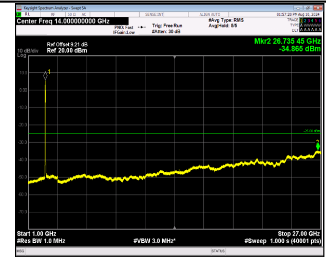
7-7-20MHz-20MHz-16QAM-16QAM-20850-21048-100RB#0-100RB#0-1000~27000MHz-PASS
