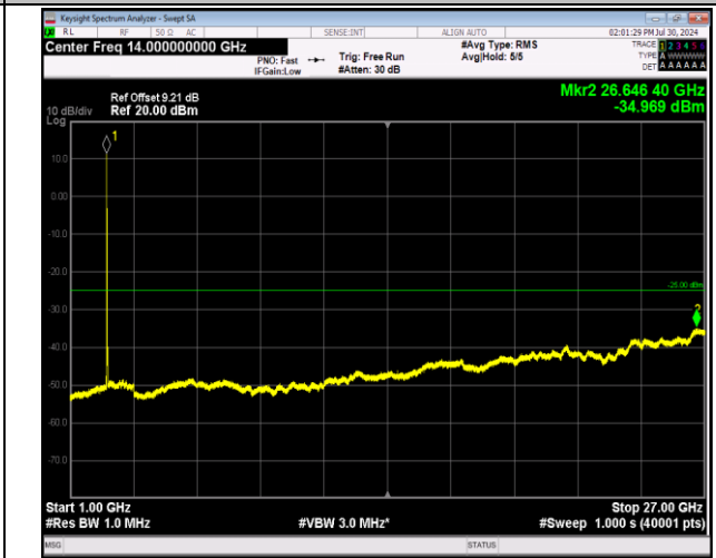
7-7-20MHz-10MHz-64QAM-64QAM-20850-20994-1RB#0-1 RB#49-1000~27000MHz-PASS
