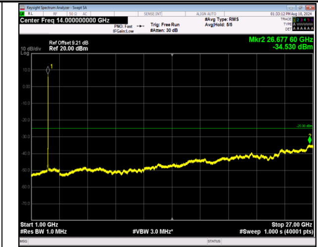
7-7-20MHz-10MHz-16QAM-16QAM-21251-21395-100RB#0 -50RB#0-1000~27000MHz-PASS
