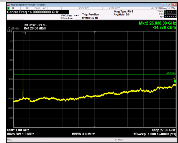
7-7-20MHz-10MHz-16QAM-16QAM-21051-21195-1RB#99- ORB#0-1000~27000MHz-PASS
