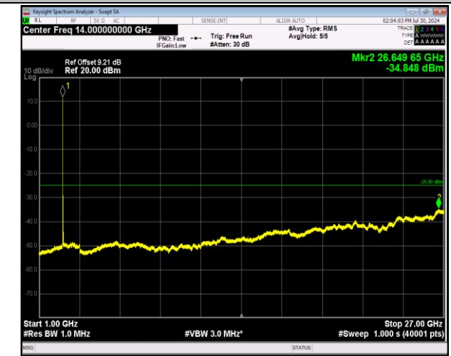
7-7-20MHz-10MHz-64QAM-64QAM-21051-21195-1RB#0-1 RB#49-1000~27000MHz-PASS
