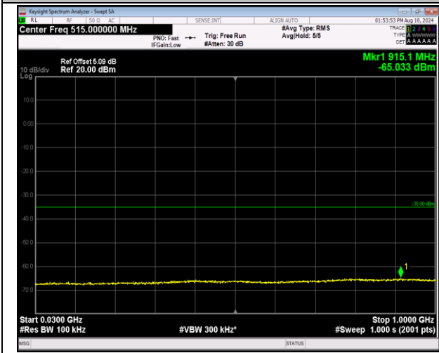
7-7-20MHz-20MHz-QPSK-QPSK-20850-21048-1RB#99-0RB#0-30~1000MHz-PASS
