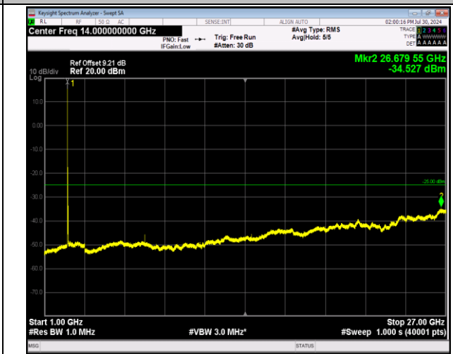
7-7-20MHz-10MHz-64QAM-64QAM-20850-20994-1RB#0-0 RB#0-1000~27000MHz-PASS
