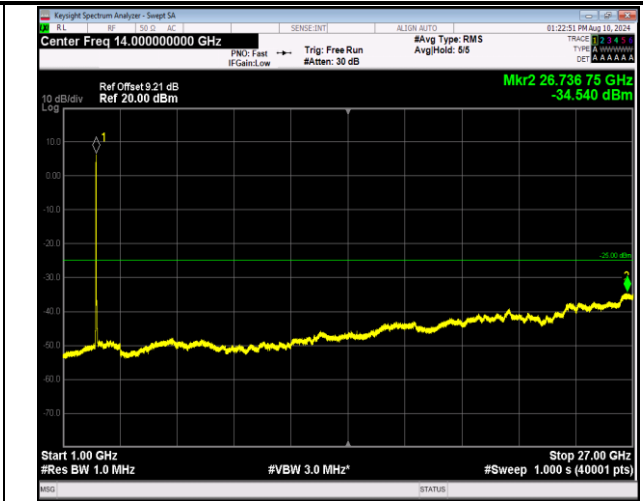
7-7-20MHz-10MHz-16QAM-16QAM-20850-20994-100RB#0 -50RB#0-1000~27000MHz-PASS
