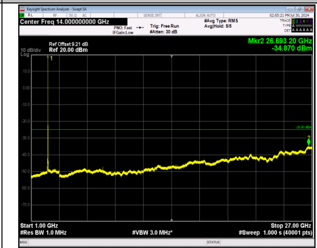
7-7-20MHz-10MHz-64QAM-64QAM-21251-21395-1RB#0-0 RB#0-1000~27000MHz-PASS
