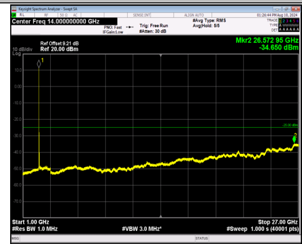
7-7-20MHz-10MHz-16QAM-16QAM-21051-21195-1RB#0-1 RB#49-1000~27000MHz-PASS
