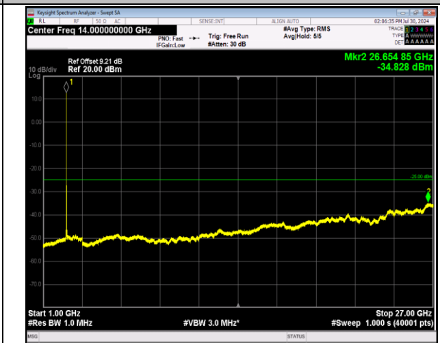
7-7-20MHz-10MHz-64QAM-64QAM-21251-21395-1RB#0-1 RB#49-1000~27000MHz-PASS
