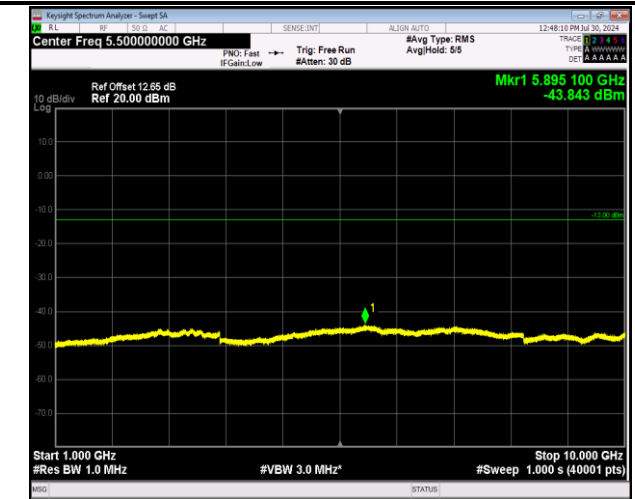
5-5-10MHz-10MHz-64QAM-64QAM-20450-20549-1RB#49- ORB#0-1000~10000MHz-PASS
