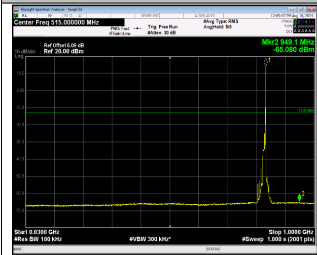
5-5-10MHz-10MHz-QPSK-QPSK-20476-20575-1RB#49-0R 0RB#0-30~1000MHz-PASS
