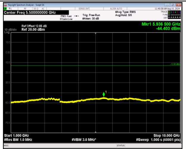
5-5-5MHz-3MHz-QPSK-QPSK-20510-20549-25RB#0-15RB #0-1000~10000MHz-PASS
