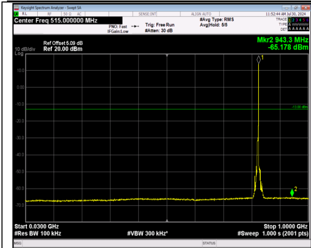
5-5-5MHz-3MHz-64QAM-64QAM-20425-20464-1RB#24-0RB#0-30~1000MHz-PASS
