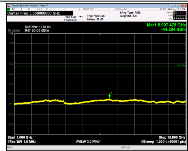
5-5-10MHz-10MHz-QPSK-QPSK-20450-20549-1RB#49-0RB#0-1000~10000MHz-PASS
