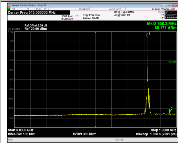
5-5-5MHz-3MHz-64QAM-64QAM-20425-20464-1RB#0-0RB#0-30~1000MHz-PASS
