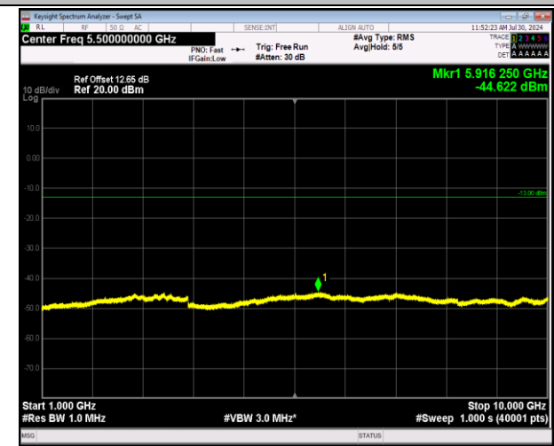
5-5-5MHz-3MHz-64QAM-64QAM-20425-20464-1RB#0-0RB#0-1000~10000MHz-PASS
