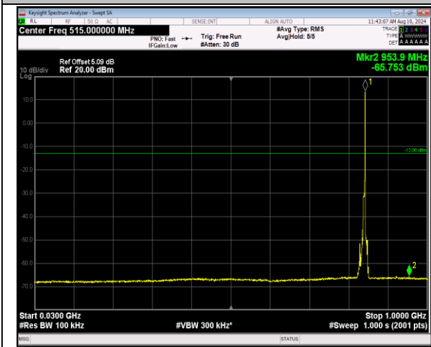
5-5-5MHz-3MHz-QPSK-QPSK-20595-20634-1RB#24-0R B#0-30~1000MHz-PASS
