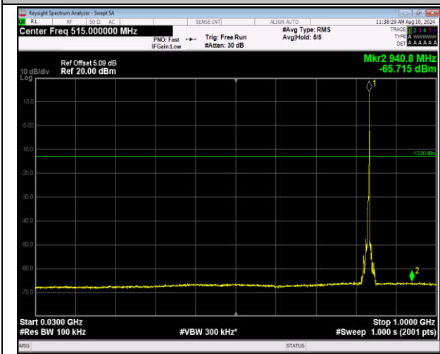
5-5-5MHz-3MHz-QPSK-QPSK-20510-20549-1RB#24-0R B#0-30~1000MHz-PASS
