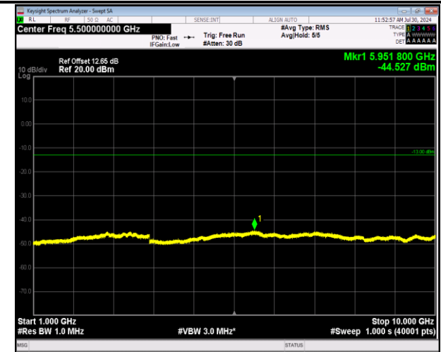
5-5-5MHz-3MHz-64QAM-64QAM-20425-20464-1RB#24-0RB#0-1000~10000MHz-PASS
