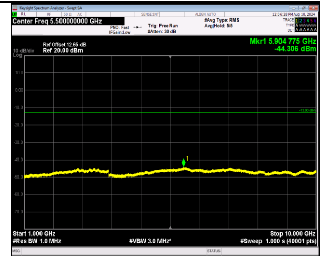
5-5-10MHz-10MHz-QPSK-QPSK-20450-20549-1RB#0-1RB #49-1000~10000MHz-PASS
