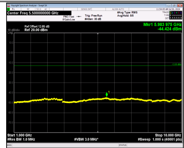
5-5-5MHz-3MHz-64QAM-64QAM-20425-20464-25RB#0-15RB#0-1000~10000MHz-PASS
