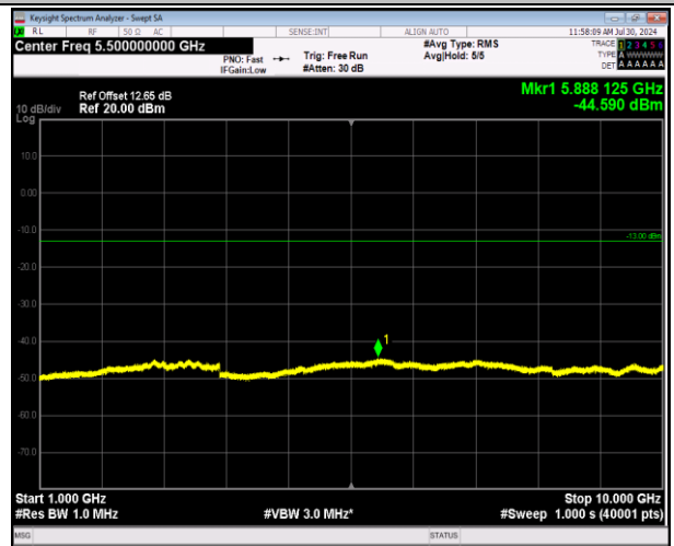
5-5-5MHz-3MHz-64QAM-64QAM-20595-20634-1RB#0-1RB#15-1000~10000MHz-PASS
