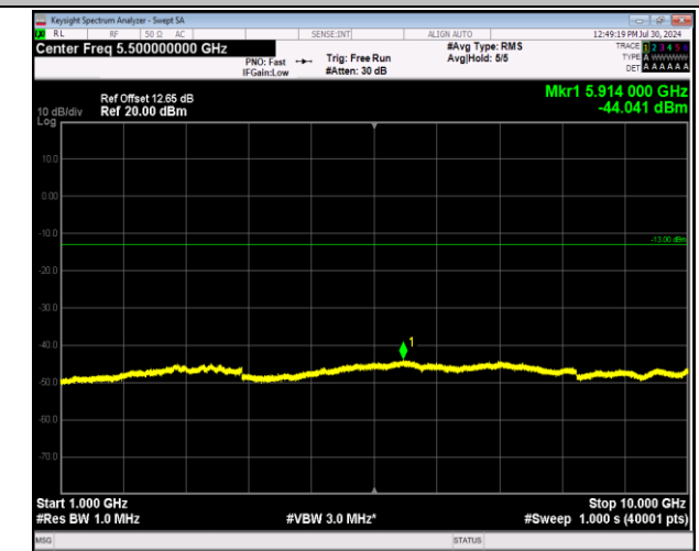
5-5-10MHz-10MHz-64QAM-64QAM-20450-20549-50RB#0- 50RB#0-1000~10000MHz-PASS
