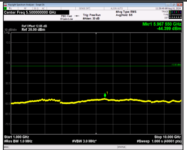
5-5-5MHz-3MHz-QPSK-QPSK-20510-20549-1RB#0-1RB#1 5-1000~10000MHz-PASS
