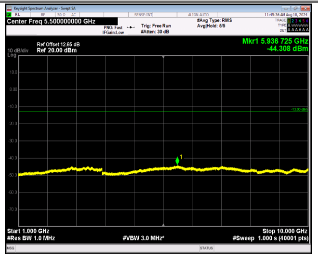
5-5-5MHz-3MHz-QPSK-QPSK-20595-20634-25RB#0-15RB #0-1000~10000MHz-PASS
