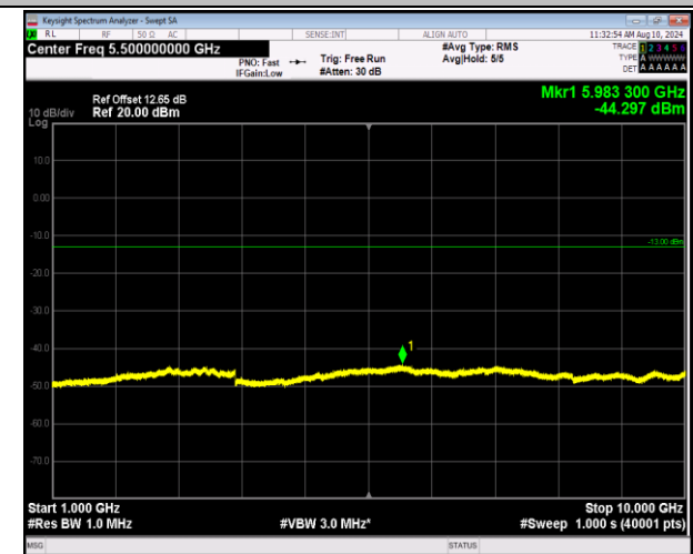
5-5-5MHz-3MHz-QPSK-QPSK-20425-20464-1RB#0-0RB#0 -1000~10000MHz-PASS
