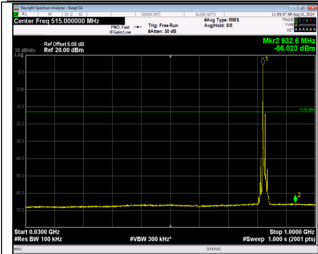
5-5-3MHz-5MHz-QPSK-QPSK-20416-20455-1RB#0-1RB #24-30~1000MHz-PASS
