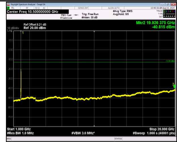
2-2-20MHz-20MHz-16QAM-16QAM-18902-19100-1RB#0-0 RB#0-1000~20000MHz-PASS
