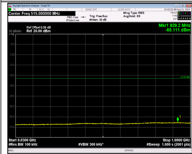
2-2-20MHz-20MHz-16QAM-16QAM-18902-19100-1RB#0 -1RB#99-30~1000MHz-PASS
