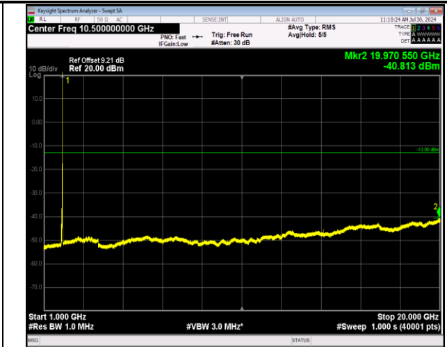
2-2-20MHz-20MHz-64QAM-64QAM-18902-19100-1RB#99- ORB#0-1000~20000MHz-PASS
