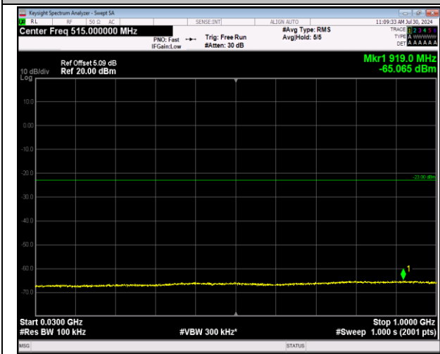
2-2-20MHz-20MHz-64QAM-64QAM-18902-19100-1RB#0-0RB#0-30~1000MHz-PASS
