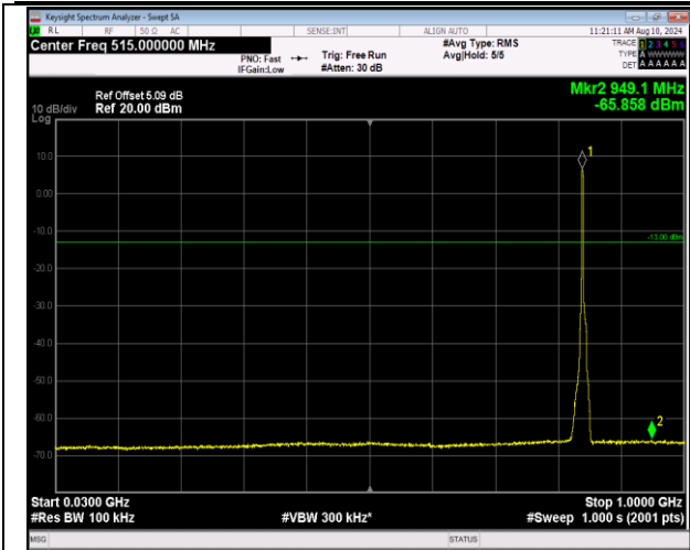
5-5-3MHz-5MHz-16QAM-16QAM-20586-20625-15RB#0-25RB#0-30~1000MHz-PASS
