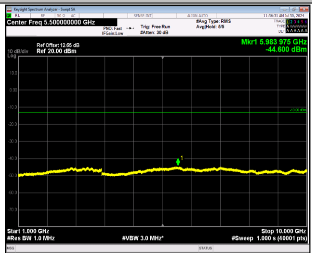
5-5-3MHz-5MHz-64QAM-64QAM-20501-20540-1RB#0-0RB#0-1000~10000MHz-PASS
