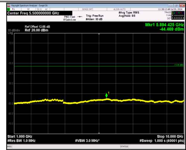
5-5-3MHz-5MHz-64QAM-64QAM-20501-20540-15RB#0-25RB#0-1000~10000MHz-PASS
