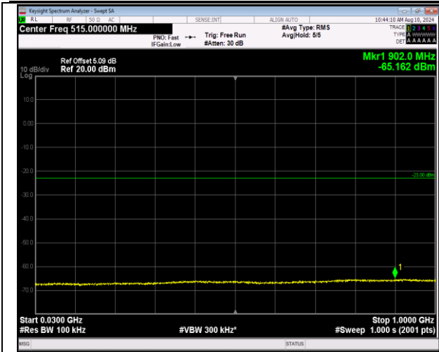
2-2-20MHz-20MHz-16QAM-16QAM-18902-19100-100RB#0-100RB#0-30~1000MHz-PASS
