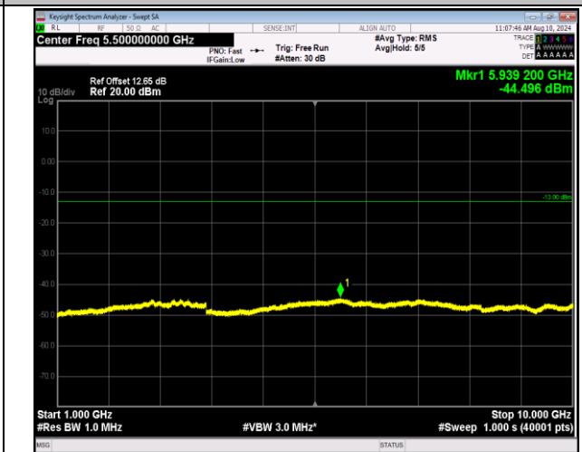
5-5-3MHz-5MHz-QPSK-QPSK-20416-20455-1RB#0-0RB#0 -1000~10000MHz-PASS
