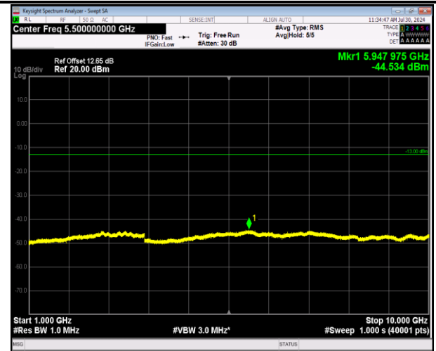
5-5-3MHz-5MHz-64QAM-64QAM-20416-20455-1RB#14-0RB#0-1000~10000MHz-PASS
