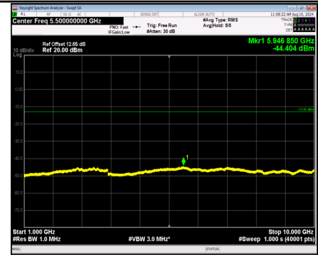
5-5-3MHz-5MHz-16QAM-16QAM-20416-20455-1RB#0-0R B#0-1000~10000MHz-PASS
