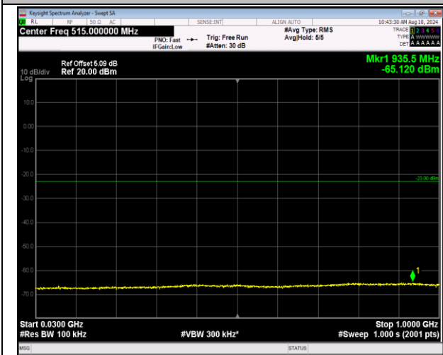
2-2-20MHz-20MHz-QPSK-QPSK-18902-19100-100RB#0 -100RB#0-30~1000MHz-PASS
