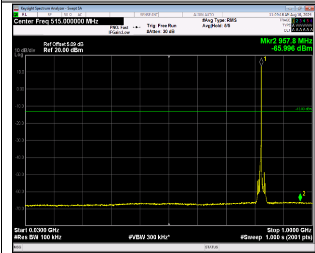
5-5-3MHz-5MHz-16QAM-16QAM-20416-20455-1RB#14- ORB#0-30~1000MHz-PASS
