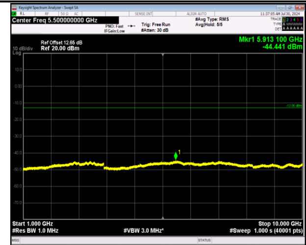
5-5-3MHz-5MHz-64QAM-64QAM-20501-20540-1RB#14-0RB#0-1000~10000MHz-PASS
