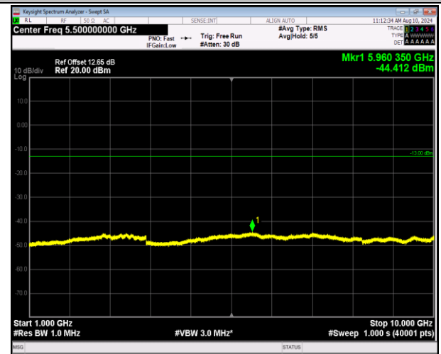
5-5-3MHz-5MHz-QPSK-QPSK-20501-20540-1RB#0-0RB#0-1000~10000MHz-PASS
