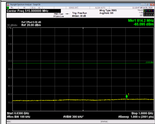
2-2-20MHz-20MHz-64QAM-64QAM-18902-19100-1RB#0-1RB#99-30~1000MHz-PASS
