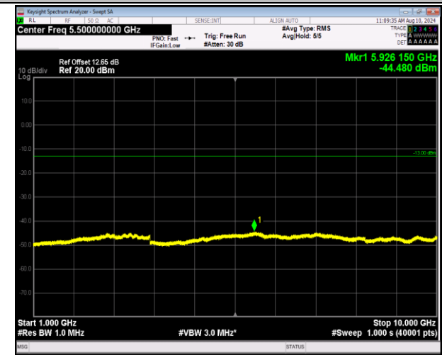
5-5-3MHz-5MHz-16QAM-16QAM-20416-20455-1RB#14-0R B#0-1000~10000MHz-PASS
