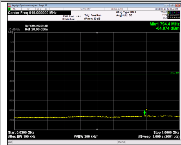
2-2-20MHz-20MHz-64QAM-64QAM-18902-19100-100RB #0-100RB#0-30~1000MHz-PASS
