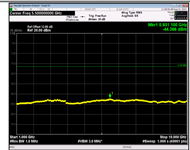
5-5-3MHz-5MHz-QPSK-QPSK-20416-20455-1RB#14-0RB# 0-1000~10000MHz-PASS
