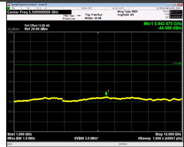
5-5-3MHz-5MHz-64QAM-64QAM-20586-20625-1RB#14-0R B#0-1000~10000MHz-PASS
