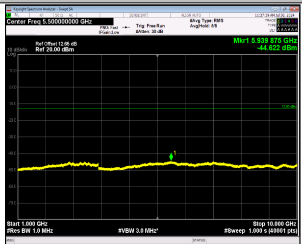
5-5-3MHz-5MHz-64QAM-64QAM-20501-20540-1RB#0-1RB#24-1000~10000MHz-PASS
