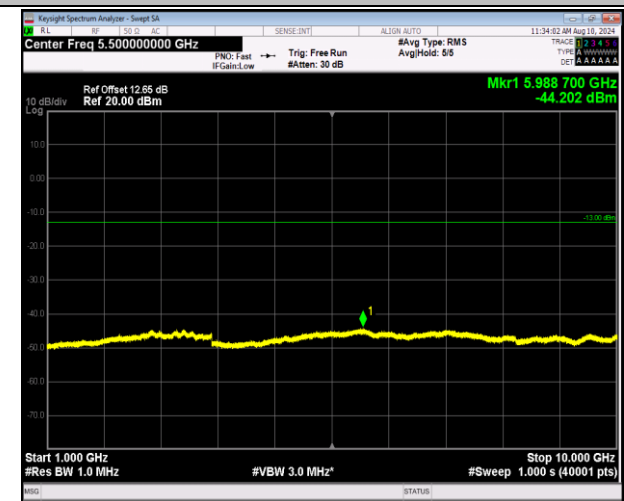
5-5-5MHz-3MHz-QPSK-QPSK-20425-20464-1RB#24-0RB# 0-1000~10000MHz-PASS
