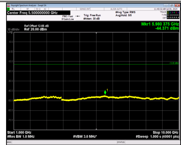
5-5-3MHz-5MHz-64QAM-64QAM-20586-20625-15RB#0-25 RB#0-1000~10000MHz-PASS
