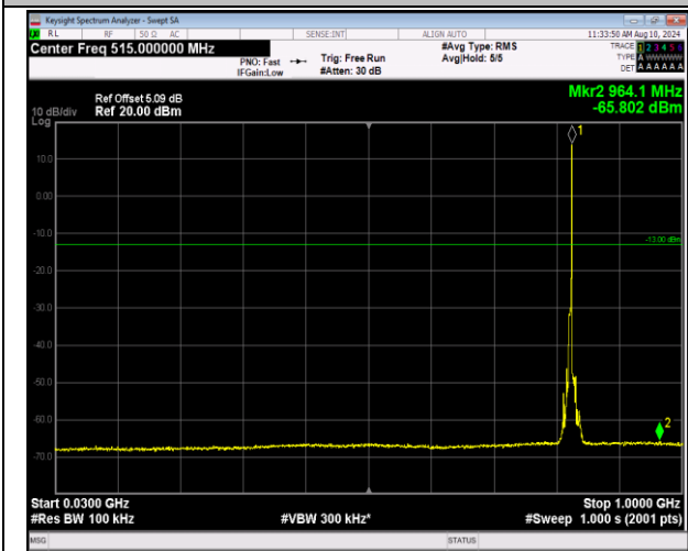
5-5-5MHz-3MHz-QPSK-QPSK-20425-20464-1RB#24-0R B#0-30~1000MHz-PASS
