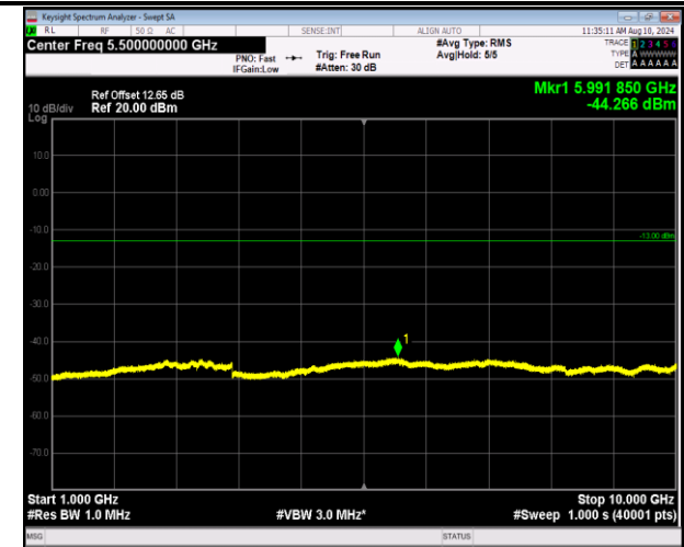
5-5-5MHz-3MHz-QPSK-QPSK-20425-20464-1RB#0-1RB#1 5-1000~10000MHz-PASS
