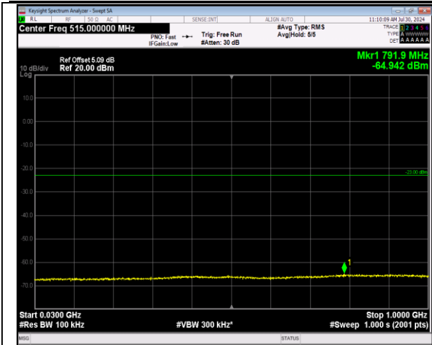
2-2-20MHz-20MHz-64QAM-64QAM-18902-19100-1RB#9 9-ORB#0-30~1000MHz-PASS
