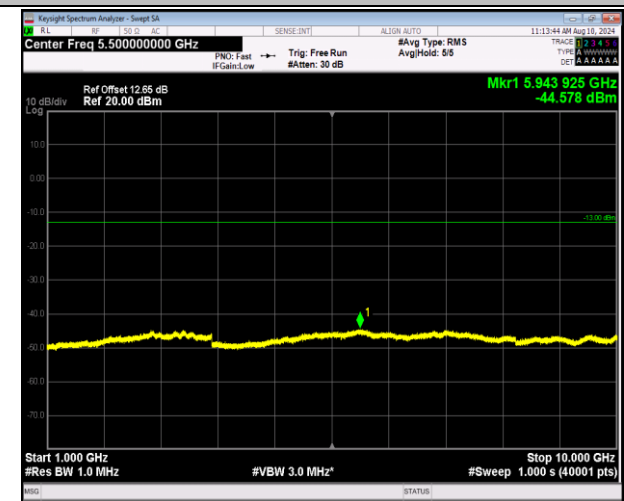
5-5-3MHz-5MHz-QPSK-QPSK-20501-20540-1RB#14-0RB# 0-1000~10000MHz-PASS
