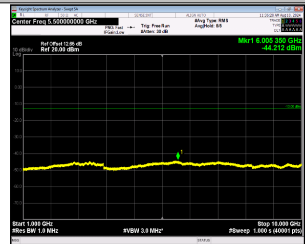
5-5-5MHz-3MHz-QPSK-QPSK-20425-20464-25RB#0-15RB #0-1000~10000MHz-PASS
