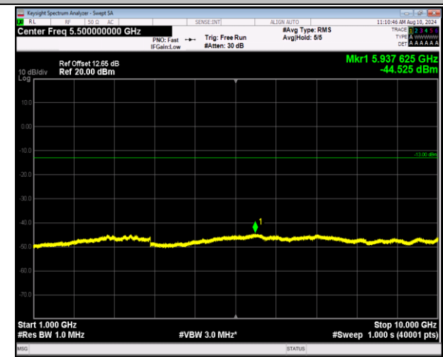
5-5-3MHz-5MHz-16QAM-16QAM-20416-20455-1RB#0-1R B#24-1000~10000MHz-PASS
