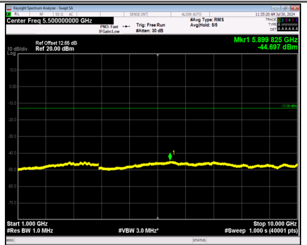
5-5-3MHz-5MHz-64QAM-64QAM-20416-20455-1RB#0-1RB#24-1000~10000MHz-PASS
