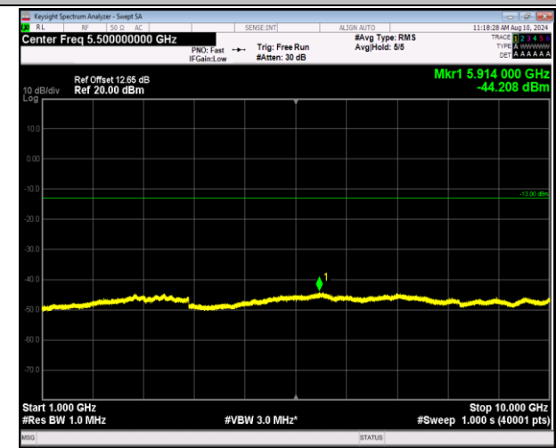
5-5-3MHz-5MHz-QPSK-QPSK-20586-20625-1RB#14-0RB# 0-1000~10000MHz-PASS
