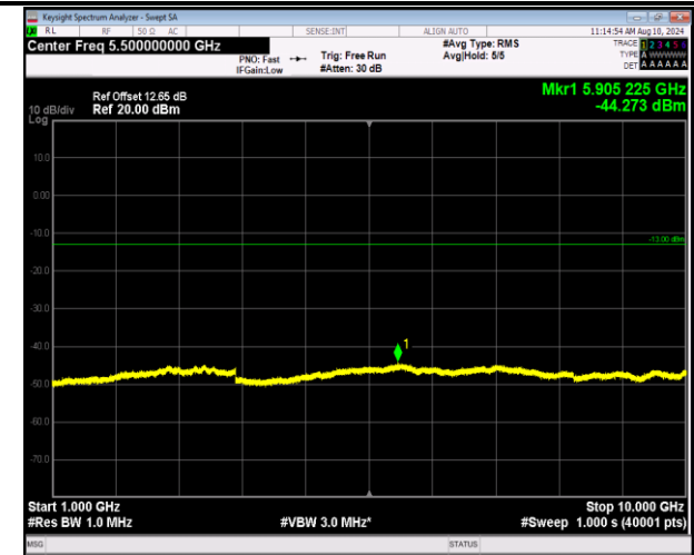
5-5-3MHz-5MHz-QPSK-QPSK-20501-20540-1RB#0-1RB#2 4-1000~10000MHz-PASS
