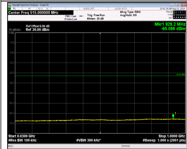
2-2-20MHz-20MHz-16QAM-16QAM-18902-19100-1RB#9 9-ORB#0-30~1000MHz-PASS
