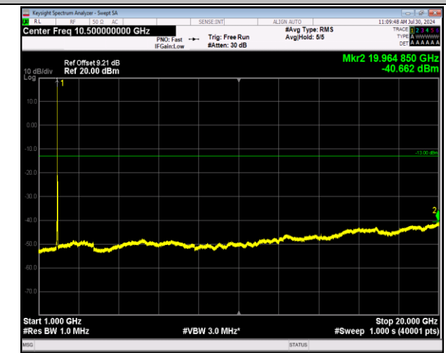
2-2-20MHz-20MHz-64QAM-64QAM-18902-19100-1RB#0-0RB#0-1000~20000MHz-PASS
