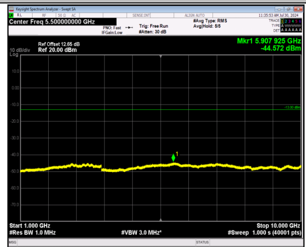
5-5-3MHz-5MHz-64QAM-64QAM-20416-20455-15RB#0-25RB#0-1000~10000MHz-PASS
