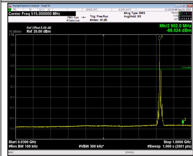
5-5-3MHz-5MHz-16QAM-16QAM-20416-20455-1RB#0-1 RB#24-30~1000MHz-PASS
