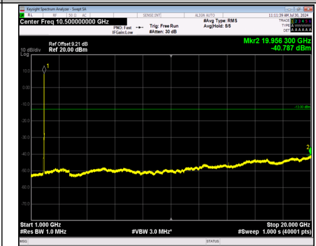
2-2-20MHz-20MHz-64QAM-64QAM-18902-19100-100RB#0 -100RB#0-1000~20000MHz-PASS
