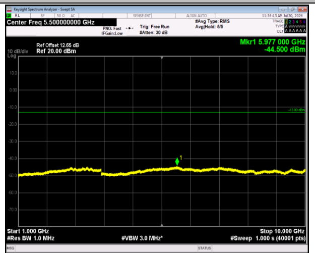
5-5-3MHz-5MHz-64QAM-64QAM-20416-20455-1RB#0-0RB#0-1000~10000MHz-PASS
