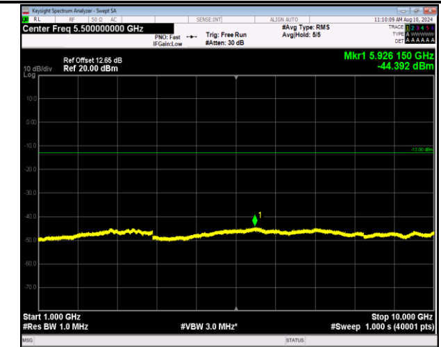
5-5-3MHz-5MHz-QPSK-QPSK-20416-20455-1RB#0-1RB#2 4-1000~10000MHz-PASS
