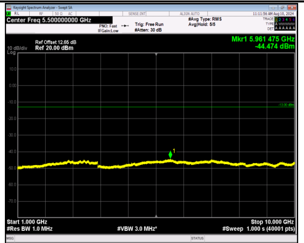
5-5-3MHz-5MHz-16QAM-16QAM-20416-20455-15RB#0-25RB#0-1000~10000MHz-PASS
