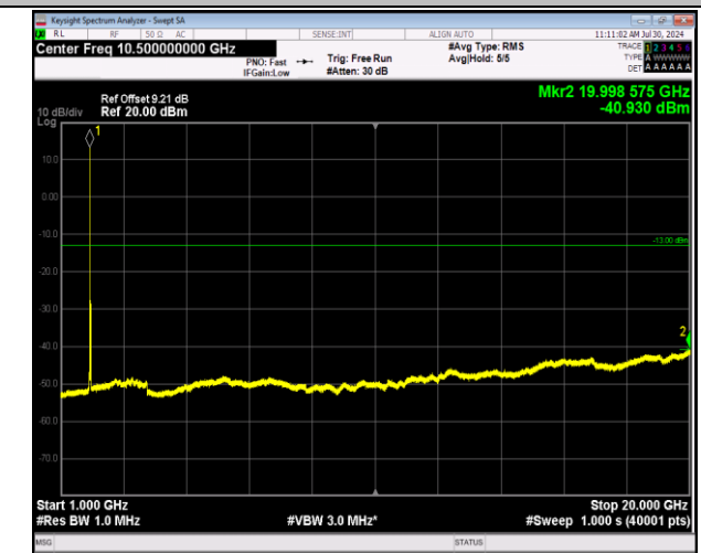
2-2-20MHz-20MHz-64QAM-64QAM-18902-19100-1RB#0-1RB#99-1000~20000MHz-PASS
