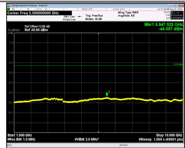
5-5-3MHz-5MHz-QPSK-QPSK-20586-20625-1RB#0-0RB#0-1000~10000MHz-PASS
