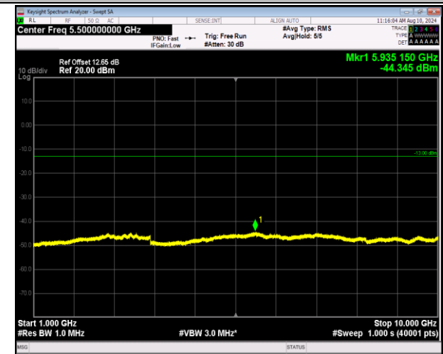
5-5-3MHz-5MHz-QPSK-QPSK-20501-20540-15RB#0-25RB #0-1000~10000MHz-PASS
