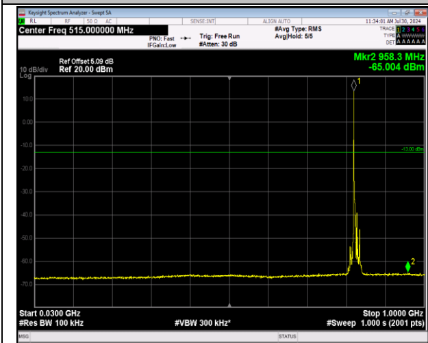
5-5-3MHz-5MHz-64QAM-64QAM-20416-20455-1RB#0-0RB#0-30~1000MHz-PASS
