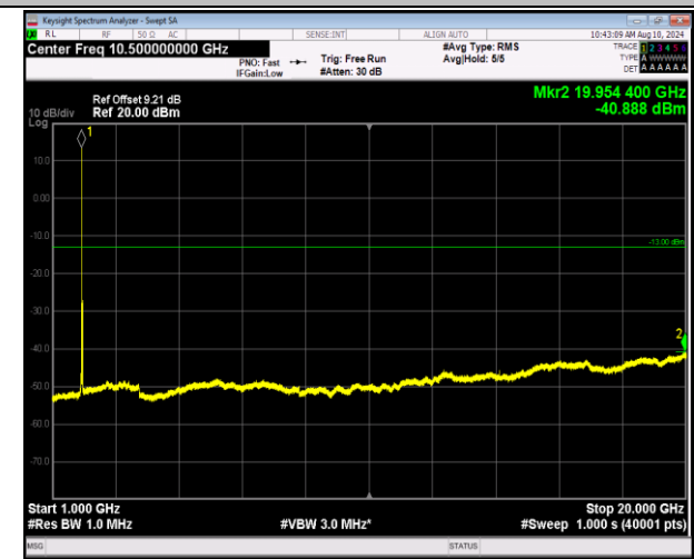
2-2-20MHz-20MHz-16QAM-16QAM-18902-19100-1RB#0-1 RB#99-1000~20000MHz-PASS
