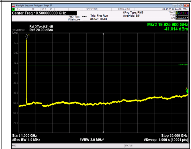
2-2-5MHz-20MHz-16QAM-16QAM-18983-19100-1RB#0-1RB#99-1000~20000MHz-PASS
