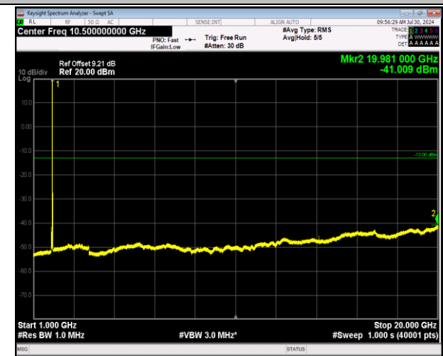
2-2-5MHz-20MHz-64QAM-64QAM-18983-19100-1RB#0-OR B#0-1000~20000MHz-PASS
