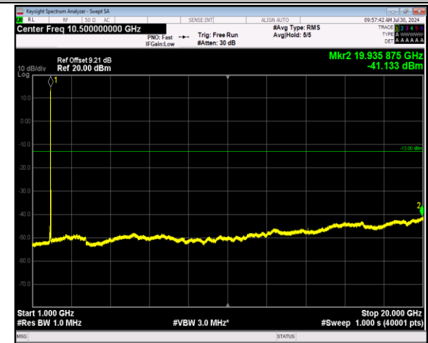
2-2-5MHz-20MHz-64QAM-64QAM-18983-19100-1RB#0-1R B#99-1000~20000MHz-PASS
