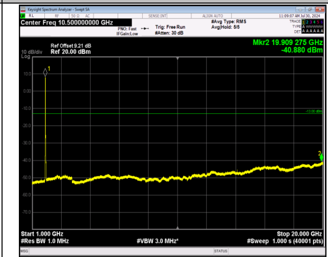
2-2-20MHz-20MHz-64QAM-64QAM-18801-18999-100RB#0 -100RB#0-1000~20000MHz-PASS
