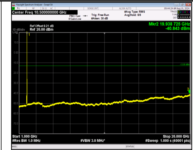
2-2-5MHz-20MHz-16QAM-16QAM-18983-19100-1RB#0-0RB#0-1000~20000MHz-PASS
