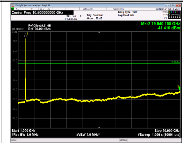
2-2-5MHz-20MHz-16QAM-16QAM-18808-18925-1RB#0-1RB#99-1000~20000MHz-PASS
