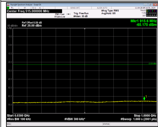
2-2-20MHz-20MHz-64QAM-64QAM-18700-18898-1RB#0-0RB#0-30~1000MHz-PASS
