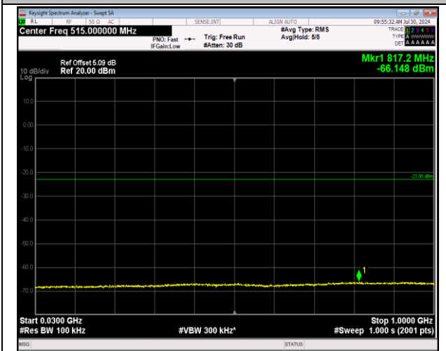
2-2-5MHz-20MHz-64QAM-64QAM-18808-18925-25RB#0 -100RB#0-30~1000MHz-PASS
