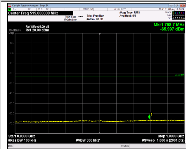
2-2-5MHz-20MHz-16QAM-16QAM-18808-18925-1RB#0-1RB#99-30~1000MHz-PASS
