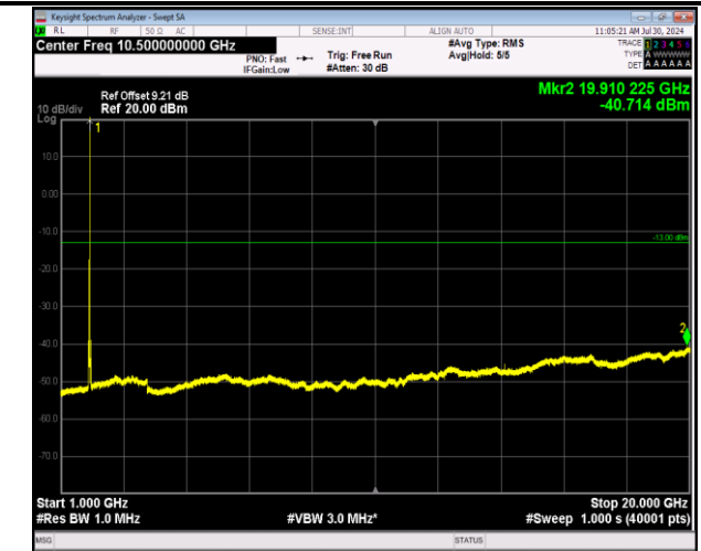
2-2-20MHz-20MHz-64QAM-64QAM-18700-18898-1RB#99- ORB#0-1000~20000MHz-PASS
