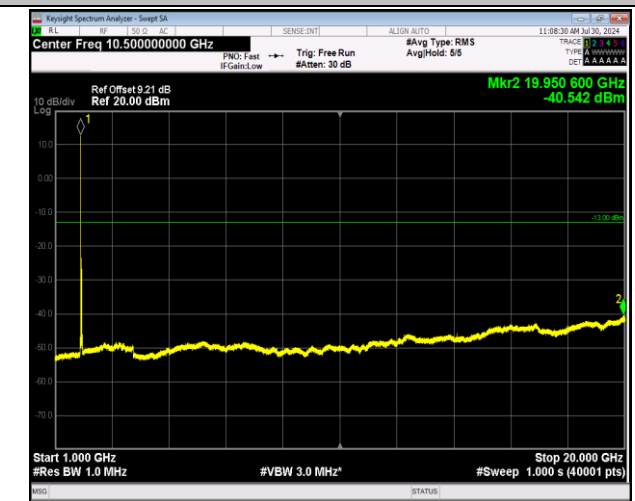
2-2-20MHz-20MHz-64QAM-64QAM-18801-18999-1RB#0-1 RB#99-1000~20000MHz-PASS
