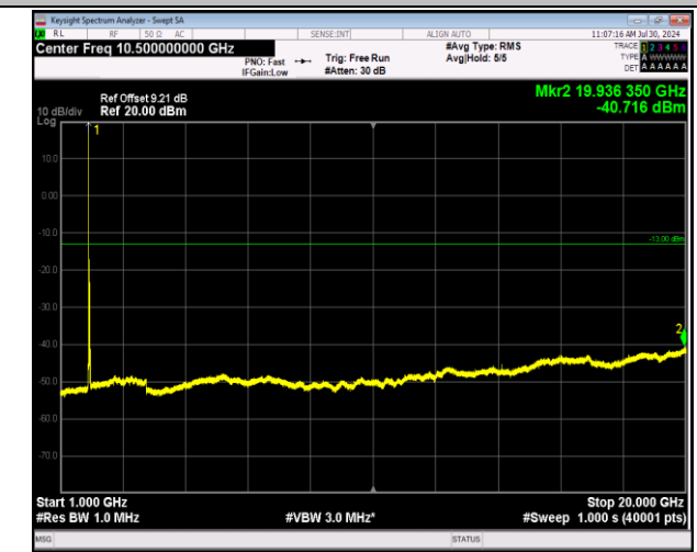
2-2-20MHz-20MHz-64QAM-64QAM-18801-18999-1RB#0-0 RB#0-1000~20000MHz-PASS
