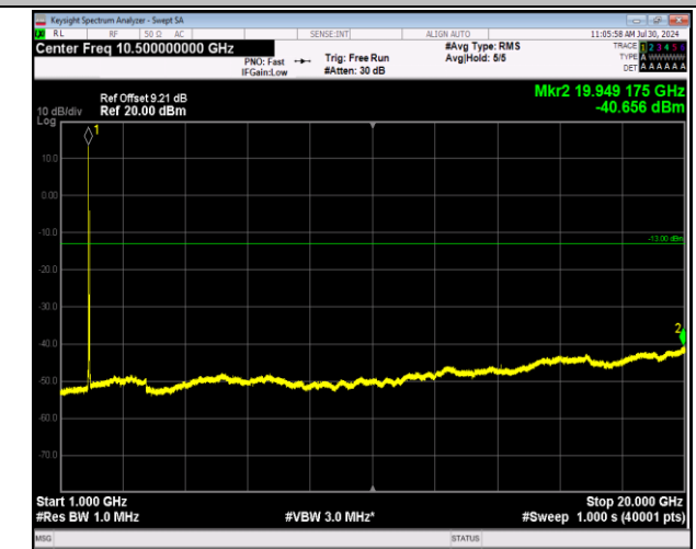
2-2-20MHz-20MHz-64QAM-64QAM-18700-18898-1RB#0-1RB#99-1000~20000MHz-PASS
