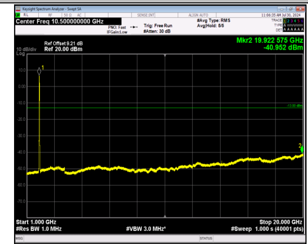
2-2-20MHz-20MHz-64QAM-64QAM-18700-18898-100RB#0 -100RB#0-1000~20000MHz-PASS
