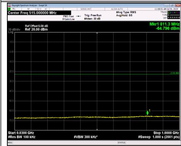
2-2-20MHz-20MHz-64QAM-64QAM-18801-18999-100RB #0-100RB#0-30~1000MHz-PASS
