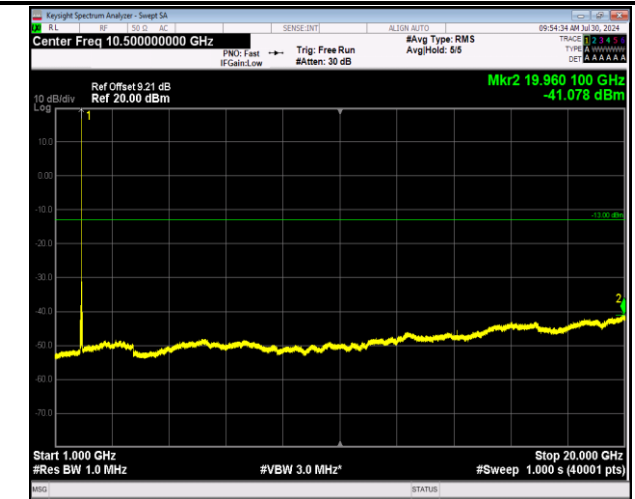
2-2-5MHz-20MHz-64QAM-64QAM-18808-18925-1RB#24-0 RB#0-1000~20000MHz-PASS
