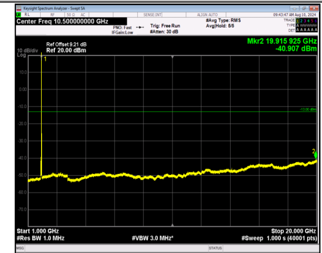
2-2-5MHz-20MHz-QPSK-QPSK-18983-19100-1RB#0-0RB#0 0-1000~20000MHz-PASS
