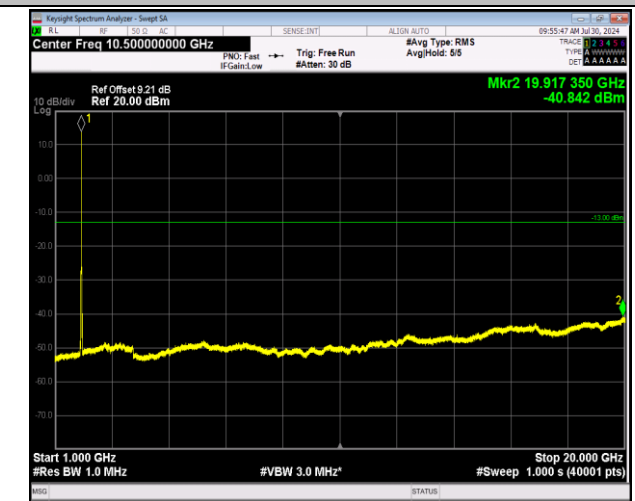
2-2-5MHz-20MHz-64QAM-64QAM-18808-18925-25RB#0-1 00RB#0-1000~20000MHz-PASS
