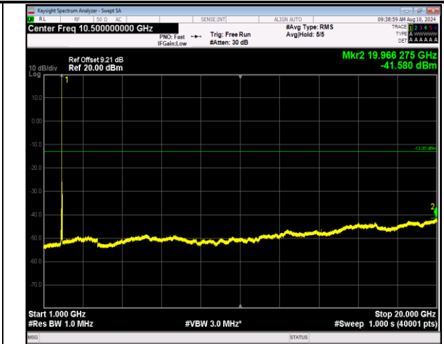
2-2-5MHz-20MHz-16QAM-16QAM-18808-18925-1RB#0-0RB#0-1000~20000MHz-PASS
