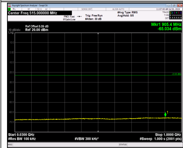
2-2-20MHz-20MHz-64QAM-64QAM-18801-18999-1RB#0 -0RB#0-30~1000MHz-PASS
