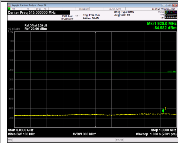
2-2-20MHz-20MHz-64QAM-64QAM-18700-18898-100RB #0-100RB#0-30~1000MHz-PASS
