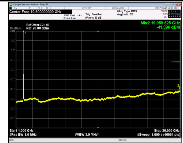
2-2-5MHz-20MHz-64QAM-64QAM-18983-19100-1RB#24-0 RB#0-1000~20000MHz-PASS
