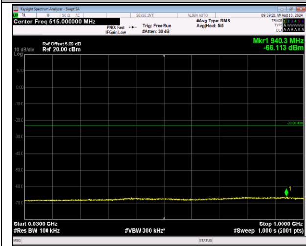
2-2-5MHz-20MHz-QPSK-QPSK-18808-18925-1RB#24-0 RB#0-30~1000MHz-PASS
