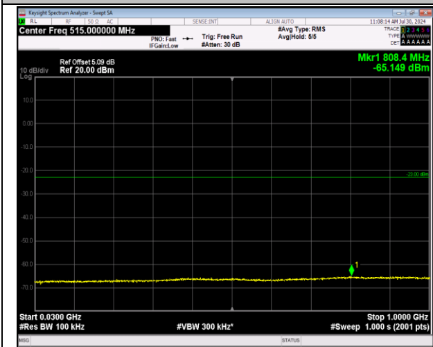
2-2-20MHz-20MHz-64QAM-64QAM-18801-18999-1RB#0 -1RB#99-30~1000MHz-PASS
