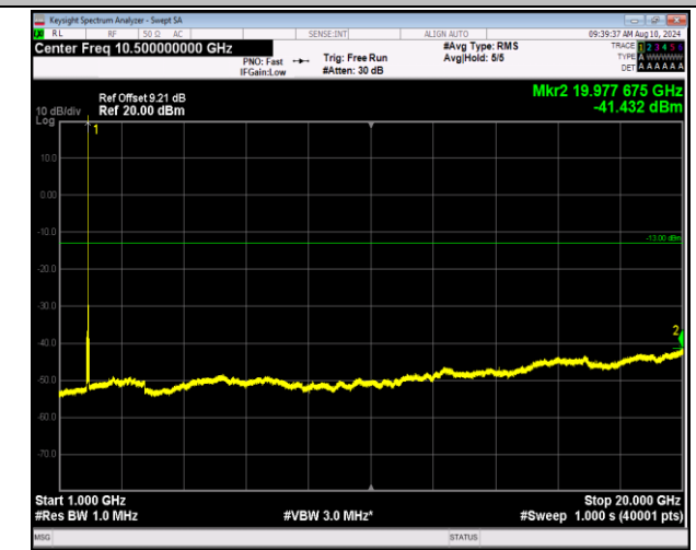
2-2-5MHz-20MHz-QPSK-QPSK-18808-18925-1RB#24-ORB #0-1000~20000MHz-PASS
