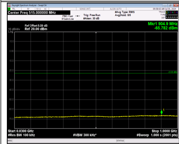
2-2-5MHz-20MHz-64QAM-64QAM-18983-19100-25RB#0 -100RB#0-30~1000MHz-PASS
