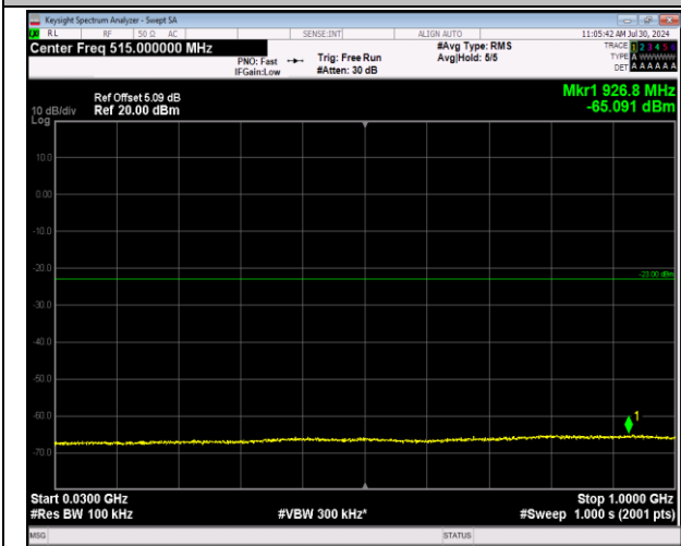
2-2-20MHz-20MHz-64QAM-64QAM-18700-18898-1RB#0-1RB#99-30~1000MHz-PASS
