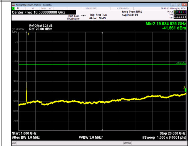
2-2-5MHz-20MHz-16QAM-16QAM-18808-18925-1RB#24-0RB#0-1000~20000MHz-PASS
