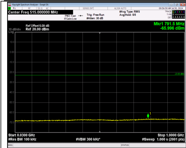
2-2-5MHz-20MHz-64QAM-64QAM-18983-19100-1RB#24 -0RB#0-30~1000MHz-PASS
