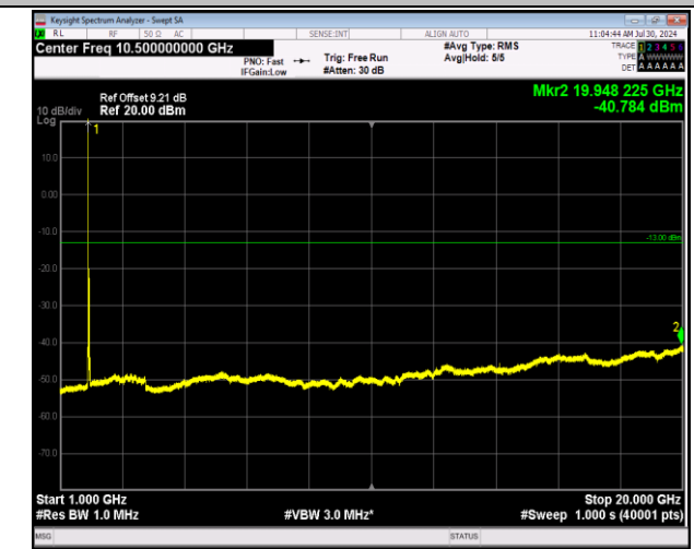
2-2-20MHz-20MHz-64QAM-64QAM-18700-18898-1RB#0-0RB#0-1000~20000MHz-PASS
