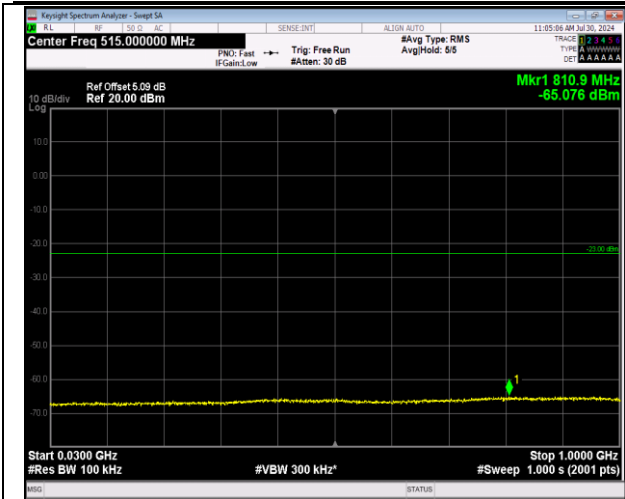
2-2-20MHz-20MHz-64QAM-64QAM-18700-18898-1RB#9 9-ORB#0-30~1000MHz-PASS
