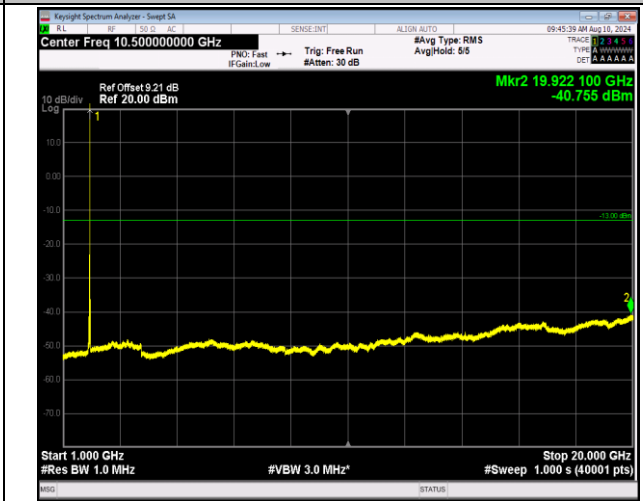
2-2-5MHz-20MHz-16QAM-16QAM-18983-19100-1RB#24-0RB#0-1000~20000MHz-PASS
