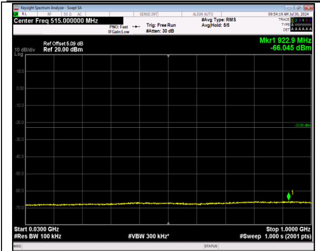
2-2-5MHz-20MHz-64QAM-64QAM-18808-18925-1RB#24 -0RB#0-30~1000MHz-PASS
