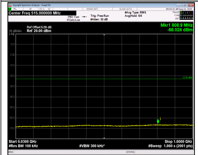
2-2-5MHz-20MHz-QPSK-QPSK-18983-19100-1RB#0-0R B#0-30~1000MHz-PASS
