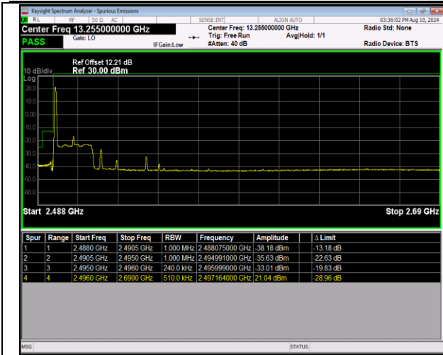
41-41-20MHz-5MHz-16QAM@16QAM-16QAM@16QAM-39750-39867-1RB#0@100RB#0-0RB#0@25RB#0-PASS
