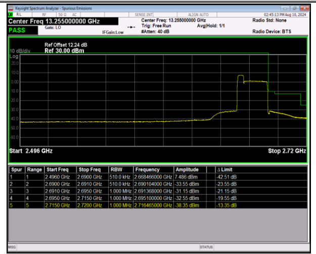
41-41-5MHz-20MHz-16QAM@16QAM-16QAM@16QAM-41373-41490-25RB#0@25RB#0-100RB#0@100RB#0-PAS
