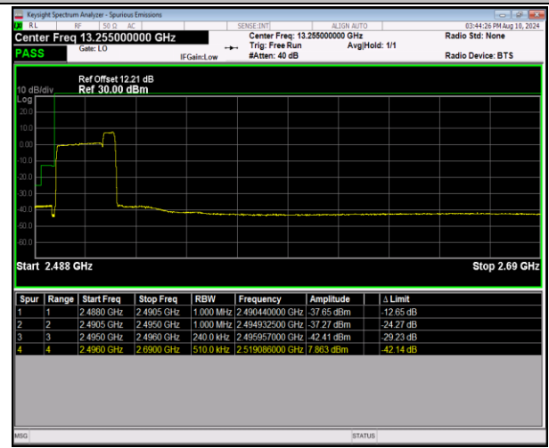
41-41-20MHz-5MHz-16QAM@16QAM-16QAM@16QAM-39750-39867-100RB#0@100RB#0-25RB#0@25RB#0-PAS
