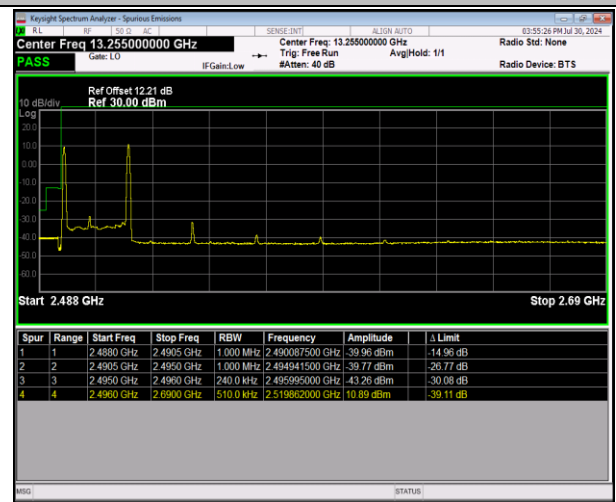
41-41-20MHz-5MHz-64QAM@64QAM-64QAM@64QAM-39750-39867-1RB#0@100RB#0-1RB#24@25RB#0-PASS
