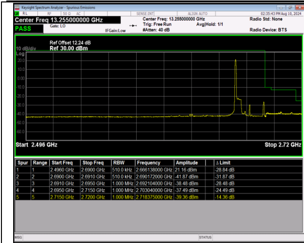
41-41-5MHz-20MHz-16QAM@16QAM-16QAM@16QAM-41373-41490-1RB#0@25RB#0-0RB#0@100RB#0-PASS
