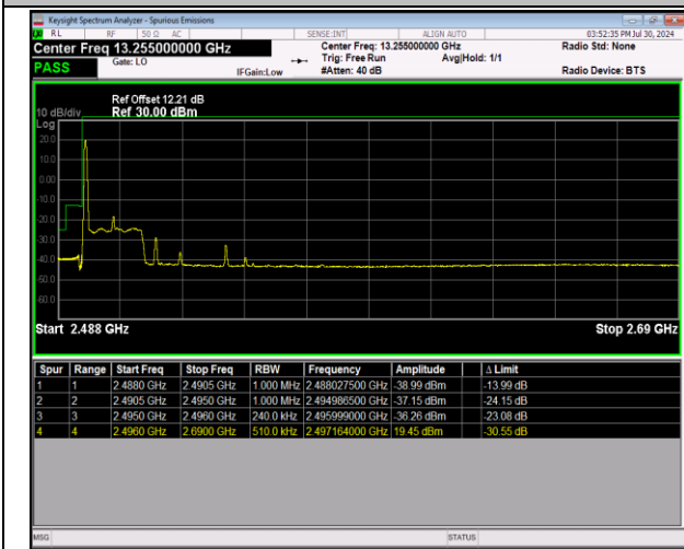
41-41-20MHz-5MHz-64QAM@64QAM-64QAM@64QAM-39750-39867-1RB#0@100RB#0-0RB#0@25RB#0-PASS
