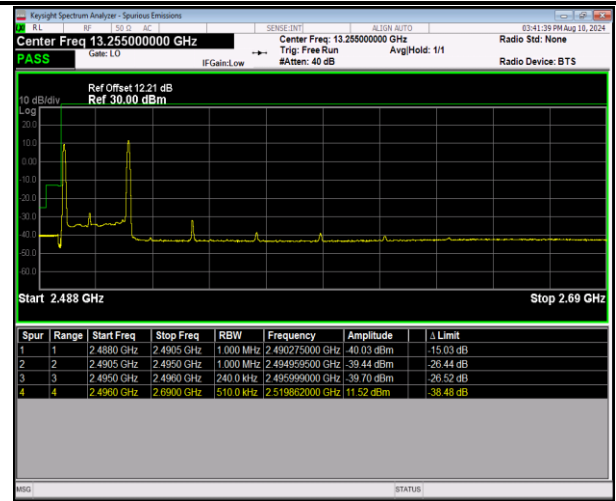
41-41-20MHz-5MHz-16QAM@16QAM-16QAM@16QAM-39750-39867-1RB#0@100RB#0-1RB#24@25RB#0-PASS
