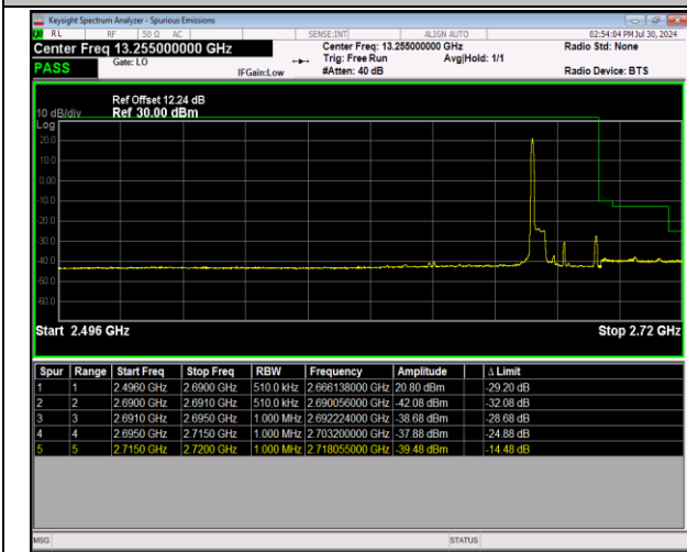
41-41-5MHz-20MHz-64QAM@64QAM-64QAM@64QAM-41373-41490-1RB#0@25RB#0-0RB#0@100RB#0-PASS
