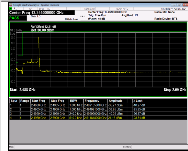
41-41-20MHz-5MHz-16QAM@16QAM-16QAM@16QAM-39750-39867-1RB#99@100RB#0-0RB#0@25RB#0-PAS
