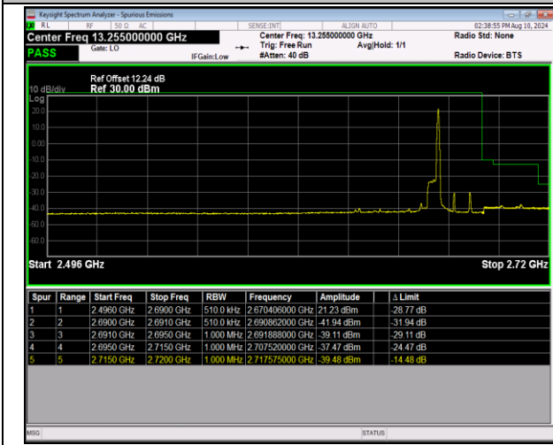
41-41-5MHz-20MHz-16QAM@16QAM-16QAM@16QAM-41373-41490-1RB#24@25RB#0-0RB#0@100RB#0-PAS
