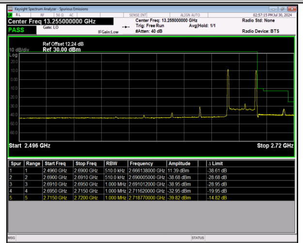
41-41-5MHz-20MHz-64QAM@64QAM-64QAM@64QAM-41373-41490-1RB#0@25RB#0-1RB#99@100RB#0-PASS
