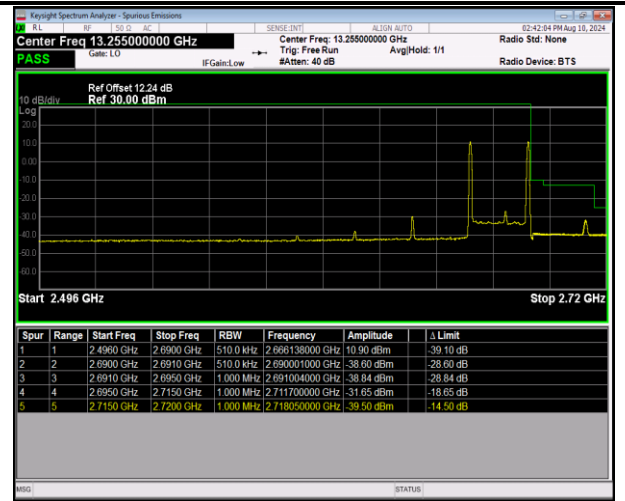
41-41-5MHz-20MHz-16QAM@16QAM-16QAM@16QAM-41373-41490-1RB#0@25RB#0-1RB#99@100RB#0-PASS
