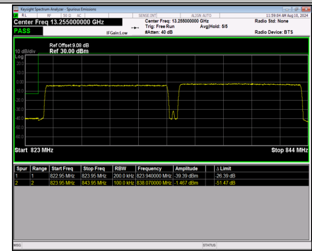
5-5-10MHz-10MHz-QPSK@QPSK-QPSK@QPSK-20450-20549-50RB#0@50RB#0-50RB#0@50RB#0-PASS
