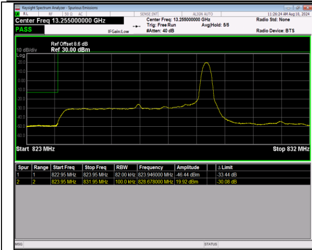
5-5-5MHz-3MHz-16QAM@16QAM-16QAM@16QAM-204 25-20464-1RB#24@25RB#0-0RB#0@15RB#0-PASS
