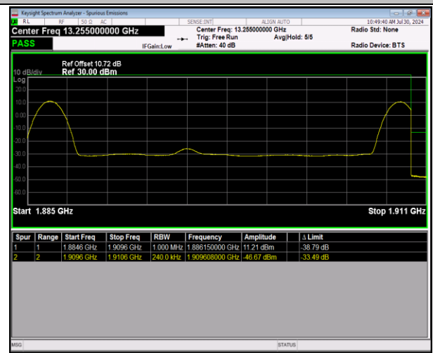
2-2-20MHz-5MHz-64QAM@64QAM-64QAM@64QAM-19050-19167-1RB#0@100RB#0-1RB#24@25RB#0-PASS
