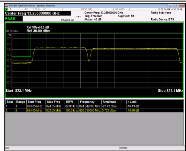
5-5-3MHz-5MHz-64QAM@64QAM-64QAM@64QAM-2041 6-20455-15RB#0@15RB#0-25RB#0@25RB#0-PASS
