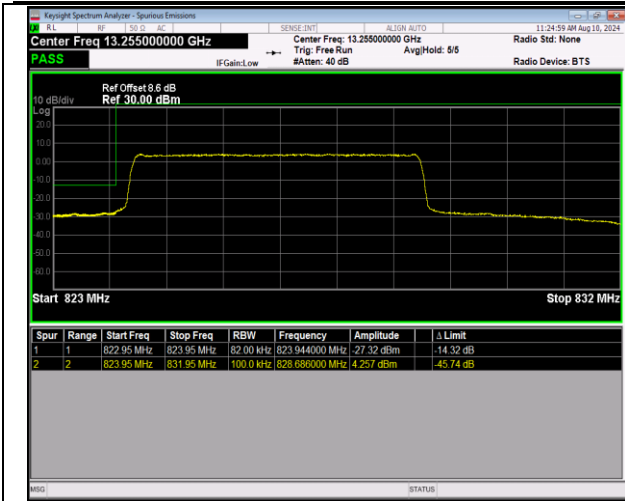
5-5-5MHz-3MHz-QPSK@QPSK-QPSK@QPSK-20425-20 464- 1RB#0@25RB#0-0RB#0@15RB#0-PASS
