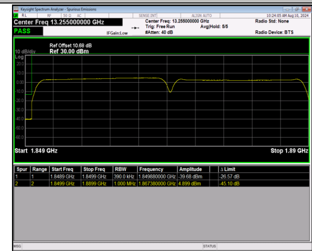
2-2-20MHz-20MHz-QPSK@QPSK-QPSK@QPSK-18700-18898-100RB#0@100RB#0-100RB#0@100RB#0-PASS
