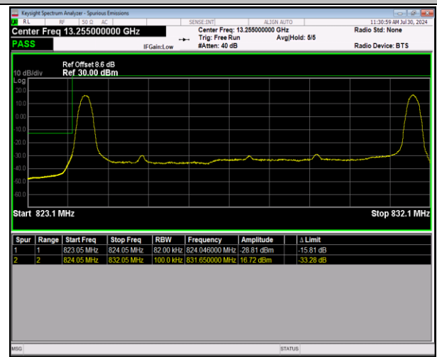
5-5-3MHz-5MHz-64QAM@64QAM-64QAM@64QAM-2041 6-20455-1RB#0@15RB#0-1RB#24@25RB#0-PASS
