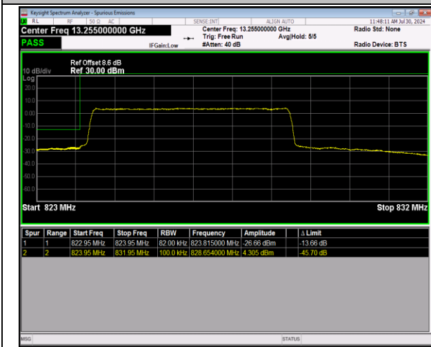
5-5-5MHz-3MHz-64QAM@64QAM-64QAM@64QAM-204 25-20464-1RB#0@25RB#0-0RB#0@15RB#0-PASS
