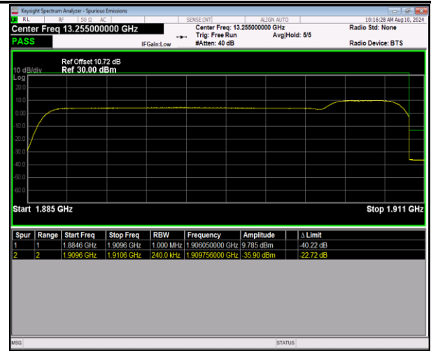
2-2-20MHz-5MHz-16QAM@16QAM-16QAM@16QAM-19050-19167-100RB#0@100RB#0-25RB#0@25RB#0-PASS
