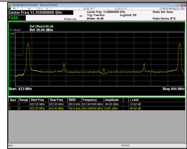
5-5-10MHz-10MHz-16QAM@16QAM-16QAM@16QAM-20450-20549-1RB#0@50RB#0-1RB#49@50RB#0-PASS
