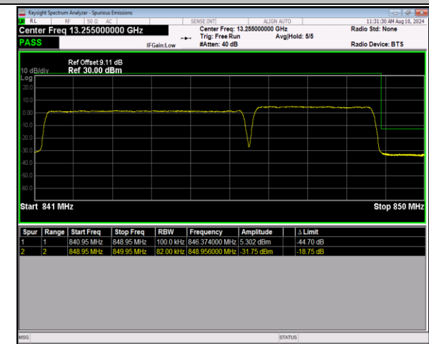
5-5-5MHz-3MHz-QPSK@QPSK-QPSK@QPSK-20595-206 34-25RB#0@25RB#0-15RB#0@15RB#0-PASS
