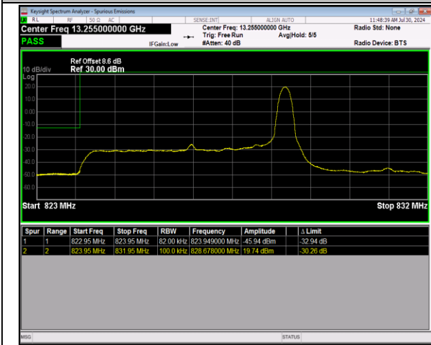
5-5-5MHz-3MHz-64QAM@64QAM-64QAM@64QAM-204 25-20464-1RB#24@25RB#0-0RB#0@15RB#0-PASS
