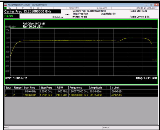
2-2-20MHz-5MHz-64QAM@64QAM-64QAM@64QAM-19050-19167-100RB#0@100RB#0-25RB#0@25RB#0-PASS
