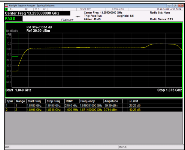
2-2-20MHz-5MHz-64QAM@64QAM-64QAM@64QAM-18700-18817-100RB#0@100RB#0-25RB#0@25RB#0-PASS
