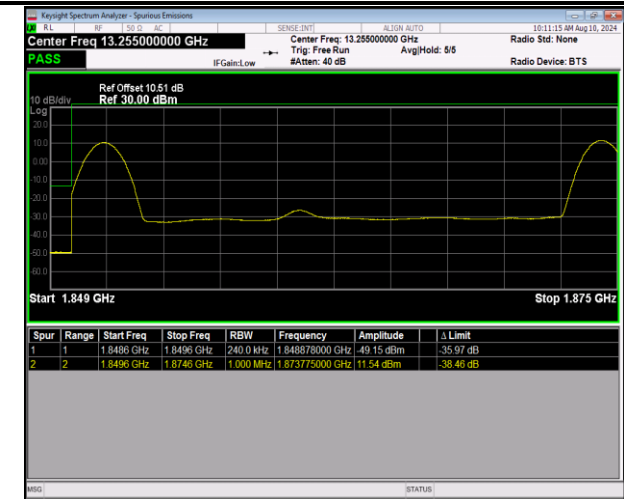
2-2-20MHz-5MHz-QPSK@QPSK-QPSK@QPSK-18700-18 817-1RB#0@100RB#0-1RB#24@25RB#0-PASS
