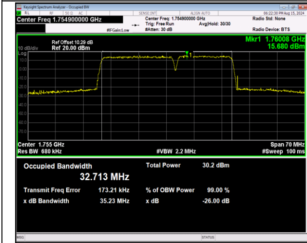
66-66-20MHz-15MHz-16QAM-16QAM-132348-132519-10 ORB#0-75RB#0-PASS
