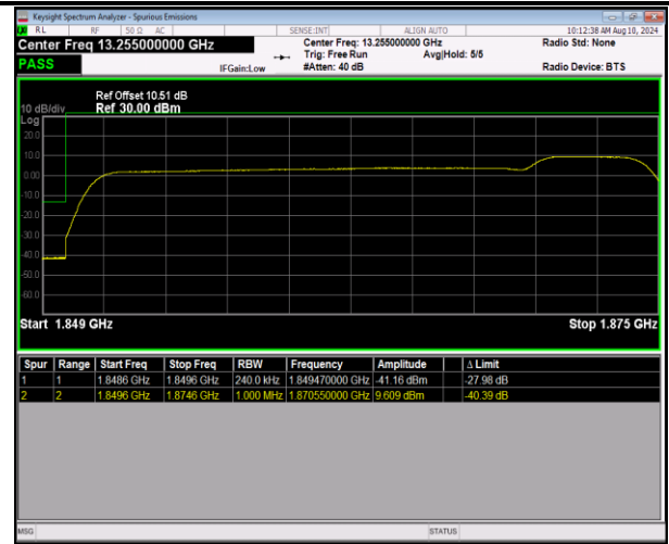
2-2-20MHz-5MHz-16QAM@16QAM-16QAM@16QAM-18700-18817-100RB#0@100RB#0-25RB#0@25RB#0-PASS
