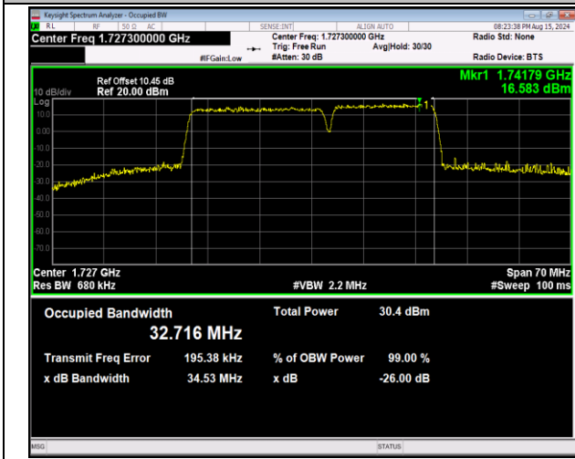
66-66-20MHz-15MHz-64QAM-64QAM-132072-132243-10 ORB#0-75RB#0-PASS
