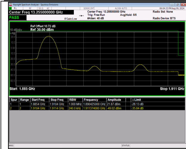
2-2-5MHz-20MHz-16QAM@16QAM-16QAM@16QAM-18 983-19100-1RB#24@25RB#0-0RB#0@100RB#0-PASS
