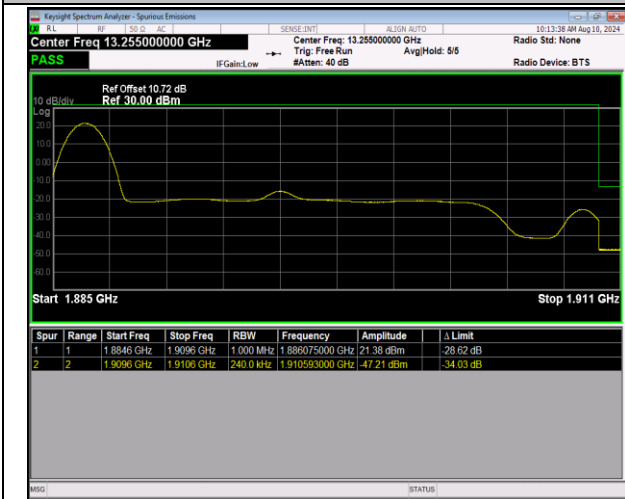
2-2-20MHz-5MHz-16QAM@16QAM-16QAM@16QAM-19050-19167-1RB#0@100RB#0-0RB#0@25RB#0-PASS
