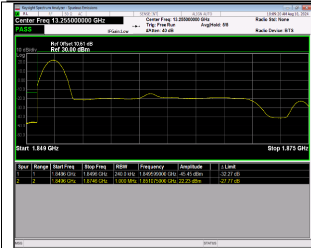
2-2-20MHz-5MHz-QPSK@QPSK-QPSK@QPSK-18700-1 8817-1RB#0@100RB#0-0RB#0@25RB#0-PASS
