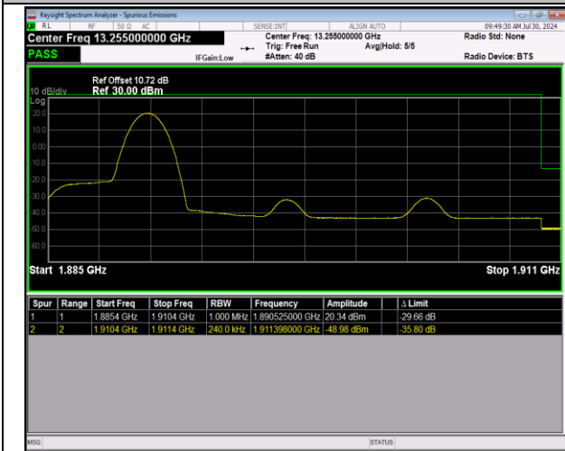
2-2-5MHz-20MHz-64QAM@64QAM-64QAM@64QAM-18 983-19100-1RB#24@25RB#0-0RB#0@100RB#0-PASS
