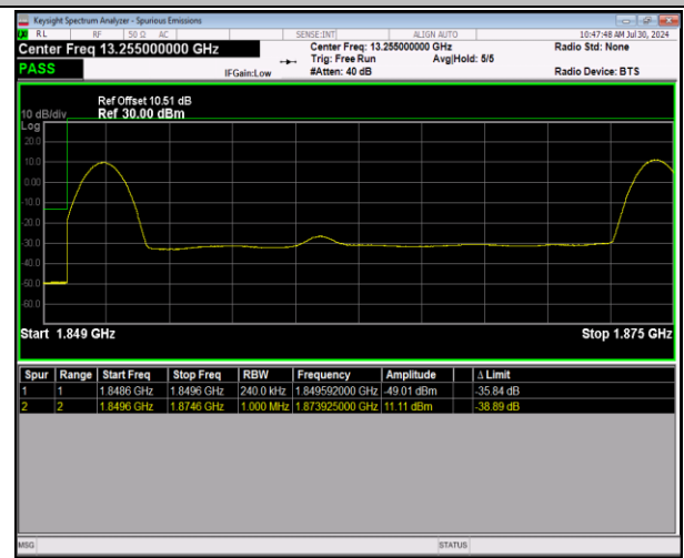
2-2-20MHz-5MHz-64QAM@64QAM-64QAM@64QAM-18700-18817-1RB#0@100RB#0-1RB#24@25RB#0-PASS
