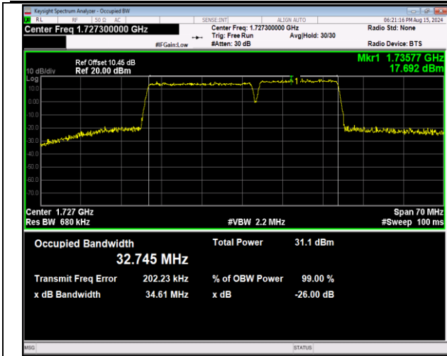
66-66-20MHz-15MHz-QPSK-QPSK-132072-132243-100R B#0-75RB#0-PASS
