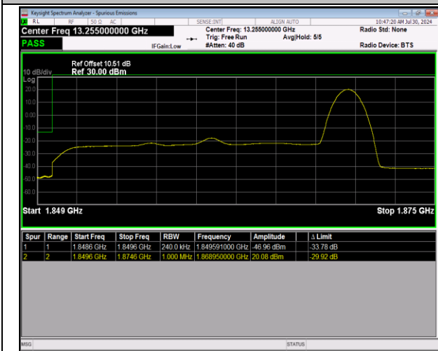
2-2-20MHz-5MHz-64QAM@64QAM-64QAM@64QAM-18700-18817-1RB#99@100RB#0-0RB#0@25RB#0-PASS
