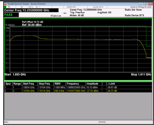
2-2-5MHz-20MHz-16QAM@16QAM-16QAM@16QAM-189 83-19100-25RB#0@25RB#0-100RB#0@100RB#0-PASS
