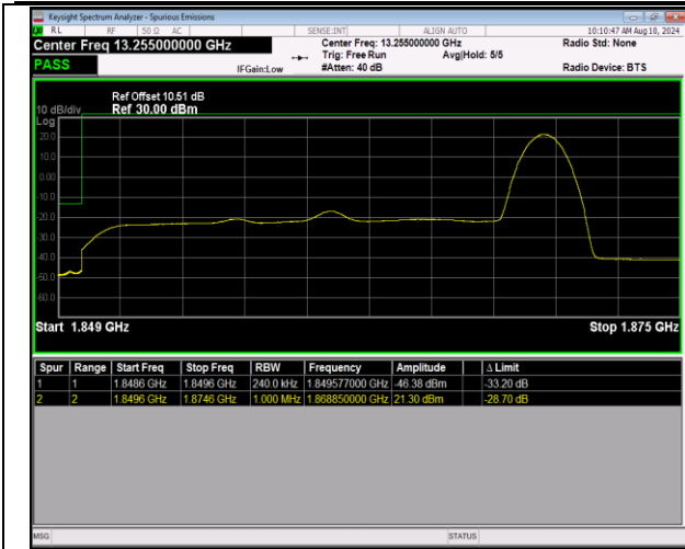
2-2-20MHz-5MHz-16QAM@16QAM-16QAM@16QAM-18700-18817-1RB#99@100RB#0-0RB#0@25RB#0-PASS
