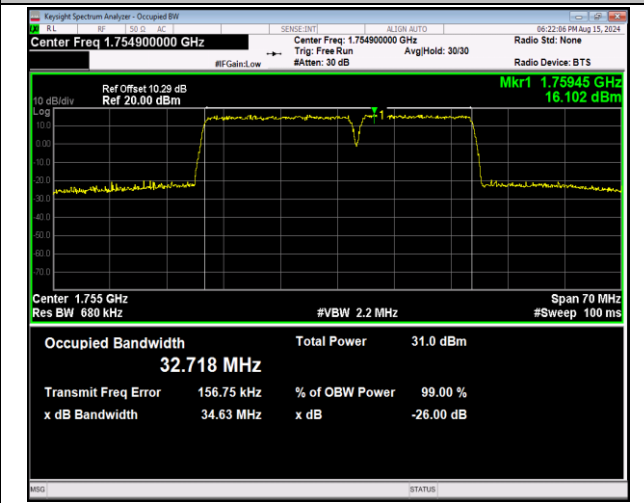
66-66-20MHz-15MHz-QPSK-QPSK-132348-132519-100R B#0-75RB#0-PASS
