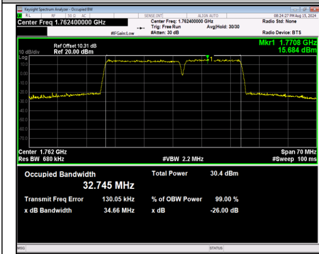
66-66-20MHz-15MHz-64QAM-64QAM-132423-132594-10 ORB#0-75RB#0-PASS
