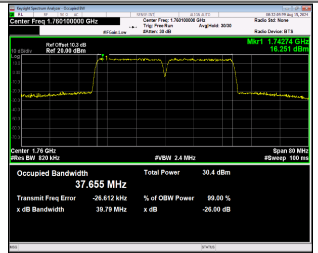
66-66-20MHz-20MHz-64QAM-64QAM-132374-132572-10 ORB#0-100RB#0-PASS
