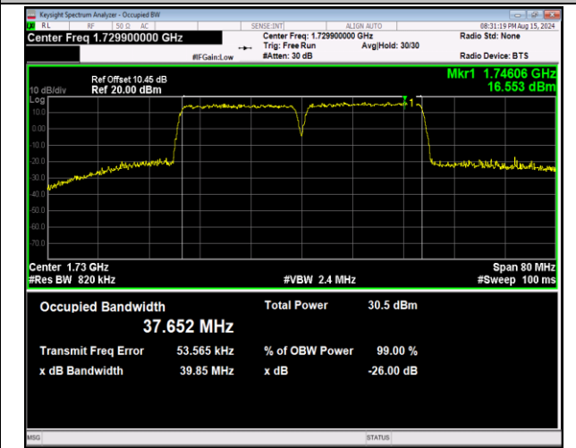
66-66-20MHz-20MHz-64QAM-64QAM-132072-132270-10 ORB#0-100RB#0-PASS
