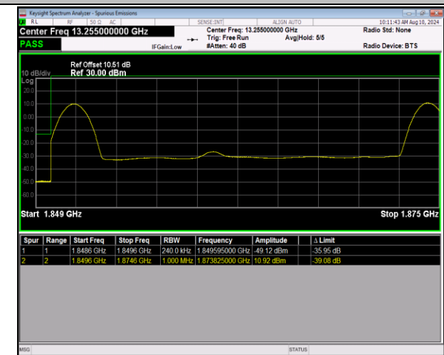
2-2-20MHz-5MHz-16QAM@16QAM-16QAM@16QAM-18 00-18817-1RB#0@100RB#0-1RB#24@25RB#0-PASS
