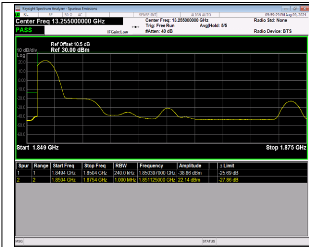
2-2-5MHz-20MHz-QPSK@QPSK-QPSK@QPSK-18633-1 8750-1RB#0@25RB#0-0RB#0@100RB#0-PASS
