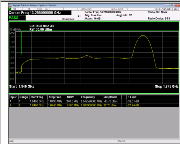
2-2-20MHz-5MHz-QPSK@QPSK-QPSK@QPSK-18700-1 8817-1RB#99@100RB#0-0RB#0@25RB#0-PASS
