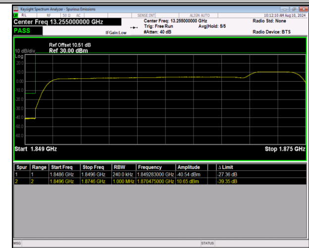
2-2-20MHz-5MHz-QPSK@QPSK-QPSK@QPSK-18700-18 817-100RB#0@100RB#0-25RB#0@25RB#0-PASS
