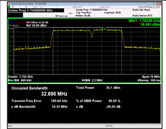
66-66-20MHz-15MHz-64QAM-64QAM-132348-132519-10 ORB#0-75RB#0-PASS
