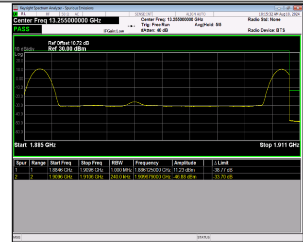
2-2-20MHz-5MHz-16QAM@16QAM-16QAM@16QAM-19050-19167-1RB#0@100RB#0-1RB#24@25RB#0-PASS
