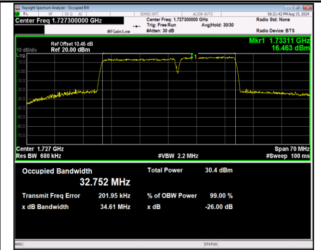
66-66-20MHz-15MHz-16QAM-16QAM-132072-132243-10 ORB#0-75RB#0-PASS
