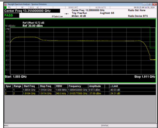
2-2-5MHz-20MHz-64QAM@64QAM-64QAM@64QAM-189 83-19100-25RB#0@25RB#0-100RB#0@100RB#0-PASS
