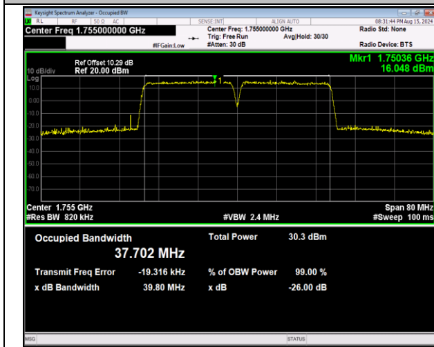
66-66-20MHz-20MHz-64QAM-64QAM-132323-132521-10 ORB#0-100RB#0-PASS
