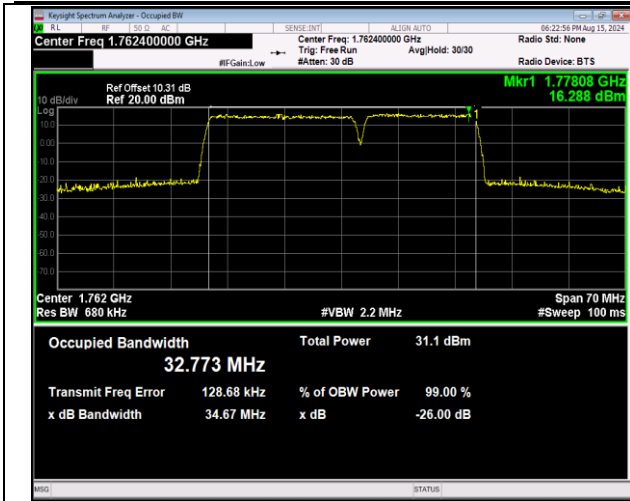
66-66-20MHz-15MHz-QPSK-QPSK-132423-132594-100R B#0-75RB#0-PASS
