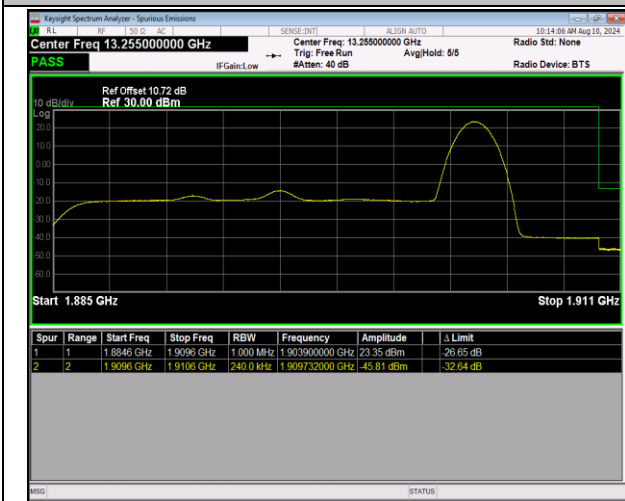
2-2-20MHz-5MHz-QPSK@QPSK-QPSK@QPSK-19050-19167-1RB#99@100RB#0-0RB#0@25RB#0-PASS
