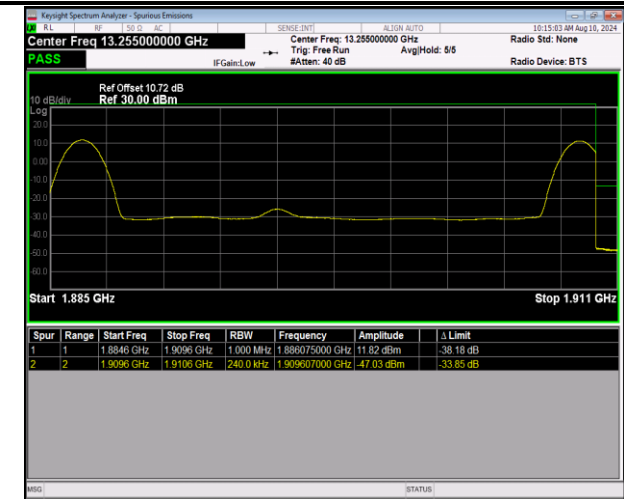
2-2-20MHz-5MHz-QPSK@QPSK-QPSK@QPSK-19050-19167-1RB#0@100RB#0-1RB#24@25RB#0-PASS
