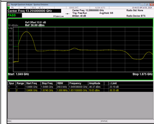
2-2-20MHz-5MHz-64QAM@64QAM-64QAM@64QAM-18700-18817-1RB#0@100RB#0-0RB#0@25RB#0-PASS
