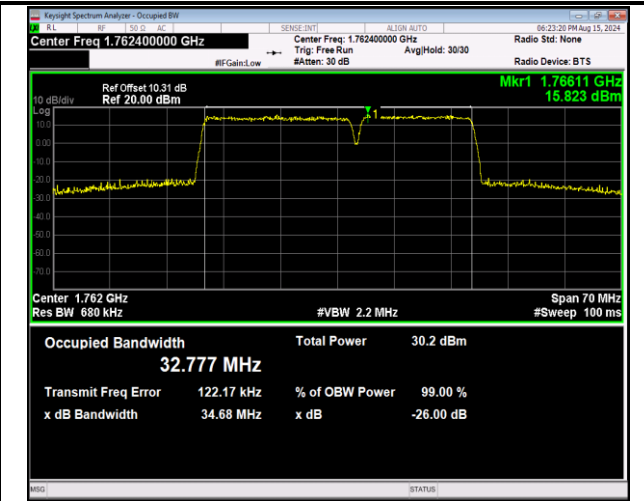
66-66-20MHz-15MHz-16QAM-16QAM-132423-132594-10 ORB#0-75RB#0-PASS
