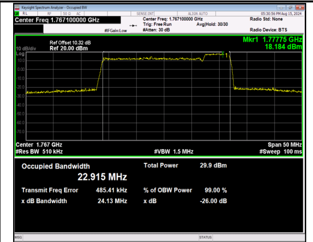
66-66-20MHz-5MHz-16QAM-16QAM-132522-132639-100RB#0-25RB#0-PASS
