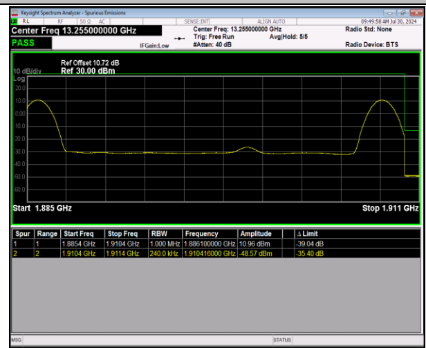
2-2-5MHz-20MHz-64QAM@64QAM-64QAM@64QAM-189 83-19100-1RB#0@25RB#0-1RB#99@100RB#0-PASS
