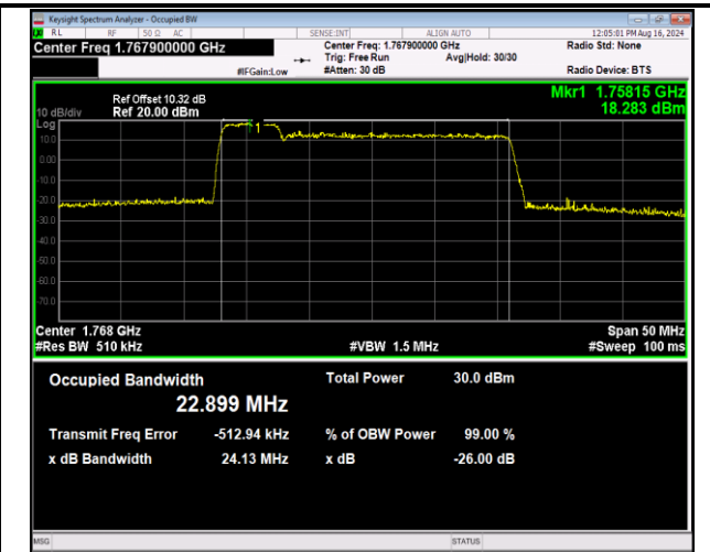
66-66-5MHz-20MHz-16QAM-16QAM-132455-132572-25RB#0-100RB#0-PASS
