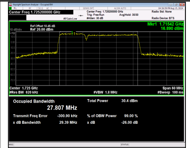
66-66-10MHz-20MHz-16QAM-16QAM-132027-132171-50RB #0-100RB#0-PASS
