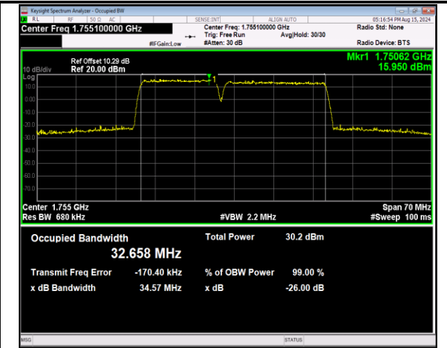
66-66-15MHz-20MHz-16QAM-16QAM-132325-132496-75RB #0-100RB#0-PASS
