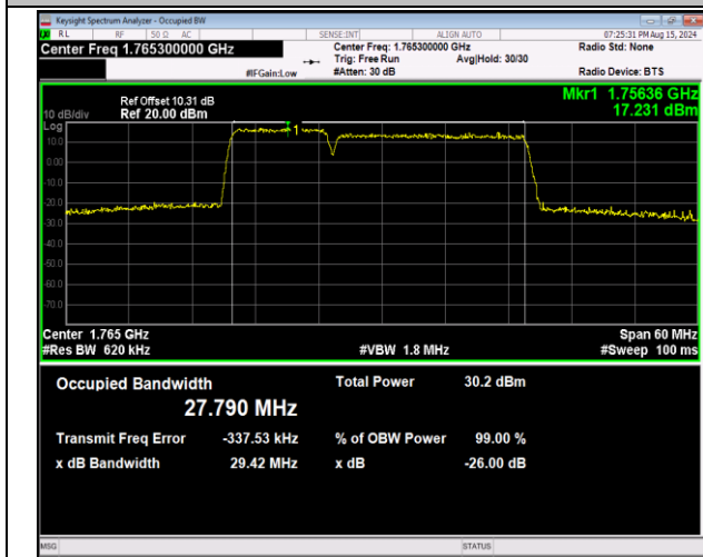
66-66-10MHz-20MHz-64QAM-64QAM-132428-132572-50RB #0-100RB#0-PASS
