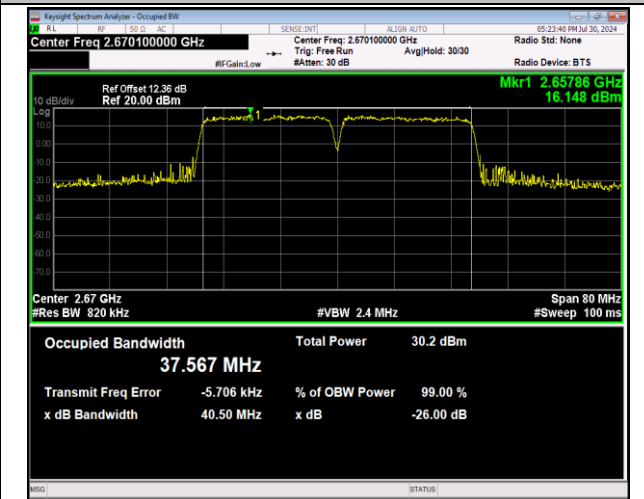
41-41-20MHz-20MHz-64QAM-64QAM-41292-41490-100R B#0-100RB#0-PASS
