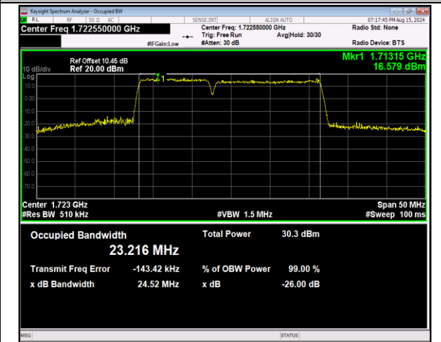
66-66-10MHz-15MHz-64QAM-64QAM-132025-132145-50RB#0-75RB#0-PASS
