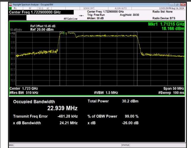
66-66-5MHz-20MHz-16QAM-16QAM-132005-132122-25R B#0-100RB#0-PASS
