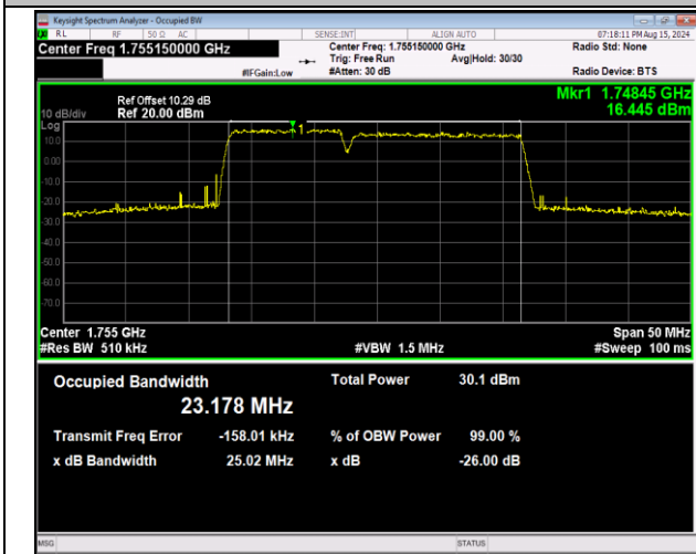
66-66-10MHz-15MHz-64QAM-64QAM-132351-132471-50RB #0-75RB#0-PASS
