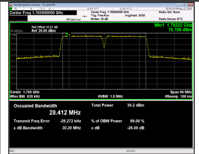
66-66-15MHz-15MHz-16QAM-16QAM-132447-132597-75RB #0-75RB#0-PASS
