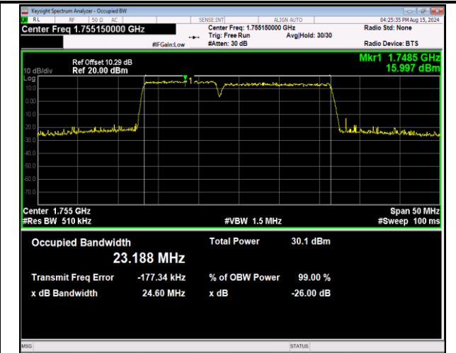
66-66-10MHz-15MHz-16QAM-16QAM-132351-132471-50RB #0-75RB#0-PASS
