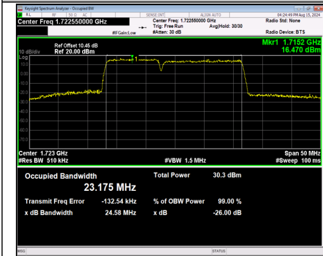
66-66-10MHz-15MHz-16QAM-16QAM-132025-132145-50RB#0-75RB#0-PASS
