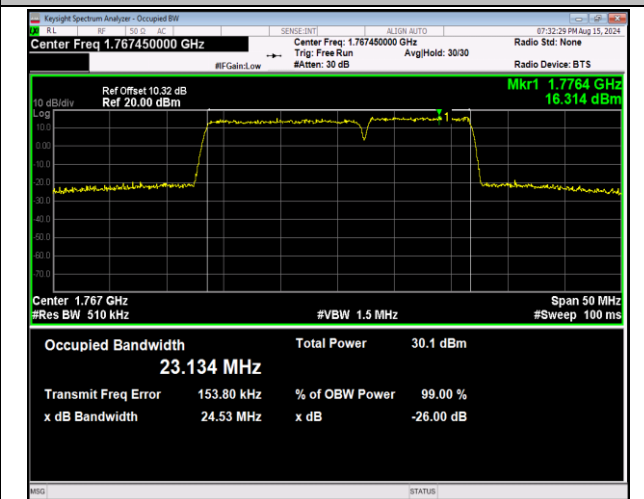
66-66-15MHz-10MHz-64QAM-64QAM-132499-132619-75RB #0-50RB#0-PASS
