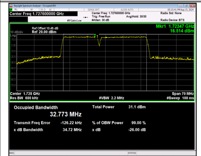
66-66-15MHz-20MHz-QPSK-QPSK-132050-132221-75RB #0-100RB#0-PASS
