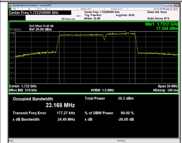
66-66-15MHz-10MHz-64QAM-64QAM-132047-132167-75RB #0-50RB#0-PASS
