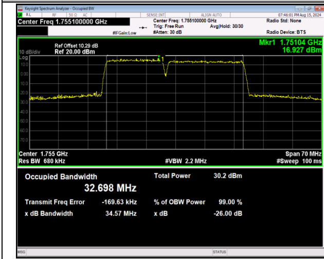
66-66-15MHz-20MHz-64QAM-64QAM-132325-132496-75RB #0-100RB#0-PASS
