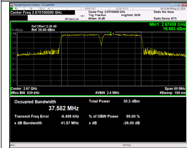
41-41-20MHz-20MHz-16QAM-16QAM-41292-41490-100R B#0-100RB#0-PASS
