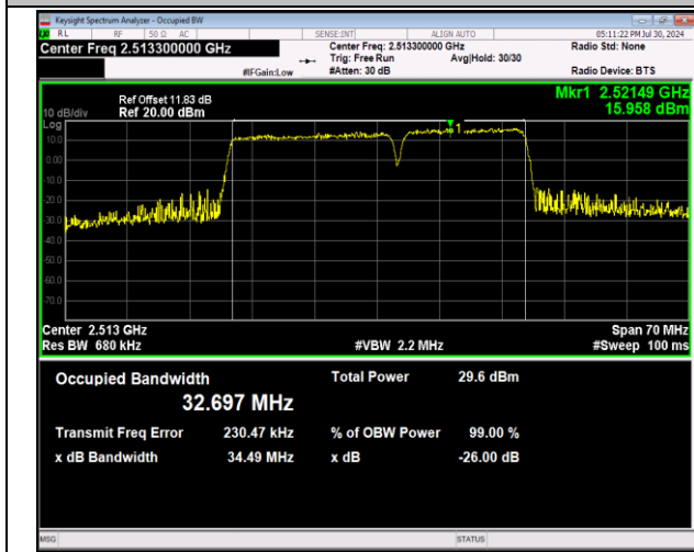
41-41-20MHz-15MHz-64QAM-64QAM-39750-39921-100R B#0-75RB#0-PASS
