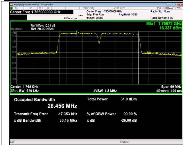
66-66-15MHz-15MHz-QPSK-QPSK-132447-132597-75RB #0-75RB#0-PASS
