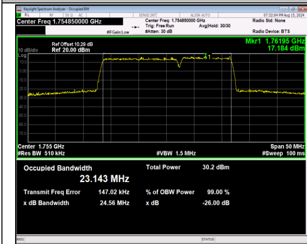
66-66-15MHz-10MHz-64QAM-64QAM-132373-132493-75RB #0-50RB#0-PASS
