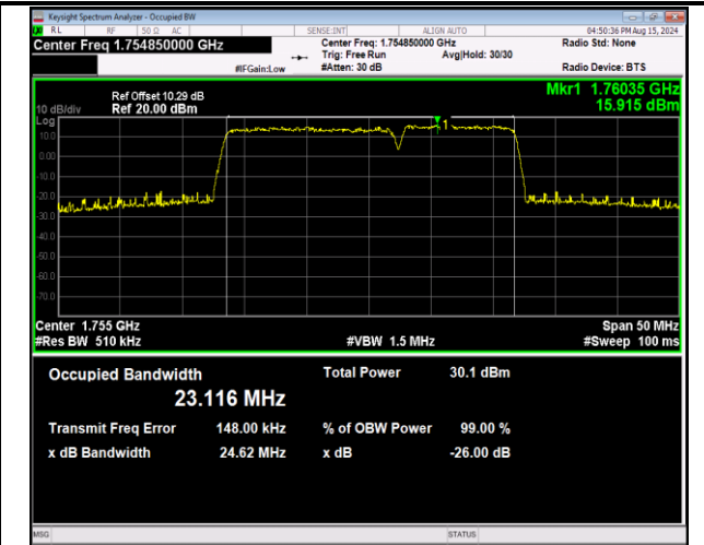
66-66-15MHz-10MHz-16QAM-16QAM-132373-132493-75RB #0-50RB#0-PASS
