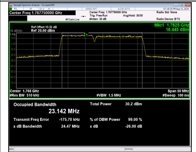
66-66-10MHz-15MHz-64QAM-64QAM-132477-132597-50RB #0-75RB#0-PASS
