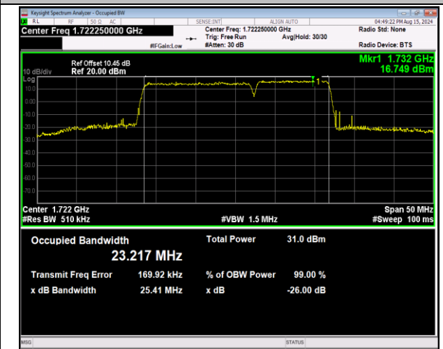
66-66-15MHz-10MHz-QPSK-QPSK-132047-132167-75RB #0-50RB#0-PASS
