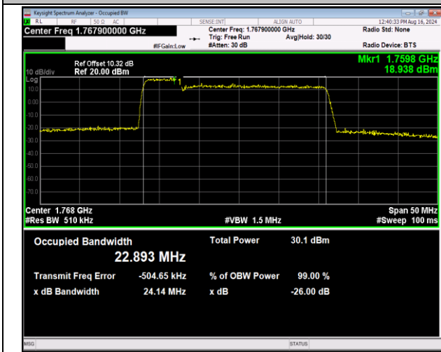
66-66-5MHz-20MHz-64QAM-64QAM-132455-132572-25RB#0-100RB#0-PASS
