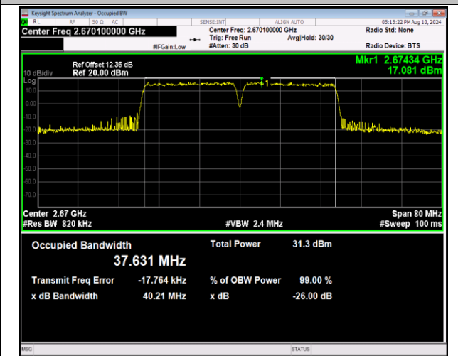
41-41-20MHz-20MHz-QPSK-QPSK-41292-41490-100RB# 0-100RB#0-PASS
