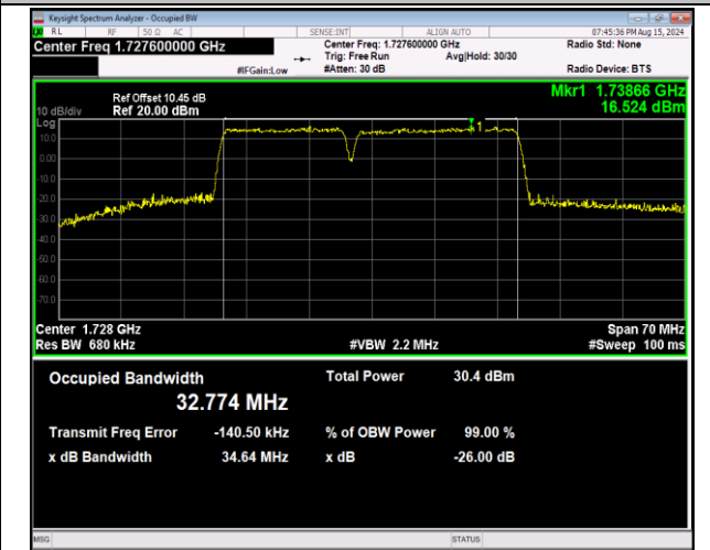
66-66-15MHz-20MHz-64QAM-64QAM-132050-132221-75RB #0-100RB#0-PASS
