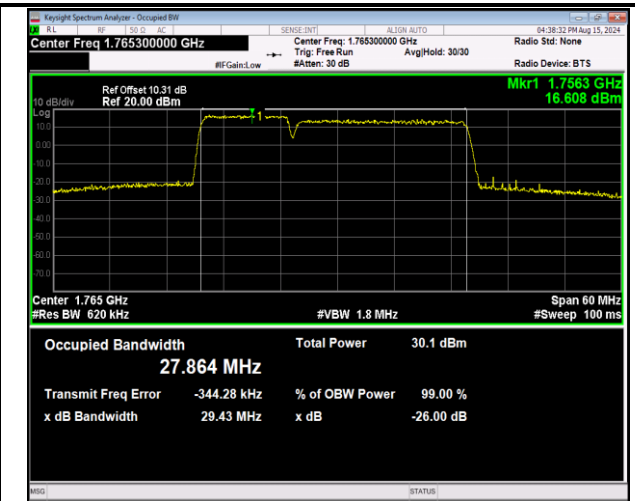
66-66-10MHz-20MHz-16QAM-16QAM-132428-132572-50RB #0-100RB#0-PASS
