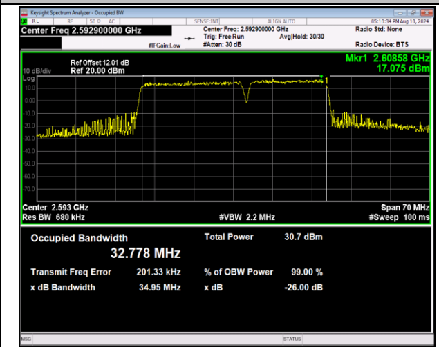
41-41-20MHz-15MHz-QPSK-QPSK-40546-40717-100RB# 0-75RB#0-PASS
