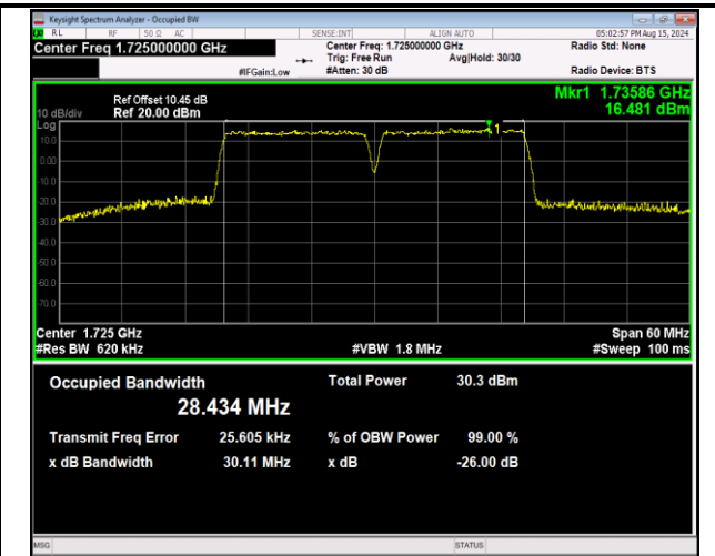
66-66-15MHz-15MHz-16QAM-16QAM-132047-132197-75RB#0-75RB#0-PASS
