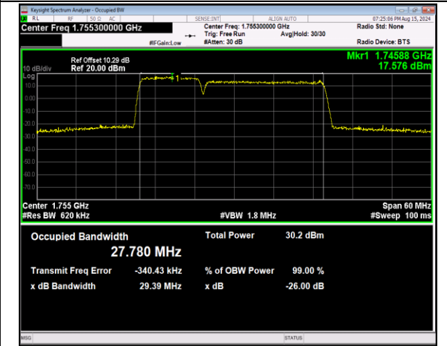
66-66-10MHz-20MHz-64QAM-64QAM-132328-132472-50RB #0-100RB#0-PASS
