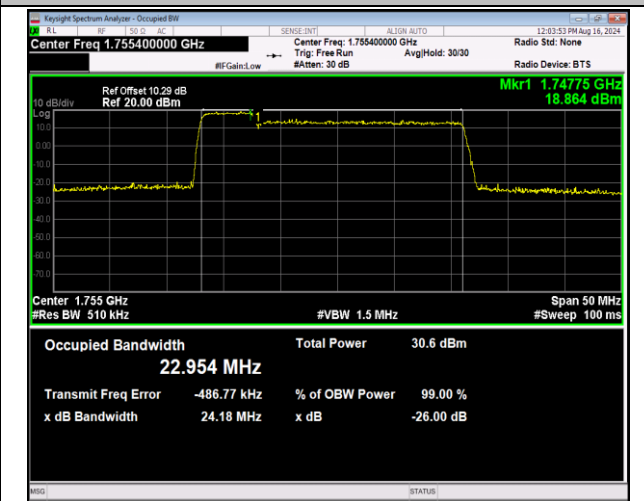
66-66-5MHz-20MHz-QPSK-QPSK-132330-132447-25RB# 0-100RB#0-PASS
