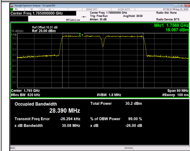
66-66-15MHz-15MHz-64QAM-64QAM-132447-132597-75RB #0-75RB#0-PASS
