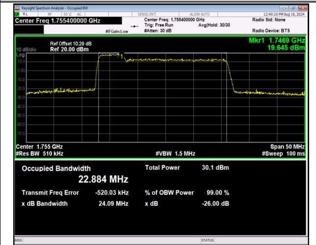
66-66-5MHz-20MHz-64QAM-64QAM-132330-132447-25R B#0-100RB#0-PASS
