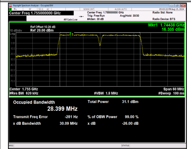
66-66-15MHz-15MHz-QPSK-QPSK-132347-132497-75RB#0-75RB#0-PASS
