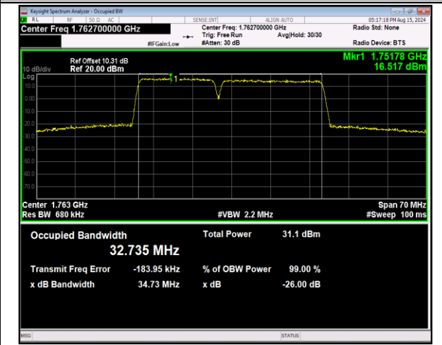
66-66-15MHz-20MHz-QPSK-QPSK-132401-132572-75RB #0-100RB#0-PASS
