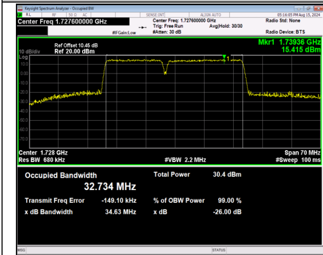
66-66-15MHz-20MHz-16QAM-16QAM-132050-132221-75RB #0-100RB#0-PASS
