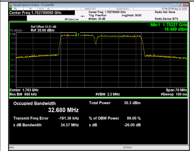
66-66-15MHz-20MHz-64QAM-64QAM-132401-132572-75RB #0-100RB#0-PASS
