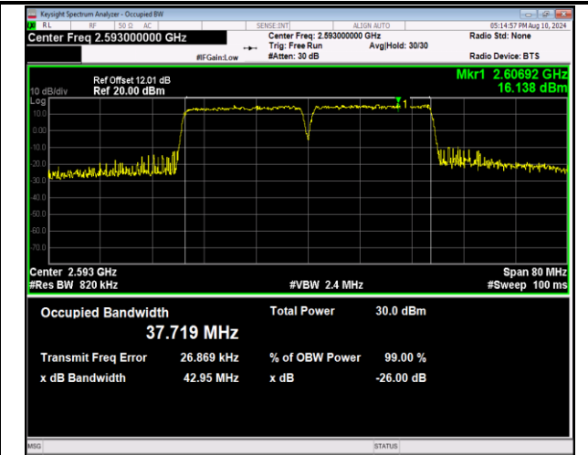
41-41-20MHz-20MHz-16QAM-16QAM-40521-40719-100R B#0-100RB#0-PASS
