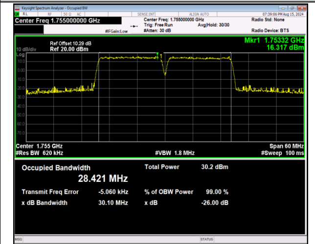
66-66-15MHz-15MHz-64QAM-64QAM-132347-132497-75RB#0-75RB#0-PASS
