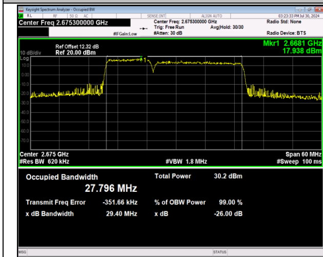
41-41-10MHz-20MHz-64QAM-64QAM-41346-41490-50RB #0-100RB#0-PASS
