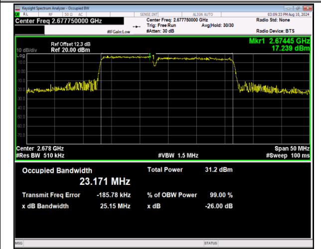
41-41-10MHz-15MHz-QPSK-QPSK-41395-41515-50RB#0 -75RB#0-PASS
