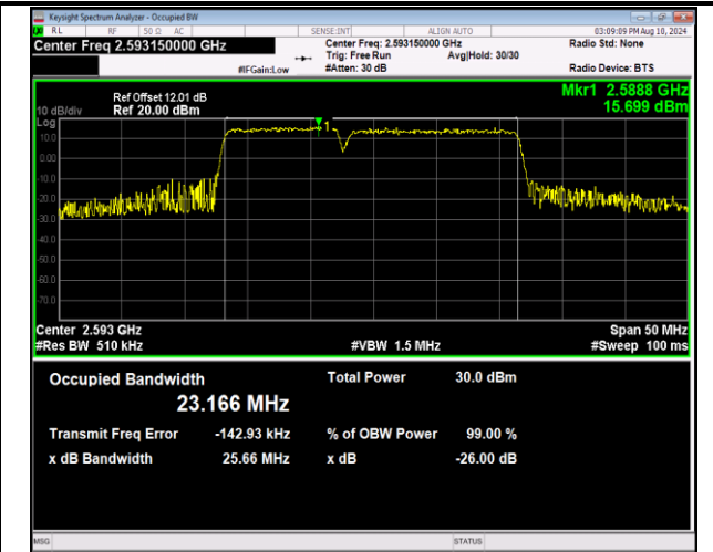
41-41-10MHz-15MHz-16QAM-16QAM-40549-40669-50RB #0-75RB#0-PASS
