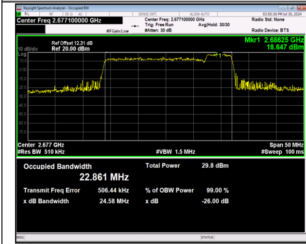
41-41-20MHz-5MHz-64QAM-64QAM-41440-41557-100RB#0-25RB#0-PASS
