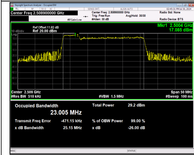
41-41-5MHz-20MHz-64QAM-64QAM-39683-39800-25RB#0-100RB#0-PASS
