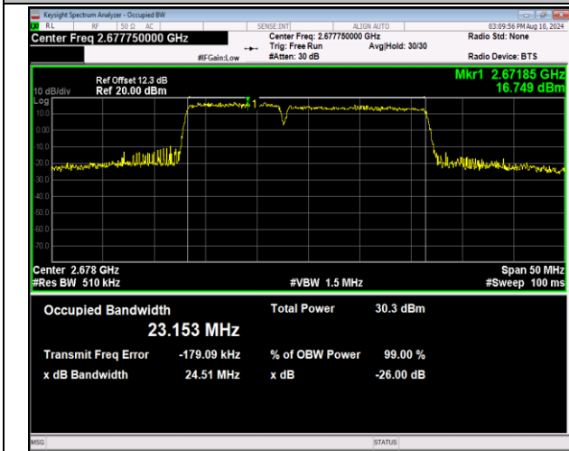
41-41-10MHz-15MHz-16QAM-16QAM-41395-41515-50RB #0-75RB#0-PASS
