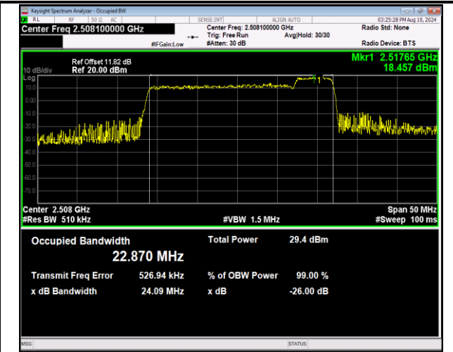
41-41-20MHz-5MHz-16QAM-16QAM-39750-39867-100RB #0-25RB#0-PASS
