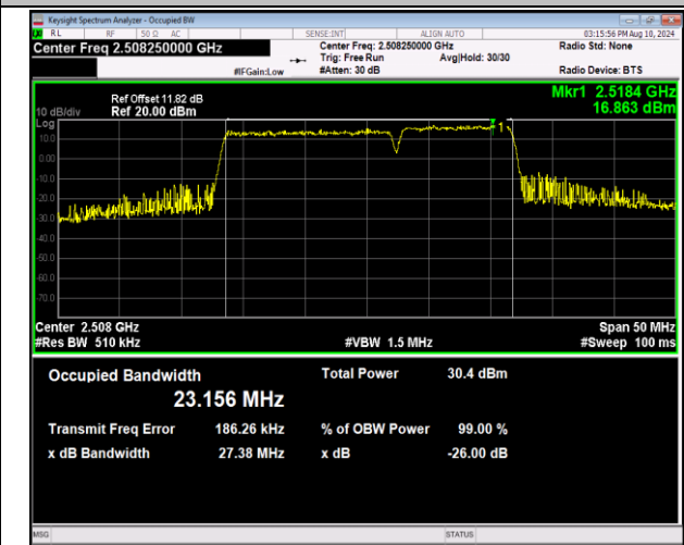
41-41-15MHz-10MHz-QPSK-QPSK-39725-39845-75RB#0 -50RB#0-PASS
