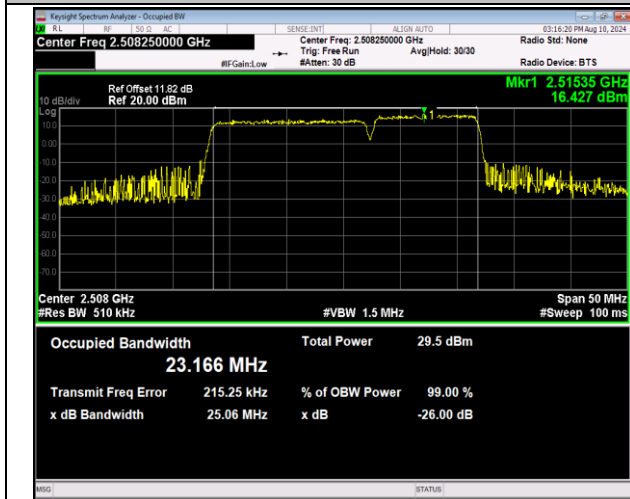
41-41-15MHz-10MHz-16QAM-16QAM-39725-39845-75RB #0-50RB#0-PASS
