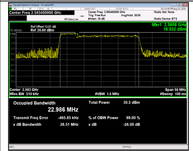
41-41-5MHz-20MHz-QPSK-QPSK-40528-40645-25RB#0-100RB#0-PASS
