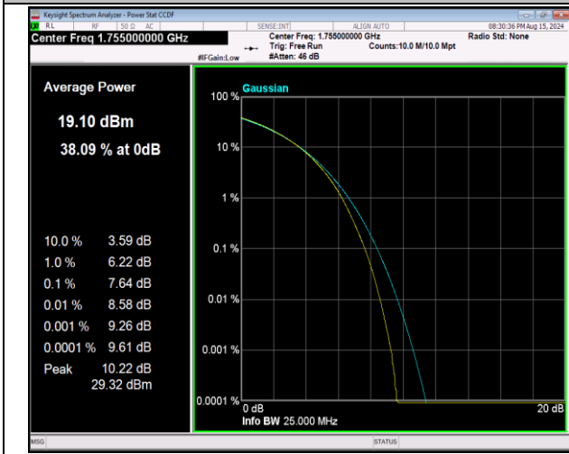
66-66-20MHz-20MHz-64QAM-64QAM-132323-132521-10 ORB#0-100RB#0-PASS
