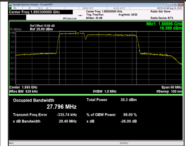
2-2-10MHz-20MHz-16QAM-16QAM-18956-19100-50RB#0-100RB#0-PASS
