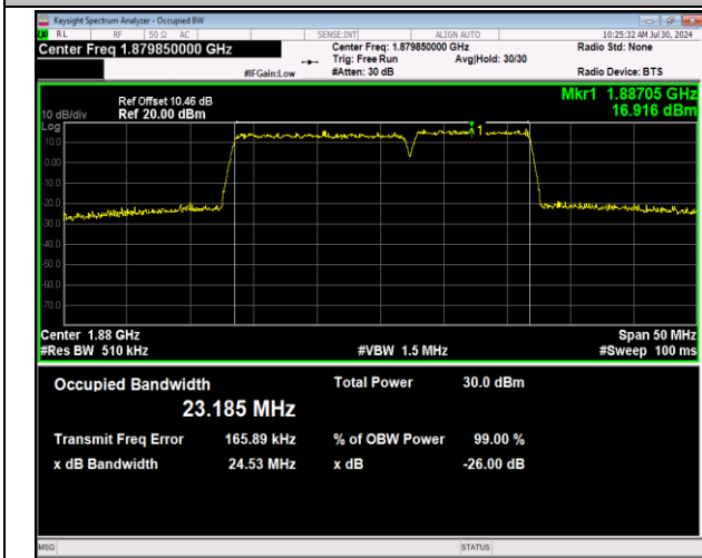
2-2-15MHz-10MHz-64QAM-64QAM-18851-18971-75RB#0-5 -50RB#0-PASS
