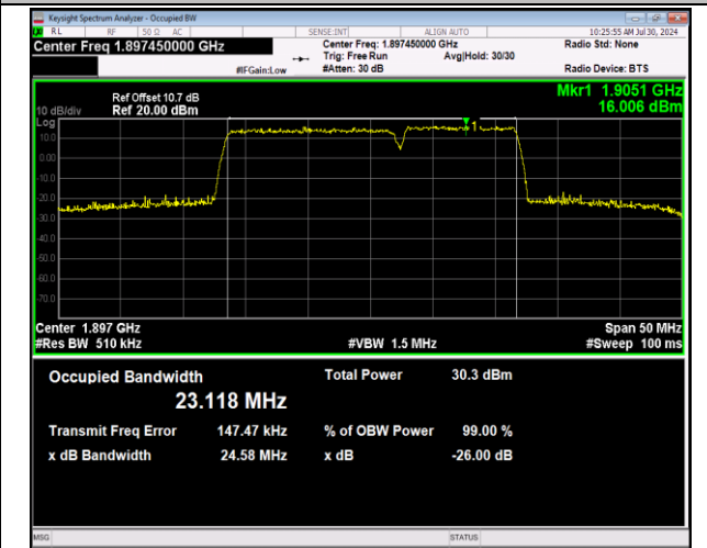
2-2-15MHz-10MHz-64QAM-64QAM-19027-19147-75RB#0-5 -50RB#0-PASS
