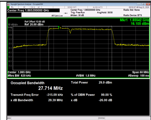
2-2-10MHz-20MHz-16QAM-16QAM-18655-18799-50RB#0-1 -100RB#0-PASS
