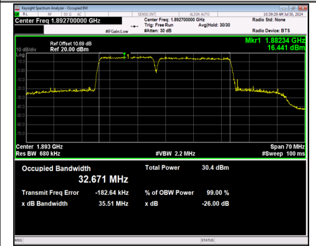
2-2-15MHz-20MHz-64QAM-64QAM-18929-19100-75RB#0 -100RB#0-PASS
