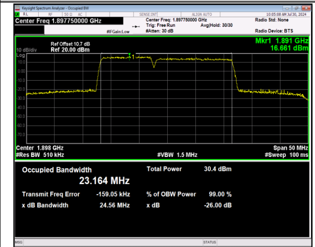
2-2-10MHz-15MHz-64QAM-64QAM-19005-19125-50RB#0-7 -75RB#0-PASS
