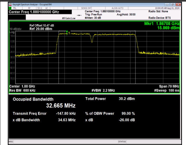
2-2-15MHz-20MHz-16QAM-16QAM-18803-18974-75RB#0 -100RB#0-PASS
