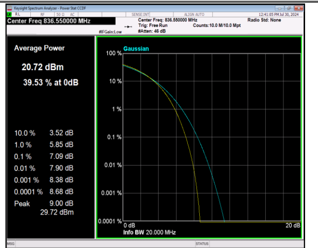
5-5-10MHz-10MHz-64QAM-64QAM-20476-20575-50RB#0-5-0RB#0-PASS
