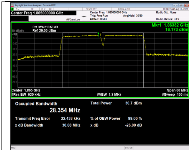
2-2-15MHz-15MHz-QPSK-QPSK-18675-18825-75RB#0-7 5RB#0-PASS
