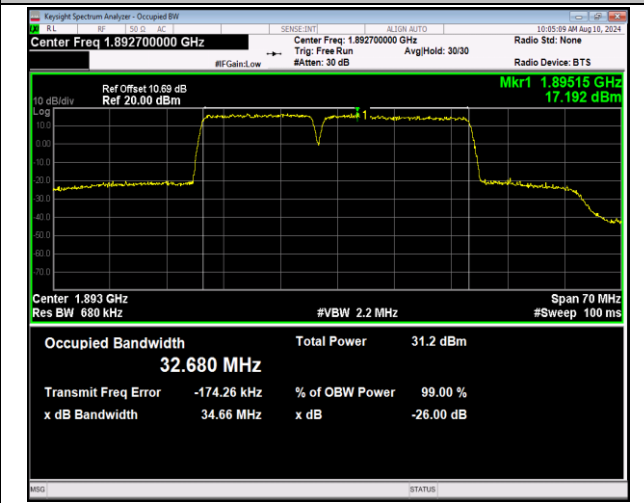
2-2-15MHz-20MHz-QPSK-QPSK-18929-19100-75RB#0-1 00RB#0-PASS
