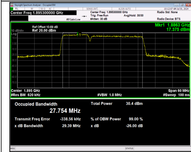
2-2-10MHz-20MHz-64QAM-64QAM-18956-19100-50RB#0-100RB#0-PASS
