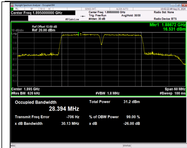
2-2-15MHz-15MHz-QPSK-QPSK-18975-19125-75RB#0-7 5RB#0-PASS
