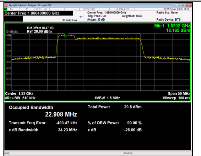
2-2-5MHz-20MHz-64QAM-64QAM-18808-18925-25RB#0-100RB#0-PASS
