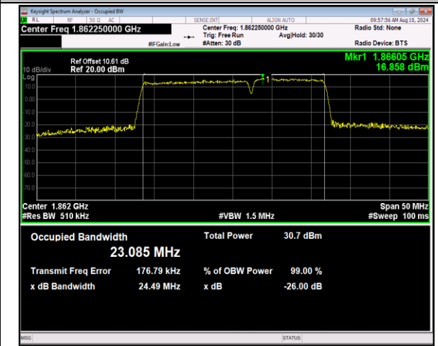
2-2-15MHz-10MHz-QPSK-QPSK-18675-18795-75RB#0-50RB#0-PASS
