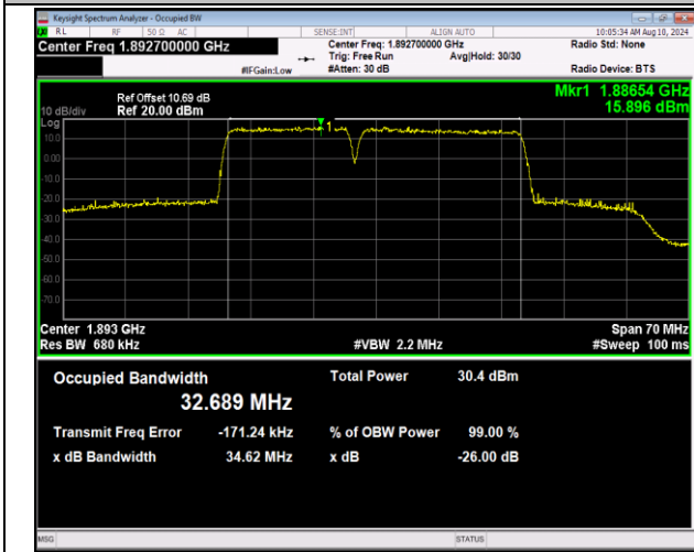
2-2-15MHz-20MHz-16QAM-16QAM-18929-19100-75RB#0 -100RB#0-PASS
