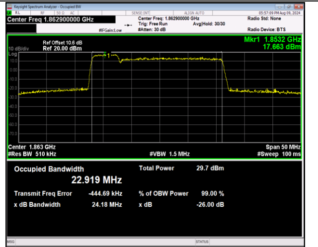
2-2-5MHz-20MHz-16QAM-16QAM-18633-18750-25RB#0-100RB#0-PASS
