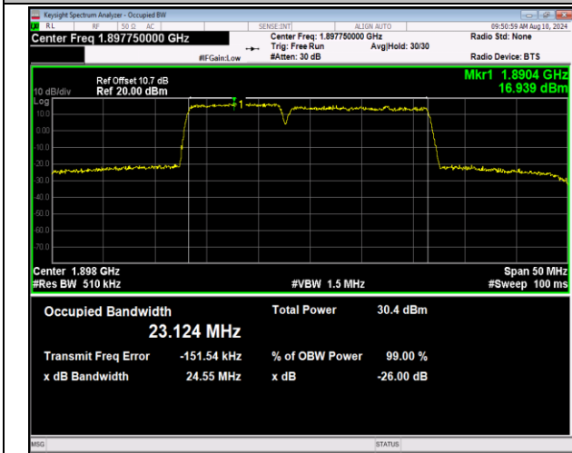
2-2-10MHz-15MHz-16QAM-16QAM-19005-19125-50RB#0-7 -75RB#0-PASS
