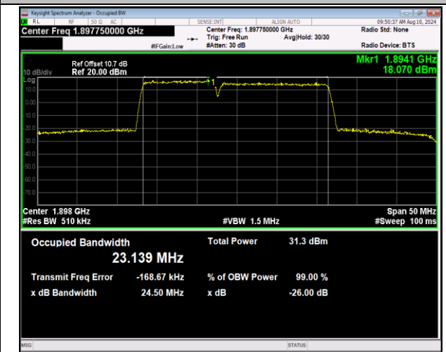
2-2-10MHz-15MHz-QPSK-QPSK-19005-19125-50RB#0-7 5RB#0-PASS
