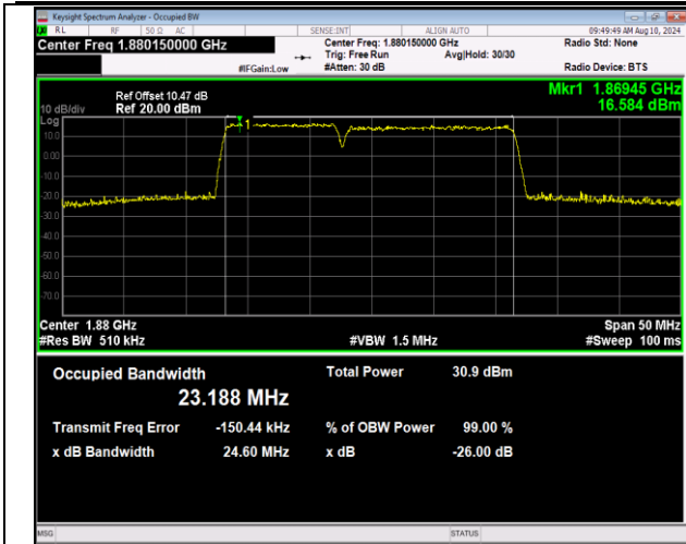
2-2-10MHz-15MHz-QPSK-QPSK-18829-18949-50RB#0-7 5RB#0-PASS
