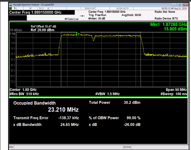
2-2-10MHz-15MHz-16QAM-16QAM-18829-18949-50RB#0-7 -75RB#0-PASS
