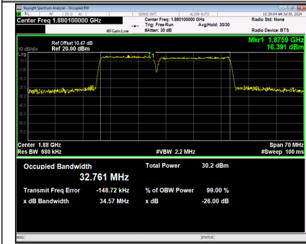
2-2-15MHz-20MHz-64QAM-64QAM-18803-18974-75RB#0 -100RB#0-PASS
