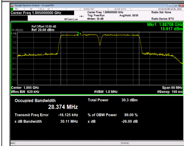
2-2-15MHz-15MHz-64QAM-64QAM-18975-19125-75RB#0-7 -75RB#0-PASS
