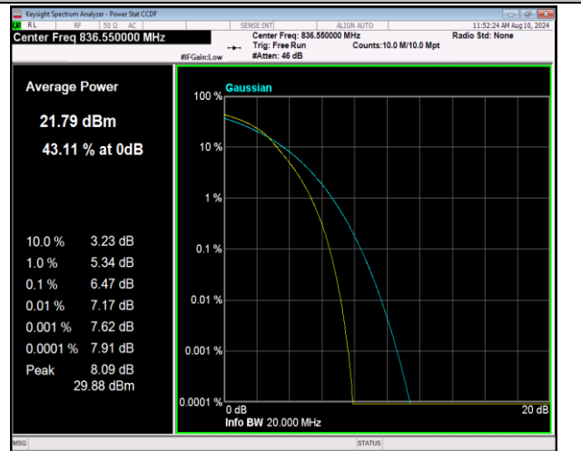
5-5-10MHz-10MHz-QPSK-QPSK-20476-20575-50RB#0-5-0RB#0-PASS
