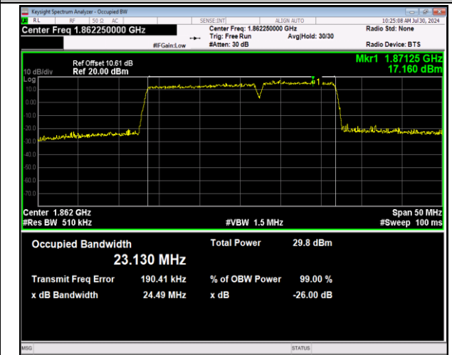
2-2-15MHz-10MHz-64QAM-64QAM-18675-18795-75RB#0-50RB#0-PASS
