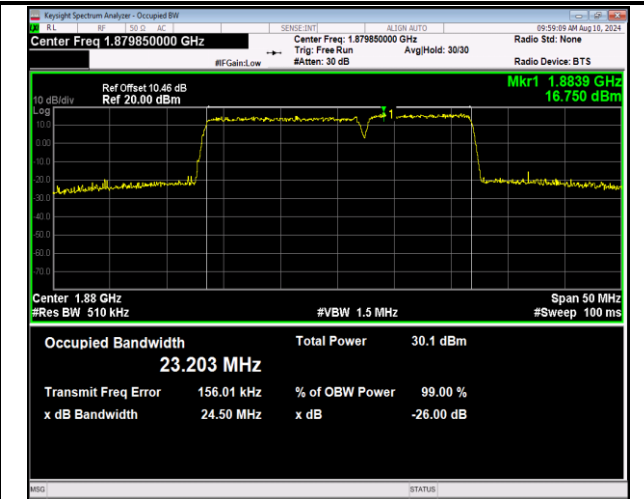
2-2-15MHz-10MHz-16QAM-16QAM-18851-18971-75RB#0-5 -50RB#0-PASS
