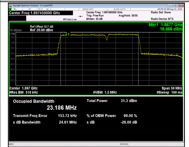
2-2-15MHz-10MHz-QPSK-QPSK-19027-19147-75RB#0-5 ORB#0-PASS
