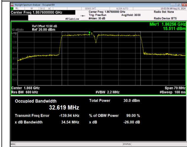
2-2-15MHz-20MHz-16QAM-16QAM-18678-18849-75RB#0-1 -100RB#0-PASS
