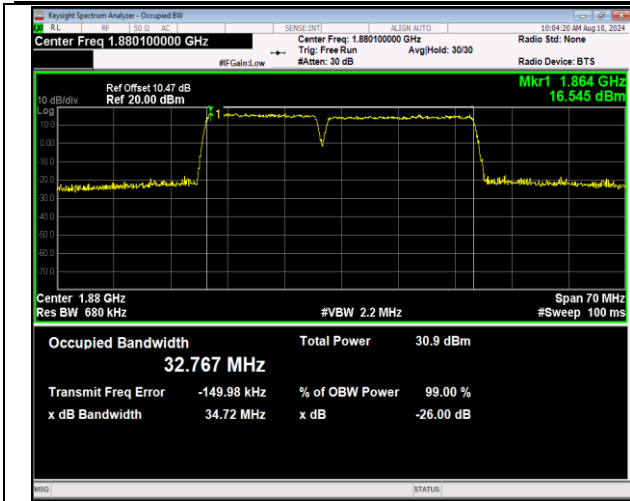
2-2-15MHz-20MHz-QPSK-QPSK-18803-18974-75RB#0-1 00RB#0-PASS
