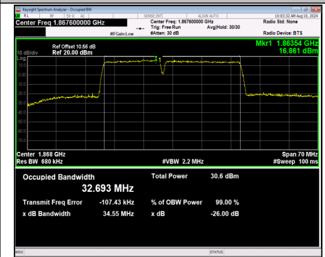
2-2-15MHz-20MHz-QPSK-QPSK-18678-18849-75RB#0-1 00RB#0-PASS
