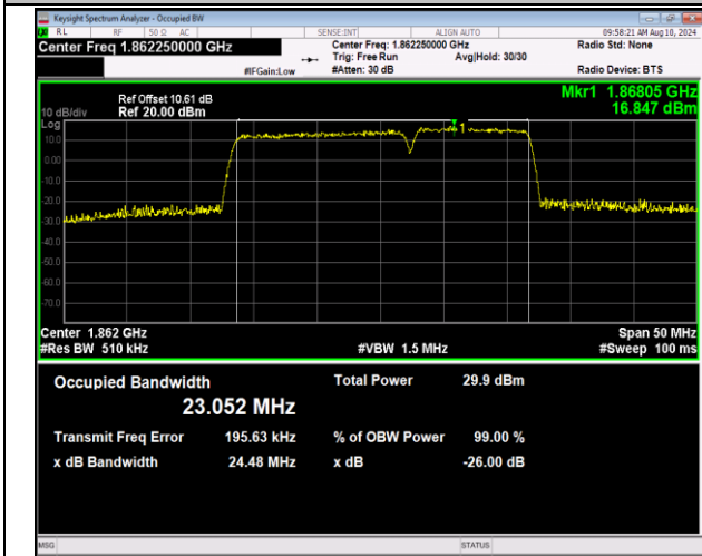
2-2-15MHz-10MHz-16QAM-16QAM-18675-18795-75RB#0-50RB#0-PASS
