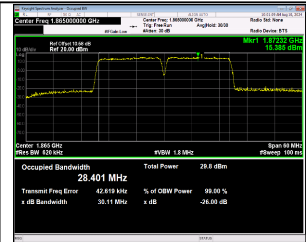
2-2-15MHz-15MHz-16QAM-16QAM-18675-18825-75RB#0-7 -75RB#0-PASS
