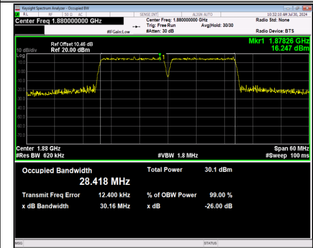
2-2-15MHz-15MHz-64QAM-64QAM-18825-18975-75RB#0-7 -75RB#0-PASS
