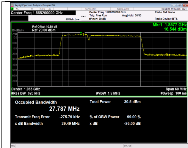
2-2-10MHz-20MHz-QPSK-QPSK-18655-18799-50RB#0-1 00RB#0-PASS
