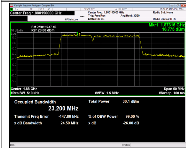
2-2-10MHz-15MHz-64QAM-64QAM-18829-18949-50RB#0-7 -75RB#0-PASS
