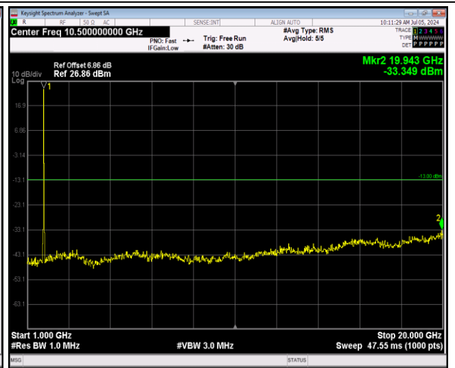
Band66-20MHz-16QAM-132072-1RB#0-Range2:100 0~20000MHz
