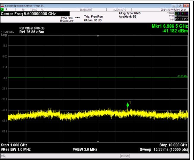
Band26-15MHz-16QAM-26915-1RB#0-Range2:1000~10000MHz
