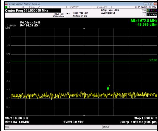
Band66-1.4MHz-16QAM-131979-1RB#0-Range1:30~1000MHz
