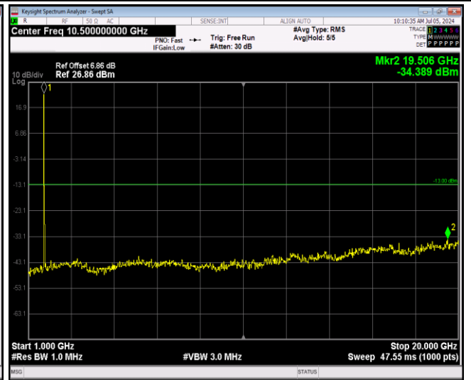
Band66-20MHz-16QAM-132322-1RB#0-Range2:100 0~20000MHz
