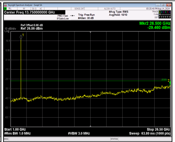
Band41-20MHz-64QAM-39750-1RB#0-Range2:1000~26500MHz
