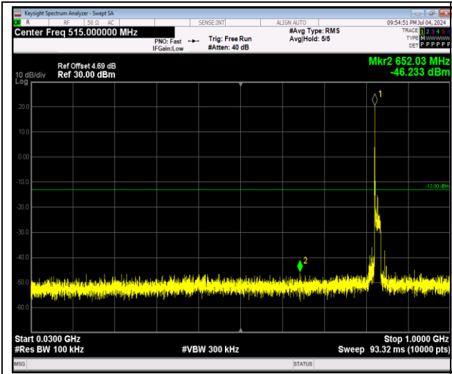
Band26-15MHz-16QAM-26915-1RB#0-Range1:30~1000MHz
