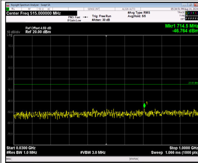
Band41-20MHz-64QAM-40620-1RB#0-Range1:30~1000MHz
