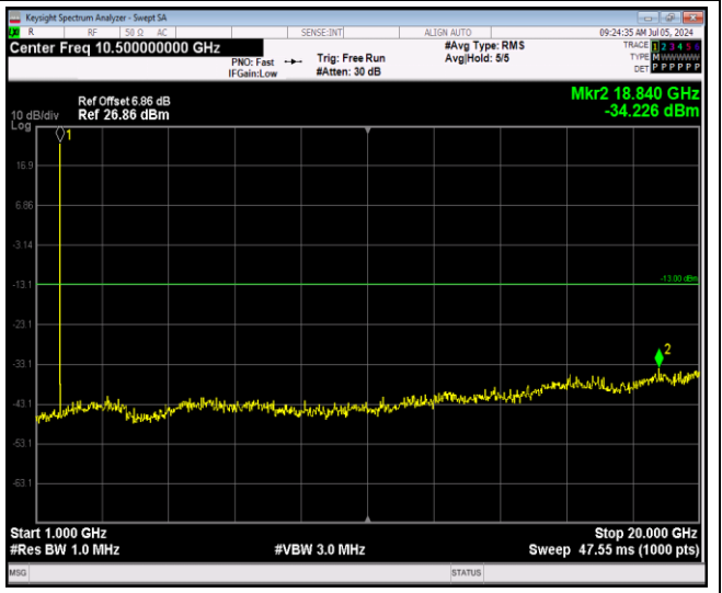
Band66-1.4MHz-16QAM-131979-1RB#0-Range2:1000~20000MHz
