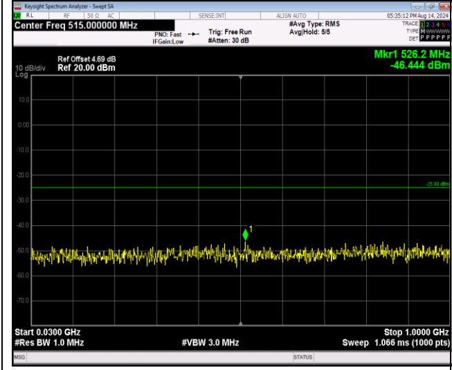
Band41-20MHz-QPSK-41490-1RB#0-Range1:30~1000MHz
