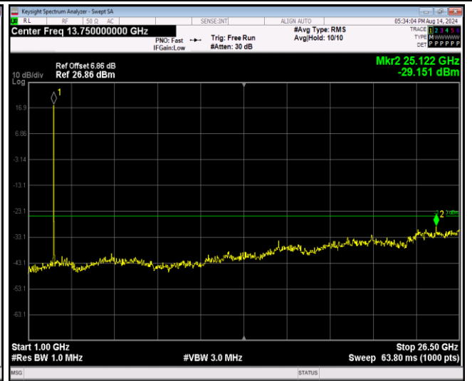
Band41-20MHz-64QAM-40620-1RB#0-Range2:1000~26500MHz
