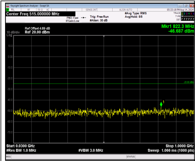
Band41-20MHz-QPSK-40620-1RB#0-Range1:30~1000MHz
