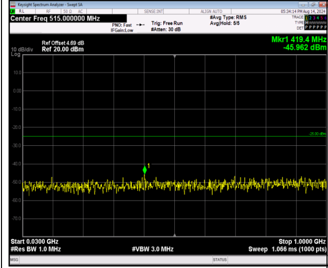
Band41-20MHz-QPSK-41490-1RB#0-Range1:30~1000MHz
