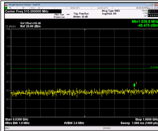
Band41-20MHz-64QAM-39750-1RB#0-Range1:30~1000MHz
