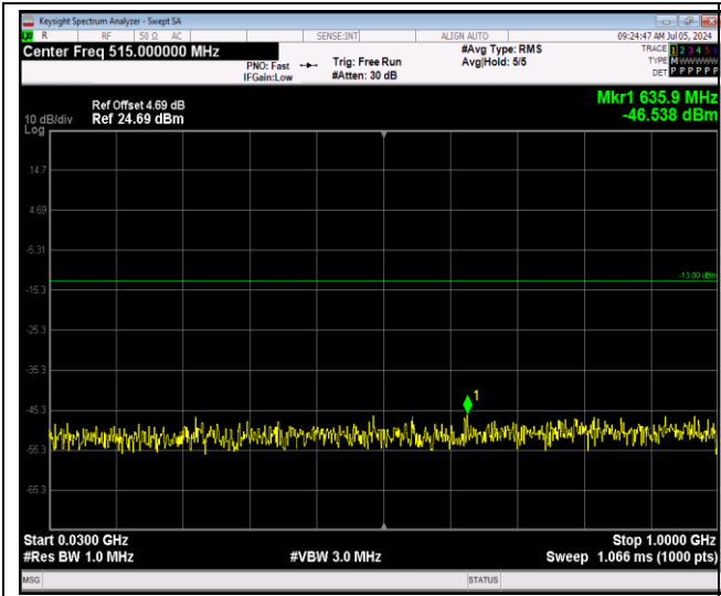
Band66-1.4MHz-QPSK-132665-1RB#0-Range1:30~1000MHz
