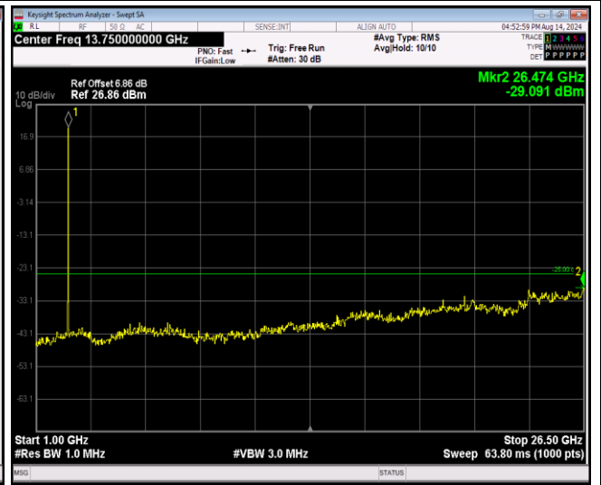
Band41-5MHz-64QAM-39675-1RB#0-Range2:1000~26500MHz
