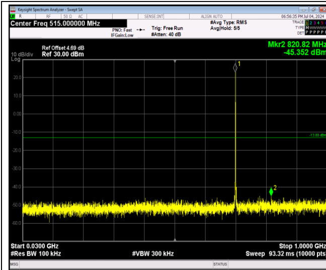
Band12-1.4MHz-16QAM-23173-1RB#0-Range1:30 ~1000MHz
