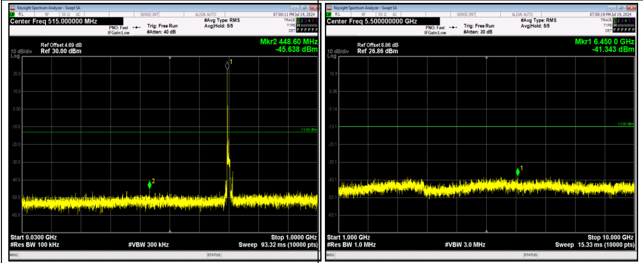
Band12-10MHz-64QAM-23095-1RB#0-Range1:30~1000MHz
