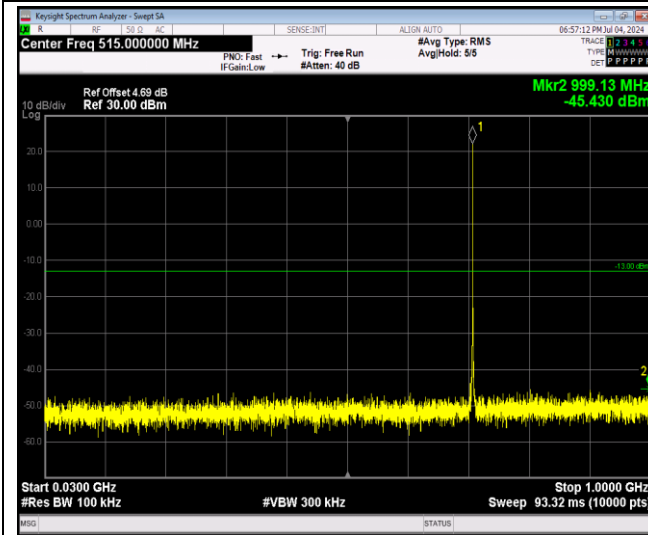
Band12-1.4MHz-64QAM-23017-1RB#0-Range1:30 ~1000MHz
