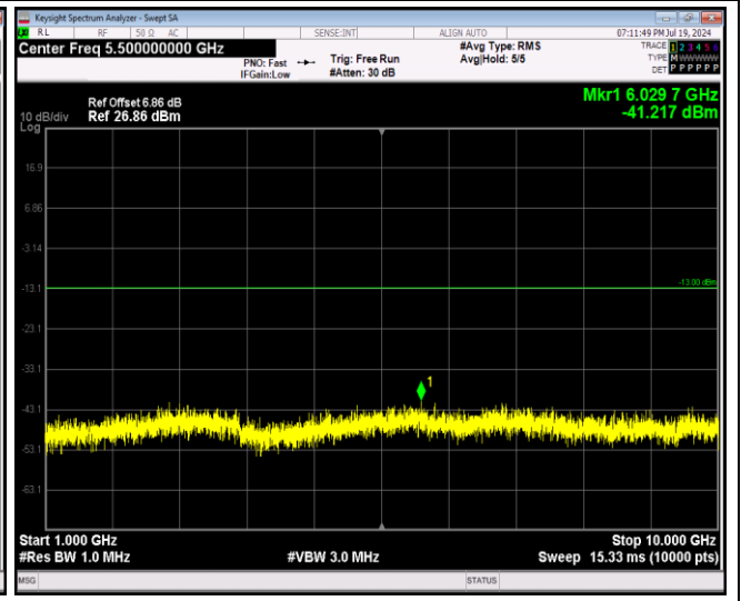
Band13-5MHz-64QAM-23205-1RB#0-Range4:1000~10000MHz
