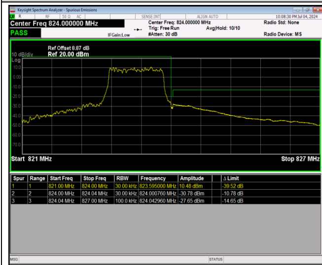
Band26-1.4MHz-QPSK-26797-1RB#5
