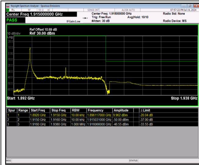
Band25-20MHz-64QAM-26590-100RB#0
