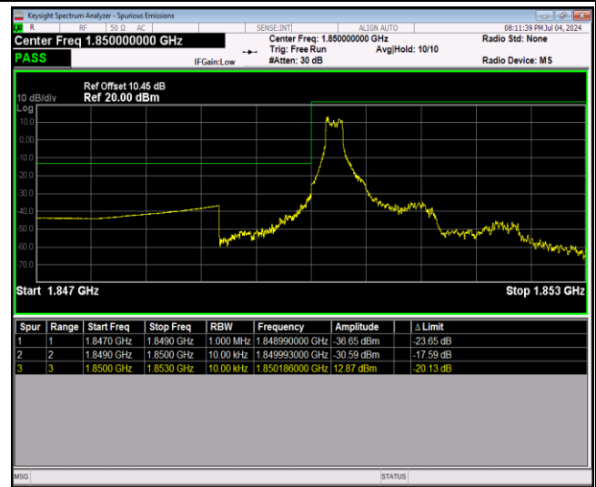
Band25-1.4MHz-16QAM-26047-6RB#0
