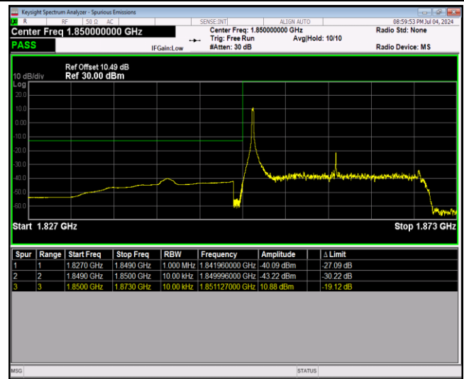
Band25-20MHz-QPSK-26140-100RB#0
