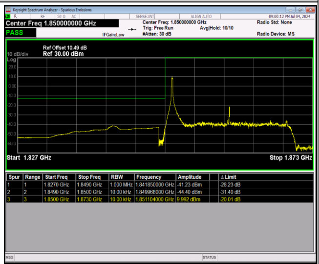
Band25-20MHz-16QAM-26140-100RB#0
