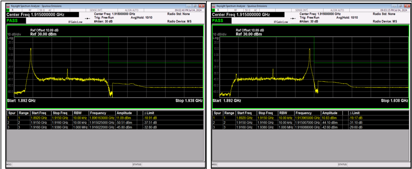
Band25-20MHz-16QAM-26590-100RB#0
