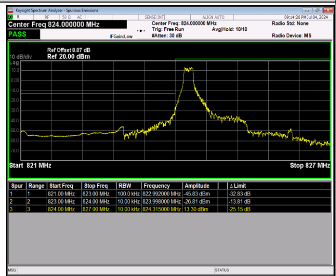
Band26-1.4MHz-QPSK-26797-6RB#0
