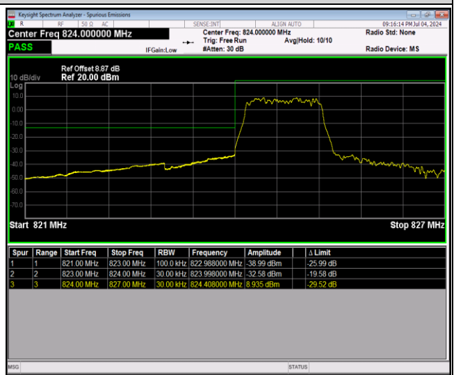
Band26-1.4MHz-16QAM-27033-1RB#5
