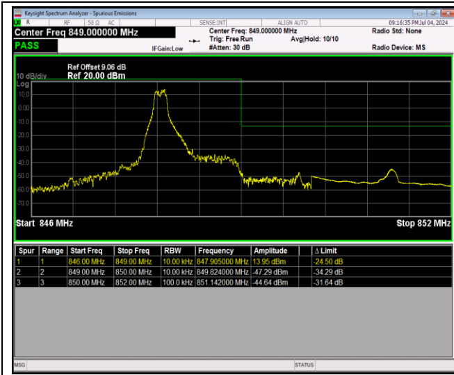
Band26-1.4MHz-QPSK-27033-6RB#0
