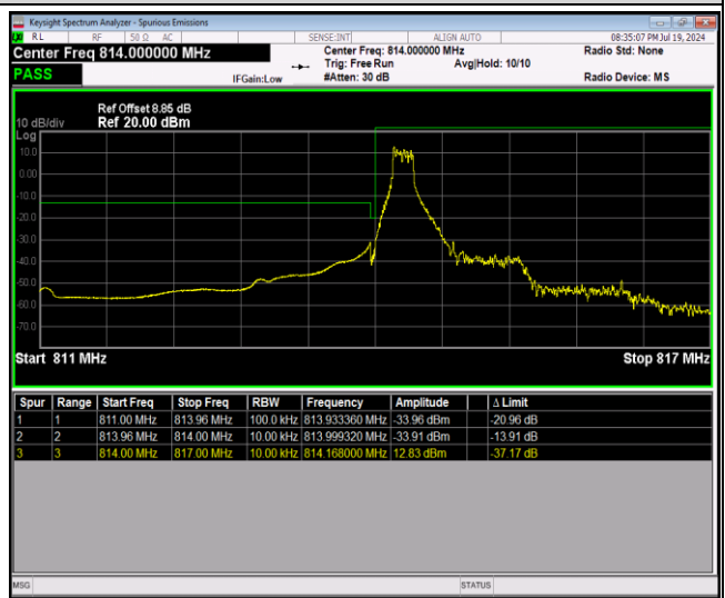
Band26-1.4MHz-64QAM-26697-6RB#0
