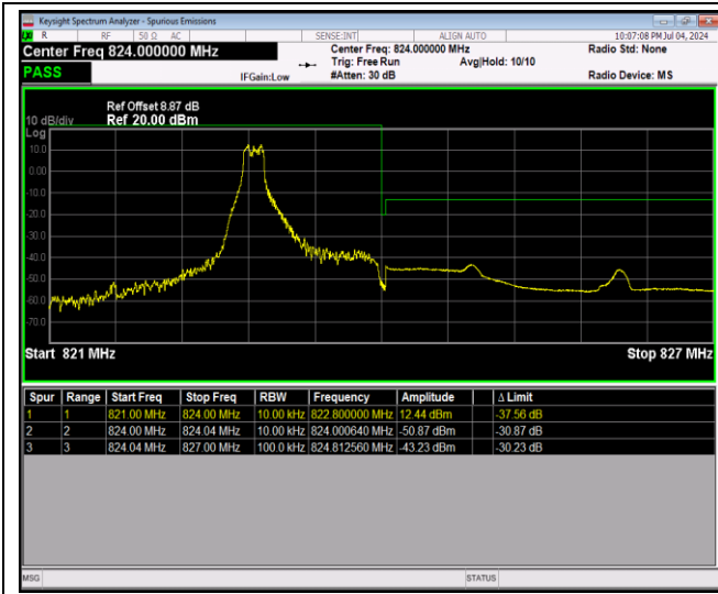
Band26-1.4MHz-16QAM-26783-6RB#0
