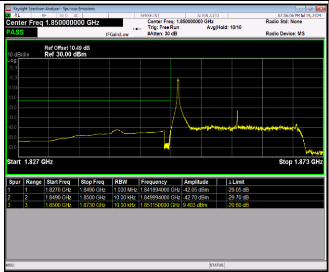
Band25-20MHz-64QAM-26140-100RB#0
