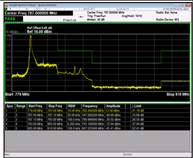
Band13-5MHz-QPSK-23255-25RB#0
