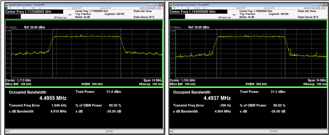
Band66-5MHz-16QAM-132647-25RB#0
