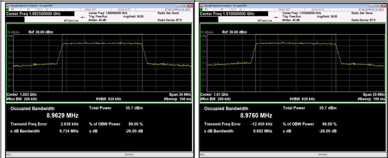
Band25-15MHz-QPSK-26115-75RB#0
