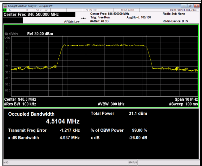
Band26-5MHz-64QAM-26740-25RB#0
