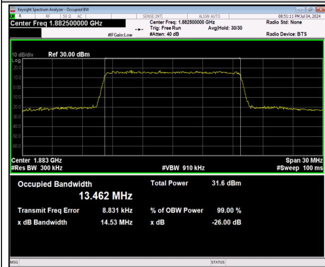
Band25-15MHz-64QAM-26115-75RB#0
