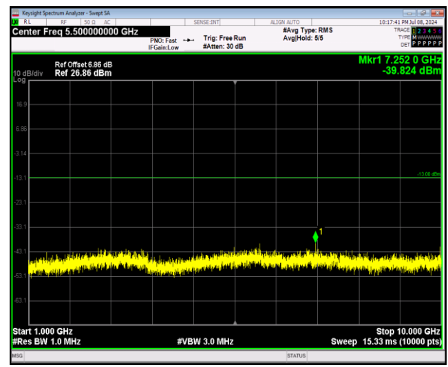
Band12-10MHz-64QAM-23095-1RB#0-Range2:1000~10000MHz
