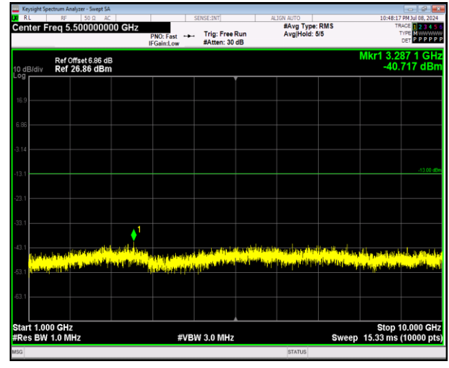
Band13-5MHz-64QAM-23205-1RB#0-Range2:1000~10000MHz
