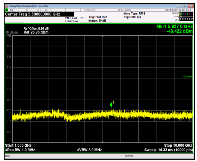
Band12-1.4MHz-QPSK-23095-1RB#0-Range2:1000~10000MHz
