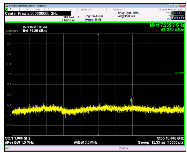
Band12-10MHz-QPSK-23130-1RB#0-Range2:1000~10000MHz
