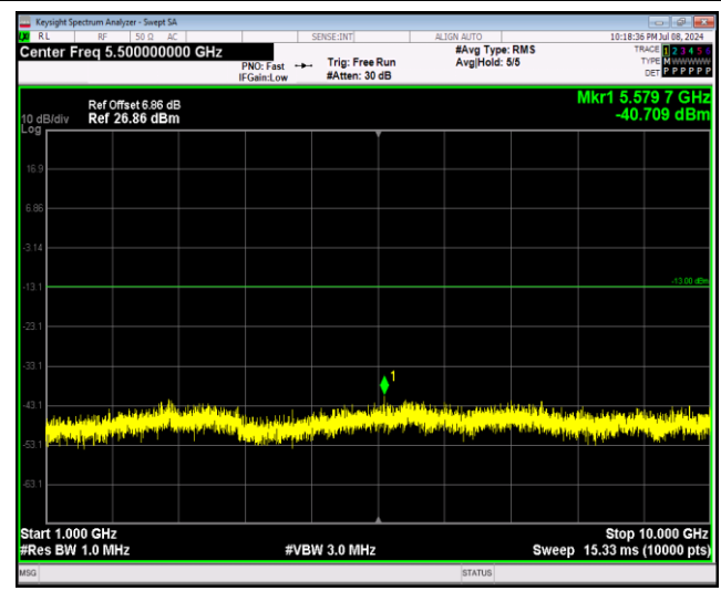
Band12-10MHz-64QAM-23095-1RB#0-Range2:1000~10000MHz
