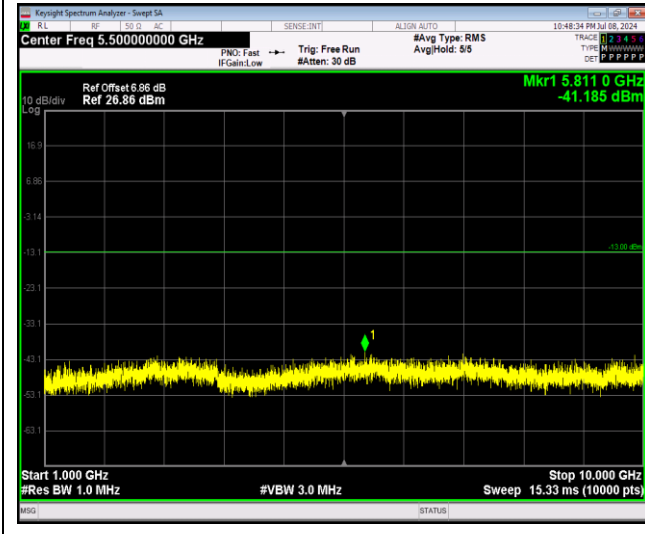
Band13-5MHz-64QAM-23205-1RB#0-Range4:1000~10000MHz
