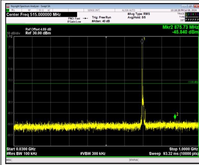
Band12-10MHz-64QAM-23095-1RB#0-Range1:30~1000MHz
