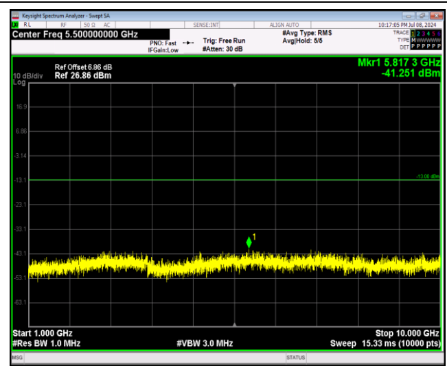
Band12-10MHz-QPSK-23095-1RB#0-Range2:1000~10000MHz
