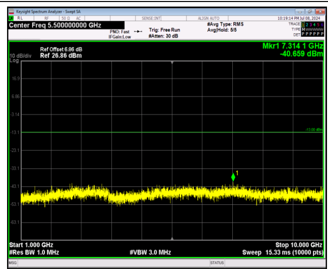
Band12-10MHz-64QAM-23060-1RB#0-Range2:1000~10000MHz
