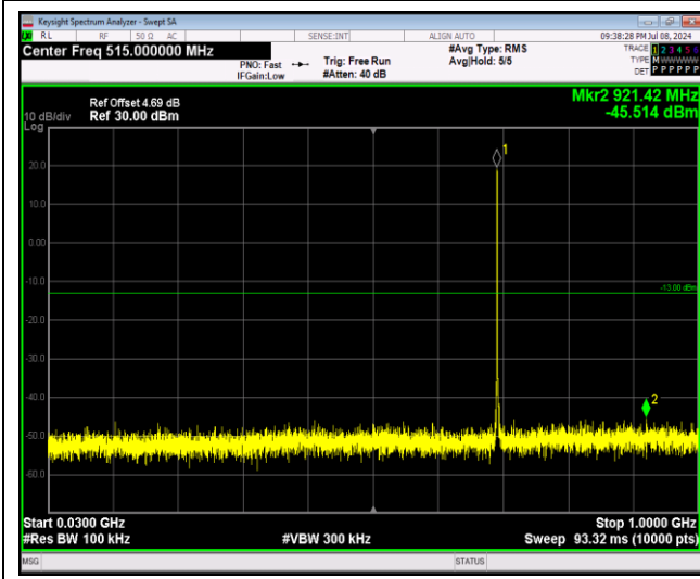
Band12-1.4MHz-64QAM-23017-1RB#0-Range1:30 ~1000MHz
