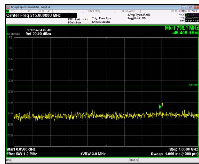
Band7-5MHz-64QAM-21425-1RB#0-Range1:30~1000MHz
