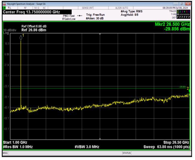
Band7-5MHz-16QAM-21100-1RB#0-Range2:1000~26500MHz
