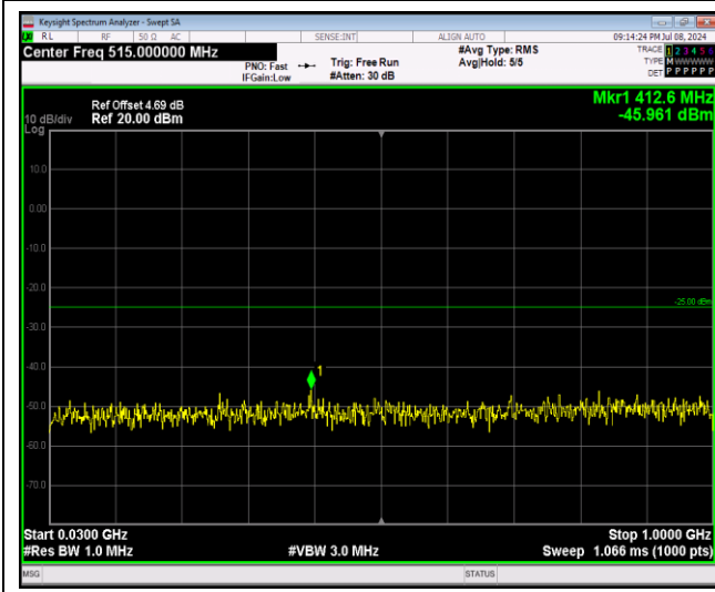
Band7-20MHz-QPSK-20850-1RB#0-Range1:30~1000MHz
