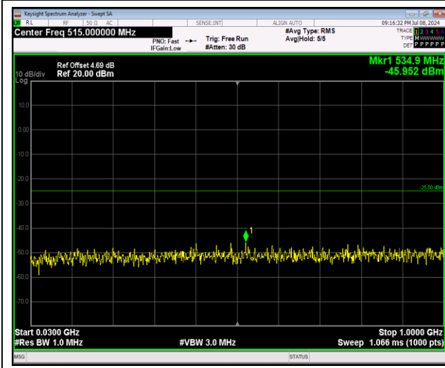
Band7-20MHz-16QAM-21350-1RB#0-Range1:30~1000MHz
