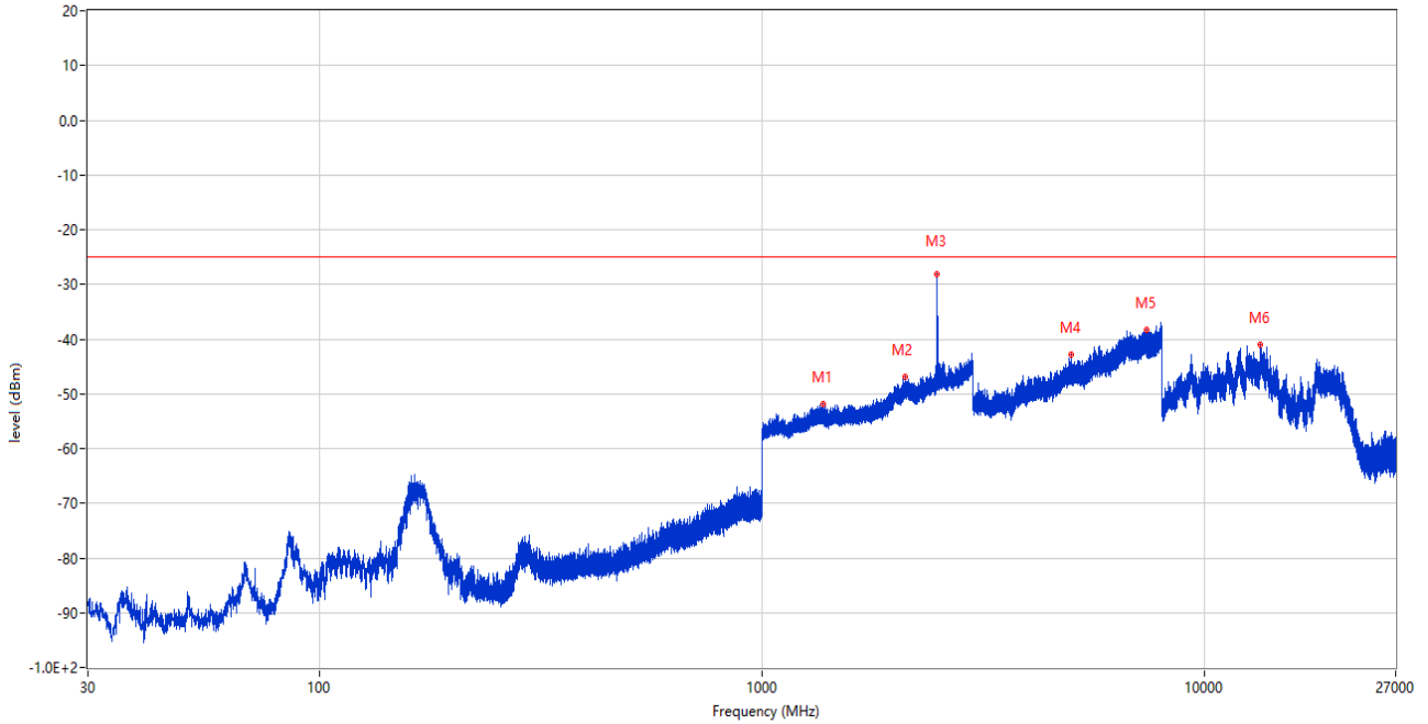
RSE (RF) _FCC PART22&24&27_LTE Band 7 & 41(low) _2496-2570_30MHz-27GHz_
