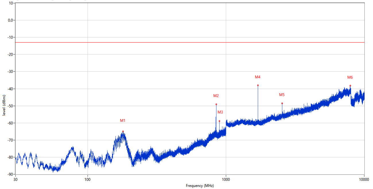
RSE (RF) _FCC PART22&24&27_GSM 850_814-849_30MHz-10GHz
