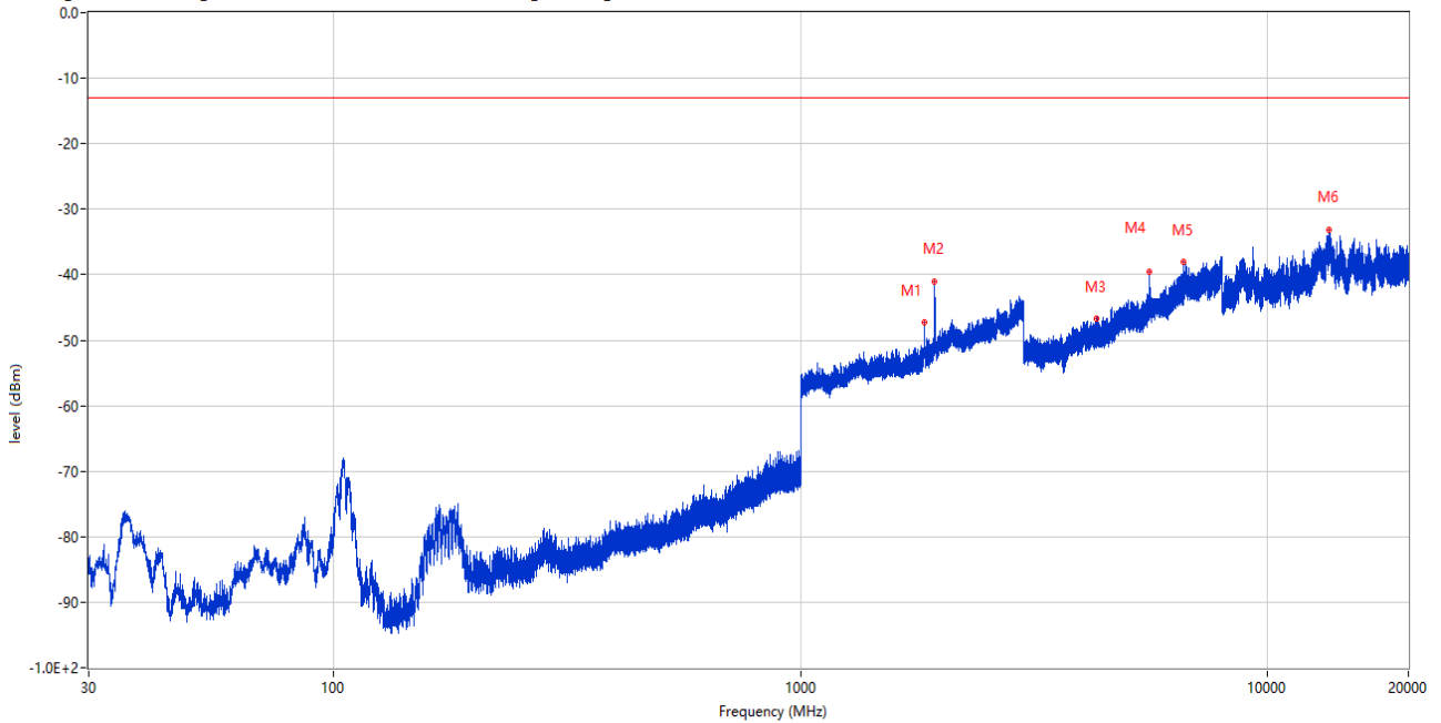
RSE (RF) _FCC PART22&24&27_CDMA BC1 & WCDMA Band 2 & LTE Band 2 & 25 _1830-1920_30MHz-20GHz
