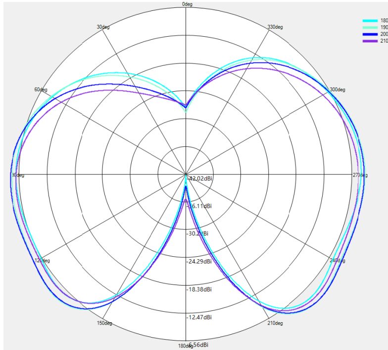
DCS/PCS/WCDMA B1/B2/B4/LTE B1/B2/B3/B4/B25/B66 Phi=90deg
