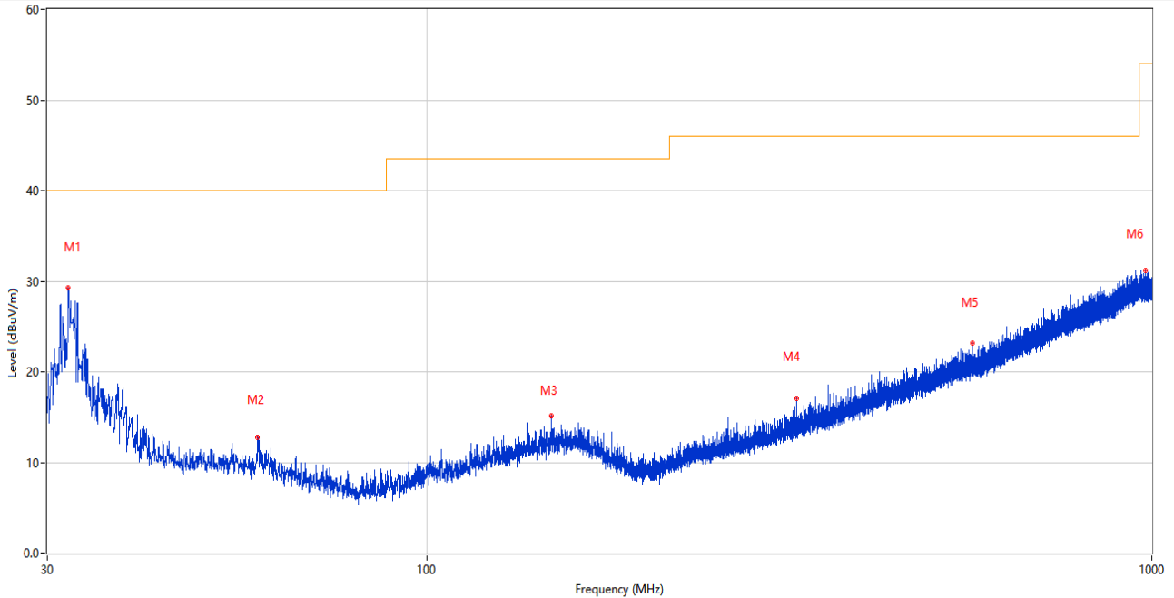
30 MHz to 1 GHz, Test Antenna Vertical, EUT Y axis
