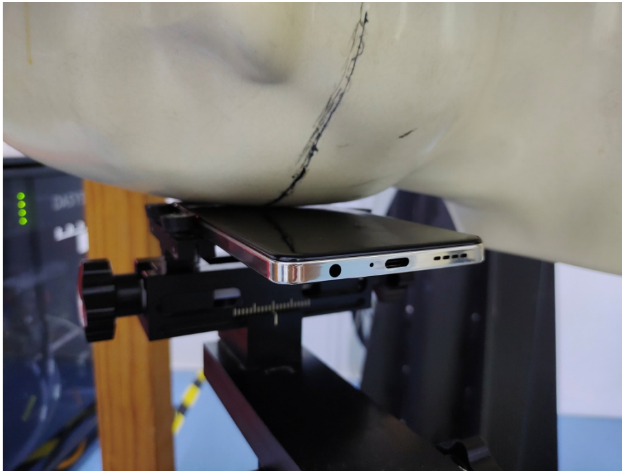
Head Right Check Setup Photo (0mm)
