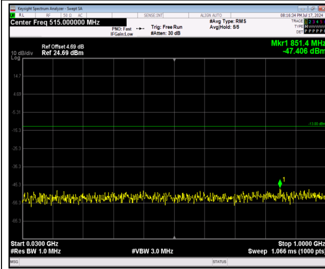
Band25-20MHz-16QAM-26140-1RB#0-Range1:30~1000MHz
