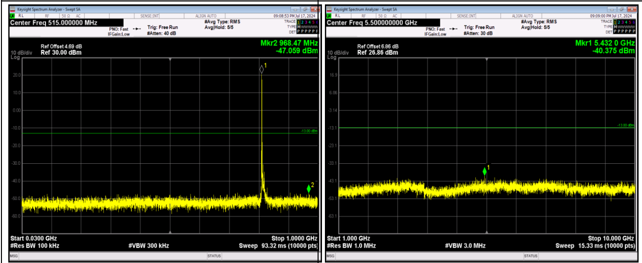
Band26-10MHz-QPSK-26740-1RB#0-Range1:30~1 000MHz
