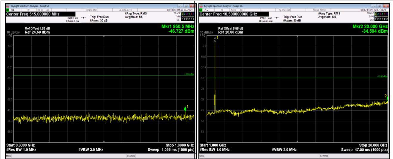
Band25-20MHz-QPSK-26590-1RB#0-Range1:30~1000MHz
