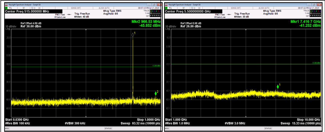
Band26-1.4MHz-16QAM-26740-1RB#0-Range1:30 ~1000MHz
