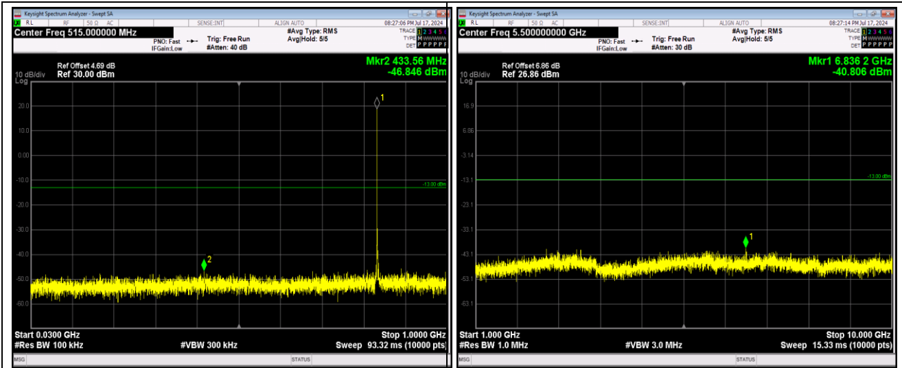
Band26-1.4MHz-16QAM-27033-1RB#0-Range1:30 ~1000MHz
