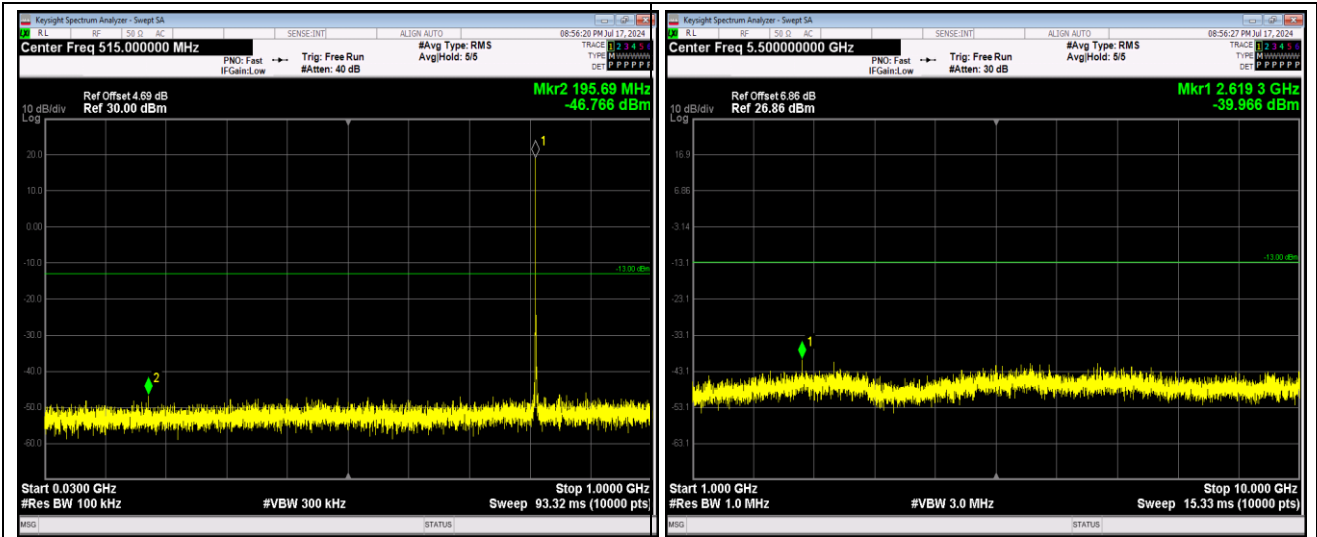
Band26-1.4MHz-QPSK-26740-1RB#0-Range1:30~1000MHz
