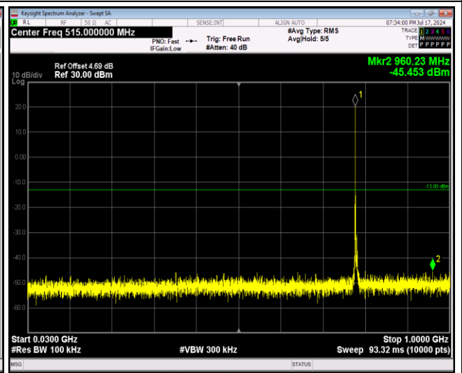
Band13-5MHz-16QAM-23255-1RB#0-Range3:30~10 00MHz
