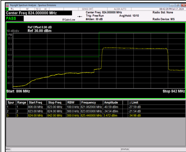
Band26-15MHz-16QAM-26965-1RB#74
