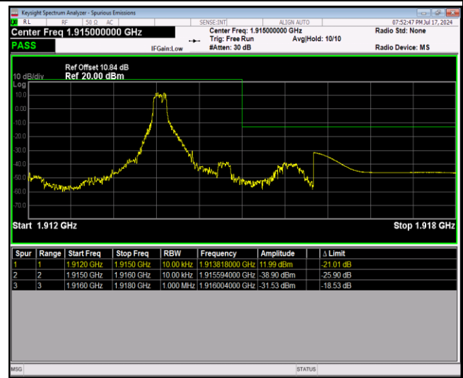
Band25-1.4MHz-16QAM-26683-6RB#0
