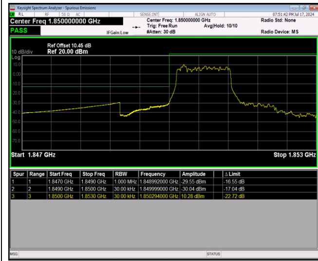
Band25-1.4MHz-QPSK-26683-1RB#5
