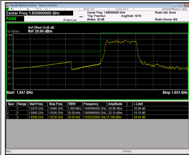
Band25-1.4MHz-16QAM-26683-1RB#5
