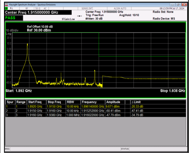
Band25-20MHz-16QAM-26590-100RB#0
