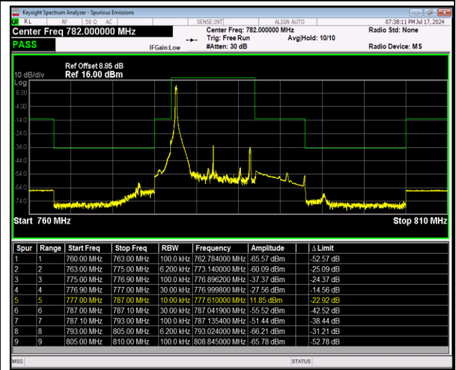
Band13-10MHz-16QAM-23230-50RB#0
