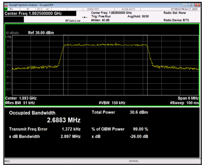
Band25-3MHz-16QAM-26055-15RB#0
