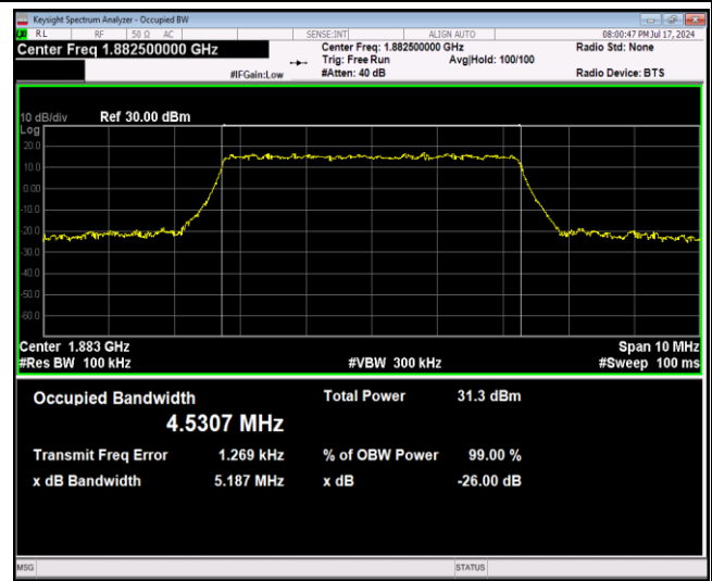
Band25-5MHz-16QAM-26065-25RB#0
