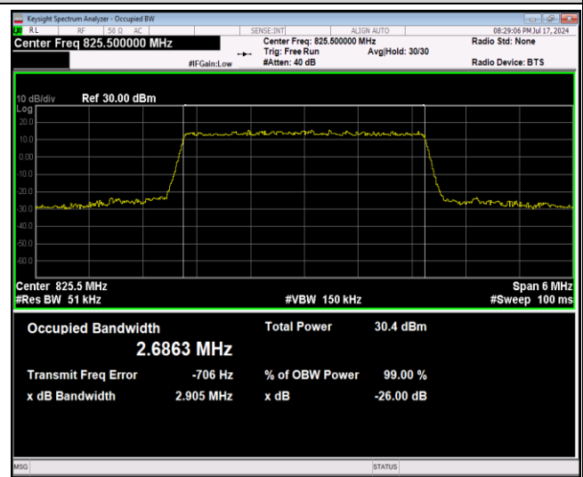
Band26-3MHz-QPSK-27025-15RB#0
