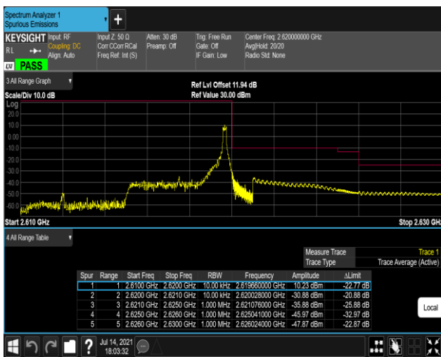
Band38-5MHz-QPSK-38225-1RB#24
