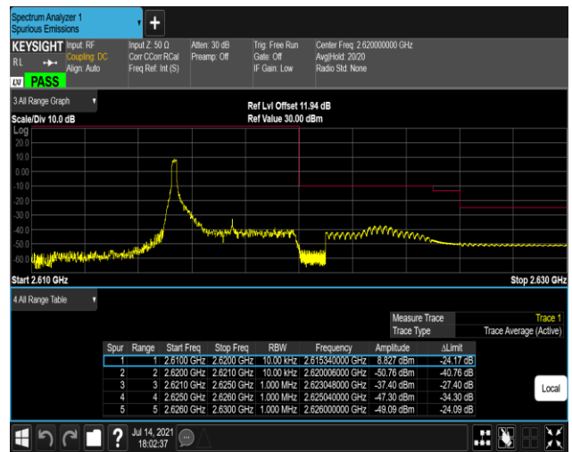
Band38-5MHz-QPSK-38225-25RB#0
