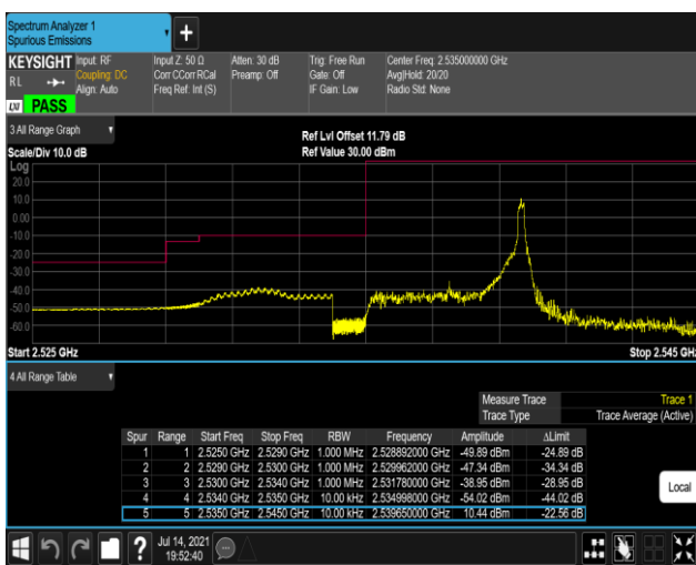
Band41-5MHz-16QAM-40065-1RB#24
