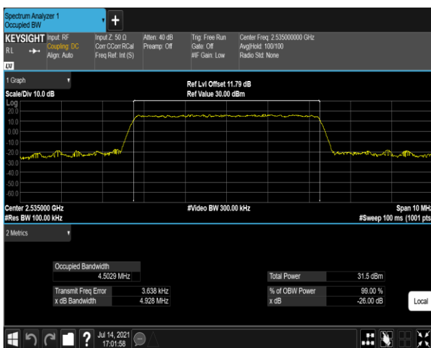
Band7-5MHz-16QAM-21100-25RB#0
