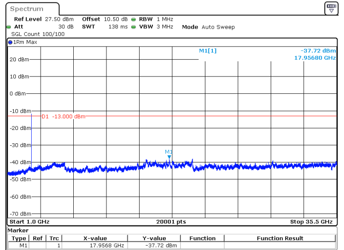
15MHz_15kHz_3500MHz_DFT-s-OFDM QPSK_RB1@78 -37.72 dBm
