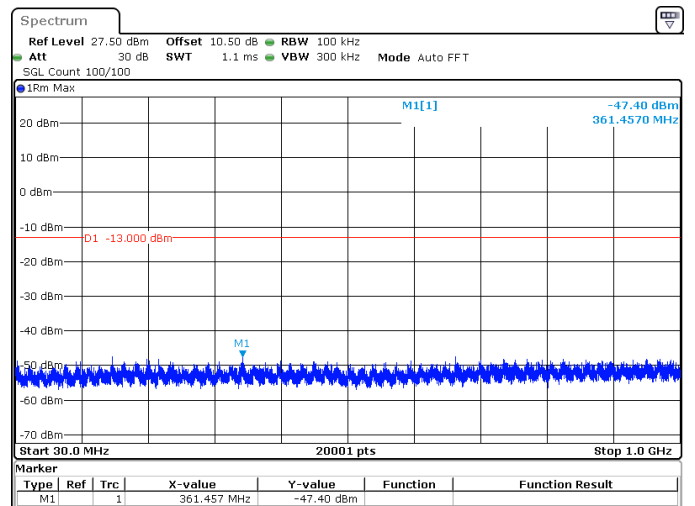
15MHz_15kHz_3500MHz_DFT-s-OFDM QPSK_RB75@0 -47.40 dBm
