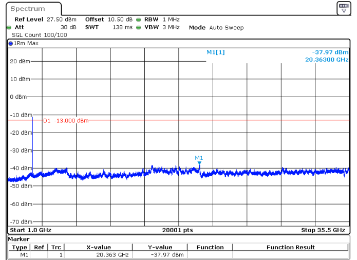
15MHz_15kHz_3500MHz_DFT-s-OFDM QPSK_RB1@0 -37.97 dBm
