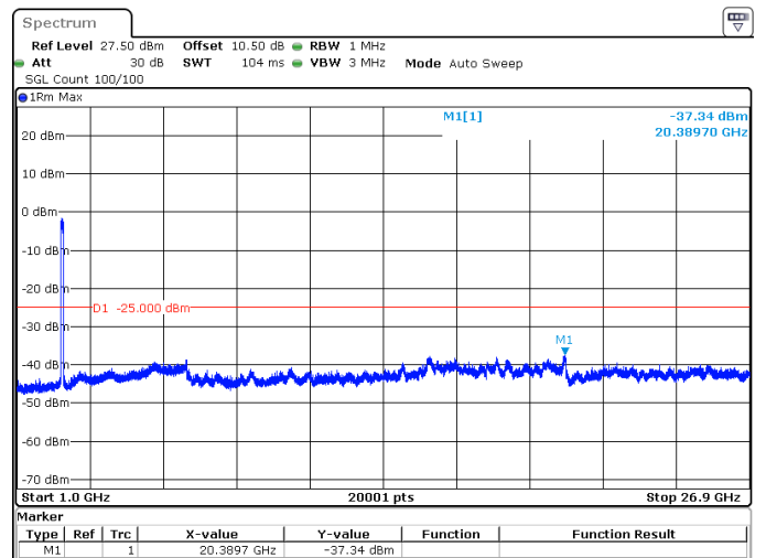
80MHz_30kHz_2592.99MHz_DFT-s-OFDM QPSK_RB216@0 -37.34 dBm
