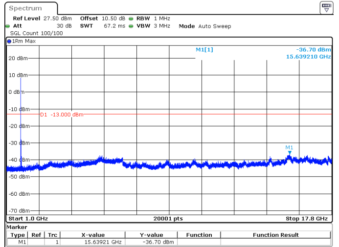
30MHz_15kHz_1745MHz_DFT-s-OFDM QPSK_RB1@0 -36.70 dBm
