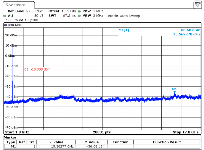
5MHz_15kHz_1712.5MHz_DFT-s-OFDM QPSK_RB1@0 -36.68 dBm
