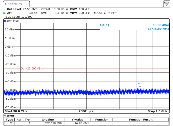
80MHz_30kHz_2536.02MHz_DFT-s-OFDM QPSK_RB1@216 -46.98 dBm
