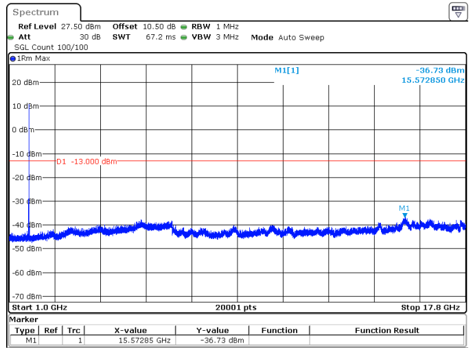
5MHz_15kHz_1712.5MHz_DFT-s-OFDM QPSK_RB1@24 -36.73 dBm
