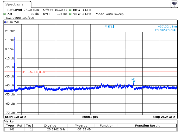
80MHz_30kHz_2592.99MHz_DFT-s-OFDM QPSK_RB1@0 -37.32 dBm
