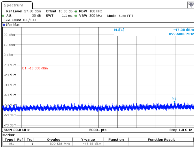
5MHz_15kHz_1712.5MHz_DFT-s-OFDM QPSK_RB1@24 -47.38 dBm
