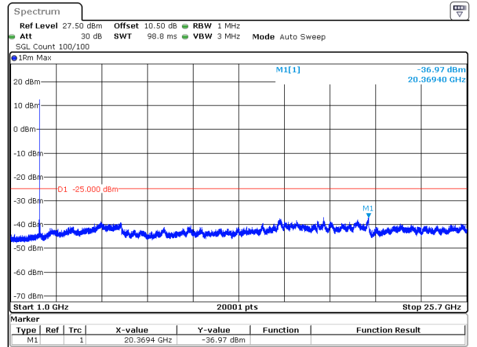
5MHz_15kHz_2567.5MHz_DFT-s-OFDM QPSK_RB1@0 -36.97 dBm
