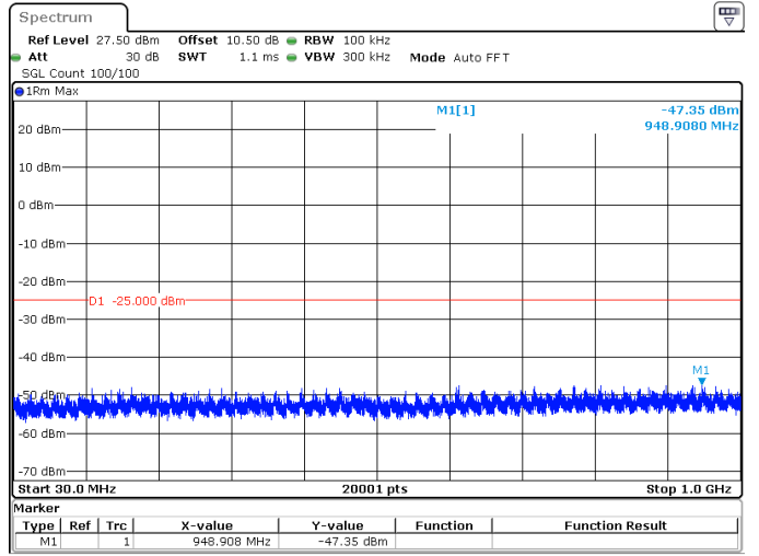
100MHz_30kHz_2592.99MHz_DFT-s-OFDM QPSK_RB1@272 -47.35 dBm
