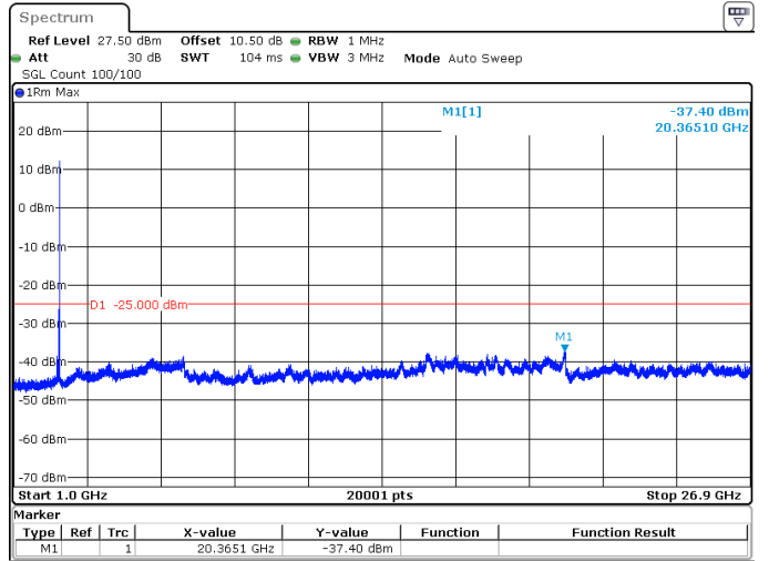
100MHz_30kHz_2546.01MHz_DFT-s-OFDM QPSK_RB1@272 -37.40 dBm
