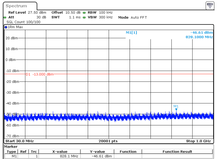
25MHz_15kHz_1745MHz_DFT-s-OFDM QPSK_RB128@0 -46.61 dBm
