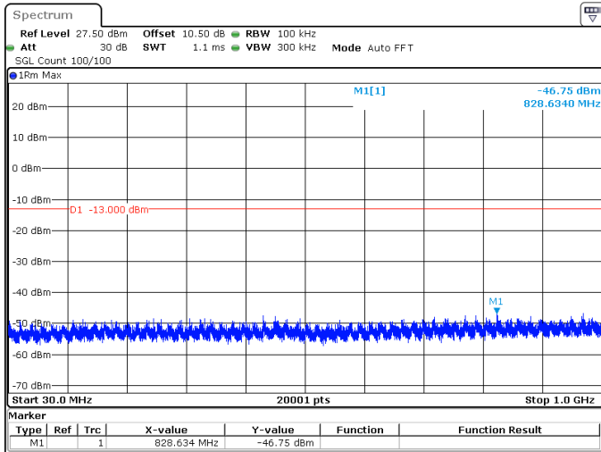
25MHz_15kHz_1745MHz_DFT-s-OFDM QPSK_RB1@0 -46.75 dBm
