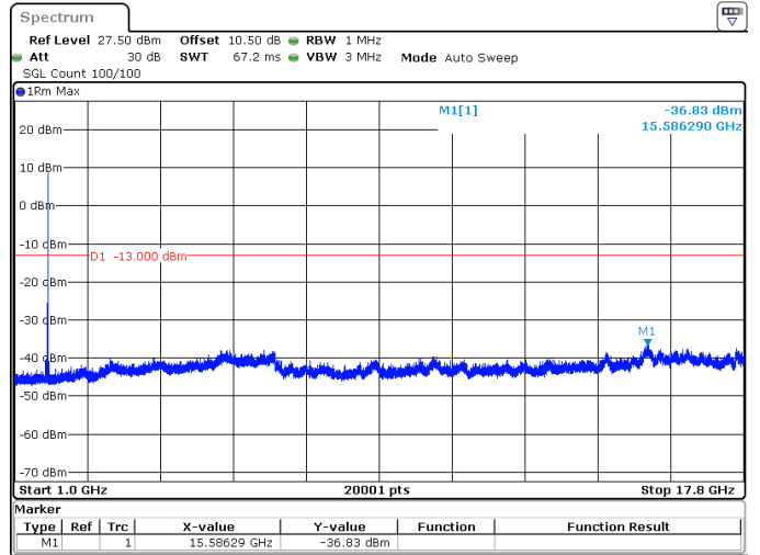
25MHz_15kHz_1745MHz_DFT-s-OFDM QPSK_RB1@132 -36.83 dBm
