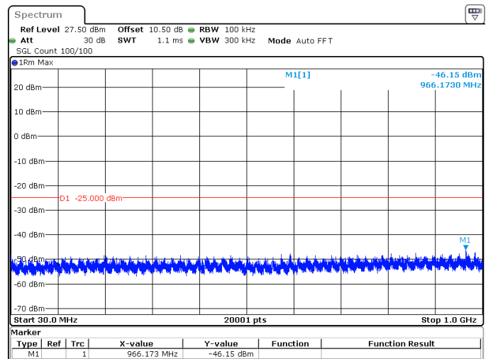
5MHz_15kHz_2567.5MHz_DFT-s-OFDM QPSK_RB25@0 -46.15 dBm
