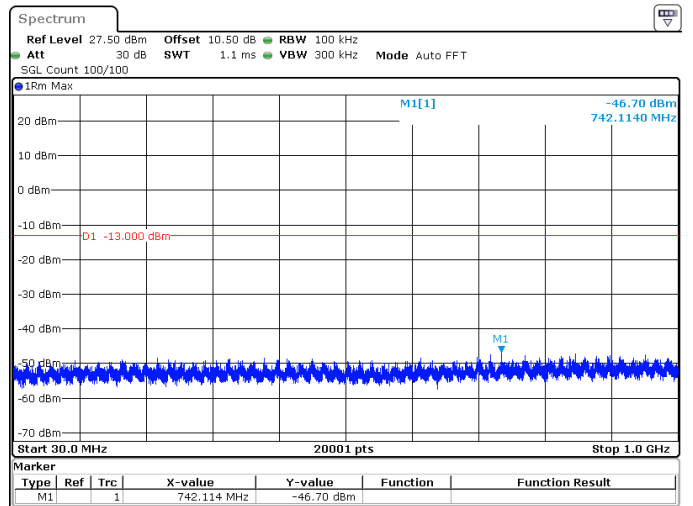
30MHz_15kHz_1745MHz_DFT-s-OFDM QPSK_RB160@0 -46.70 dBm
