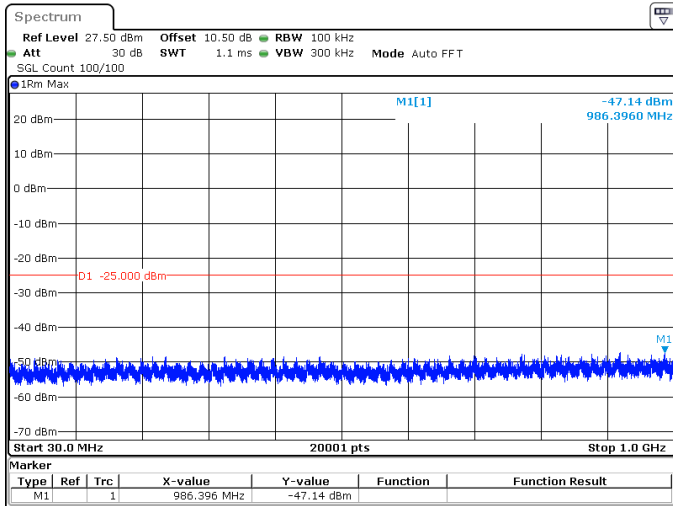
80MHz_30kHz_2592.99MHz_DFT-s-OFDM QPSK_RB1@0 -47.14 dBm
