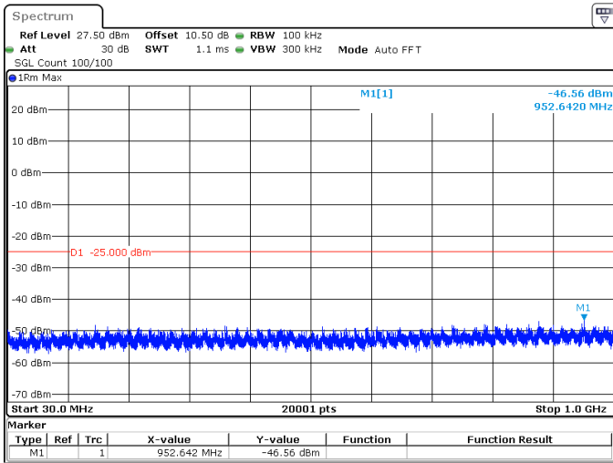
5MHz_15kHz_2502.5MHz_DFT-s-OFDM QPSK_RB1@24 -46.56 dBm
