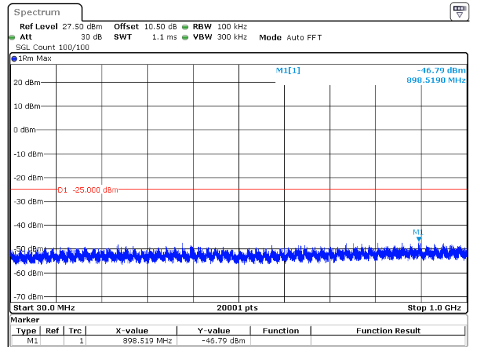
90MHz_30kHz_2592.99MHz_DFT-s-OFDM QPSK_RB1@244 -46.79 dBm
