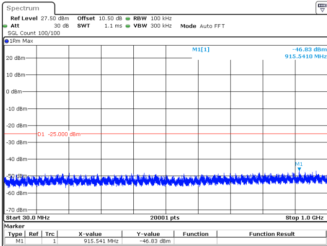
80MHz_30kHz_2536.02MHz_DFT-s-OFDM QPSK_RB1@0 -46.83 dBm
