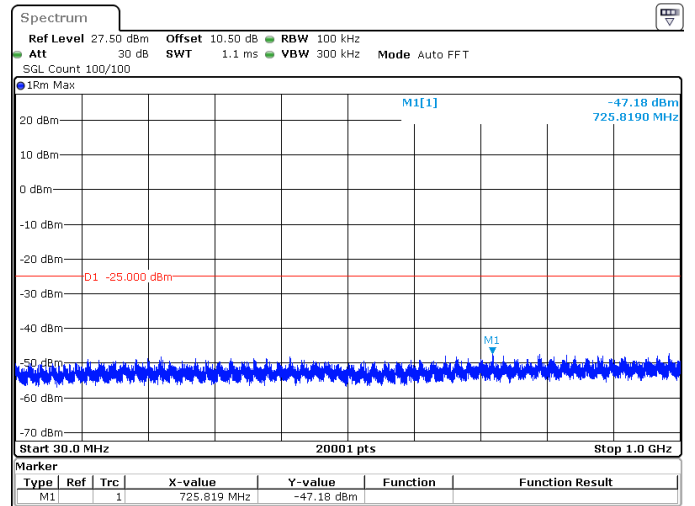
80MHz_30kHz_2592.99MHz_DFT-s-OFDM QPSK_RB1@216 -47.18 dBm
