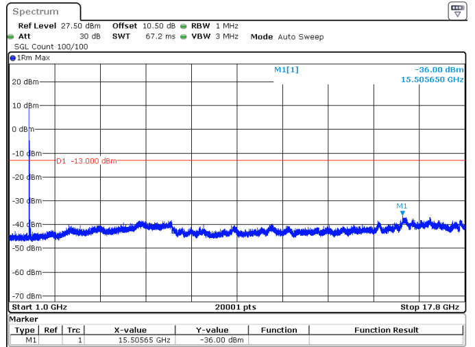
25MHz_15kHz_1745MHz_DFT-s-OFDM QPSK_RB1@0 -36.00 dBm
