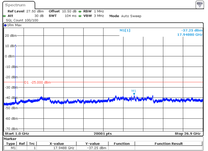
100MHz_30kHz_2546.01MHz_DFT-s-OFDM QPSK_RB1@0 -37.25 dBm
