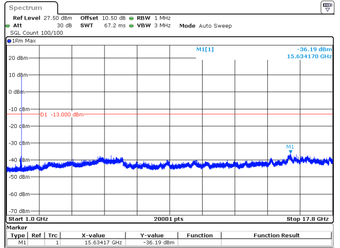
30MHz_15kHz_1745MHz_DFT-s-OFDM QPSK_RB1@159 -36.19 dBm
