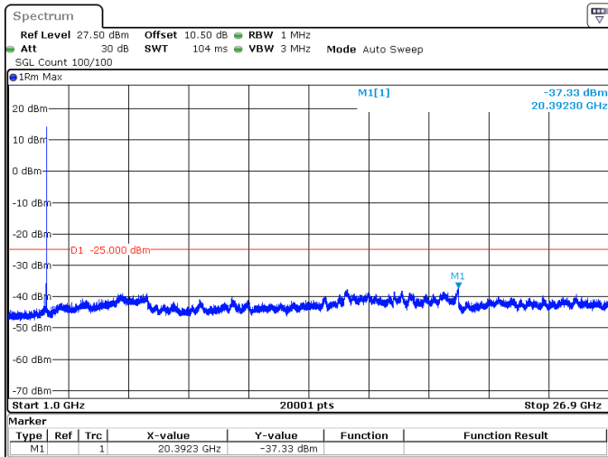
80MHz_30kHz_2592.99MHz_DFT-s-OFDM QPSK_RB1@216 -37.33 dBm
