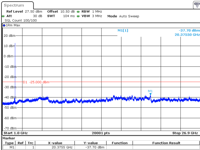
90MHz_30kHz_2592.99MHz_DFT-s-OFDM QPSK_RB1@244 -37.70 dBm
