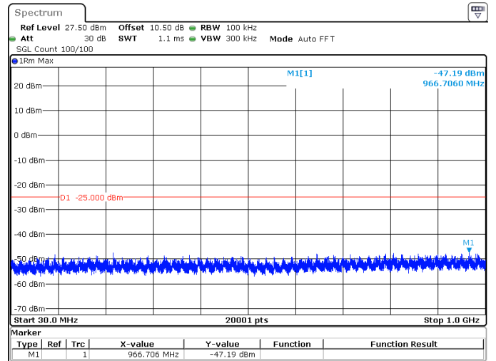
5MHz_15kHz_2567.5MHz_DFT-s-OFDM QPSK_RB1@24 -47.19 dBm
