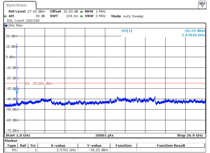
90MHz_30kHz_2592.99MHz_DFT-s-OFDM QPSK_RB1@0 -35.22 dBm
