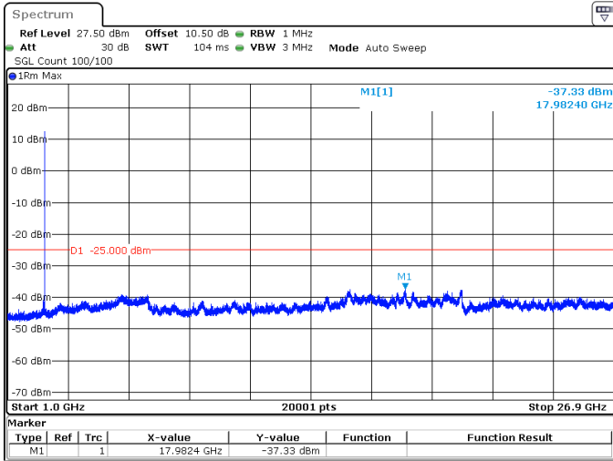
80MHz_30kHz_2536.02MHz_DFT-s-OFDM QPSK_RB1@216 -37.33 dBm
