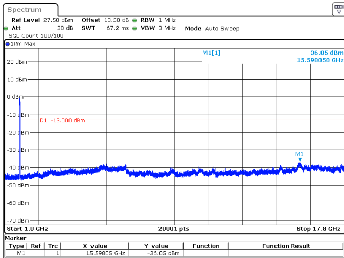
25MHz_15kHz_1745MHz_DFT-s-OFDM QPSK_RB128@0 -36.05 dBm
