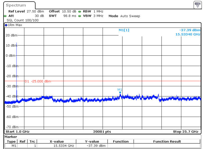
5MHz_15kHz_2502.5MHz_DFT-s-OFDM QPSK_RB1@24 -37.39 dBm
