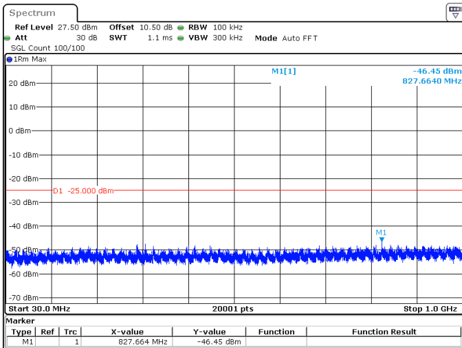
80MHz_30kHz_2536.02MHz_DFT-s-OFDM QPSK_RB216@0 -46.45 dBm
