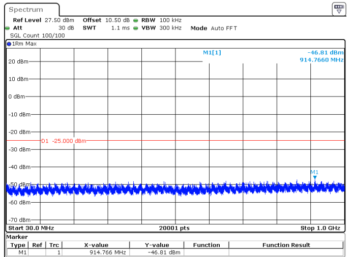
100MHz_30kHz_2546.01MHz_DFT-s-OFDM QPSK_RB270@0 -46.81 dBm
