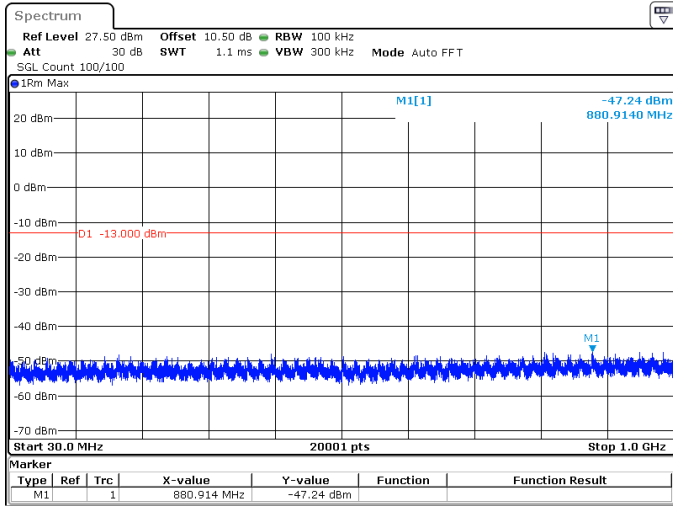
25MHz_15kHz_1745MHz_DFT-s-OFDM QPSK_RB1@132 -47.24 dBm
