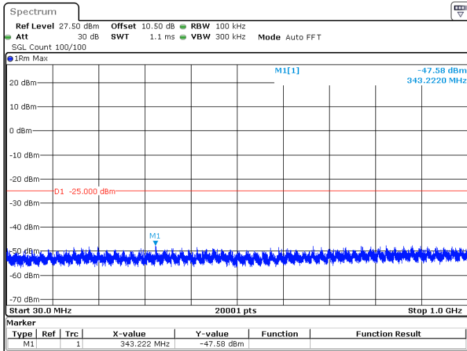
50MHz_15kHz_2664.99MHz_DFT-s-OFDM QPSK_RB1@0 -47.58 dBm
