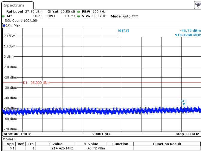
15MHz_30kHz_2592.99MHz_DFT-s-OFDM QPSK_RB1@37 -46.72 dBm
