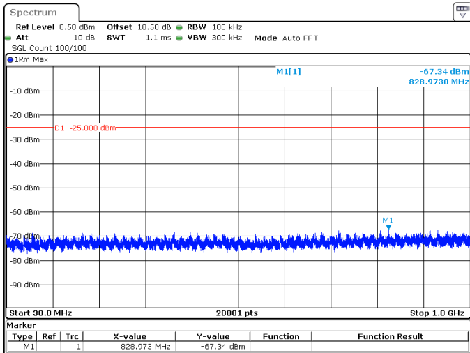
40MHz_15kHz_2516.01MHz_DFT-s-OFDM QPSK_RB1@215 -67.34 dBm
