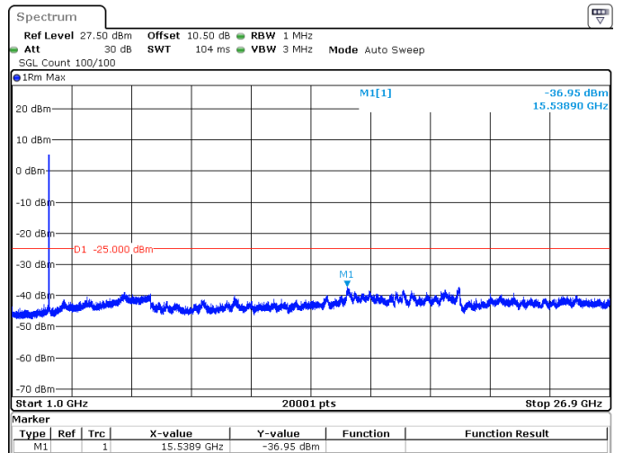
15MHz_30kHz_2592.99MHz_DFT-s-OFDM QPSK_RB36@0 -36.95 dBm
