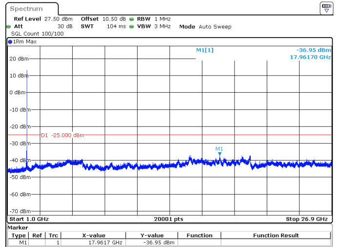
40MHz_15kHz_2516.01MHz_DFT-s-OFDM QPSK_RB1@215 -36.95 dBm
