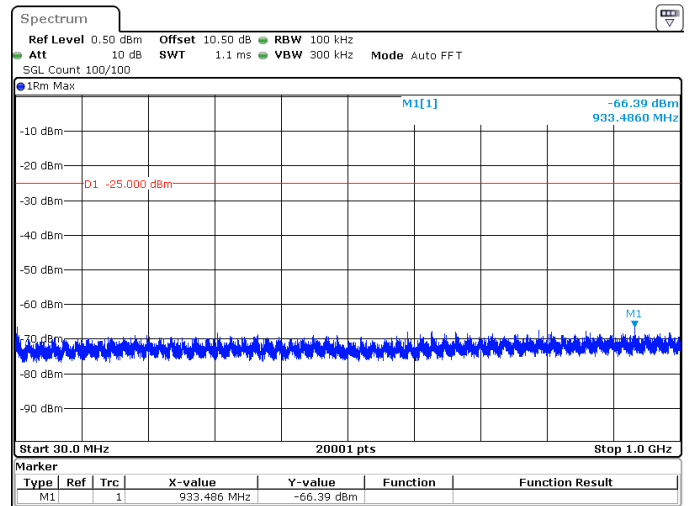
40MHz_30kHz_2516.01MHz_DFT-s-OFDM QPSK_RB100@0 -66.39 dBm
