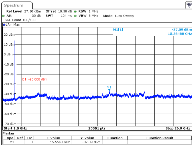
30MHz_30kHz_2592.99MHz_DFT-s-OFDM QPSK_RB1@0 -37.09 dBm
