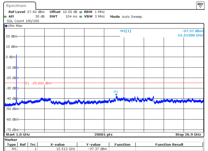
40MHz_15kHz_2516.01MHz_DFT-s-OFDM QPSK_RB216@0 -37.37 dBm
