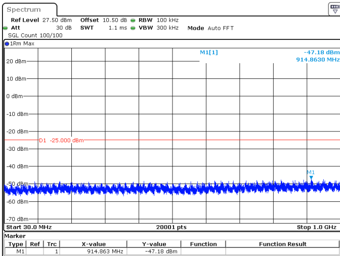
60MHz_30kHz_2592.99MHz_DFT-s-OFDM QPSK_RB162@0 -47.18 dBm
