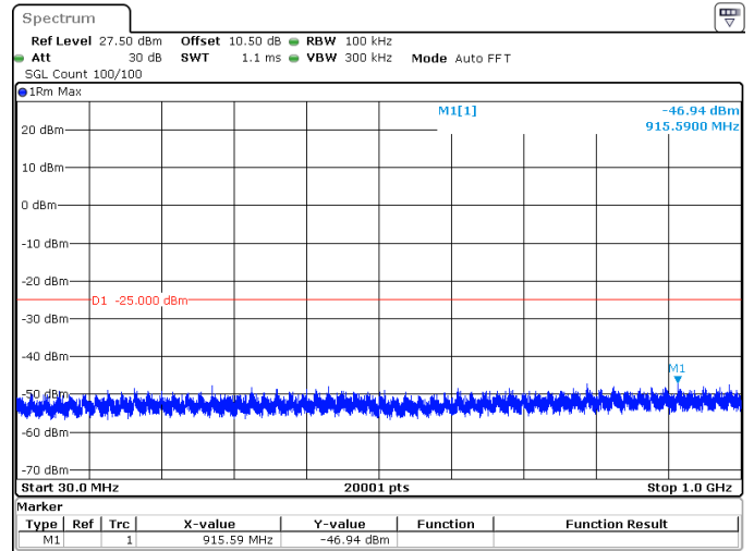
40MHz_30kHz_2516.01MHz_DFT-s-OFDM QPSK_RB1@0 -46.94 dBm
