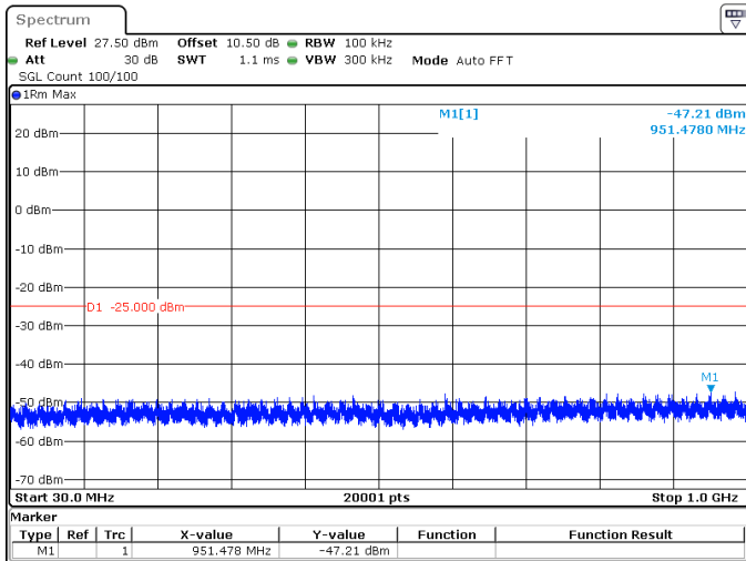
30MHz_30kHz_2592.99MHz_DFT-s-OFDM QPSK_RB1@77 -47.21 dBm
