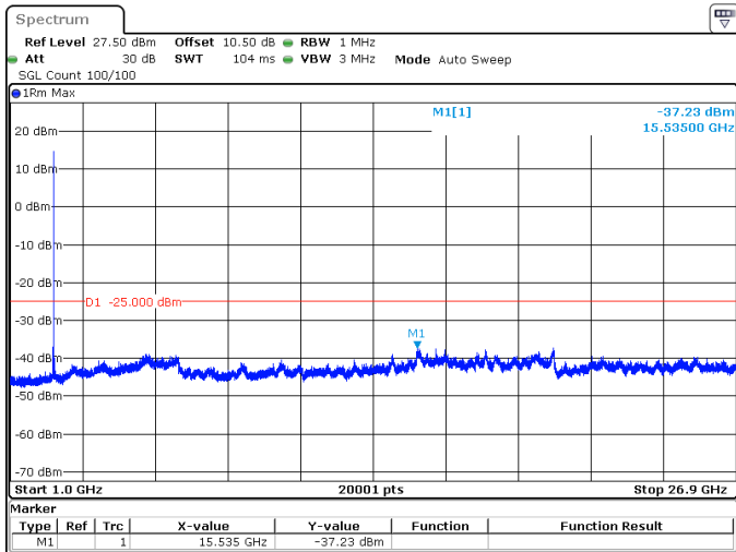
40MHz_30kHz_2516.01MHz_DFT-s-OFDM QPSK_RB1@105 -37.23 dBm
