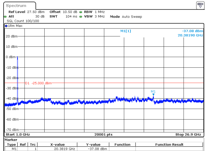
50MHz_15kHz_2664.99MHz_DFT-s-OFDM QPSK_RB270@0 -37.08 dBm
