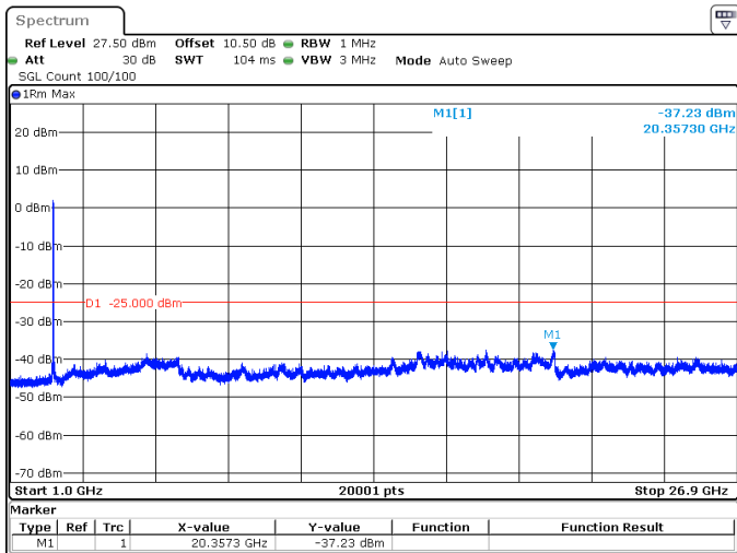
40MHz_30kHz_2516.01MHz_DFT-s-OFDM QPSK_RB100@0 -37.23 dBm
