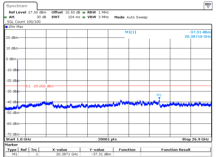
60MHz_30kHz_2592.99MHz_DFT-s-OFDM QPSK_RB162@0 -37.31 dBm
