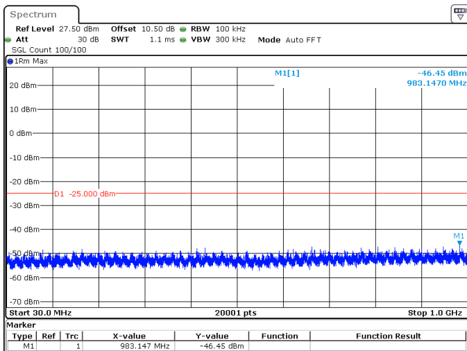
30MHz_30kHz_2592.99MHz_DFT-s-OFDM QPSK_RB75@0 -46.45 dBm
