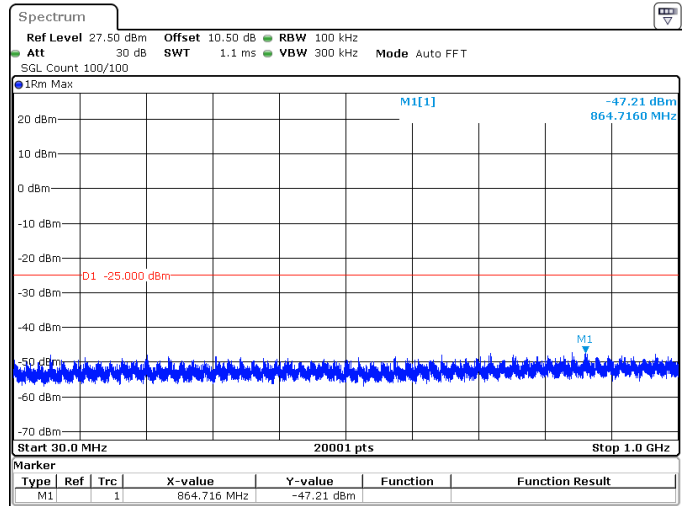
15MHz_30kHz_2592.99MHz_DFT-s-OFDM QPSK_RB1@0 -47.21 dBm
