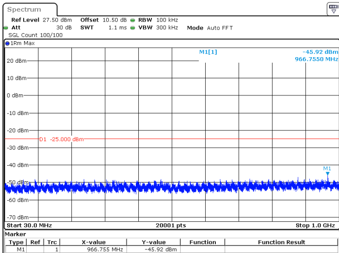
40MHz_15kHz_2516.01MHz_DFT-s-OFDM QPSK_RB216@0 -45.92 dBm
