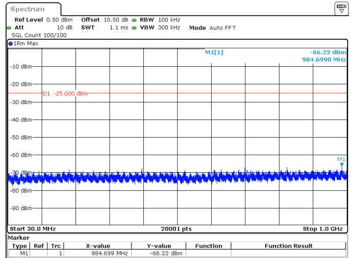
40MHz_30kHz_2516.01MHz_DFT-s-OFDM QPSK_RB1@105 -66.22 dBm
