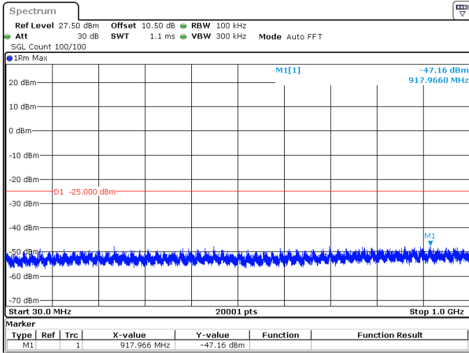
60MHz_30kHz_2592.99MHz_DFT-s-OFDM QPSK_RB1@161 -47.16 dBm
