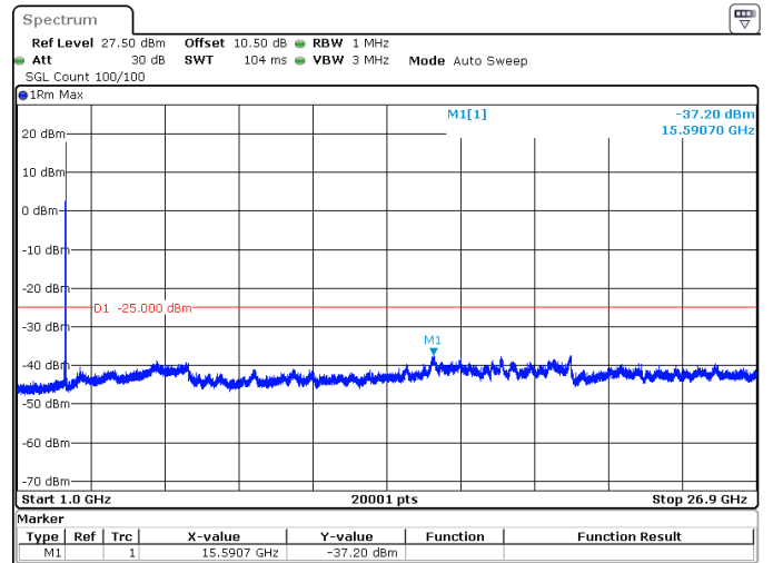
50MHz_15kHz_2664.99MHz_DFT-s-OFDM QPSK_RB1@269 -37.20 dBm
