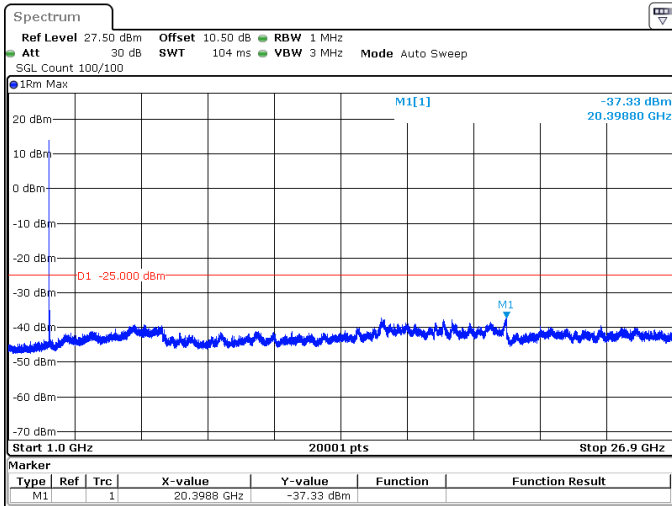
15MHz_30kHz_2592.99MHz_DFT-s-OFDM QPSK_RB1@0 -37.33 dBm
