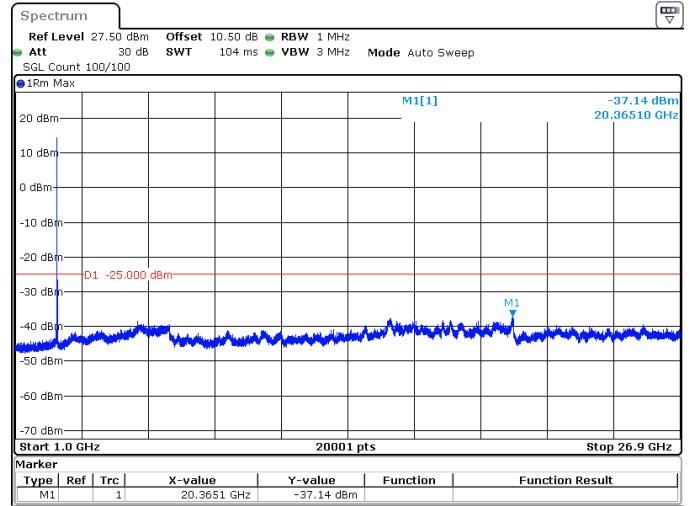
60MHz_30kHz_2592.99MHz_DFT-s-OFDM QPSK_RB1@161 -37.14 dBm
