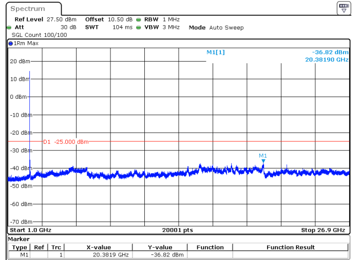
50MHz_15kHz_2664.99MHz_DFT-s-OFDM QPSK_RB1@0 -36.82 dBm
