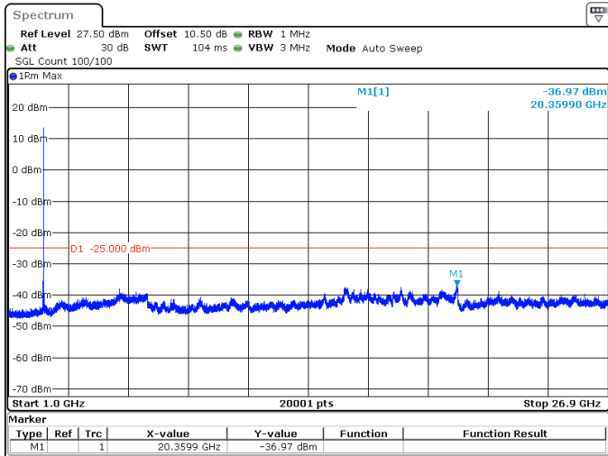
40MHz_15kHz_2516.01MHz_DFT-s-OFDM QPSK_RB1@0 -36.97 dBm
