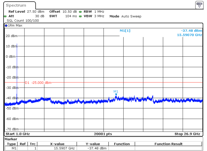
30MHz_30kHz_2592.99MHz_DFT-s-OFDM QPSK_RB1@77 -37.48 dBm
