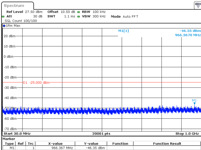
15MHz_30kHz_2592.99MHz_DFT-s-OFDM QPSK_RB36@0 -46.35 dBm
