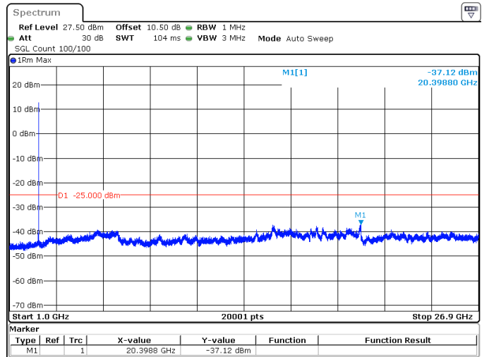
15MHz_30kHz_2592.99MHz_DFT-s-OFDM QPSK_RB1@37 -37.12 dBm
