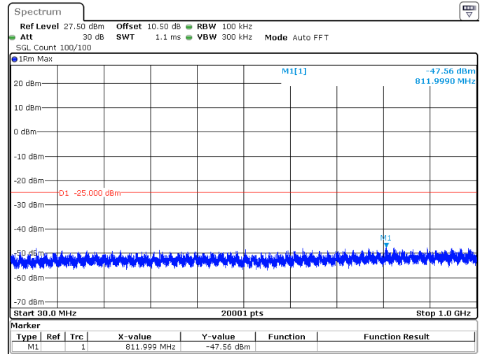
40MHz_15kHz_2516.01MHz_DFT-s-OFDM QPSK_RB1@0 -47.56 dBm
