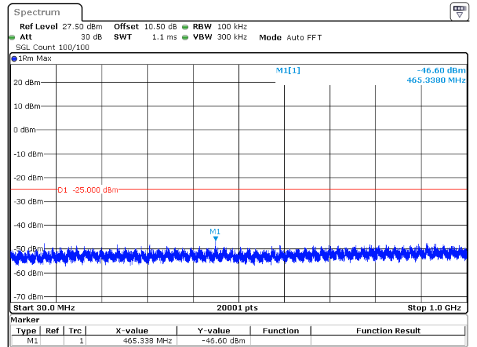
20MHz_30kHz_2592.99MHz_DFT-s-OFDM QPSK_RB1@50 -46.60 dBm
