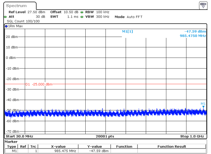
30MHz_30kHz_2592.99MHz_DFT-s-OFDM QPSK_RB1@0 -47.59 dBm
