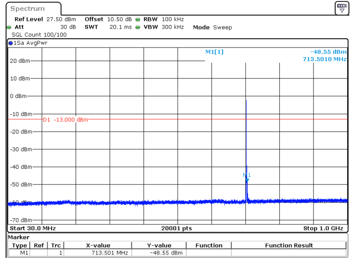
5MHz_15kHz_713.5MHz_DFT-s-OFDM QPSK_RB1@0 -48.55 dBm
