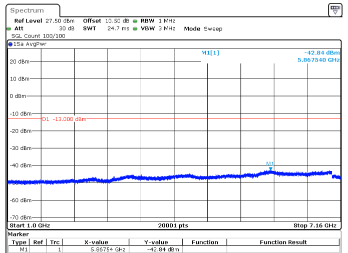
5MHz_15kHz_713.5MHz_DFT-s-OFDM QPSK_RB25@0 -42.84 dBm
