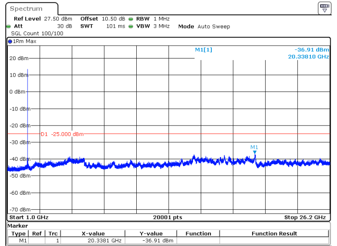
5MHz_15kHz_2572.5MHz_DFT-s-OFDM QPSK_RB1@24 -36.91 dBm
