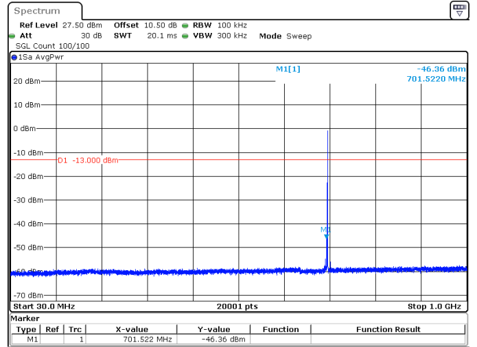
5MHz_15kHz_701.5MHz_DFT-s-OFDM QPSK_RB1@24 -46.36 dBm
