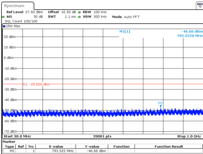
10MHz_15kHz_2501.01MHz_DFT-s-OFDM QPSK_RB1@0 -46.66 dBm
