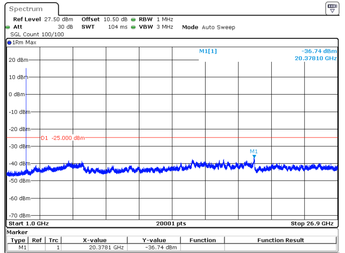
10MHz_15kHz_2501.01MHz_DFT-s-OFDM QPSK_RB1@51 -36.74 dBm
