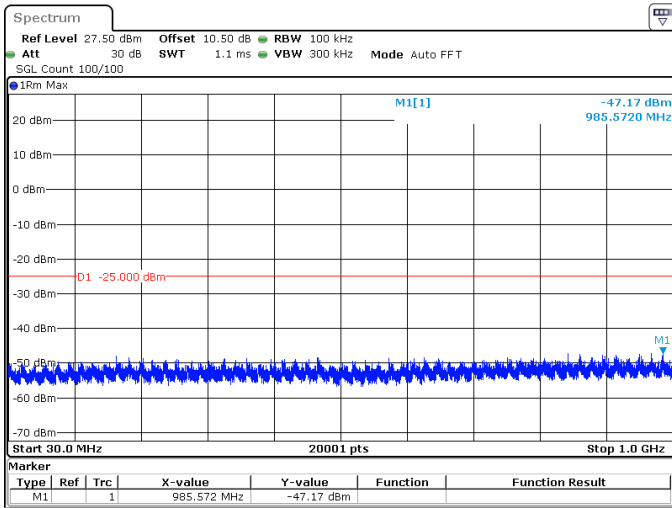
10MHz_15kHz_2501.01MHz_DFT-s-OFDM QPSK_RB1@51 -47.17 dBm
