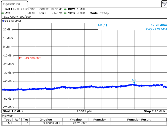
5MHz_15kHz_701.5MHz_DFT-s-OFDM QPSK_RB1@24 -42.78 dBm
