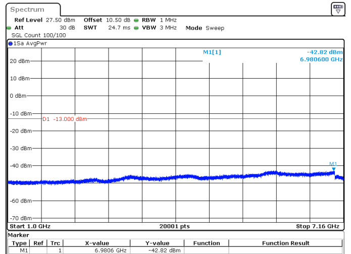
5MHz_15kHz_701.5MHz_DFT-s-OFDM QPSK_RB25@0 -42.82 dBm
