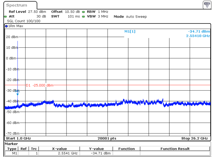
5MHz_15kHz_2572.5MHz_DFT-s-OFDM QPSK_RB1@0 -34.71 dBm
