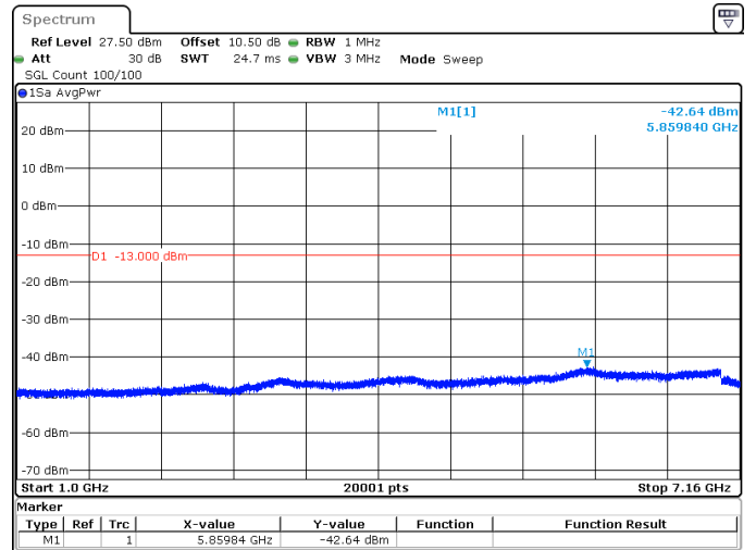
5MHz_15kHz_713.5MHz_DFT-s-OFDM QPSK_RB1@24 -42.64 dBm
