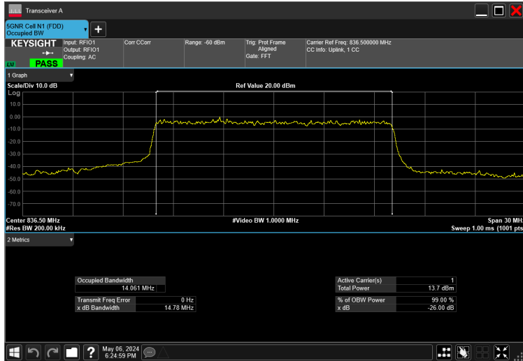
15MHz_15kHz_836.5MHz_CP-OFDM 16 QAM_RB79@0 14.061 MHz
