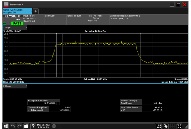
20MHz_15kHz_836.5MHz_DFT-s-OFDM \pi/2 BPSK_RB100@0 18.736 MHz
