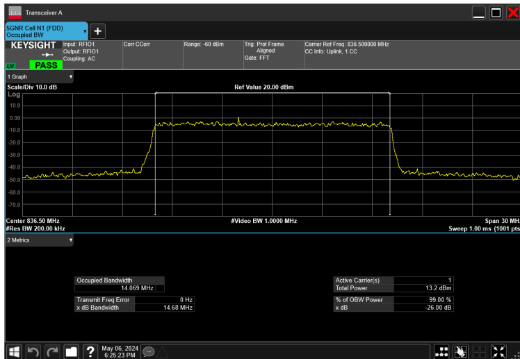
15MHz_15kHz_836.5MHz_CP-OFDM 64 QAM_RB79@0 14.069 MHz
