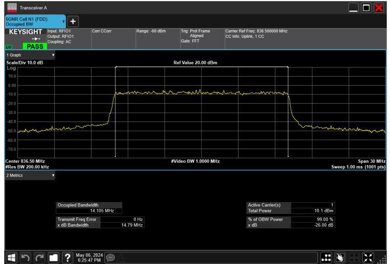
15MHz_15kHz_836.5MHz_CP-OFDM 256 QAM_RB79@0 14.105 MHz
