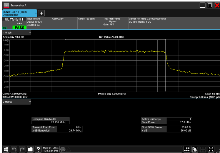
30MHz_15kHz_3840MHz_CP-OFDM QPSK_RB160@0 28.499 MHz
