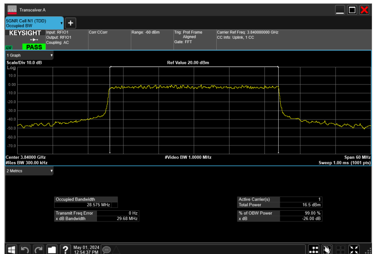
30MHz_15kHz_3840MHz_CP-OFDM 64 QAM_RB160@0 28.575 MHz
