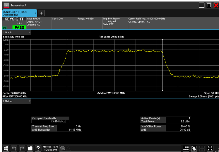
15MHz_30kHz_3840MHz_CP-OFDM 64 QAM_RB38@0 13.574 MHz
