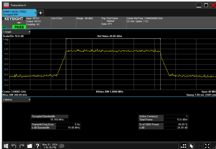
20MHz_30kHz_3840MHz_CP-OFDM 64 QAM_RB51@0 18.169 MHz
