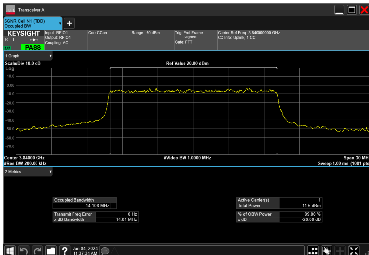
15MHz_15kHz_3840MHz_CP-OFDM 256 QAM_RB79@0 14.108 MHz
