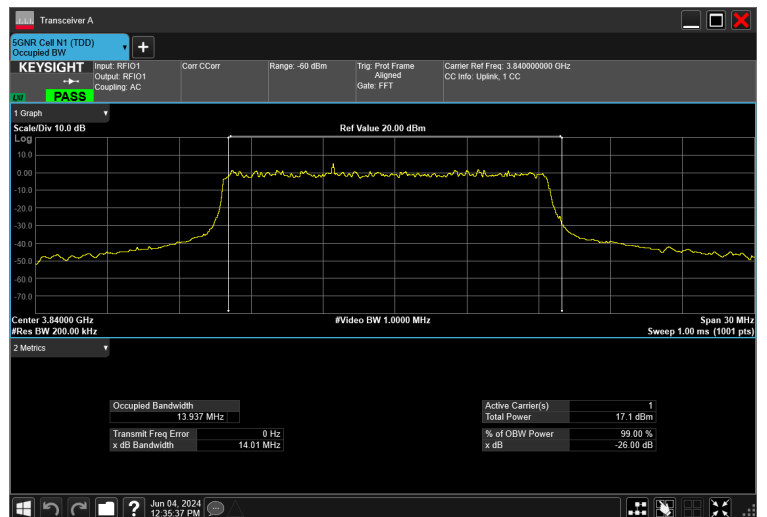
15MHz_15kHz_3840MHz_DFT-s-OFDM \pi/2 BPSK_RB75@0 13.937 MHz
