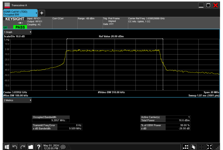
10MHz_15kHz_3840MHz_DFT-s-OFDM 64 QAM_RB50@0 9.206 MHz
