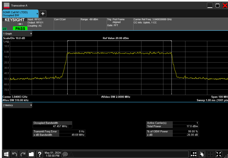
50MHz_30kHz_3840MHz_CP-OFDM QPSK_RB133@0 47.457 MHz
