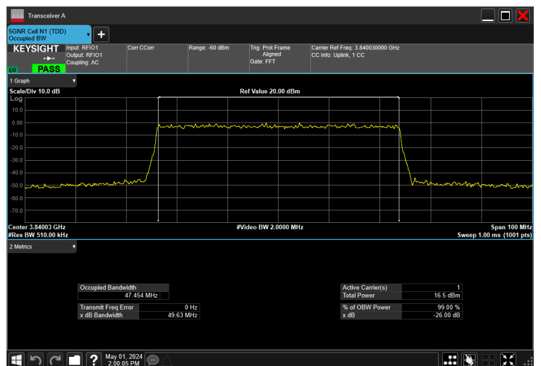
50MHz_30kHz_3840MHz_CP-OFDM 64 QAM_RB133@0 47.454 MHz
