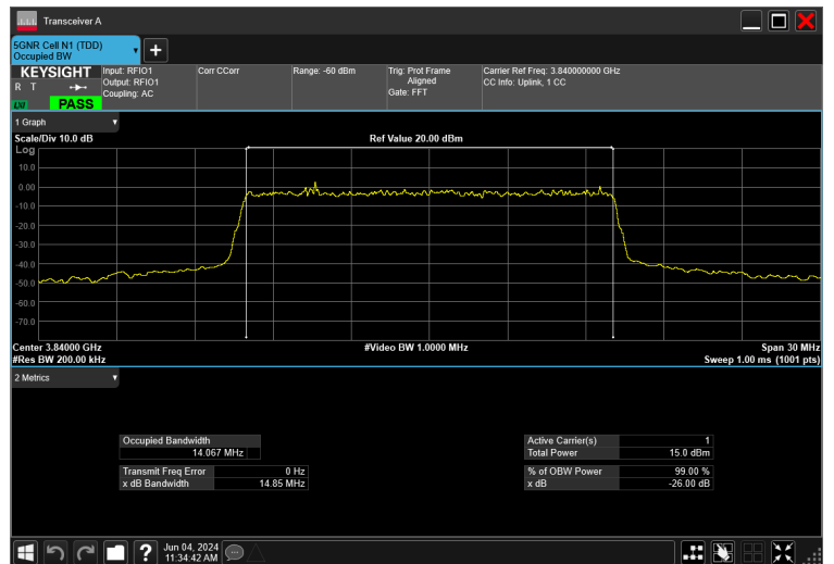
15MHz_15kHz_3840MHz_CP-OFDM 16 QAM_RB79@0 14.067 MHz
