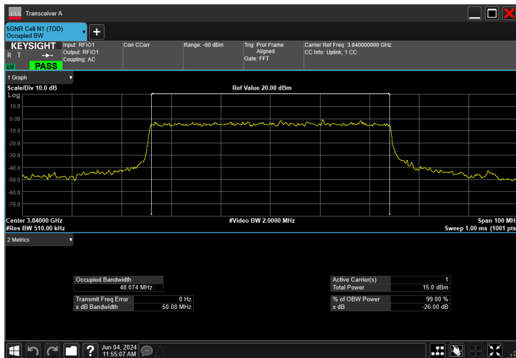
50MHz_15kHz_3840MHz_CP-OFDM 64 QAM_RB270@0 48.074 MHz
