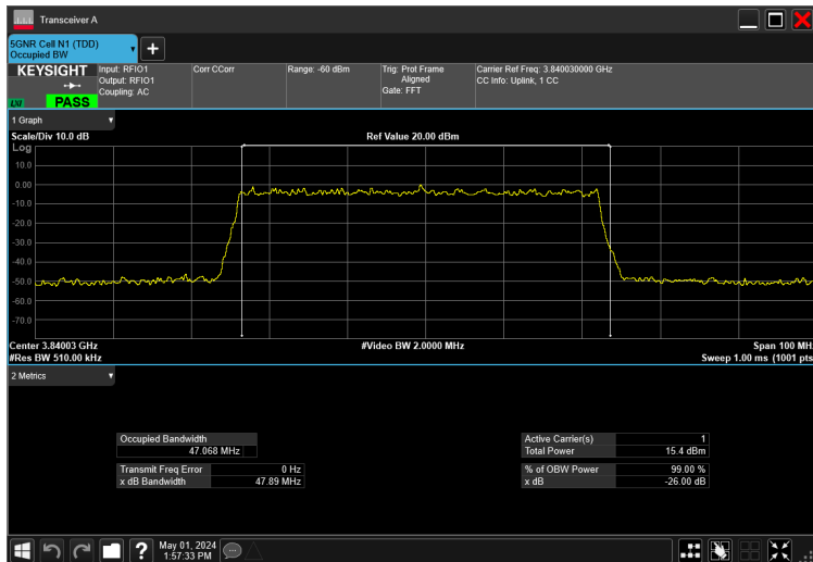
50MHz_30kHz_3840MHz_DFT-s-OFDM 256 QAM_RB128@0 47.068 MHz
