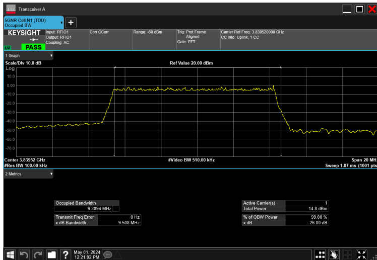
10MHz_15kHz_3840MHz_DFT-s-OFDM 256 QAM_RB50@0 9.209 MHz
