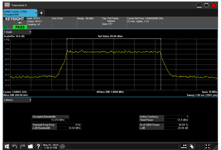
15MHz_30kHz_3840MHz_CP-OFDM 256 QAM_RB38@0 13.576 MHz
