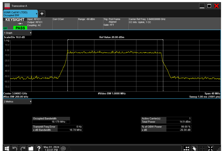
20MHz_30kHz_3840MHz_DFT-s-OFDM 256 QAM_RB50@0 18.179 MHz
