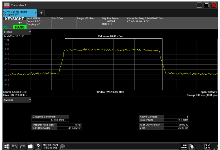
50MHz_30kHz_3840MHz_DFT-s-OFDM 16 QAM_RB128@0 47.026 MHz
