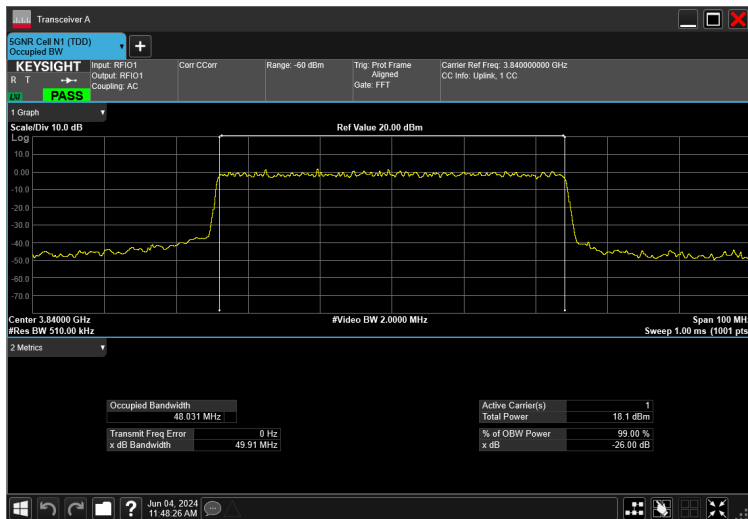
50MHz_15kHz_3840MHz_DFT-s-OFDM \pi/2 BPSK_RB270@0 48.031 MHz
