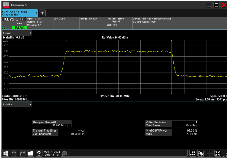
60MHz_30kHz_3840MHz_CP-OFDM 64 QAM_RB162@0 57.695 MHz
