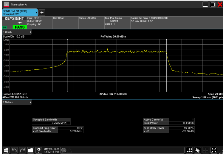
10MHz_15kHz_3840MHz_CP-OFDM QPSK_RB52@0 9.251 MHz
