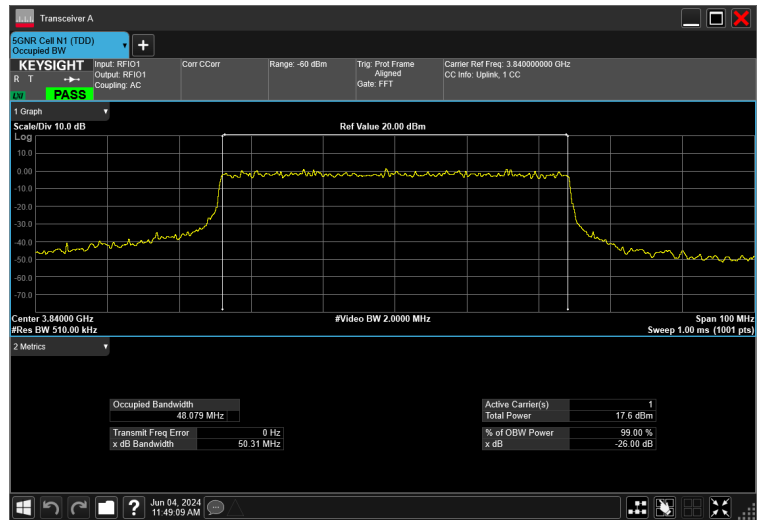
50MHz_15kHz_3840MHz_DFT-s-OFDM QPSK_RB270@0 48.079 MHz
