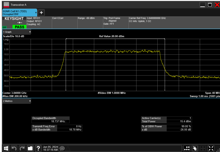
20MHz_15kHz_3840MHz_DFT-s-OFDM 256 QAM_RB100@0 18.737 MHz
