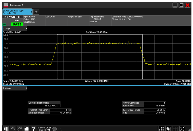
50MHz_30kHz_3840MHz_DFT-s-OFDM \pi/2 BPSK_RB128@0 46.800 MHz
