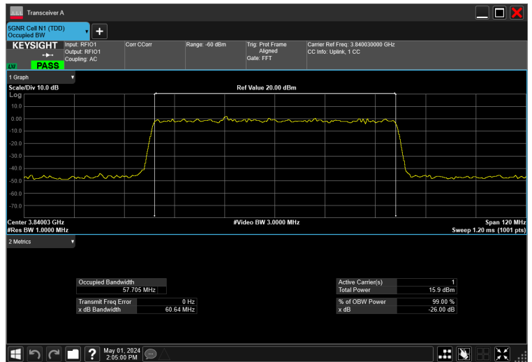
60MHz_30kHz_3840MHz_DFT-s-OFDM 256 QAM_RB162@0 57.705 MHz
