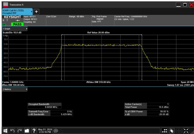
10MHz_30kHz_3840MHz_DFT-s-OFDM 64 QAM_RB24@0 8.606 MHz
