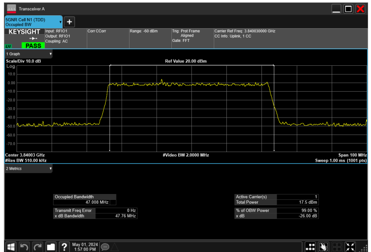
50MHz_30kHz_3840MHz_DFT-s-OFDM 64 QAM_RB128@0 47.008 MHz
