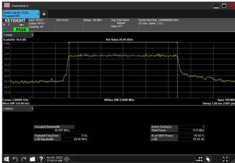
50MHz_15kHz_3840MHz_DFT-s-OFDM 64 QAM_RB270@0 48.065 MHz
