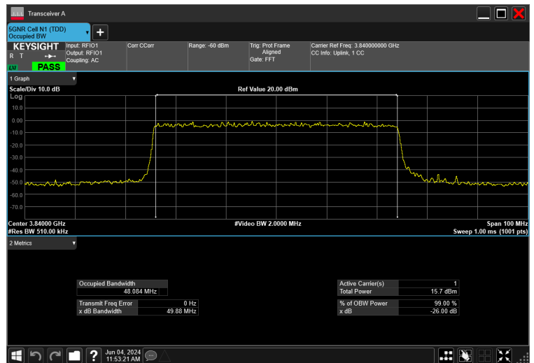
50MHz_15kHz_3840MHz_CP-OFDM QPSK_RB270@0 48.084 MHz
