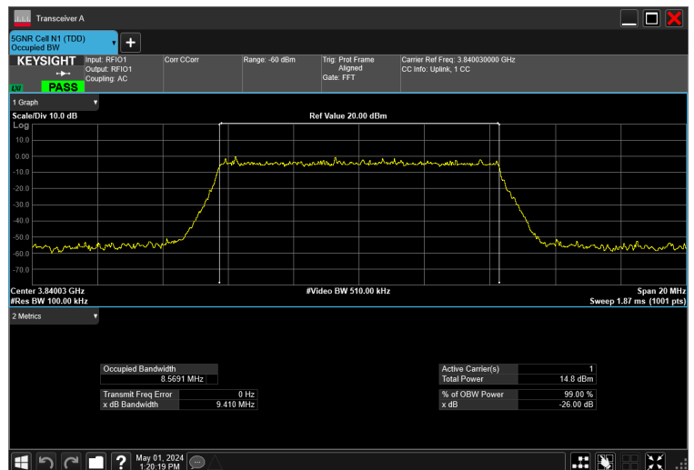
10MHz_30kHz_3840MHz_DFT-s-OFDM 256 QAM_RB24@0 8.569 MHz
