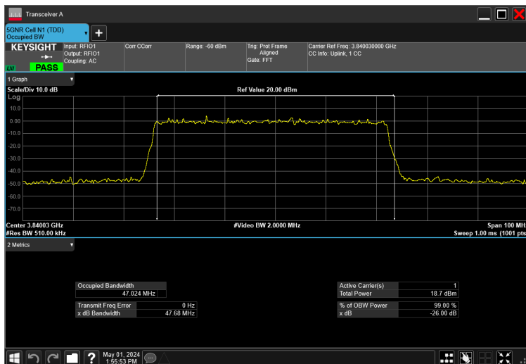
50MHz_30kHz_3840MHz_DFT-s-OFDM QPSK_RB128@0 47.024 MHz
