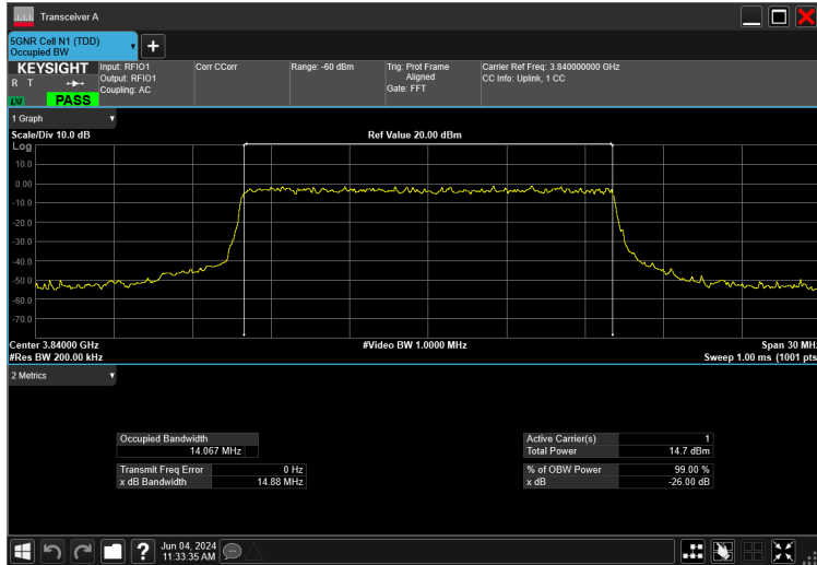
15MHz_15kHz_3840MHz_CP-OFDM QPSK_RB79@0 14.067 MHz
