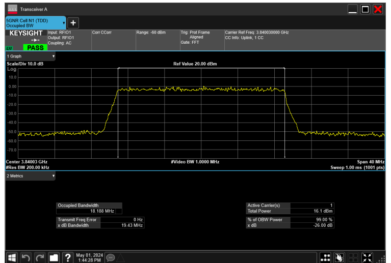
20MHz_30kHz_3840MHz_CP-OFDM QPSK_RB51@0 18.188 MHz
