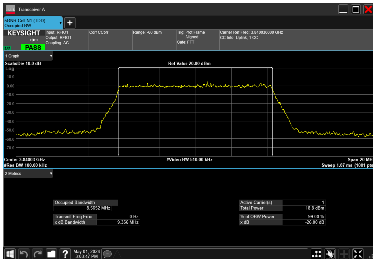
10MHz_30kHz_3840MHz_DFT-s-OFDM \pi/2 BPSK_RB24@0 8.565 MHz
