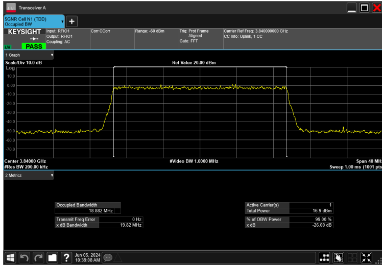
20MHz_15kHz_3840MHz_CP-OFDM QPSK_RB106@0 18.882 MHz
