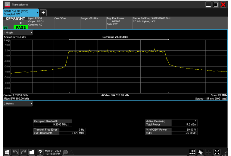
10MHz_15kHz_3840MHz_DFT-s-OFDM 16 QAM_RB50@0 9.200 MHz
