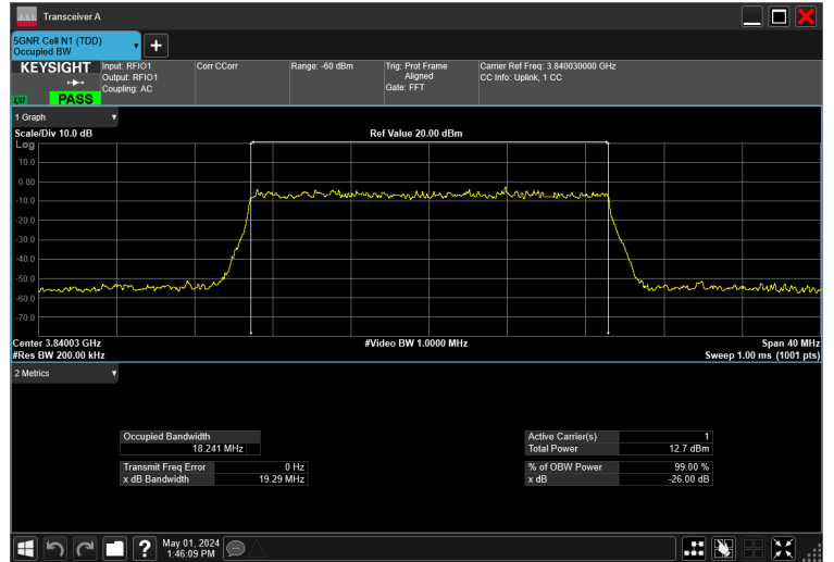
20MHz_30kHz_3840MHz_CP-OFDM 256 QAM_RB51@0 18.241 MHz
