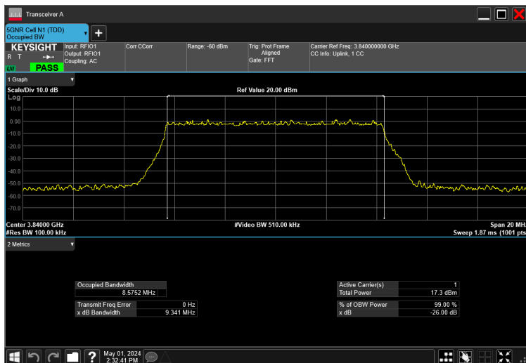
10MHz_30kHz_3840MHz_DFT-s-OFDM 16 QAM_RB24@0 8.575 MHz
