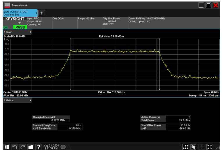
10MHz_30kHz_3840MHz_CP-OFDM QPSK_RB24@0 8.573 MHz
