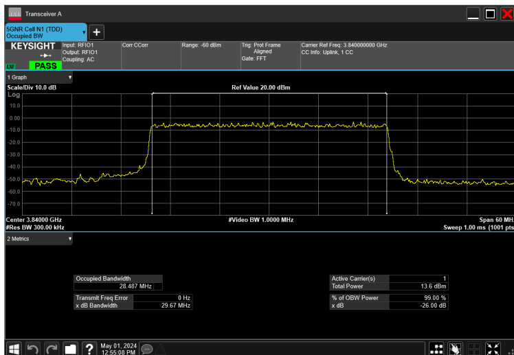
30MHz_15kHz_3840MHz_CP-OFDM 256 QAM_RB160@0 28.487 MHz
