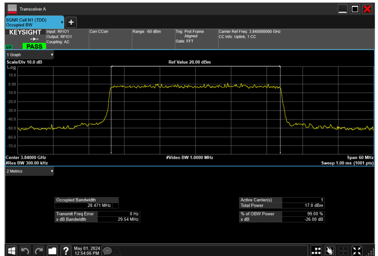
30MHz_15kHz_3840MHz_CP-OFDM 16 QAM_RB160@0 28.471 MHz
