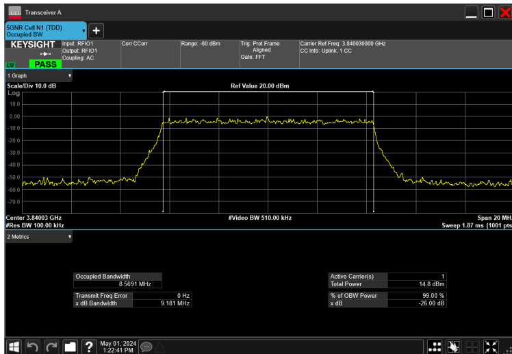
10MHz_30kHz_3840MHz_CP-OFDM 64 QAM_RB24@0 8.569 MHz
