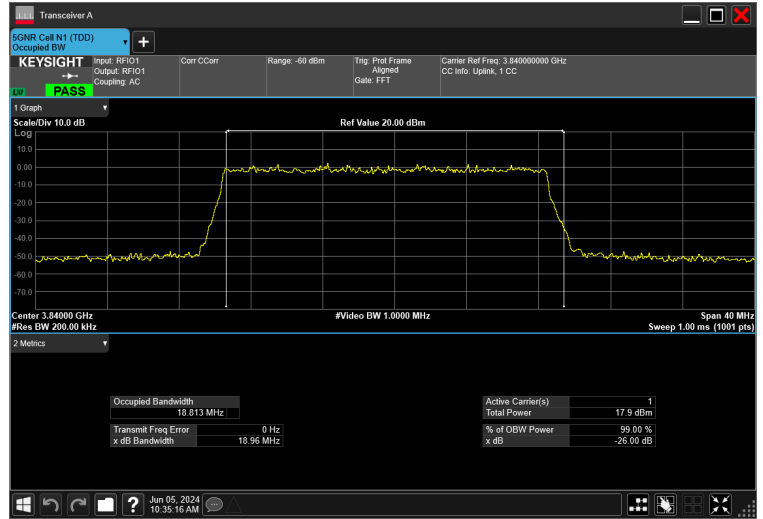
20MHz_15kHz_3840MHz_DFT-s-OFDM 16 QAM_RB100@0 18.813 MHz
