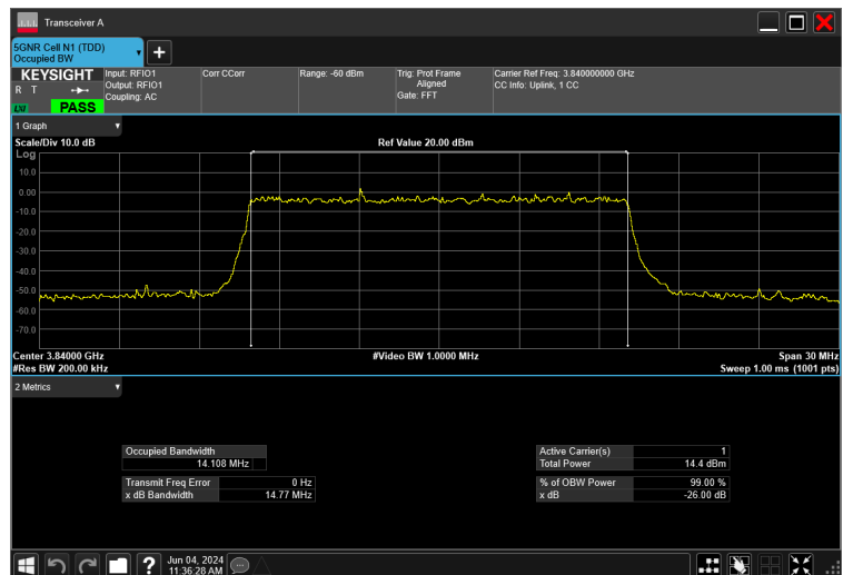
15MHz_15kHz_3840MHz_CP-OFDM 64 QAM_RB79@0 14.108 MHz
