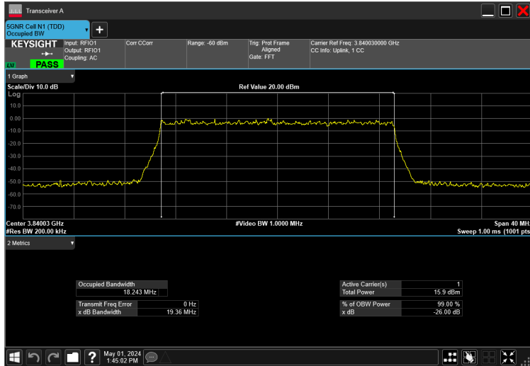
20MHz_30kHz_3840MHz_CP-OFDM 16 QAM_RB51@0 18.243 MHz
