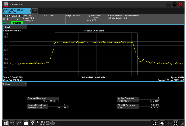
20MHz_15kHz_3840MHz_DFT-s-OFDM \pi/2 BPSK_RB100@0 18.748 MHz
