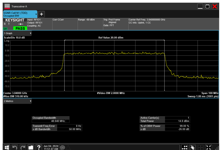
50MHz_15kHz_3840MHz_DFT-s-OFDM 256 QAM_RB270@0 48.040 MHz
