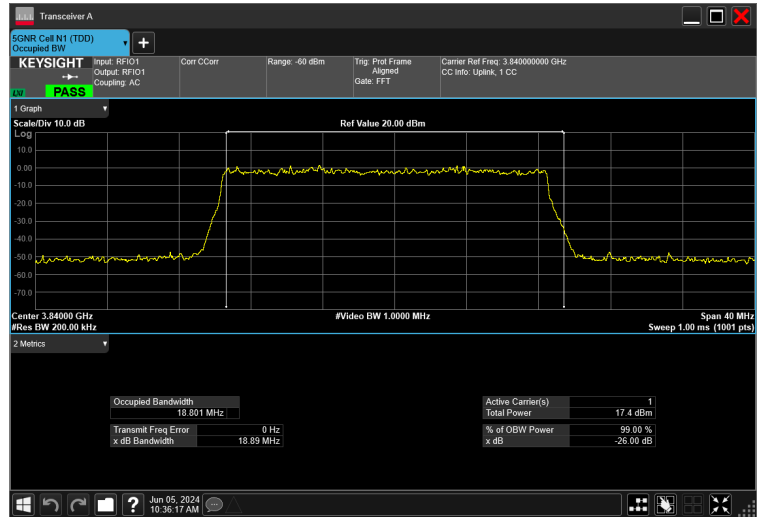
20MHz_15kHz_3840MHz_DFT-s-OFDM 64 QAM_RB100@0 18.801 MHz
