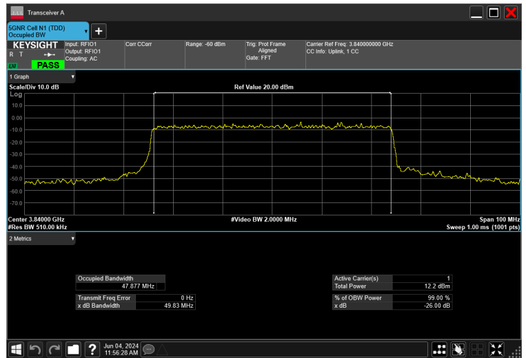
50MHz_15kHz_3840MHz_CP-OFDM 256 QAM_RB270@0 47.877 MHz
