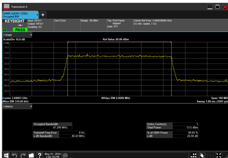
50MHz_30kHz_3840MHz_CP-OFDM 256 QAM_RB133@0 47.290 MHz
