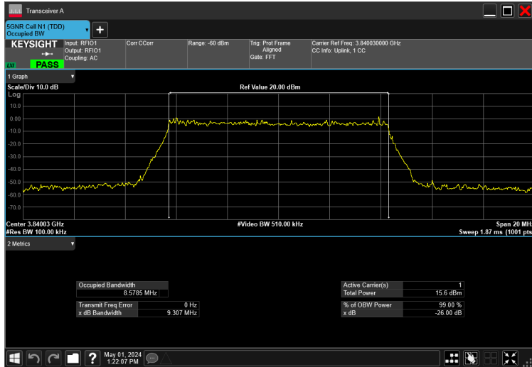
10MHz_30kHz_3840MHz_CP-OFDM 16 QAM_RB24@0 8.578 MHz
