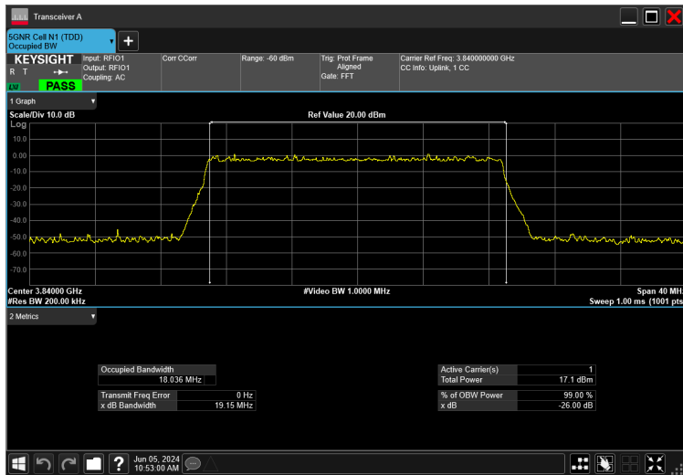
20MHz_30kHz_3840MHz_DFT-s-OFDM 64 QAM_RB50@0 18.036 MHz
