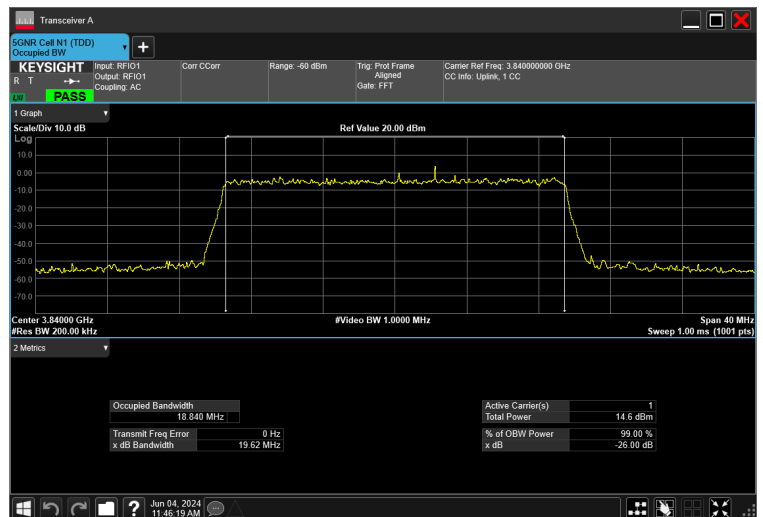
20MHz_15kHz_3840MHz_CP-OFDM 64 QAM_RB106@0 18.840 MHz
