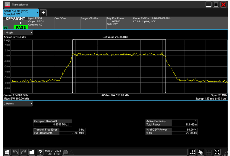
10MHz_30kHz_3840MHz_CP-OFDM 256 QAM_RB24@0 8.579 MHz
