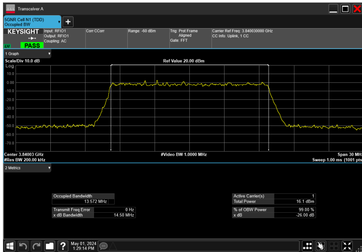
15MHz_30kHz_3840MHz_CP-OFDM 16 QAM_RB38@0 13.572 MHz
