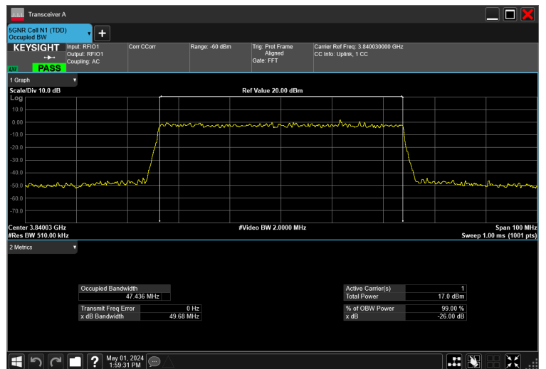
50MHz_30kHz_3840MHz_CP-OFDM 16 QAM_RB133@0 47.436 MHz
