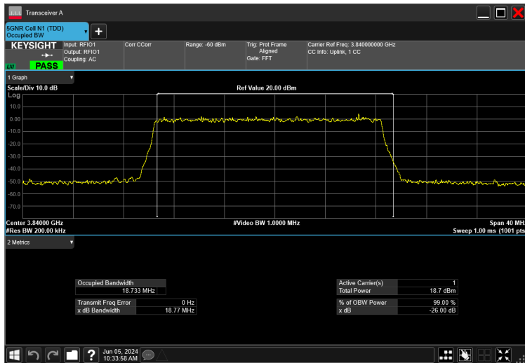
20MHz_15kHz_3840MHz_DFT-s-OFDM QPSK_RB100@0 18.733 MHz
