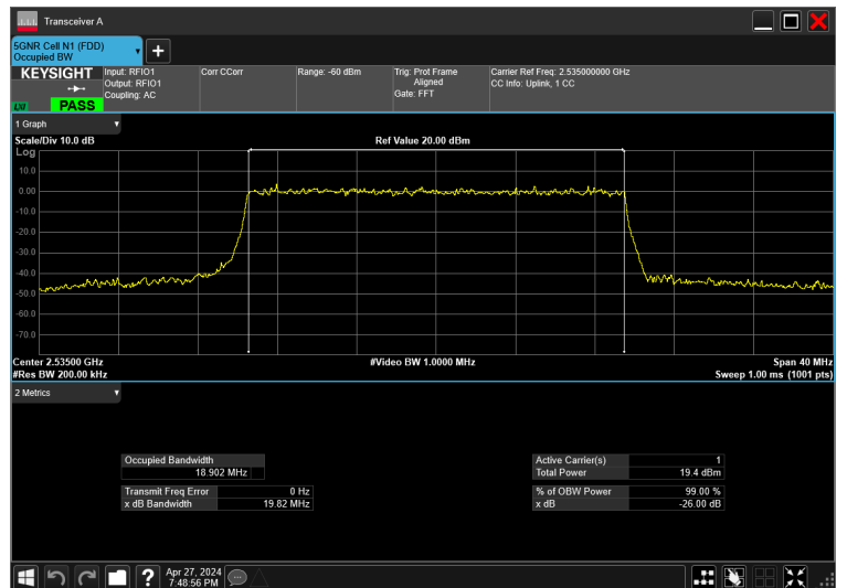
20MHz_15kHz_2535MHz_CP-OFDM QPSK_RB106@0 18.902 MHz
