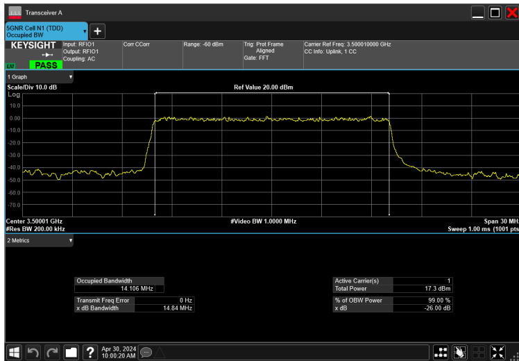
15MHz_15kHz_3500MHz_CP-OFDM QPSK_RB79@0 14.106 MHz
