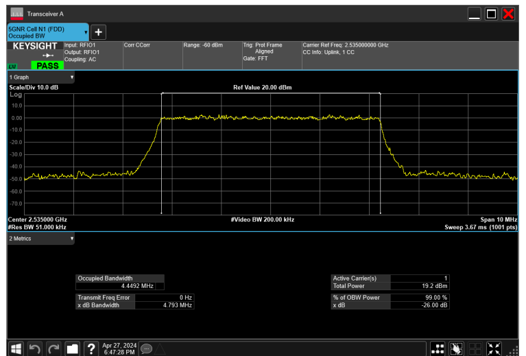
5MHz_15kHz_2535MHz_DFT-s-OFDM 64 QAM_RB25@0 4.449 MHz
