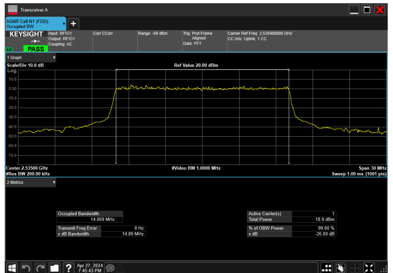
15MHz_15kHz_2535MHz_CP-OFDM 64 QAM_RB79@0 14.069 MHz
