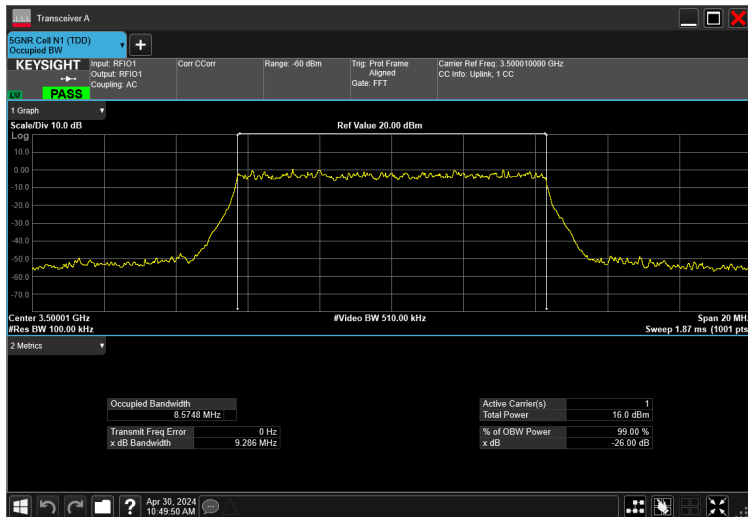
10MHz_30kHz_3500MHz_CP-OFDM 64 QAM_RB24@0 8.575 MHz
