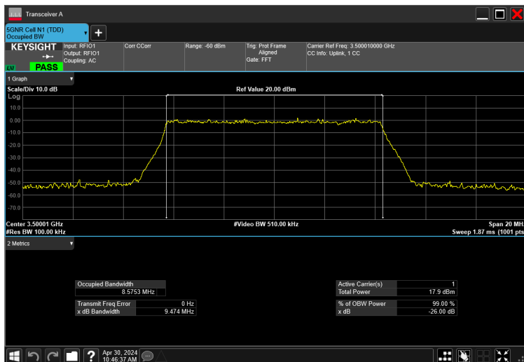
10MHz_30kHz_3500MHz_DFT-s-OFDM 16 QAM_RB24@0 8.575 MHz
