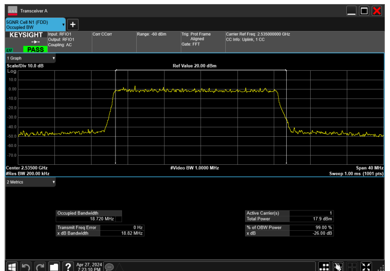
20MHz_15kHz_2535MHz_DFT-s-OFDM 256 QAM_RB100@0 18.720 MHz
