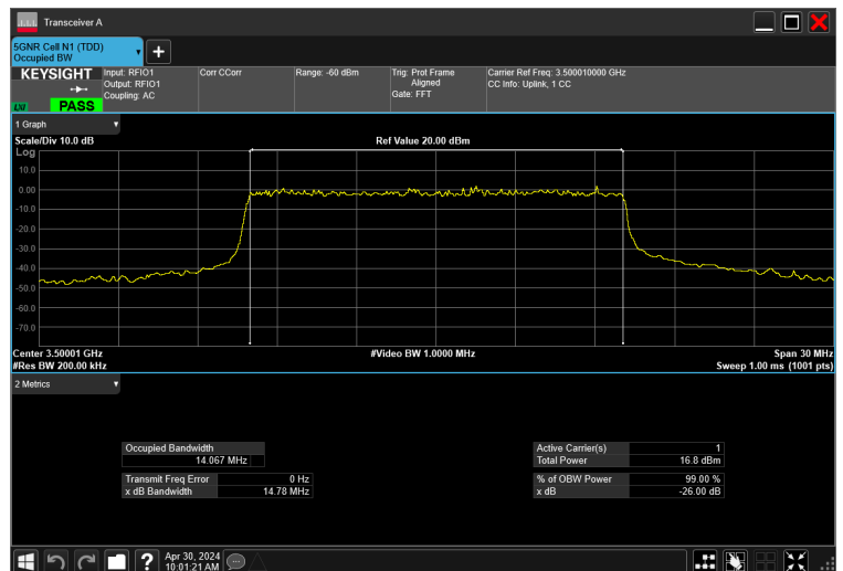
15MHz_15kHz_3500MHz_CP-OFDM 64 QAM_RB79@0 14.067 MHz
