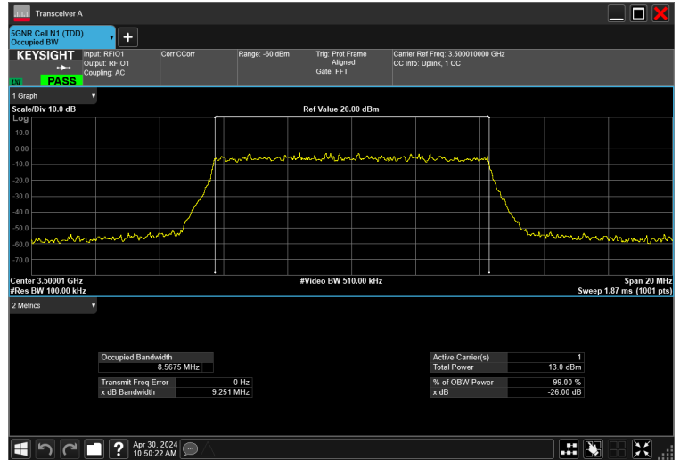
10MHz_30kHz_3500MHz_CP-OFDM 256 QAM_RB24@0 8.567 MHz
