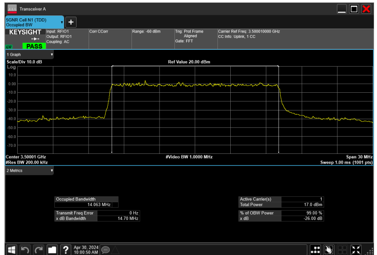
15MHz_15kHz_3500MHz_CP-OFDM 16 QAM_RB79@0 14.063 MHz
