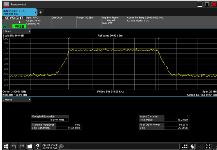
10MHz_30kHz_3500MHz_CP-OFDM 16 QAM_RB24@0 8.611 MHz
