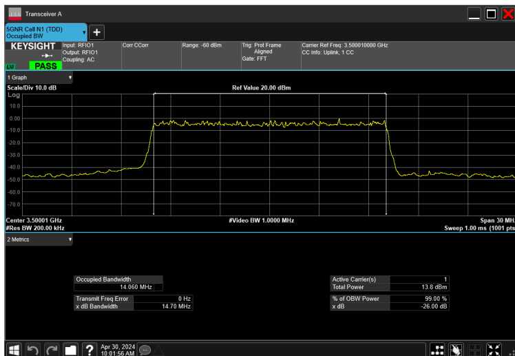
15MHz_15kHz_3500MHz_CP-OFDM 256 QAM_RB79@0 14.060 MHz
