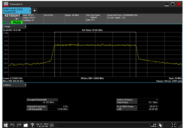
15MHz_15kHz_2535MHz_CP-OFDM 16 QAM_RB79@0 14.102 MHz
