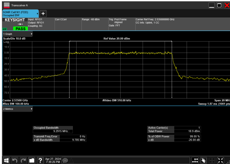
10MHz_15kHz_2535MHz_CP-OFDM 16 QAM_RB52@0 9.291 MHz
