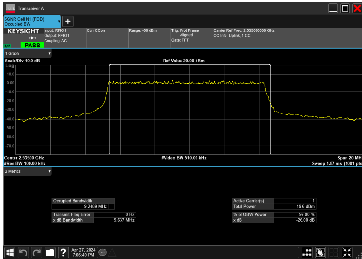
10MHz_15kHz_2535MHz_DFT-s-OFDM 64 QAM_RB50@0 9.249 MHz
