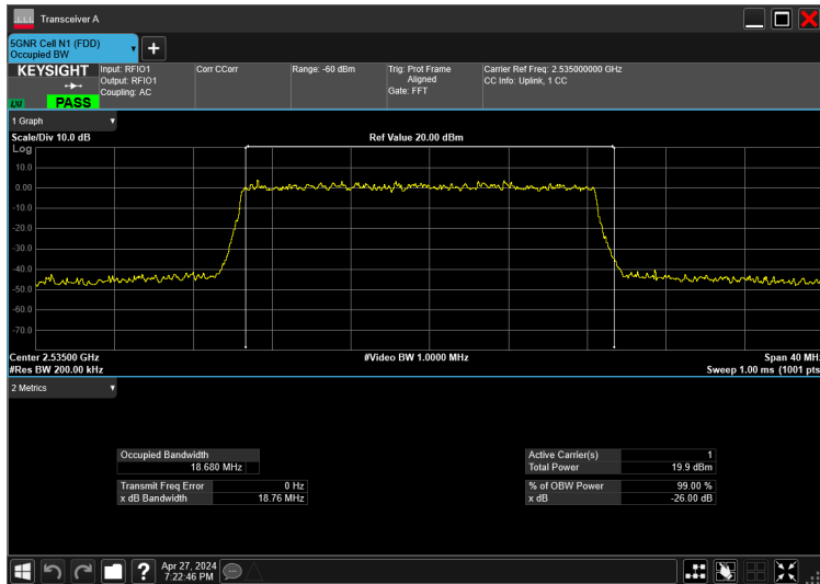
20MHz_15kHz_2535MHz_DFT-s-OFDM 64 QAM_RB100@0 18.680 MHz
