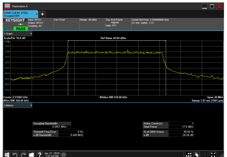
10MHz_15kHz_2535MHz_DFT-s-OFDM 256 QAM_RB50@0 9.205 MHz
