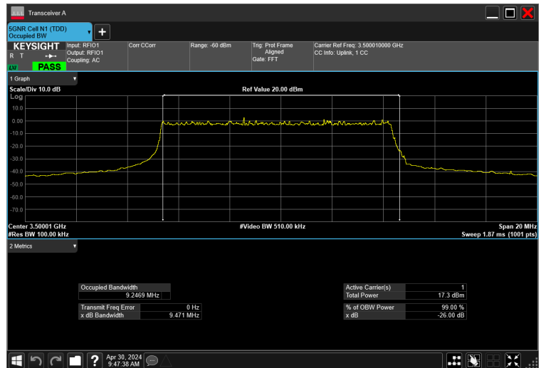
10MHz_15kHz_3500MHz_DFT-s-OFDM 64 QAM_RB50@0 9.247 MHz
