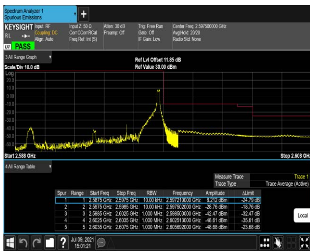
Band41-5MHz-QPSK-40640-1RB#24
