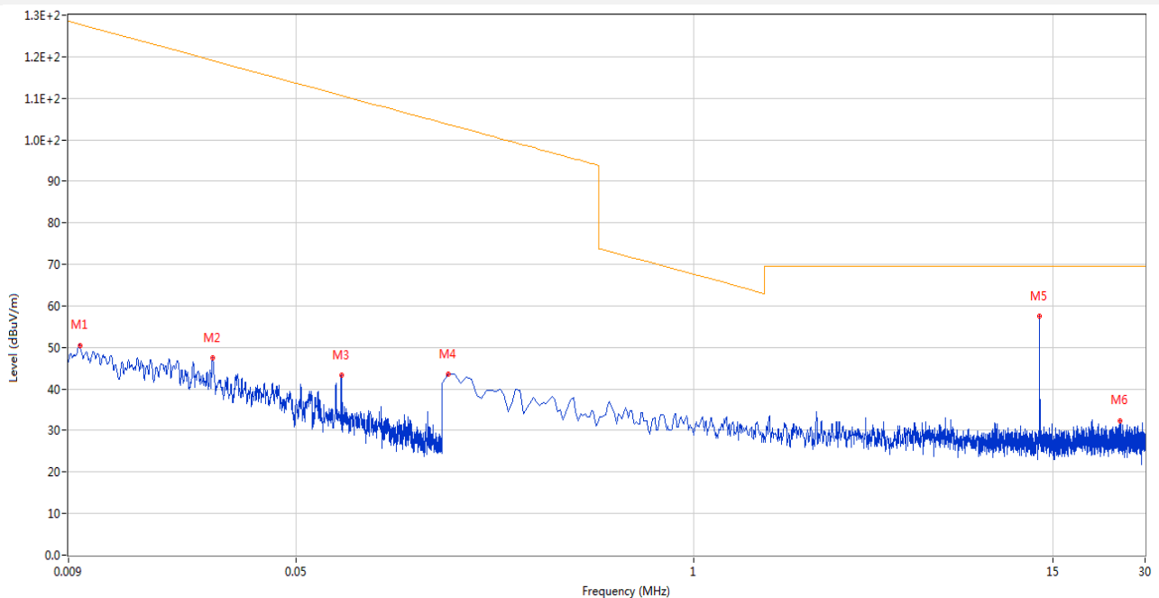
Below 30 MHz, Test Antenna LOOP, EUT Horizontal
