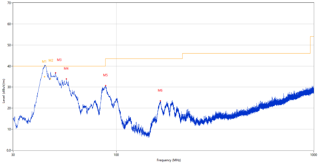
30 MHz to 1 GHz, Test Antenna Vertical
