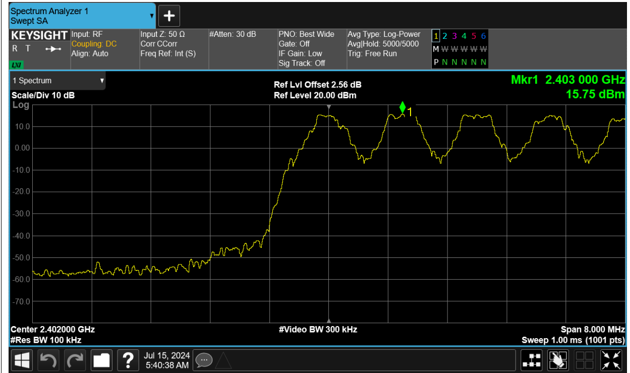
Band Edge(Hopping) NVNT 1-DH1 2402MHz ANT14 Hopping Emission
