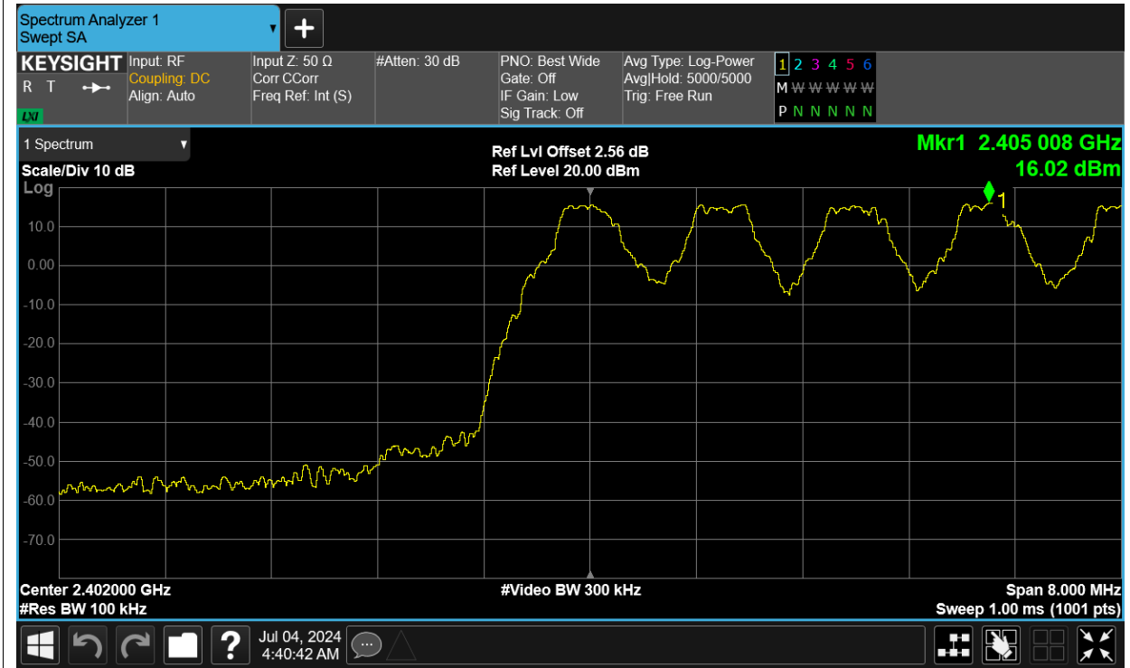
Band Edge(Hopping) NVNT 1-DH1 2402MHz ANT13 Hopping Emission
