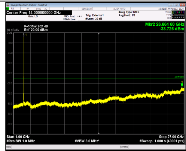
41-41-20MHz-5MHz-16QAM-16QAM-40715-40832-1RB# 0-0RB#0-1000~27000MHz-PASS
