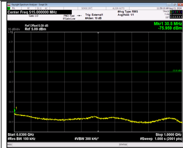
41-41-20MHz-20MHz-QPSK-QPSK-40340-40538-100R B#0-100RB#0-30~1000MHz-PASS
