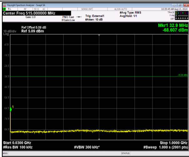
41-41-20MHz-5MHz-16QAM-16QAM-40715-40832-1RB #0-1RB#24-30~1000MHz-PASS
