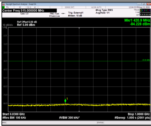
41-41-20MHz-20MHz-QPSK-QPSK-40641-40839-1RB# 0-1RB#99-30~1000MHz-PASS
