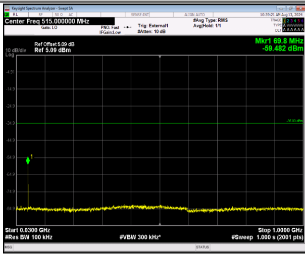
41-41-20MHz-5MHz-16QAM-16QAM-41090-41207-1RB #0-0RB#0-30~1000MHz-PASS
