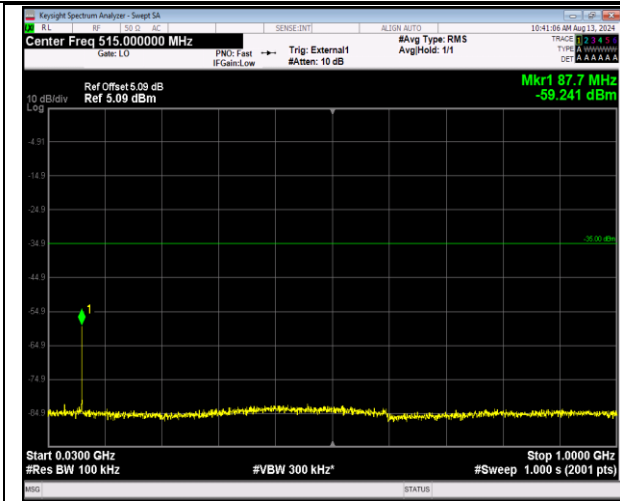
41-41-20MHz-5MHz-16QAM-16QAM-41090-41207-1RB #99-ORB#0-30~1000MHz-PASS
