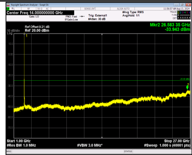
41-41-20MHz-20MHz-16QAM-16QAM-40340-40538-1RB #99-ORB#0-1000~27000MHz-PASS
