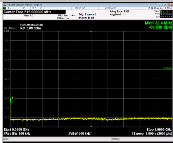
41-41-20MHz-5MHz-QPSK-QPSK-40715-40832-1RB#0-1RB#24-30~1000MHz-PASS
