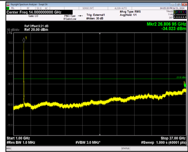
41-41-20MHz-5MHz-64QAM-64QAM-40340-40457-100R B#0-25RB#0-1000~27000MHz-PASS
