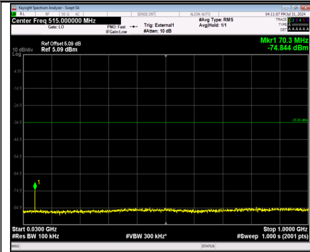
41-41-20MHz-5MHz-64QAM-64QAM-41090-41207-1RB #0-1RB#24-30~1000MHz-PASS
