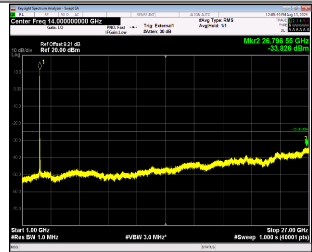
41-41-20MHz-20MHz-16QAM-16QAM-40641-40839-1RB #0-1RB#99-1000~27000MHz-PASS
