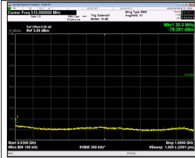
41-41-20MHz-20MHz-64QAM-64QAM-40340-40538-100 RB#0-100RB#0-30~1000MHz-PASS
