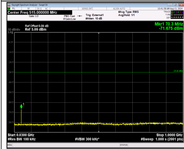
41-41-20MHz-5MHz-QPSK-QPSK-41090-41207-1RB#0-1RB#24-30~1000MHz-PASS
