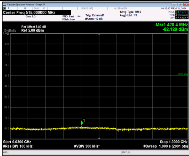
41-41-20MHz-20MHz-64QAM-64QAM-40340-40538-1R B#0-ORB#0-30~1000MHz-PASS
