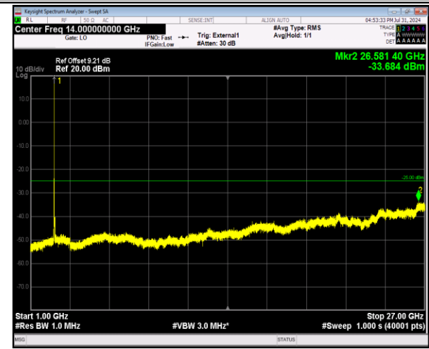
41-41-20MHz-20MHz-64QAM-64QAM-40340-40538-1RB #99-0RB#0-1000~27000MHz-PASS
