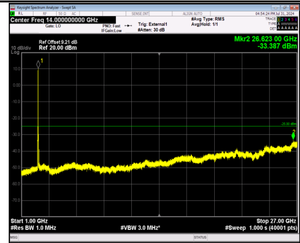
41-41-20MHz-20MHz-64QAM-64QAM-40340-40538-1RB #0-1RB#99-1000~27000MHz-PASS
