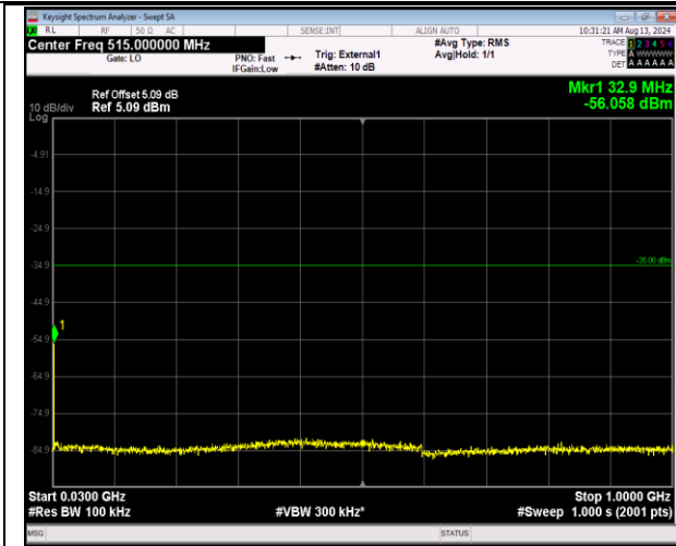
41-41-20MHz-5MHz-QPSK-QPSK-40715-40832-1RB#0-ORB#0-30~1000MHz-PASS
