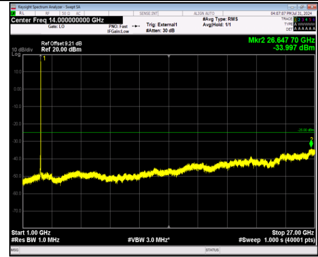
41-41-20MHz-5MHz-64QAM-64QAM-40715-40832-1RB# 99-0RB#0-1000~27000MHz-PASS
