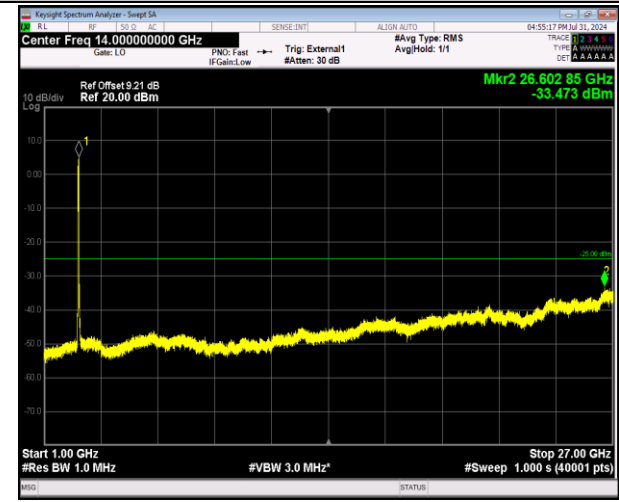
41-41-20MHz-20MHz-64QAM-64QAM-40340-40538-100 RB#0-100RB#0-1000~27000MHz-PASS
