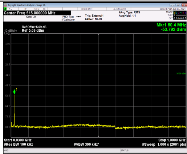
41-41-20MHz-5MHz-QPSK-QPSK-40715-40832-1RB#9-9-ORB#0-30~1000MHz-PASS
