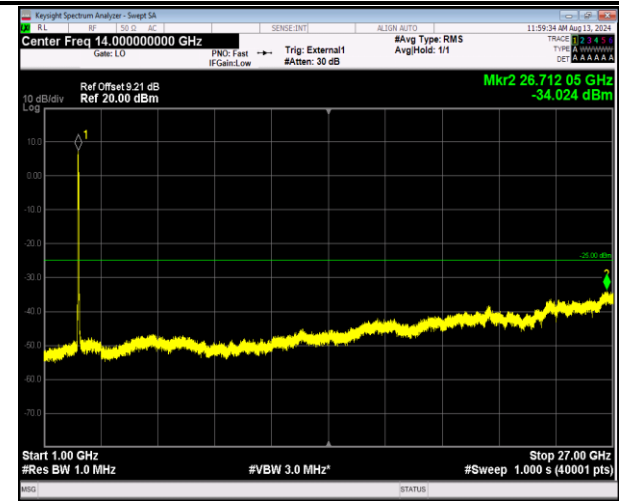
41-41-20MHz-20MHz-QPSK-QPSK-40340-40538-100RB #0-100RB#0-1000~27000MHz-PASS
