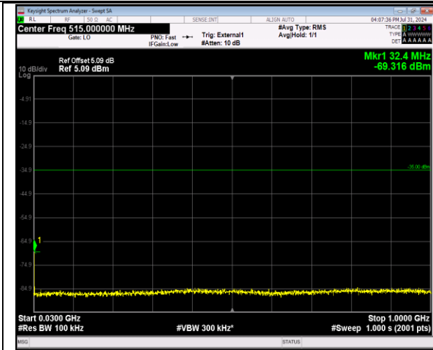
41-41-20MHz-5MHz-64QAM-64QAM-40715-40832-1RB #0-1RB#24-30~1000MHz-PASS
