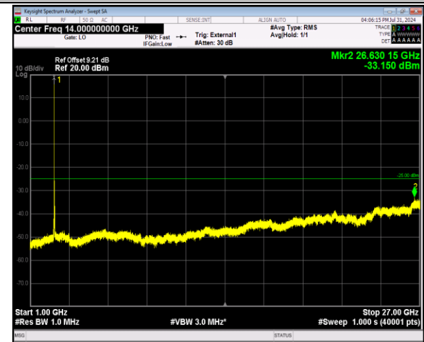
41-41-20MHz-5MHz-64QAM-64QAM-40715-40832-1RB# 0-ORB#0-1000~27000MHz-PASS
