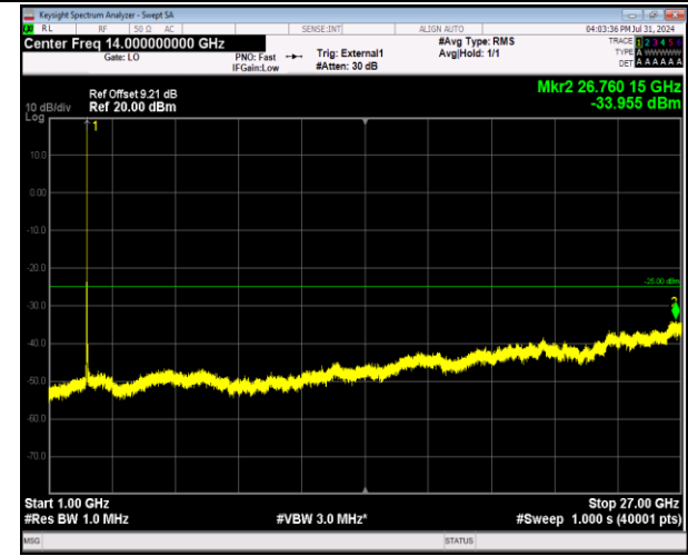
41-41-20MHz-5MHz-64QAM-64QAM-40340-40457-1RB# 99-0RB#0-1000~27000MHz-PASS
