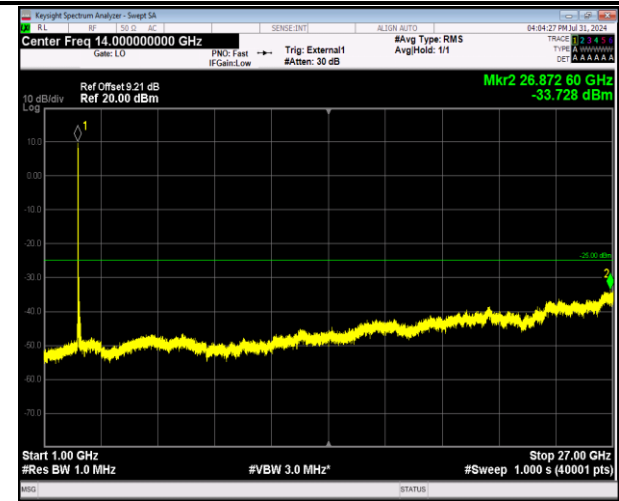
41-41-20MHz-5MHz-64QAM-64QAM-40340-40457-1RB# 0-1RB#24-1000~27000MHz-PASS
