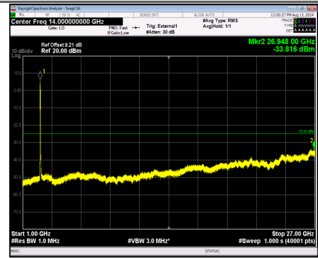
41-41-20MHz-20MHz-16QAM-16QAM-40340-40538-100 RB#0-100RB#0-1000~27000MHz-PASS
