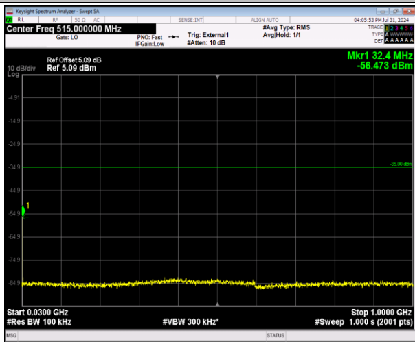
41-41-20MHz-5MHz-64QAM-64QAM-40715-40832-1RB #0-ORB#0-30~1000MHz-PASS
