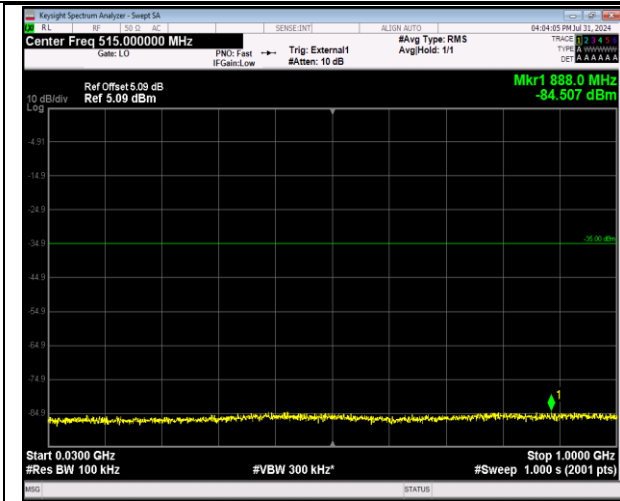
41-41-20MHz-5MHz-64QAM-64QAM-40340-40457-1RB #0-1RB#24-30~1000MHz-PASS
