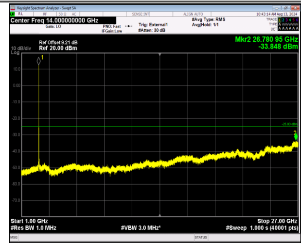
41-41-20MHz-5MHz-16QAM-16QAM-41090-41207-1RB# 0-1RB#24-1000~27000MHz-PASS
