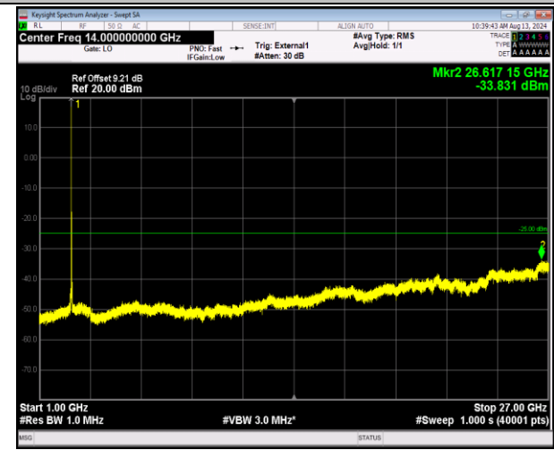
41-41-20MHz-5MHz-16QAM-16QAM-41090-41207-1RB# 0-0RB#0-1000~27000MHz-PASS
