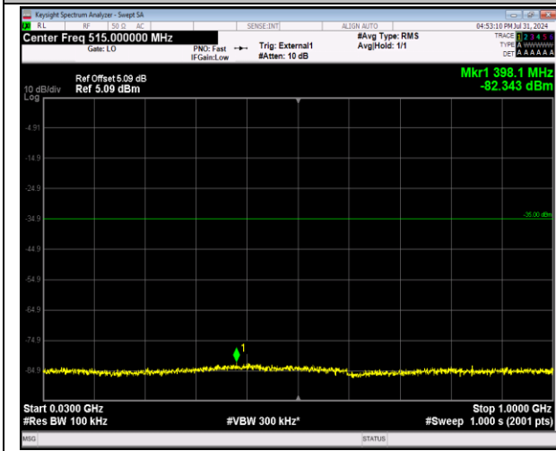
41-41-20MHz-20MHz-64QAM-64QAM-40340-40538-1R B#99-0RB#0-30~1000MHz-PASS
