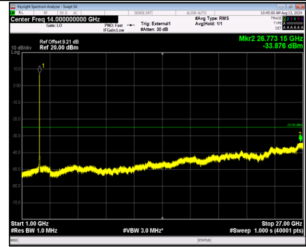
41-41-20MHz-5MHz-16QAM-16QAM-41090-41207-100R B#0-25RB#0-1000~27000MHz-PASS
