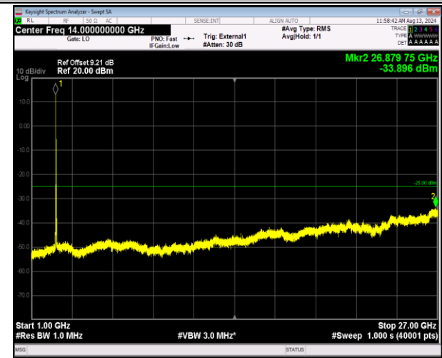
41-41-20MHz-20MHz-16QAM-16QAM-40340-40538-1RB #0-1RB#99-1000~27000MHz-PASS
