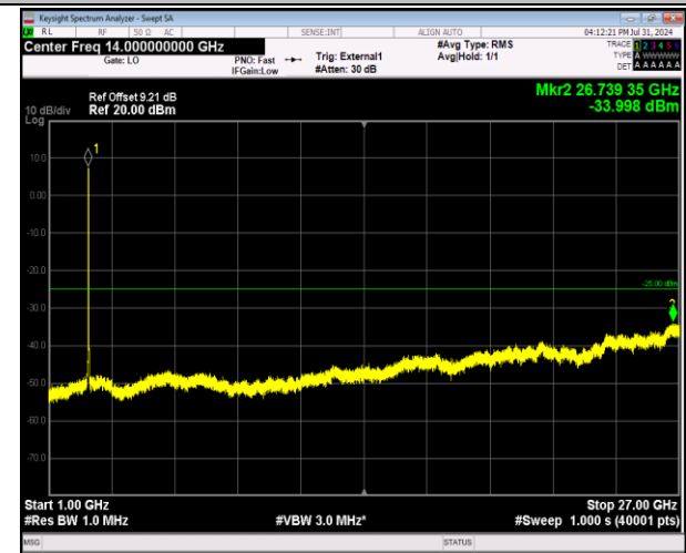
41-41-20MHz-5MHz-64QAM-64QAM-41090-41207-100R B#0-25RB#0-1000~27000MHz-PASS
