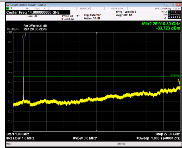
41-41-20MHz-5MHz-QPSK-QPSK-41090-41207-1RB#0-1RB#24-1000~27000MHz-PASS
