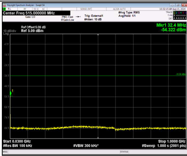
41-41-20MHz-5MHz-16QAM-16QAM-40715-40832-1RB #0-0RB#0-30~1000MHz-PASS
