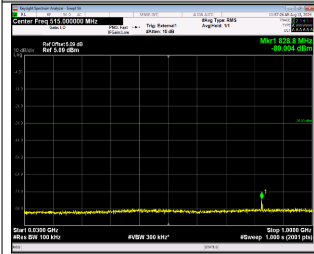
41-41-20MHz-20MHz-QPSK-QPSK-40340-40538-1RB# 0-1RB#99-30~1000MHz-PASS
