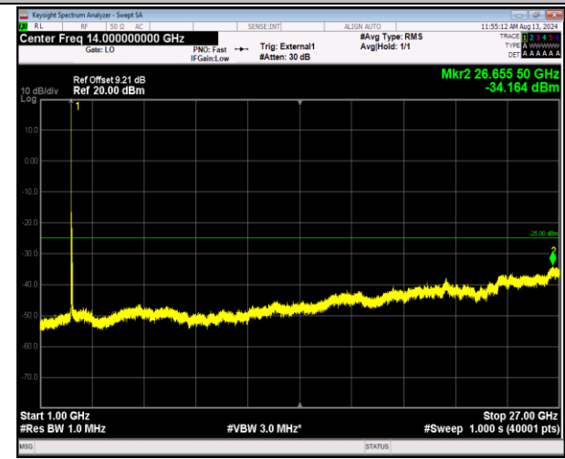
41-41-20MHz-20MHz-16QAM-16QAM-40340-40538-1RB #0-0RB#0-1000~27000MHz-PASS
