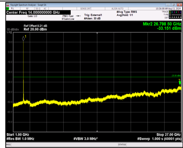
41-41-20MHz-5MHz-16QAM-16QAM-40715-40832-1RB# 0-1RB#24-1000~27000MHz-PASS
