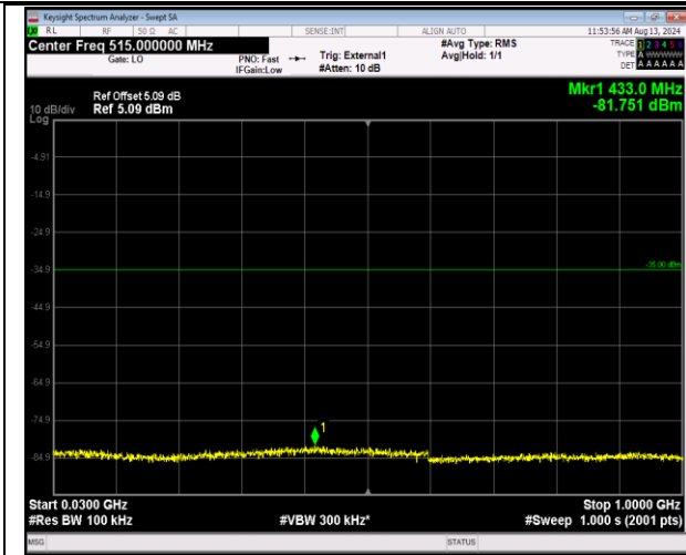
41-41-20MHz-20MHz-QPSK-QPSK-40340-40538-1RB# 0-ORB#0-30~1000MHz-PASS
