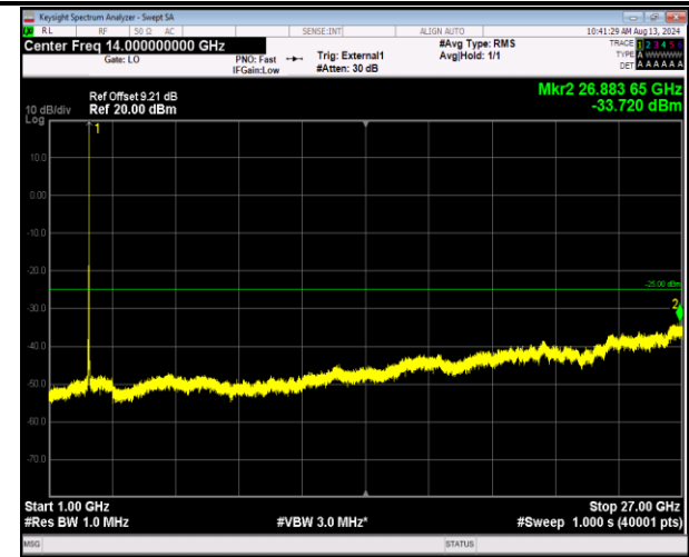
41-41-20MHz-5MHz-16QAM-16QAM-41090-41207-1RB# 99-ORB#0-1000~27000MHz-PASS
