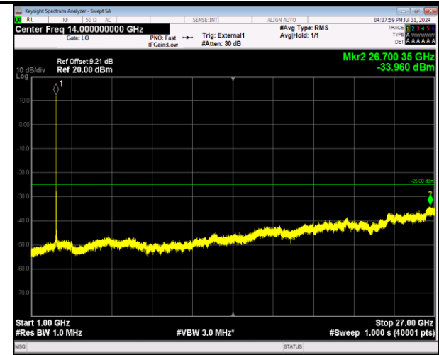
41-41-20MHz-5MHz-64QAM-64QAM-40715-40832-1RB# 0-1RB#24-1000~27000MHz-PASS
