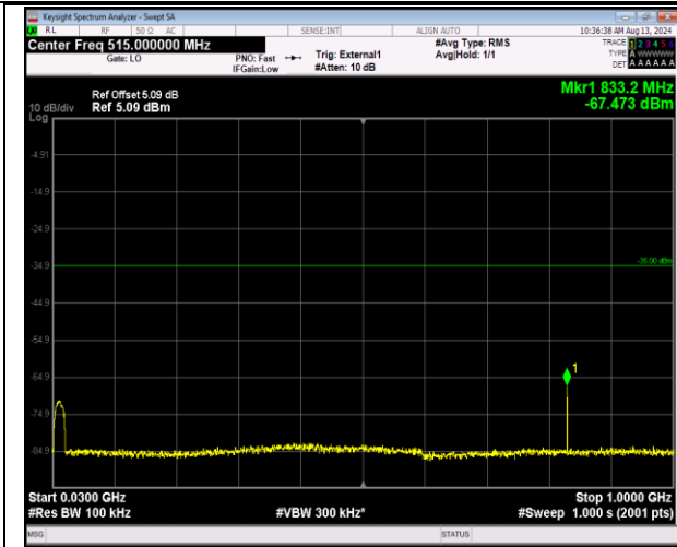
41-41-20MHz-5MHz-QPSK-QPSK-40715-40832-100RB #0-25RB#0-30~1000MHz-PASS
