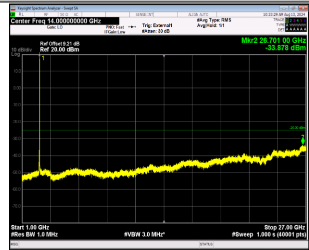
41-41-20MHz-5MHz-QPSK-QPSK-40715-40832-1RB#99-ORB#0-1000~27000MHz-PASS
