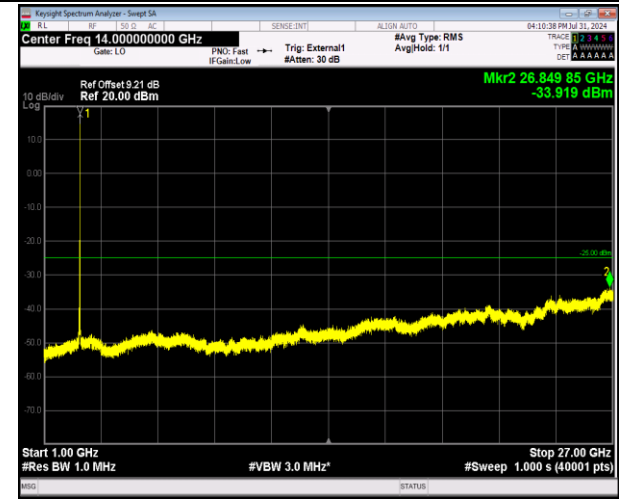
41-41-20MHz-5MHz-64QAM-64QAM-41090-41207-1RB# 99-0RB#0-1000~27000MHz-PASS
