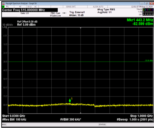
41-41-20MHz-20MHz-16QAM-16QAM-40641-40839-1R B#0-0RB#0-30~1000MHz-PASS
