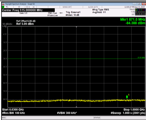
41-41-20MHz-20MHz-16QAM-16QAM-40641-40839-1R B#0-1RB#99-30~1000MHz-PASS
