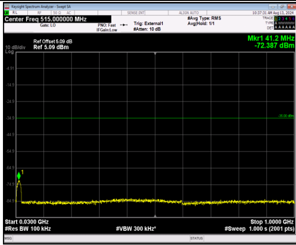
41-41-20MHz-5MHz-16QAM-16QAM-40715-40832-100 RB#0-25RB#0-30~1000MHz-PASS
