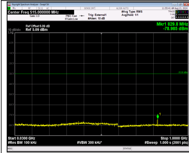
41-41-20MHz-20MHz-QPSK-QPSK-40340-40538-1RB# 99-ORB#0-30~1000MHz-PASS
