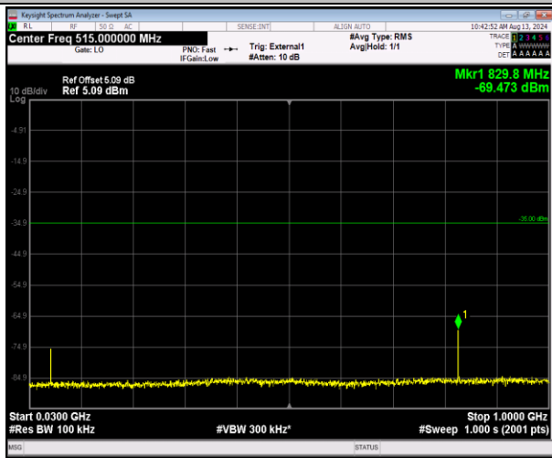
41-41-20MHz-5MHz-16QAM-16QAM-41090-41207-1RB #0-1RB#24-30~1000MHz-PASS
