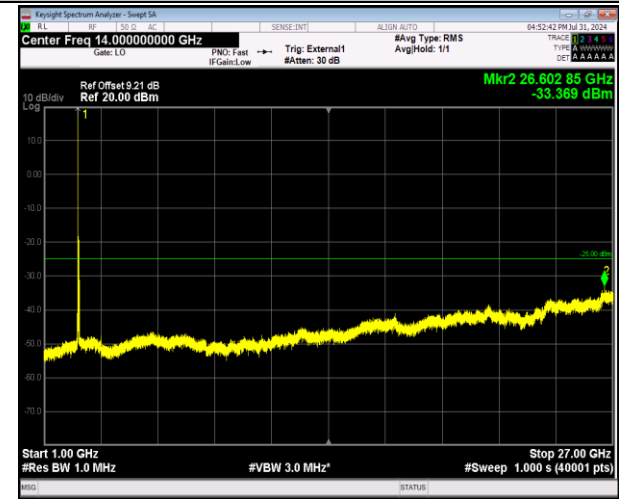
41-41-20MHz-20MHz-64QAM-64QAM-40340-40538-1RB #0-ORB#0-1000~27000MHz-PASS
