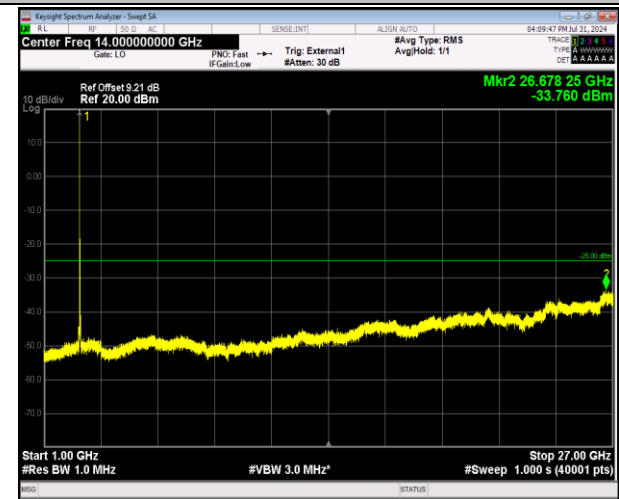
41-41-20MHz-5MHz-64QAM-64QAM-41090-41207-1RB# 0-ORB#0-1000~27000MHz-PASS
