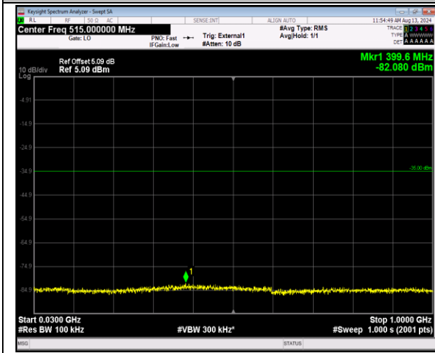
41-41-20MHz-20MHz-16QAM-16QAM-40340-40538-1R B#0-0RB#0-30~1000MHz-PASS
