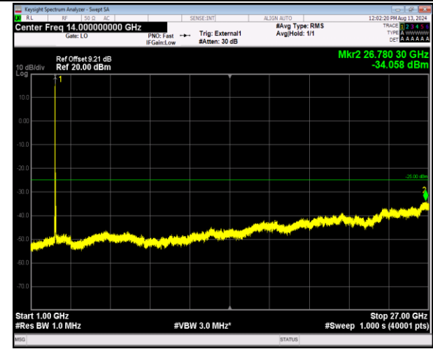
41-41-20MHz-20MHz-16QAM-16QAM-40641-40839-1RB #0-0RB#0-1000~27000MHz-PASS
