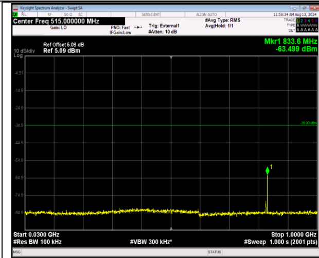
41-41-20MHz-20MHz-16QAM-16QAM-40340-40538-1R B#99-ORB#0-30~1000MHz-PASS
