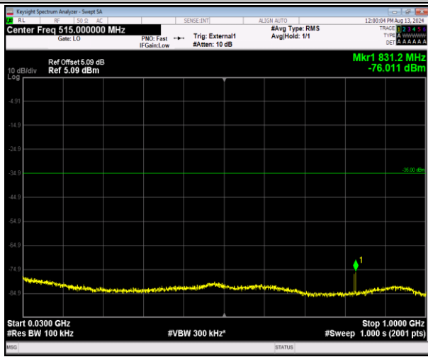
41-41-20MHz-20MHz-16QAM-16QAM-40340-40538-100 RB#0-100RB#0-30~1000MHz-PASS
