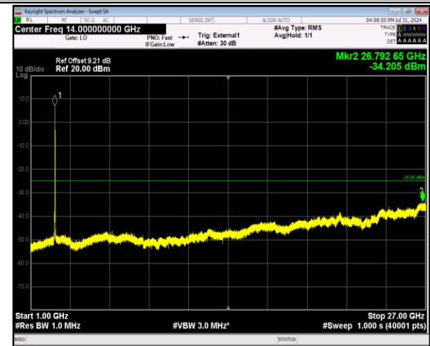
41-41-20MHz-5MHz-64QAM-64QAM-40715-40832-100R B#0-25RB#0-1000~27000MHz-PASS
