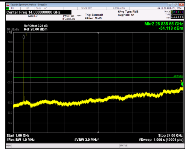
41-41-20MHz-5MHz-64QAM-64QAM-41090-41207-1RB# 0-1RB#24-1000~27000MHz-PASS
