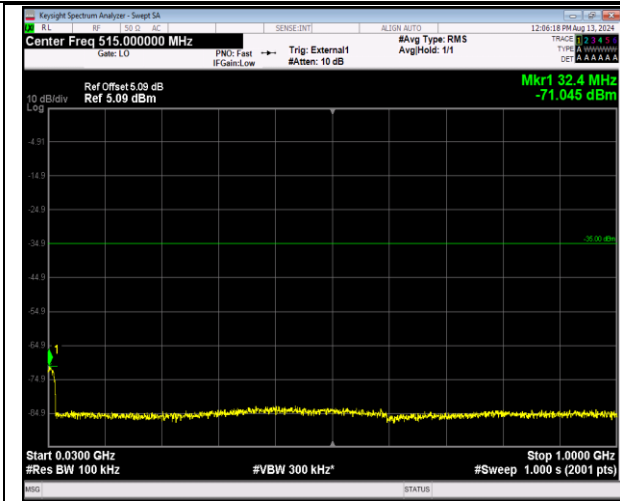
41-41-20MHz-20MHz-QPSK-QPSK-40641-40839-100R B#0-100RB#0-30~1000MHz-PASS
