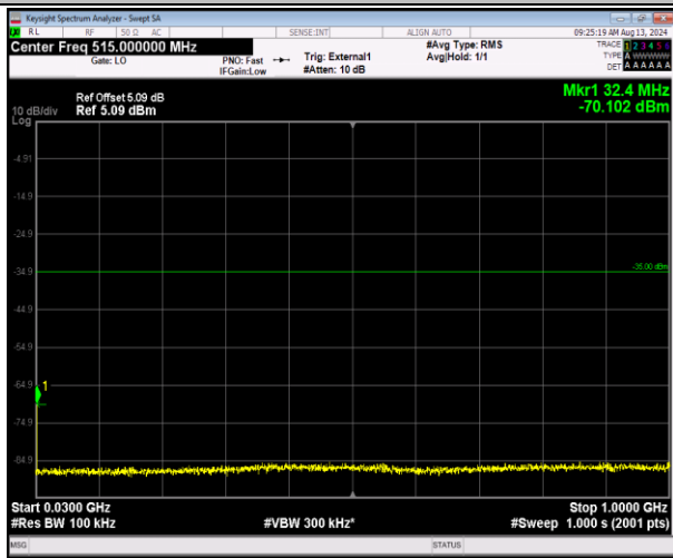
41-41-5MHz-20MHz-16QAM-16QAM-40648-40765-1RB #0-1RB#99-30~1000MHz-PASS
