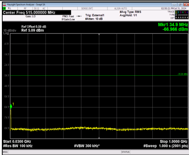
41-41-5MHz-20MHz-64QAM-64QAM-40648-40765-25R B#0-100RB#0-30~1000MHz-PASS
