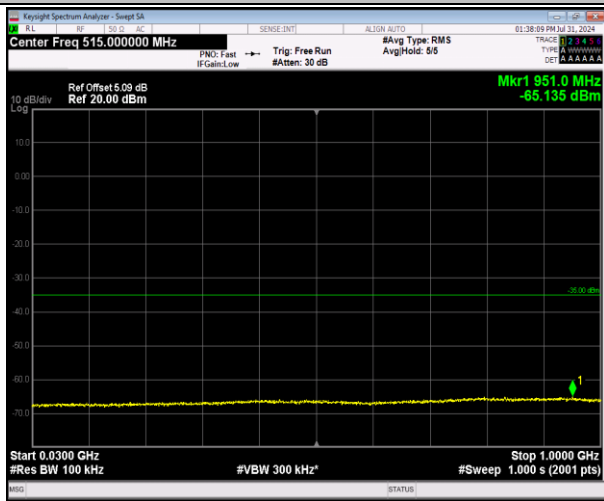
7-7-20MHz-20MHz-64QAM-64QAM-21152-21350-100R B#0-100RB#0-30~1000MHz-PASS
