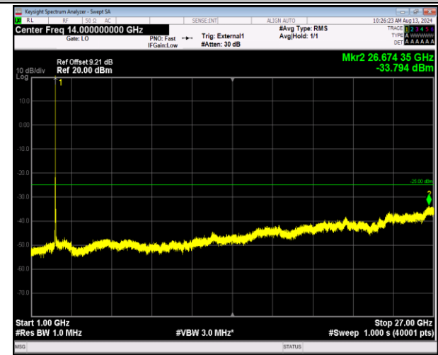
41-41-20MHz-5MHz-QPSK-QPSK-40340-40457-1RB#99-0RB#0-1000~27000MHz-PASS
