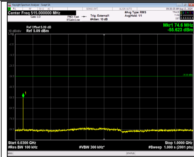
41-41-5MHz-20MHz-16QAM-16QAM-41023-41140-1RB #24-ORB#0-30~1000MHz-PASS
