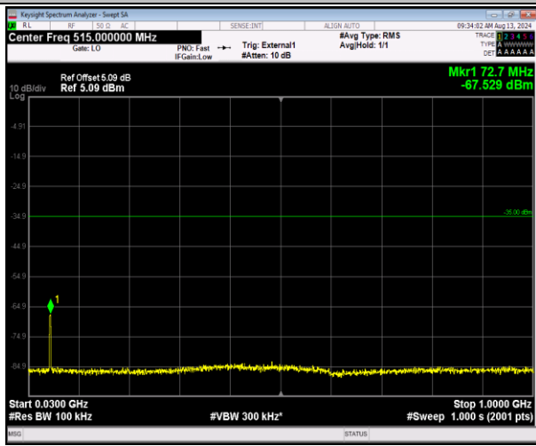
41-41-5MHz-20MHz-16QAM-16QAM-41023-41140-25R B#0-100RB#0-30~1000MHz-PASS
