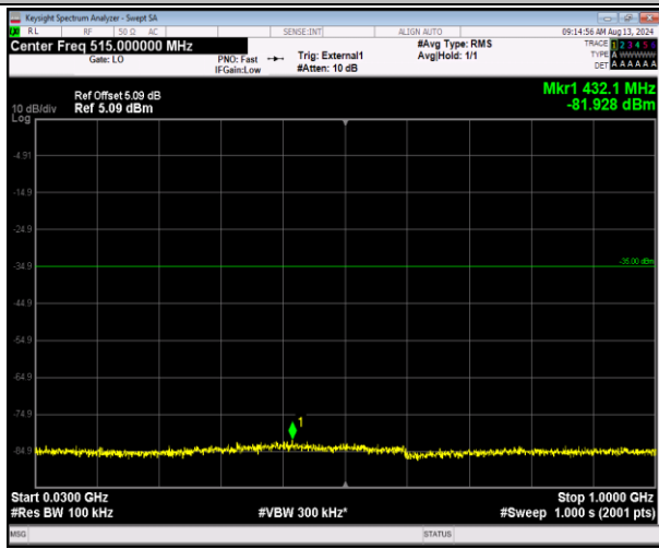
41-41-5MHz-20MHz-16QAM-16QAM-40273-40390-1RB #0-0RB#0-30~1000MHz-PASS
