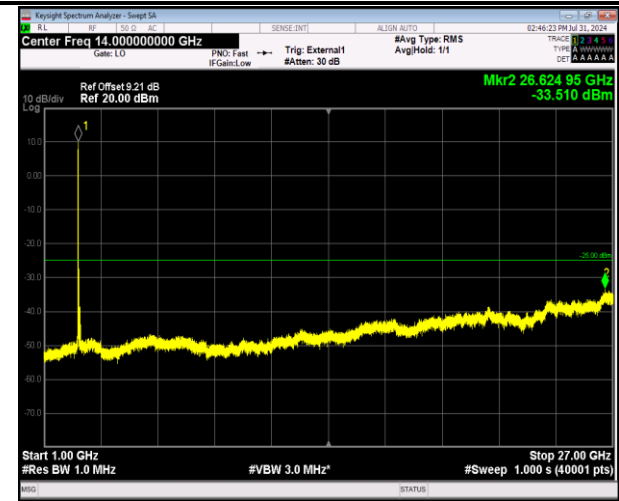
41-41-5MHz-20MHz-64QAM-64QAM-40273-40390-1RB# 0-1RB#99-1000~27000MHz-PASS
