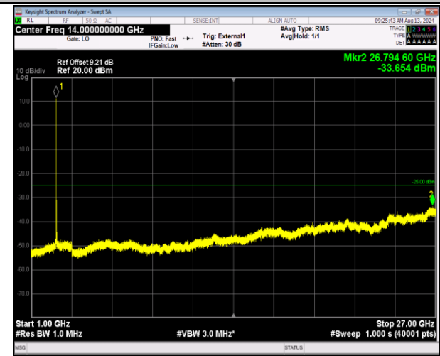
41-41-5MHz-20MHz-16QAM-16QAM-40648-40765-1RB# 0-1RB#99-1000~27000MHz-PASS
