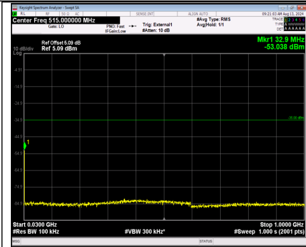
41-41-5MHz-20MHz-QPSK-QPSK-40648-40765-1RB#0-ORB#0-30~1000MHz-PASS
