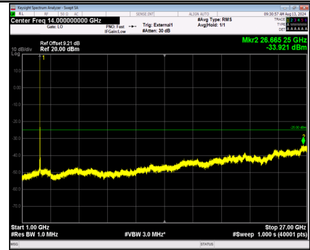
41-41-5MHz-20MHz-16QAM-16QAM-41023-41140-1RB# 24-ORB#0-1000~27000MHz-PASS
