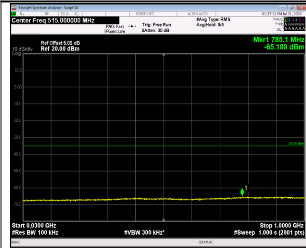
7-7-20MHz-20MHz-64QAM-64QAM-21152-21350-1RB# 0-1RB#99-30~1000MHz-PASS
