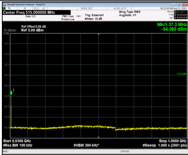
41-41-5MHz-20MHz-QPSK-QPSK-40648-40765-1RB#24-ORB#0-30~1000MHz-PASS
