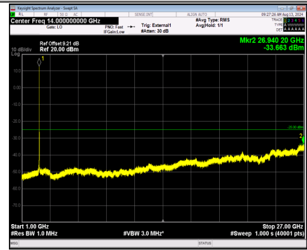
41-41-5MHz-20MHz-16QAM-16QAM-40648-40765-25RB #0-100RB#0-1000~27000MHz-PASS
