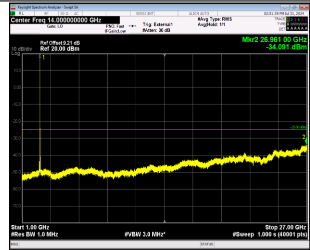
41-41-5MHz-20MHz-64QAM-64QAM-41023-41140-1RB# 0-ORB#0-1000~27000MHz-PASS
