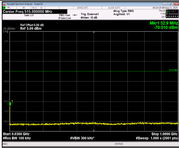
41-41-5MHz-20MHz-QPSK-QPSK-40648-40765-1RB#0-1RB#99-30~1000MHz-PASS
