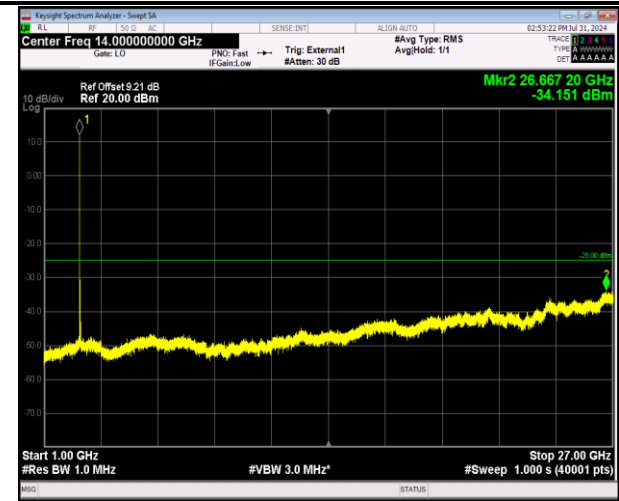
41-41-5MHz-20MHz-64QAM-64QAM-41023-41140-1RB# 0-1RB#99-1000~27000MHz-PASS
