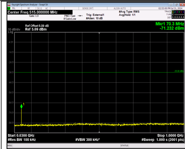
41-41-5MHz-20MHz-64QAM-64QAM-41023-41140-1RB #0-1RB#99-30~1000MHz-PASS
