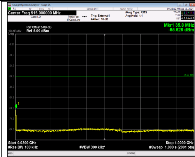
41-41-5MHz-20MHz-QPSK-QPSK-40648-40765-25RB# 0-100RB#0-30~1000MHz-PASS
