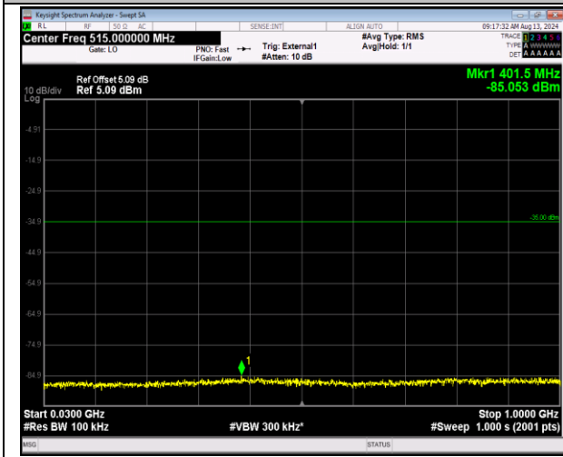
41-41-5MHz-20MHz-QPSK-QPSK-40273-40390-1RB#0-1RB#99-30~1000MHz-PASS
