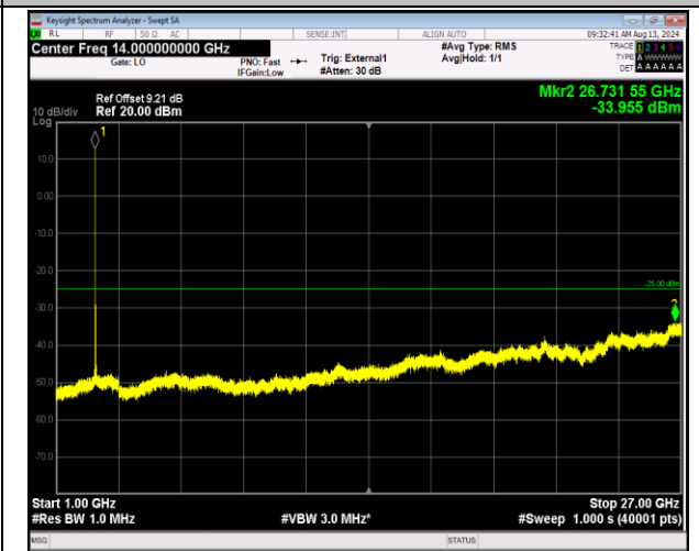
41-41-5MHz-20MHz-16QAM-16QAM-41023-41140-1RB#0-1RB#99-1000~27000MHz-PASS
