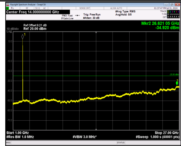
7-7-20MHz-20MHz-64QAM-64QAM-21152-21350-1RB#0- 1RB#99-1000~27000MHz-PASS
