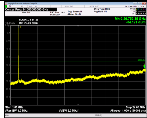
41-41-20MHz-5MHz-64QAM-64QAM-40340-40457-1RB# 0-ORB#0-1000~27000MHz-PASS
