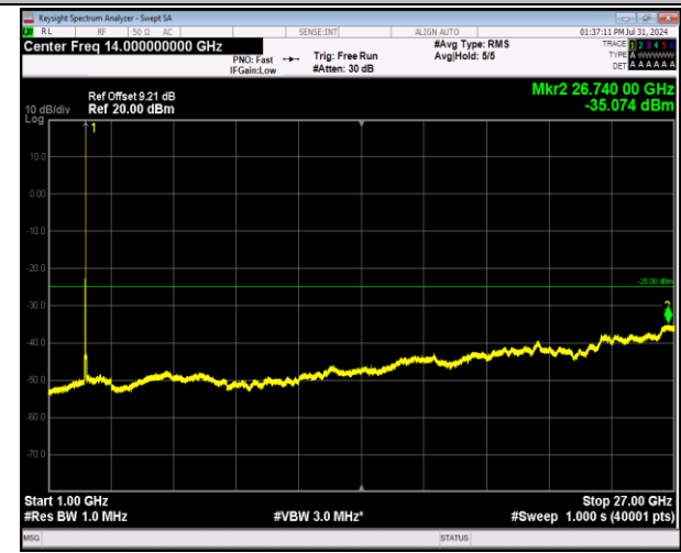
7-7-20MHz-20MHz-64QAM-64QAM-21152-21350-1RB#9 9-0RB#0-1000~27000MHz-PASS
