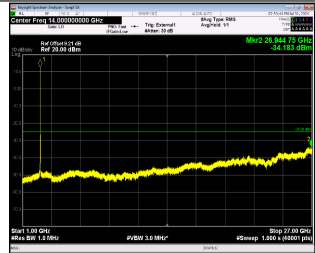
41-41-5MHz-20MHz-64QAM-64QAM-40648-40765-25RB #0-100RB#0-1000~27000MHz-PASS
