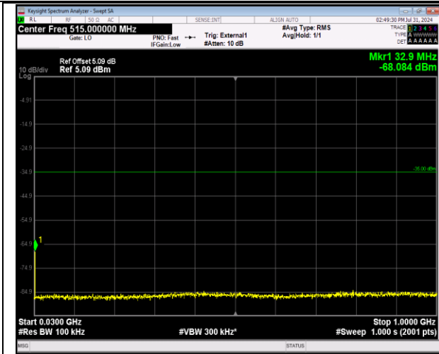
41-41-5MHz-20MHz-64QAM-64QAM-40648-40765-1RB #0-1RB#99-30~1000MHz-PASS
