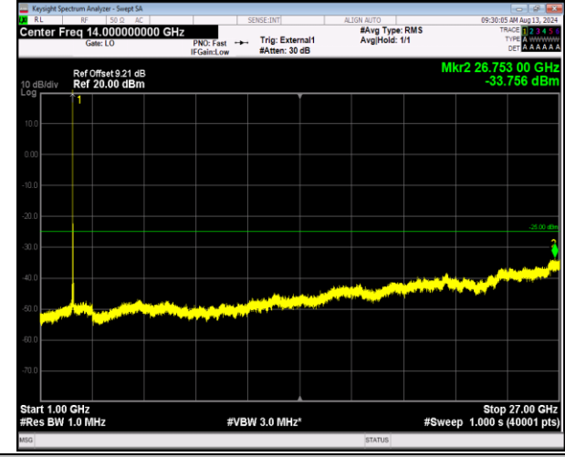
41-41-5MHz-20MHz-QPSK-QPSK-41023-41140-1RB#24-ORB#0-1000~27000MHz-PASS
