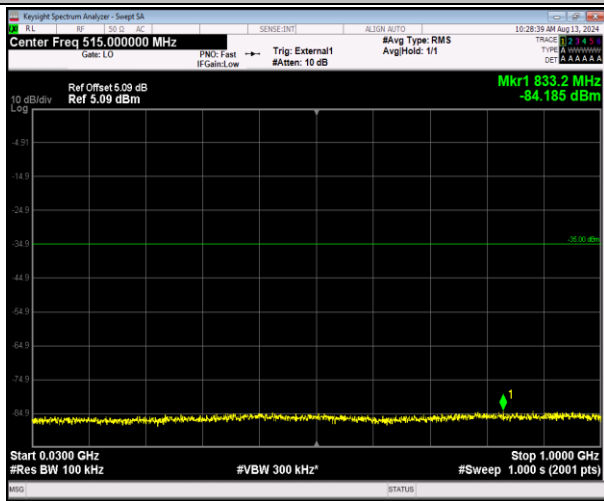
41-41-20MHz-5MHz-16QAM-16QAM-40340-40457-1RB #0-1RB#24-30~1000MHz-PASS
