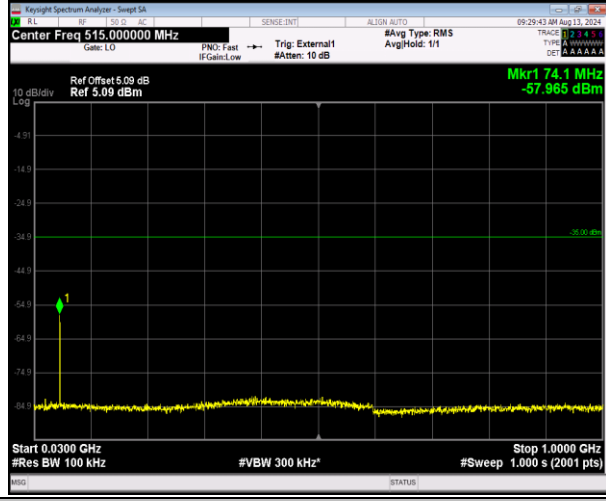
41-41-5MHz-20MHz-QPSK-QPSK-41023-41140-1RB#24-ORB#0-30~1000MHz-PASS
