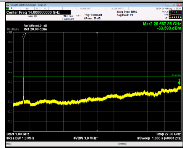
41-41-5MHz-20MHz-16QAM-16QAM-41023-41140-25RB #0-100RB#0-1000~27000MHz-PASS
