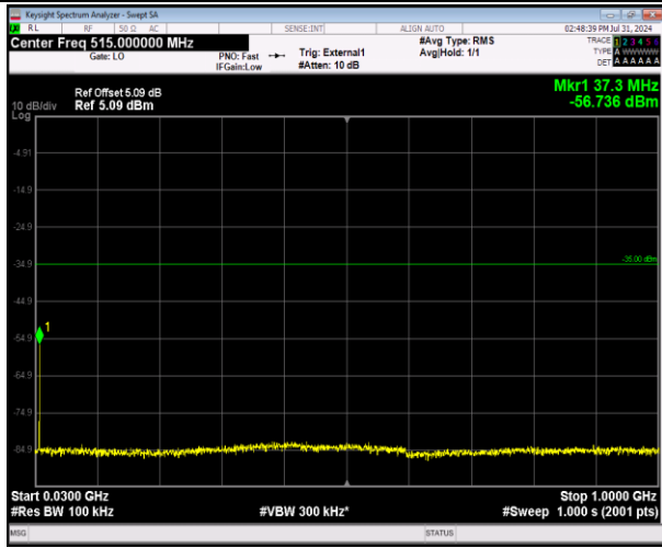
41-41-5MHz-20MHz-64QAM-64QAM-40648-40765-1RB #24-0RB#0-30~1000MHz-PASS
