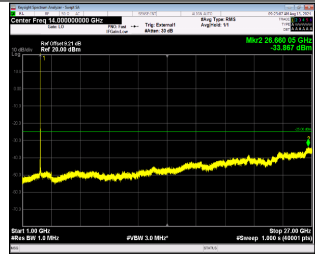
41-41-5MHz-20MHz-QPSK-QPSK-40648-40765-1RB#24-ORB#0-1000~27000MHz-PASS
