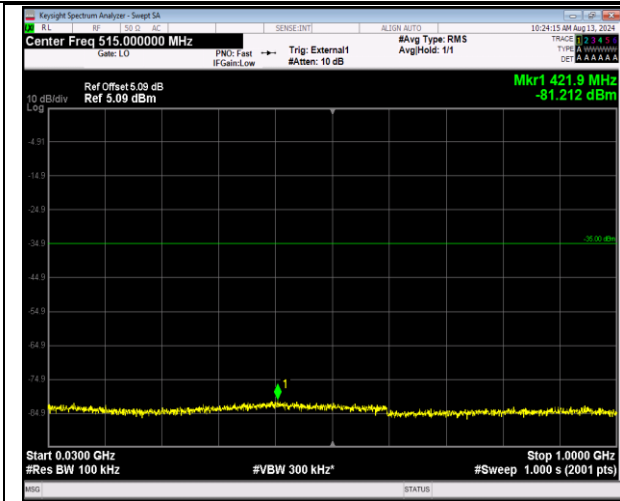
41-41-20MHz-5MHz-QPSK-QPSK-40340-40457-1RB#0-ORB#0-30~1000MHz-PASS
