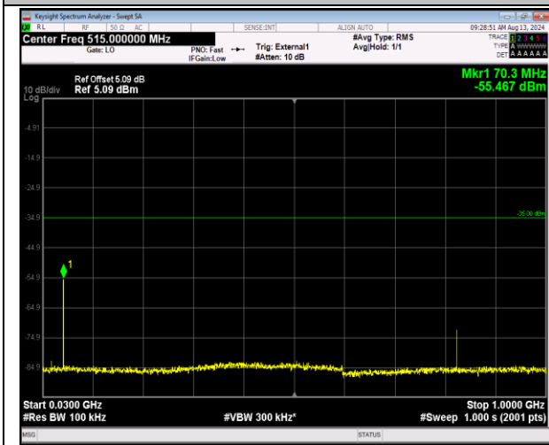
41-41-5MHz-20MHz-16QAM-16QAM-41023-41140-1RB#0-0RB#0-30~1000MHz-PASS
