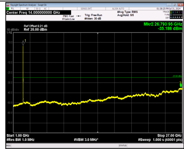
7-7-20MHz-20MHz-64QAM-64QAM-21152-21350-100RB #0-100RB#0-1000~27000MHz-PASS
