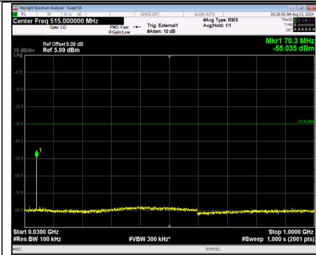
41-41-5MHz-20MHz-QPSK-QPSK-41023-41140-1RB#0-ORB#0-30~1000MHz-PASS
