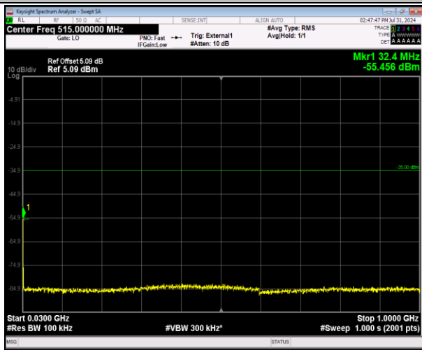
41-41-5MHz-20MHz-64QAM-64QAM-40648-40765-1RB #0-ORB#0-30~1000MHz-PASS
