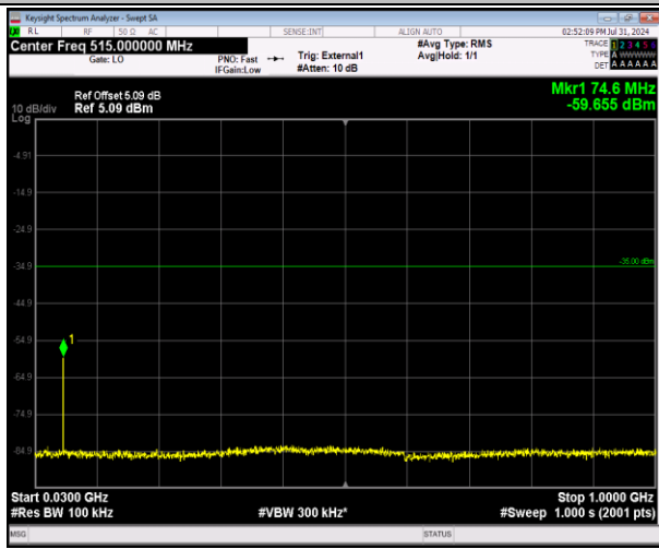
41-41-5MHz-20MHz-64QAM-64QAM-41023-41140-1RB #24-0RB#0-30~1000MHz-PASS
