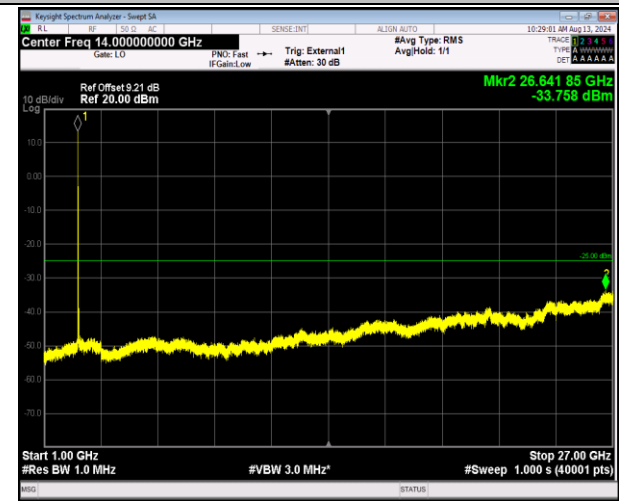
41-41-20MHz-5MHz-16QAM-16QAM-40340-40457-1RB# 0-1RB#24-1000~27000MHz-PASS
