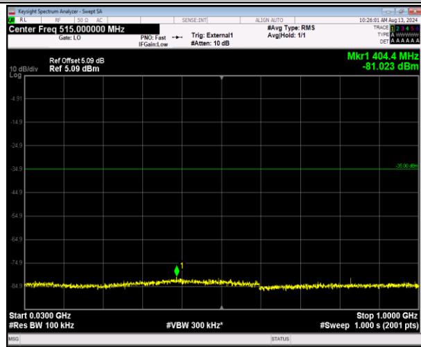
41-41-20MHz-5MHz-QPSK-QPSK-40340-40457-1RB#9-0RB#0-30~1000MHz-PASS
