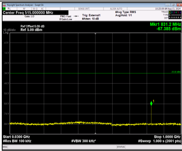
41-41-20MHz-5MHz-16QAM-16QAM-40340-40457-1RB #0-0RB#0-30~1000MHz-PASS
