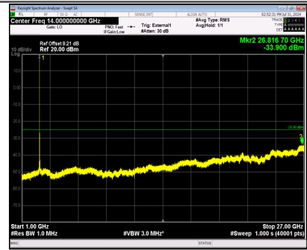
41-41-5MHz-20MHz-64QAM-64QAM-41023-41140-1RB# 24-0RB#0-1000~27000MHz-PASS
