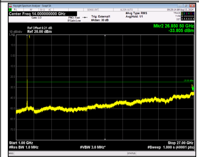
41-41-5MHz-20MHz-16QAM-16QAM-41023-41140-1RB#0-0RB#0-1000~27000MHz-PASS
