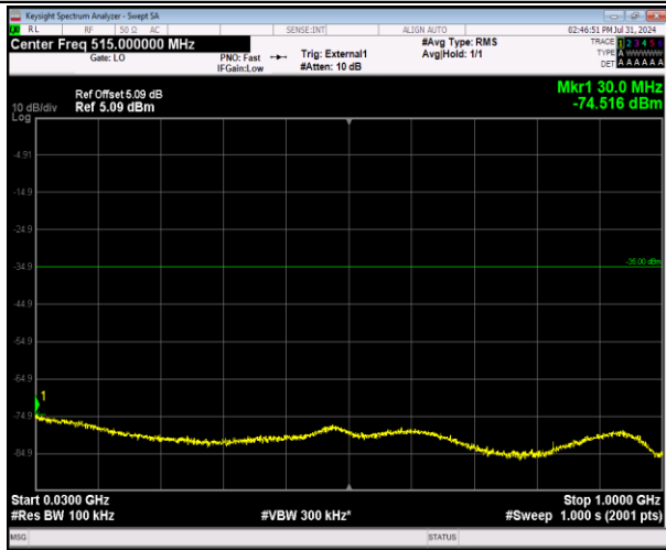
41-41-5MHz-20MHz-64QAM-64QAM-40273-40390-25R B#0-100RB#0-30~1000MHz-PASS
