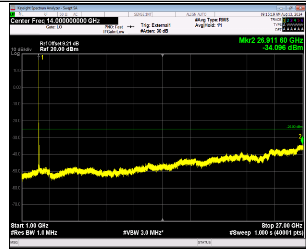
41-41-5MHz-20MHz-16QAM-16QAM-40273-40390-1RB# 0-0RB#0-1000~27000MHz-PASS
