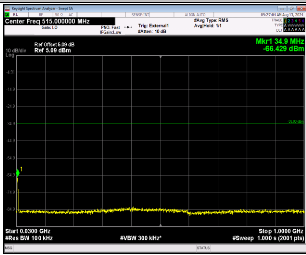
41-41-5MHz-20MHz-16QAM-16QAM-40648-40765-25R B#0-100RB#0-30~1000MHz-PASS
