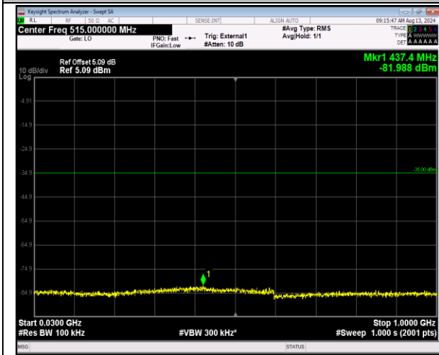
41-41-5MHz-20MHz-QPSK-QPSK-40273-40390-1RB#24-0RB#0-30~1000MHz-PASS
