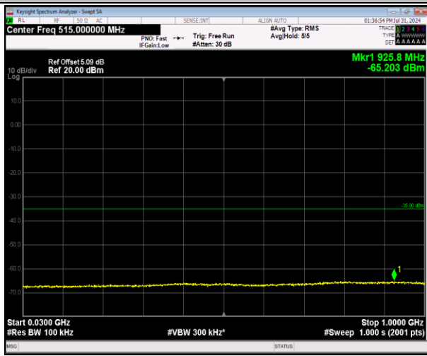
7-7-20MHz-20MHz-64QAM-64QAM-21152-21350-1RB# 99-0RB#0-30~1000MHz-PASS
