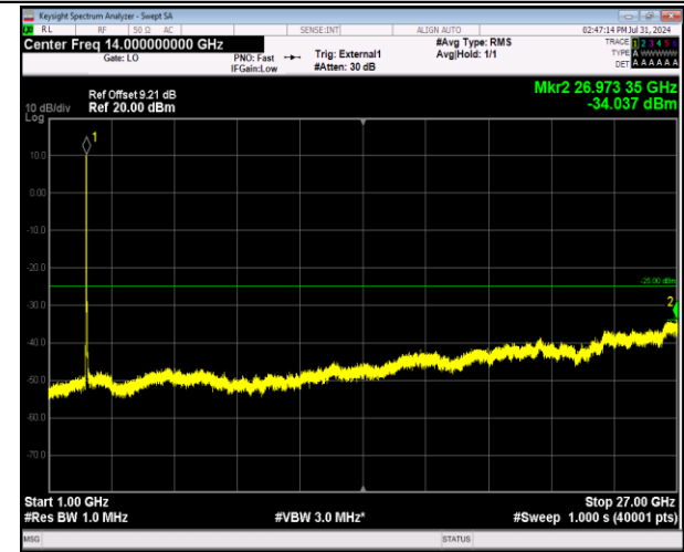
41-41-5MHz-20MHz-64QAM-64QAM-40273-40390-25RB #0-100RB#0-1000~27000MHz-PASS
