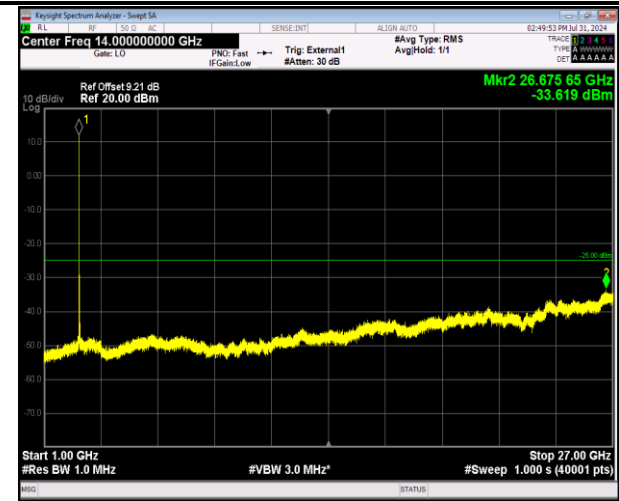
41-41-5MHz-20MHz-64QAM-64QAM-40648-40765-1RB# 0-1RB#99-1000~27000MHz-PASS
