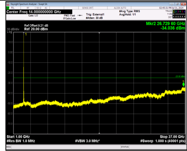
41-41-5MHz-20MHz-64QAM-64QAM-40273-40390-1RB# 24-0RB#0-1000~27000MHz-PASS
