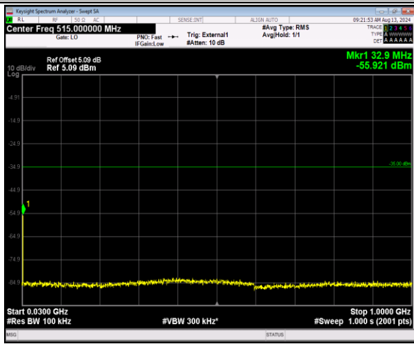
41-41-5MHz-20MHz-16QAM-16QAM-40648-40765-1RB #0-0RB#0-30~1000MHz-PASS
