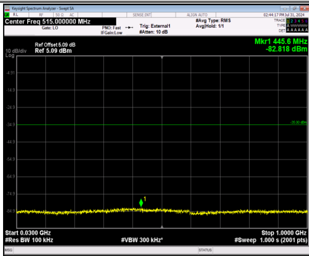
41-41-5MHz-20MHz-64QAM-64QAM-40273-40390-1RB #0-ORB#0-30~1000MHz-PASS
