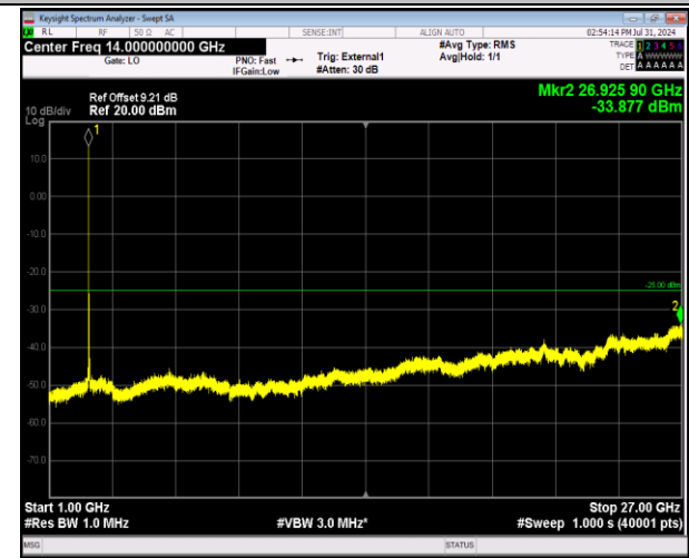
41-41-5MHz-20MHz-64QAM-64QAM-41023-41140-25RB #0-100RB#0-1000~27000MHz-PASS
