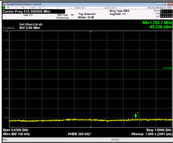
41-41-5MHz-20MHz-16QAM-16QAM-40273-40390-1RB #0-1RB#99-30~1000MHz-PASS
