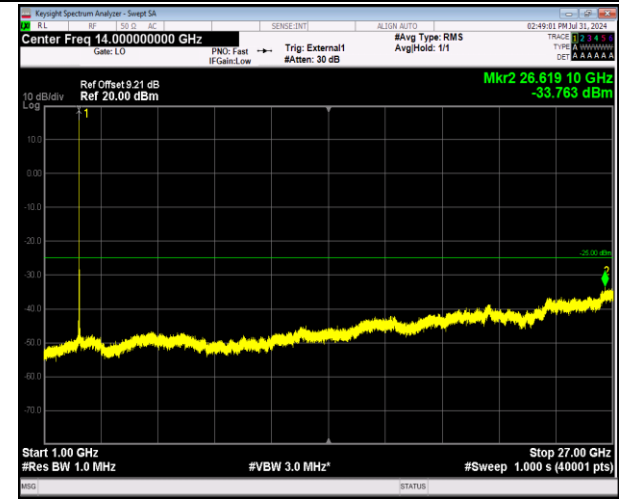
41-41-5MHz-20MHz-64QAM-64QAM-40648-40765-1RB# 24-0RB#0-1000~27000MHz-PASS
