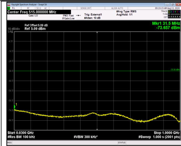
41-41-5MHz-20MHz-QPSK-QPSK-40273-40390-25RB# 0-100RB#0-30~1000MHz-PASS
