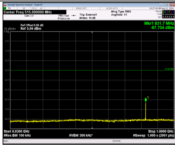
41-41-20MHz-5MHz-QPSK-QPSK-40340-40457-1RB#0-1RB#24-30~1000MHz-PASS
