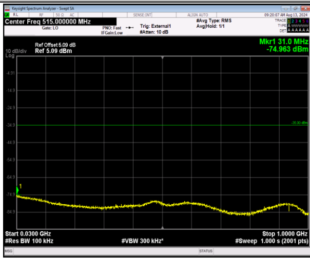
41-41-5MHz-20MHz-16QAM-16QAM-40273-40390-25R B#0-100RB#0-30~1000MHz-PASS
