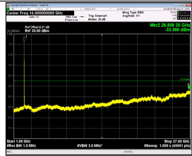
41-41-20MHz-5MHz-QPSK-QPSK-40340-40457-1RB#0-1RB#24-1000~27000MHz-PASS
