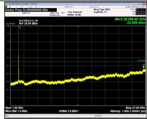
41-41-20MHz-5MHz-16QAM-16QAM-40340-40457-1RB# 0-0RB#0-1000~27000MHz-PASS
