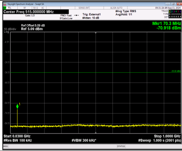
41-41-5MHz-20MHz-QPSK-QPSK-41023-41140-1RB#0-1RB#99-30~1000MHz-PASS
