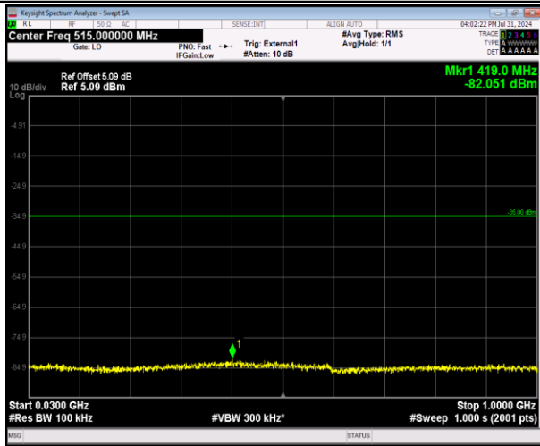
41-41-20MHz-5MHz-64QAM-64QAM-40340-40457-1RB #0-ORB#0-30~1000MHz-PASS
