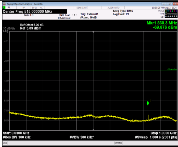
41-41-20MHz-5MHz-16QAM-16QAM-40340-40457-100 RB#0-25RB#0-30~1000MHz-PASS
