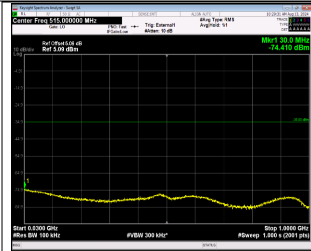
41-41-20MHz-5MHz-QPSK-QPSK-40340-40457-100RB #0-25RB#0-30~1000MHz-PASS
