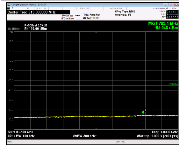
7-7-20MHz-10MHz-64QAM-64QAM-21051-21195-100RB#0-50RB#0-30~1000MHz-PASS
