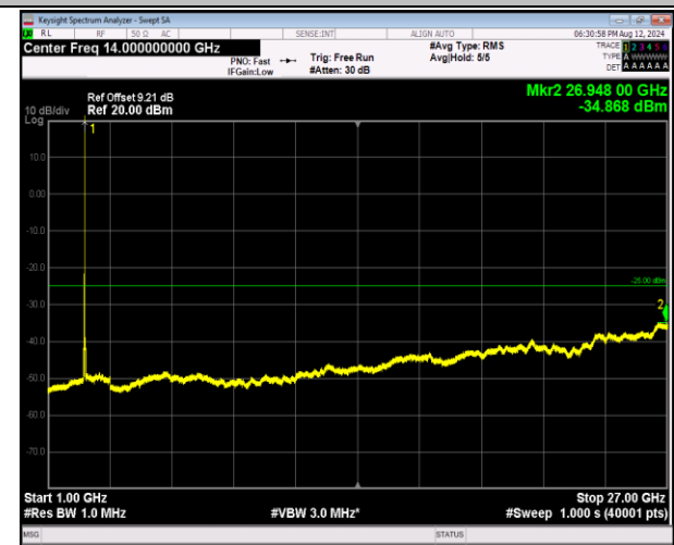
7-7-20MHz-20MHz-QPSK-QPSK-21152-21350-1RB#99-0 RB#0-1000~27000MHz-PASS
