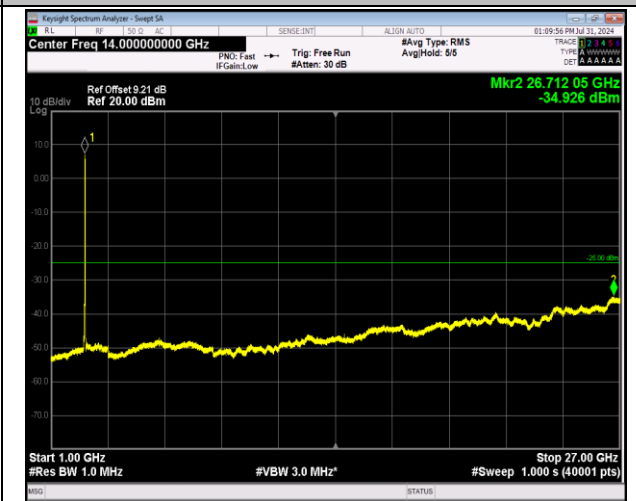
7-7-20MHz-10MHz-64QAM-64QAM-21251-21395-100RB#0-50RB#0-1000~27000MHz-PASS
