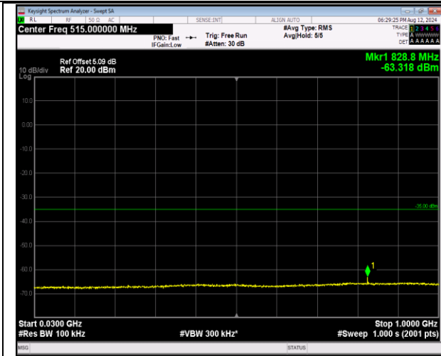
7-7-20MHz-20MHz-QPSK-QPSK-21152-21350-1RB#0-0 RB#0-30~1000MHz-PASS
