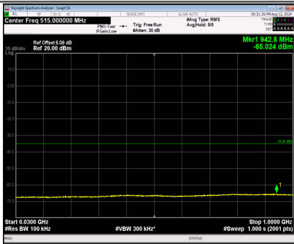
7-7-20MHz-10MHz-16QAM-16QAM-21251-21395-100R B#0-50RB#0-30~1000MHz-PASS
