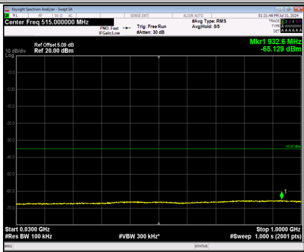
7-7-20MHz-20MHz-64QAM-64QAM-20850-21048-1RB#99-0RB#0-30~1000MHz-PASS
