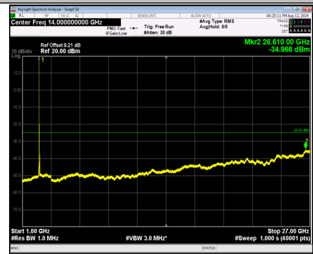
7-7-20MHz-20MHz-16QAM-16QAM-21001-21199-1RB#0-0-0RB#0-1000~27000MHz-PASS
