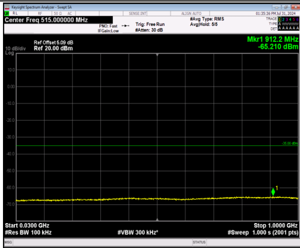
7-7-20MHz-20MHz-64QAM-64QAM-21001-21199-100RB#0-100RB#0-30~1000MHz-PASS
