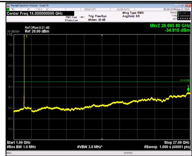
7-7-20MHz-10MHz-16QAM-16QAM-21251-21395-1RB#9 9-0RB#0-1000~27000MHz-PASS
