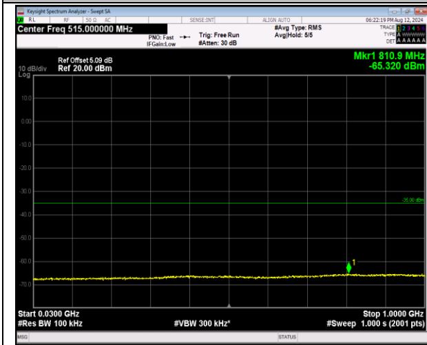
7-7-20MHz-20MHz-16QAM-16QAM-20850-21048-1RB# 0-1RB#99-30~1000MHz-PASS
