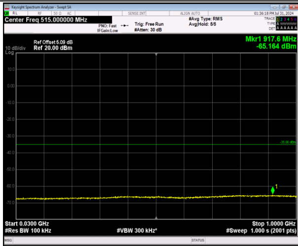
7-7-20MHz-20MHz-64QAM-64QAM-21152-21350-1RB#7-7-20MHz-20MHz-64QAM-64QAM-21152-21350-1RB#0-0-0RB#0-30~1000MHz-PASS
