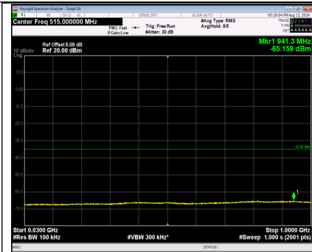
7-7-20MHz-10MHz-16QAM-16QAM-21251-21395-1RB# 99-0RB#0-30~1000MHz-PASS
