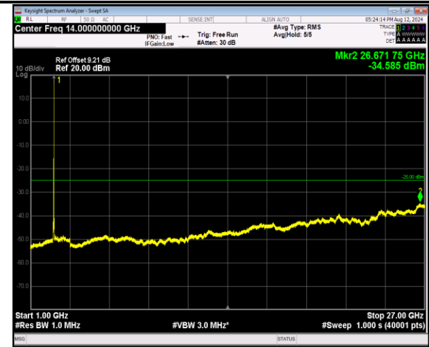
7-7-20MHz-10MHz-16QAM-16QAM-21051-21195-1RB#99-0RB#0-1000~27000MHz-PASS
