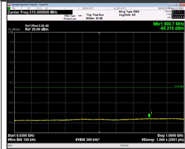
7-7-20MHz-20MHz-QPSK-QPSK-21152-21350-100RB#0 -100RB#0-30~1000MHz-PASS
