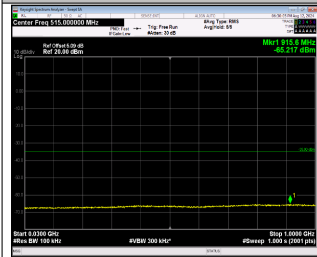
7-7-20MHz-20MHz-16QAM-16QAM-21152-21350-1RB#0 0-0RB#0-30~1000MHz-PASS
