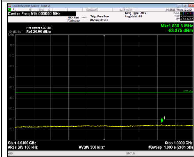
7-7-20MHz-20MHz-16QAM-16QAM-21001-21199-1RB#0-0-0RB#0-30~1000MHz-PASS
