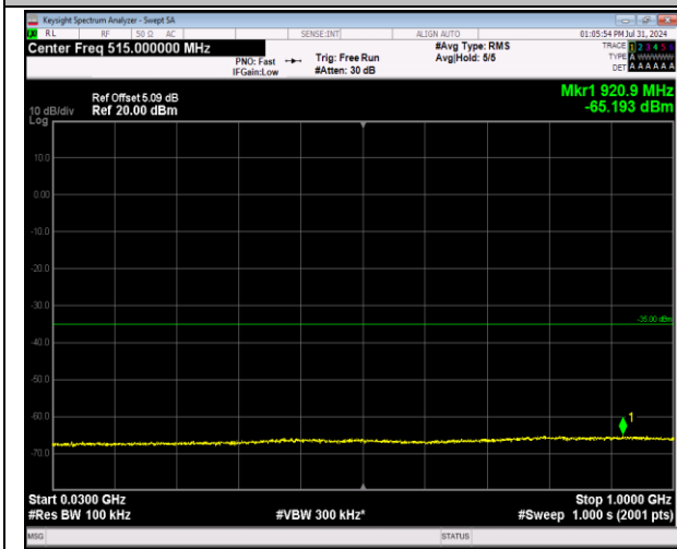
7-7-20MHz-10MHz-64QAM-64QAM-21051-21195-1RB#99-0RB#0-30~1000MHz-PASS
