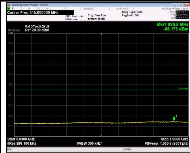
7-7-20MHz-10MHz-QPSK-QPSK-21251-21395-1RB#0-0 RB#0-30~1000MHz-PASS
