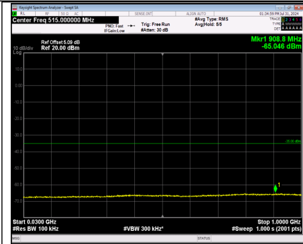
7-7-20MHz-20MHz-64QAM-64QAM-21001-21199-1RB#0-1RB#99-30~1000MHz-PASS
