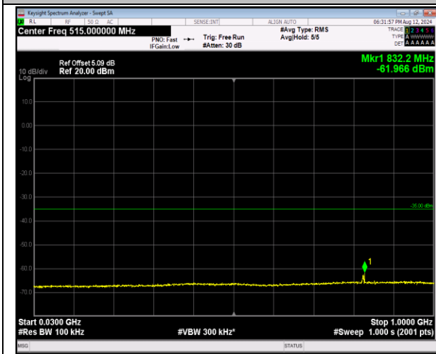
7-7-20MHz-20MHz-QPSK-QPSK-21152-21350-1RB#0-1 RB#99-30~1000MHz-PASS
