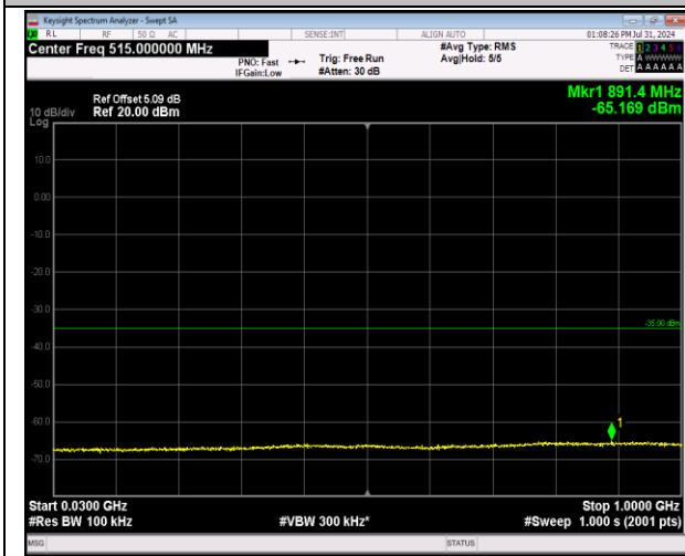
7-7-20MHz-10MHz-64QAM-64QAM-21251-21395-1RB#99-0RB#0-30~1000MHz-PASS
