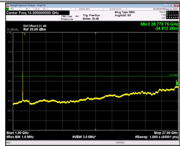
7-7-20MHz-10MHz-16QAM-16QAM-21251-21395-1RB#0 -0RB#0-1000~27000MHz-PASS
