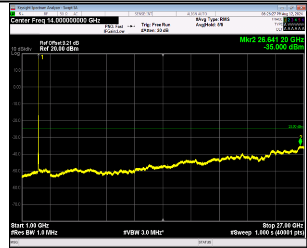
7-7-20MHz-20MHz-16QAM-16QAM-21001-21199-1RB#99-0RB#0-1000~27000MHz-PASS
