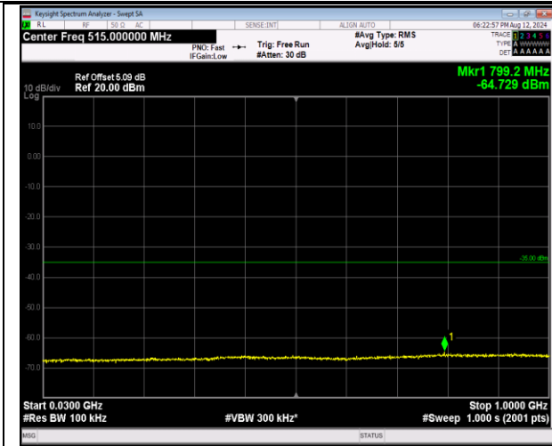
7-7-20MHz-20MHz-QPSK-QPSK-20850-21048-100RB# 0-100RB#0-30~1000MHz-PASS
