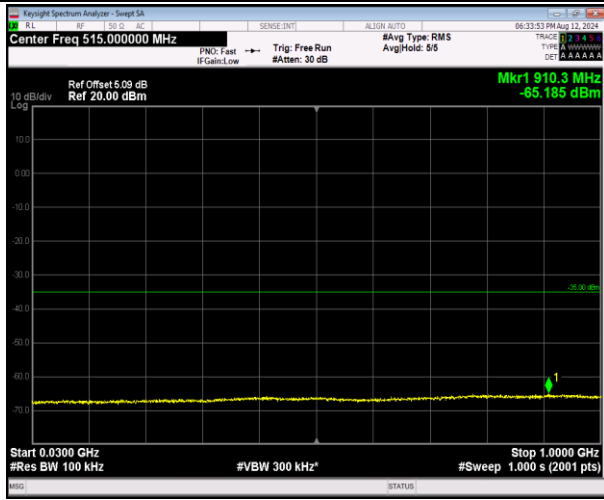
7-7-20MHz-20MHz-16QAM-16QAM-21152-21350-100RB#7-7-20MHz-20MHz-16QAM-16QAM-21152-21350-100RB#0-100RB#0-30~1000MHz-PASS
