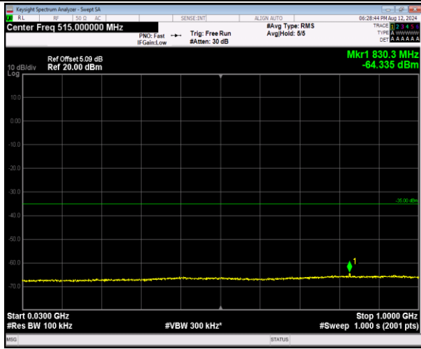
7-7-20MHz-20MHz-16QAM-16QAM-21001-21199-100RB#0-100RB#0-30~1000MHz-PASS
