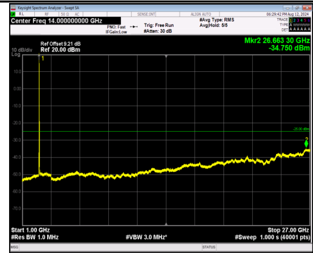
7-7-20MHz-20MHz-QPSK-QPSK-21152-21350-1RB#0-0 RB#0-1000~27000MHz-PASS
