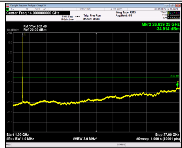
7-7-20MHz-20MHz-64QAM-64QAM-20850-21048-1RB#9-0RB#0-1000~27000MHz-PASS
