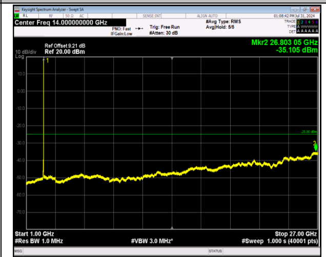
7-7-20MHz-10MHz-64QAM-64QAM-21251-21395-1RB#99-0RB#0-1000~27000MHz-PASS
