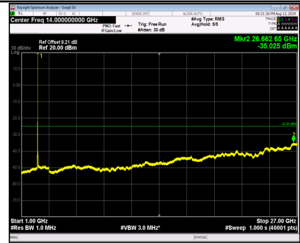
7-7-20MHz-20MHz-16QAM-16QAM-21152-21350-1RB#9-9-0RB#0-1000~27000MHz-PASS
