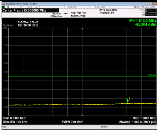
7-7-20MHz-20MHz-64QAM-64QAM-20850-21048-1RB# 0-0RB#0-30~1000MHz-PASS
