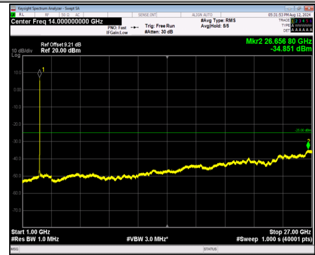
7-7-20MHz-10MHz-16QAM-16QAM-21251-21395-100RB #0-50RB#0-1000~27000MHz-PASS
