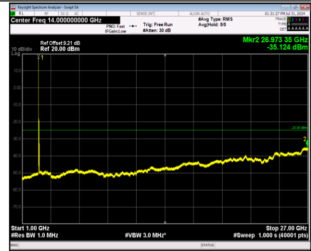
7-7-20MHz-20MHz-64QAM-64QAM-20850-21048-1RB#0 -0RB#0-1000~27000MHz-PASS
