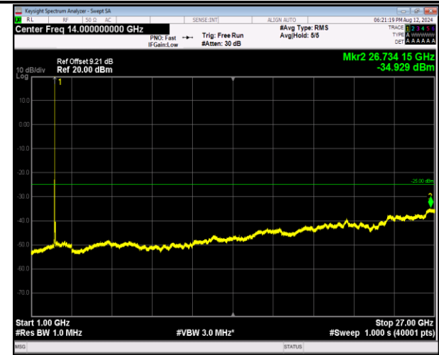
7-7-20MHz-20MHz-16QAM-16QAM-20850-21048-1RB#9 9-0RB#0-1000~27000MHz-PASS
