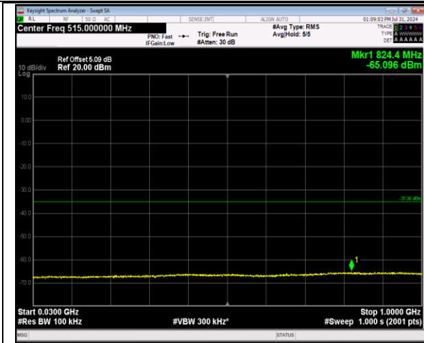
7-7-20MHz-10MHz-64QAM-64QAM-21251-21395-1RB#0-1RB#49-30~1000MHz-PASS
