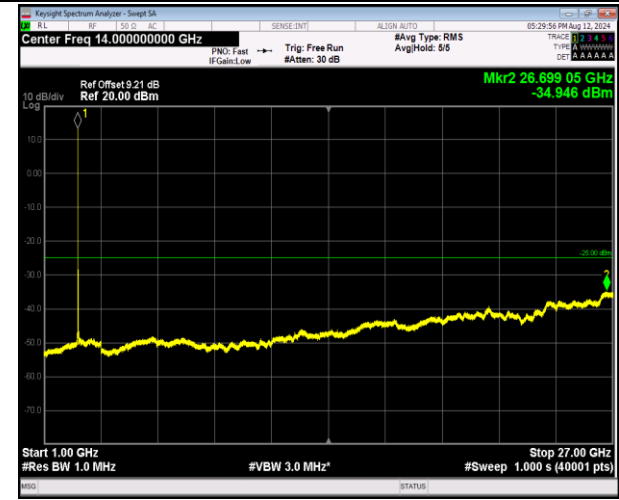
7-7-20MHz-10MHz-QPSK-QPSK-21251-21395-1RB#0-1 RB#49-1000~27000MHz-PASS
