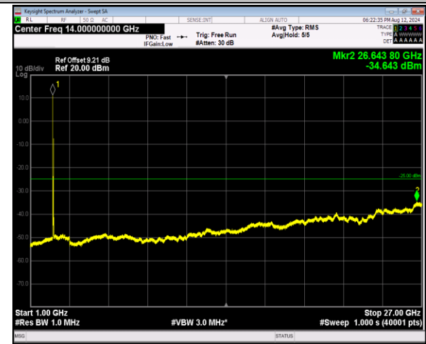
7-7-20MHz-20MHz-16QAM-16QAM-20850-21048-1RB#0 -1RB#99-1000~27000MHz-PASS
