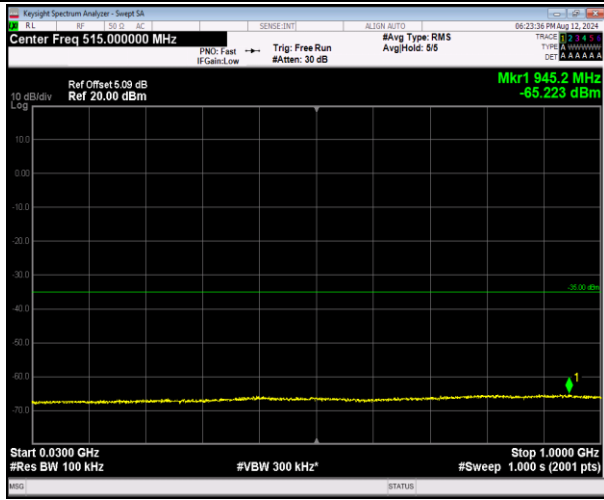
7-7-20MHz-20MHz-16QAM-16QAM-20850-21048-100R B#0-100RB#0-30~1000MHz-PASS
