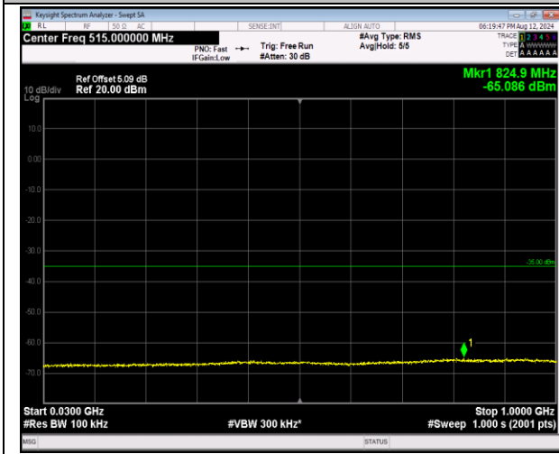
7-7-20MHz-20MHz-16QAM-16QAM-20850-21048-1RB# 0-0RB#0-30~1000MHz-PASS
