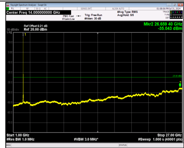
7-7-20MHz-10MHz-64QAM-64QAM-21251-21395-1RB#0 -0RB#0-1000~27000MHz-PASS
