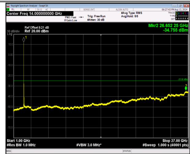
7-7-20MHz-20MHz-16QAM-16QAM-21001-21199-1RB#0-0-1RB#99-1000~27000MHz-PASS
