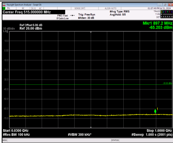
7-7-20MHz-10MHz-64QAM-64QAM-21251-21395-1RB# 0-0RB#0-30~1000MHz-PASS
