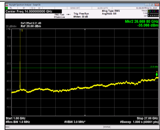
7-7-20MHz-10MHz-64QAM-64QAM-21051-21195-1RB#99-0RB#0-1000~27000MHz-PASS
