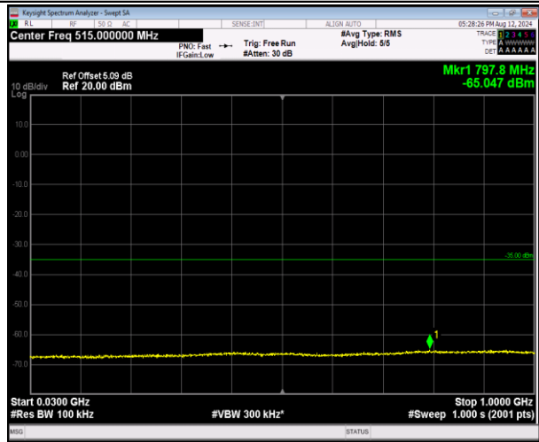
7-7-20MHz-10MHz-QPSK-QPSK-21251-21395-1RB#99-0 ORB#0-30~1000MHz-PASS
