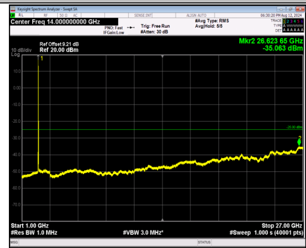
7-7-20MHz-20MHz-16QAM-16QAM-21152-21350-1RB#0- 0RB#0-1000~27000MHz-PASS
