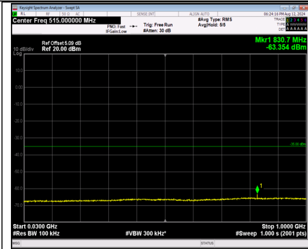
7-7-20MHz-20MHz-QPSK-QPSK-21001-21199-1RB#0-0 RB#0-30~1000MHz-PASS
