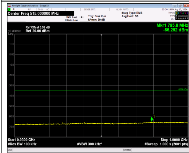
7-7-20MHz-10MHz-16QAM-16QAM-21251-21395-1RB# 0-1RB#49-30~1000MHz-PASS
