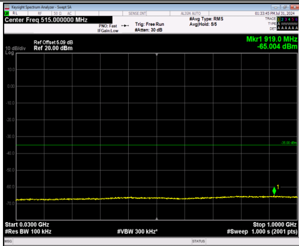
7-7-20MHz-20MHz-64QAM-64QAM-21001-21199-1RB#0-0RB#0-30~1000MHz-PASS
