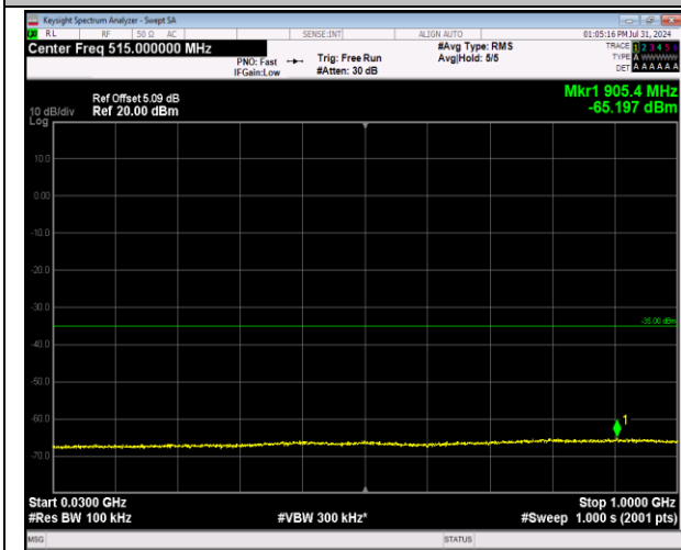
7-7-20MHz-10MHz-64QAM-64QAM-21051-21195-1RB#0-0RB#0-30~1000MHz-PASS
