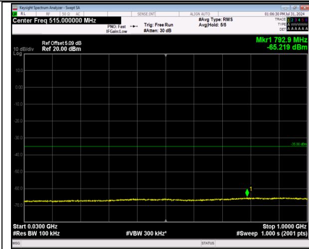
7-7-20MHz-10MHz-64QAM-64QAM-21051-21195-1RB#0-1RB#49-30~1000MHz-PASS
