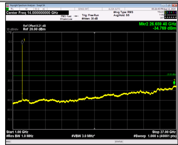
7-7-20MHz-10MHz-16QAM-16QAM-21051-21195-100RB#0-50RB#0-1000~27000MHz-PASS
