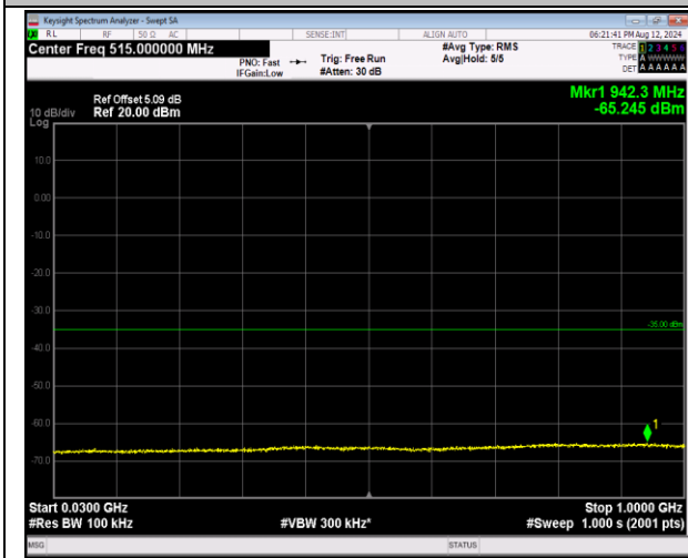
7-7-20MHz-20MHz-QPSK-QPSK-20850-21048-1RB#0-1 RB#99-30~1000MHz-PASS
