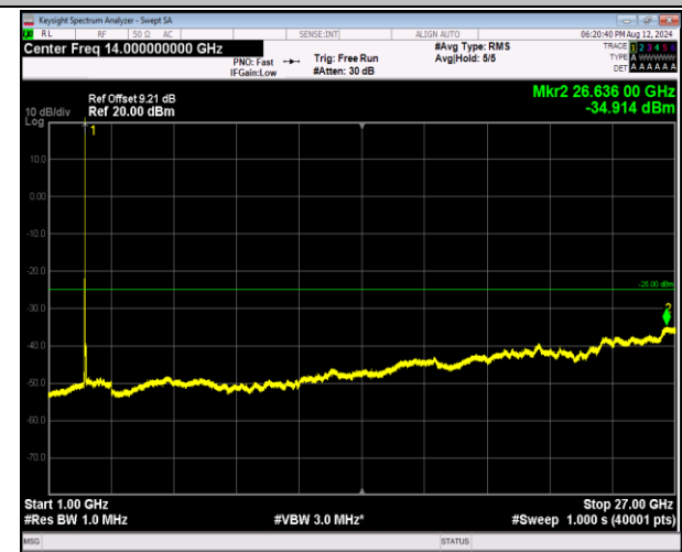
7-7-20MHz-20MHz-QPSK-QPSK-20850-21048-1RB#99-0 RB#0-1000~27000MHz-PASS
