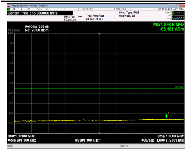
7-7-20MHz-20MHz-16QAM-16QAM-21152-21350-1RB#0 0-1RB#99-30~1000MHz-PASS
