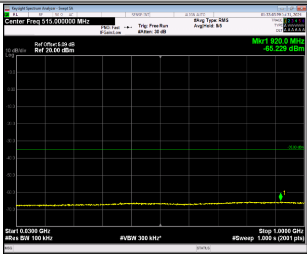
7-7-20MHz-20MHz-64QAM-64QAM-20850-21048-100RB#0-100RB#0-30~1000MHz-PASS
