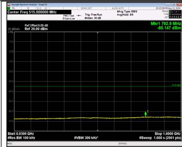
7-7-20MHz-10MHz-16QAM-16QAM-21051-21195-1RB#99-0RB#0-30~1000MHz-PASS
