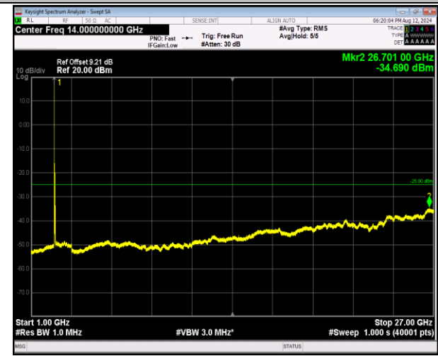
7-7-20MHz-20MHz-16QAM-16QAM-20850-21048-1RB#0 -0RB#0-1000~27000MHz-PASS
