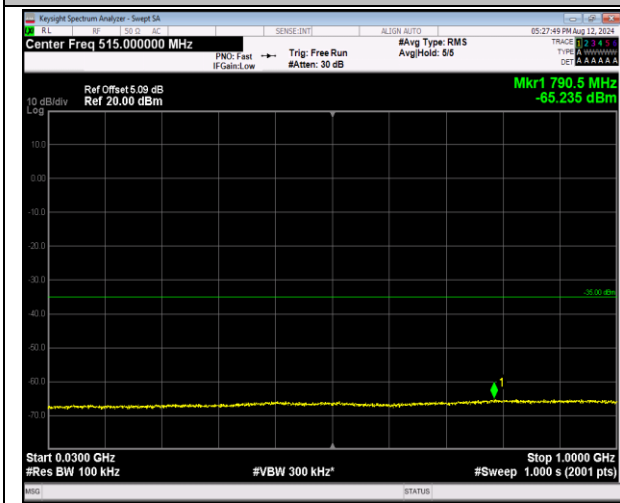
7-7-20MHz-10MHz-16QAM-16QAM-21251-21395-1RB# 0-0RB#0-30~1000MHz-PASS
