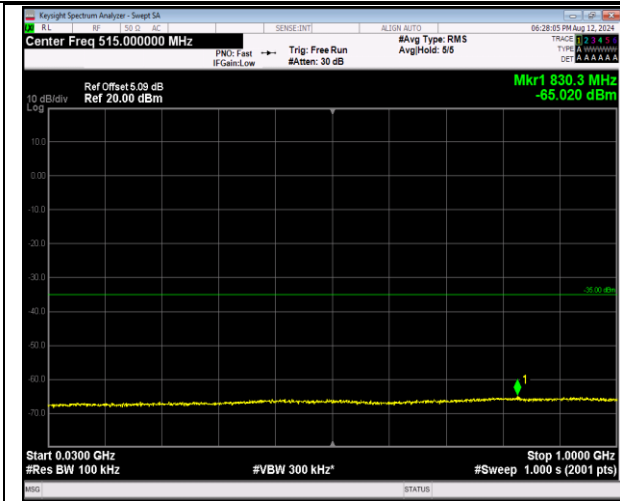
7-7-20MHz-20MHz-QPSK-QPSK-21001-21199-100RB#0-100RB#0-30~1000MHz-PASS
