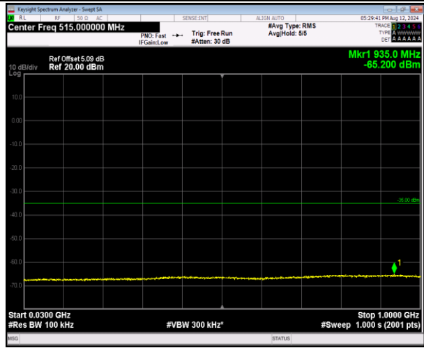
7-7-20MHz-10MHz-QPSK-QPSK-21251-21395-1RB#0-1 RB#49-30~1000MHz-PASS
