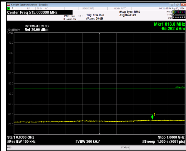
7-7-20MHz-20MHz-16QAM-16QAM-20850-21048-1RB# 99-0RB#0-30~1000MHz-PASS
