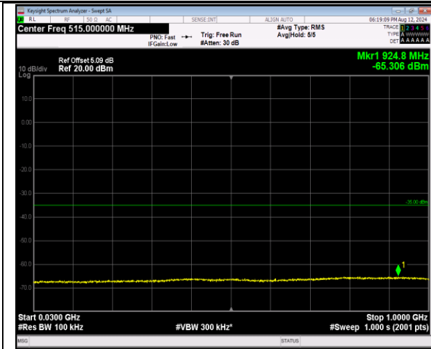
7-7-20MHz-20MHz-QPSK-QPSK-20850-21048-1RB#0-0 RB#0-30~1000MHz-PASS
