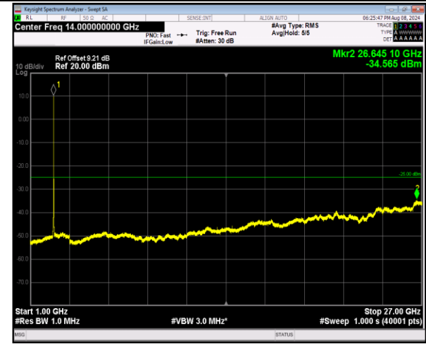
7-7-10MHz-20MHz-16QAM-16QAM-21206-21350-50RB# 0-100RB#0-1000~27000MHz-PASS
