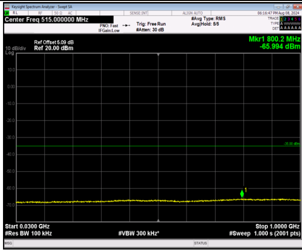
7-7-10MHz-20MHz-16QAM-16QAM-21006-21150-1RB#0-0RB#0-30~1000MHz-PASS
