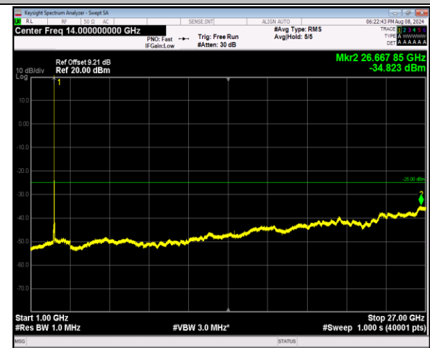
7-7-10MHz-20MHz-QPSK-QPSK-21206-21350-1RB#49-0 RB#0-1000~27000MHz-PASS
