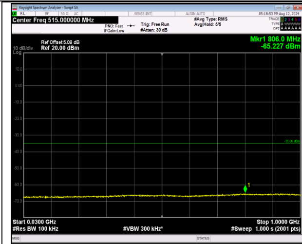
7-7-20MHz-10MHz-16QAM-16QAM-20850-20994-1RB# 99-0RB#0-30~1000MHz-PASS
