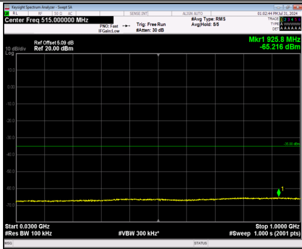
7-7-20MHz-10MHz-64QAM-64QAM-20850-20994-1RB# 0-0RB#0-30~1000MHz-PASS
