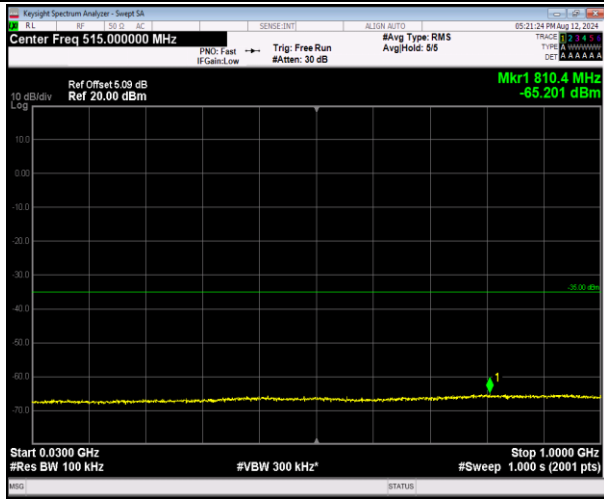
7-7-20MHz-10MHz-16QAM-16QAM-20850-20994-100R B#0-50RB#0-30~1000MHz-PASS
