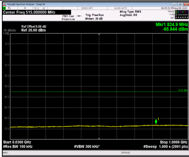
7-7-10MHz-20MHz-16QAM-16QAM-21206-21350-50RB #0-100RB#0-30~1000MHz-PASS
