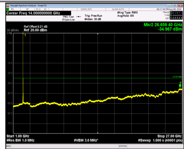
7-7-10MHz-20MHz-QPSK-QPSK-21006-21150-1RB#49-0 RB#0-1000~27000MHz-PASS
