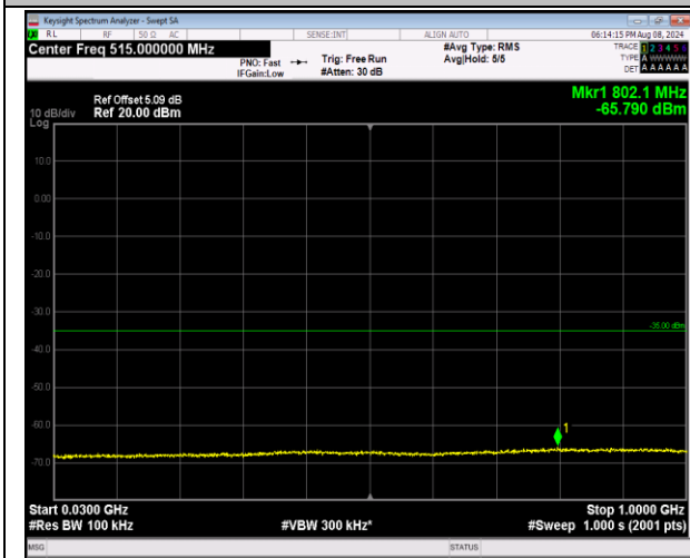
7-7-10MHz-20MHz-16QAM-16QAM-20805-20949-1RB#0-0-1RB#99-30~1000MHz-PASS
