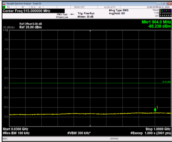
7-7-10MHz-20MHz-64QAM-64QAM-20805-20949-1RB# 0-0RB#0-30~1000MHz-PASS
