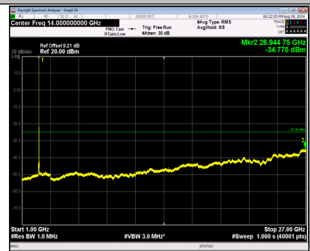
7-7-10MHz-20MHz-16QAM-16QAM-21206-21350-1RB#0-0-0RB#0-1000~27000MHz-PASS
