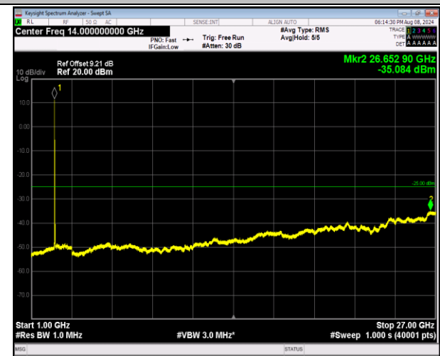
7-7-10MHz-20MHz-16QAM-16QAM-20805-20949-1RB#0-0-1RB#99-1000~27000MHz-PASS
