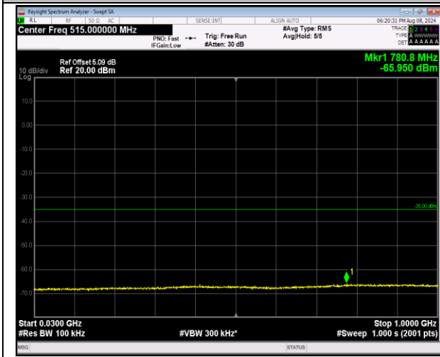
7-7-10MHz-20MHz-16QAM-16QAM-21006-21150-50RB #0-100RB#0-30~1000MHz-PASS
