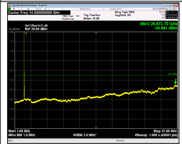
7-7-20MHz-10MHz-16QAM-16QAM-21051-21195-1RB#0-0-0RB#0-1000~27000MHz-PASS
