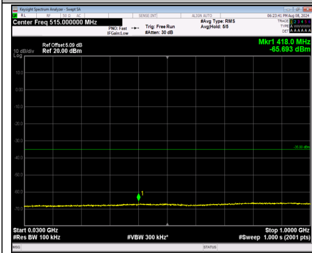
7-7-10MHz-20MHz-QPSK-QPSK-21206-21350-1RB#0-1 RB#99-30~1000MHz-PASS
