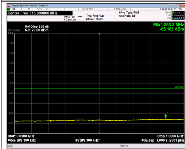
7-7-10MHz-20MHz-64QAM-64QAM-21006-21150-50RB#0-100RB#0-30~1000MHz-PASS
