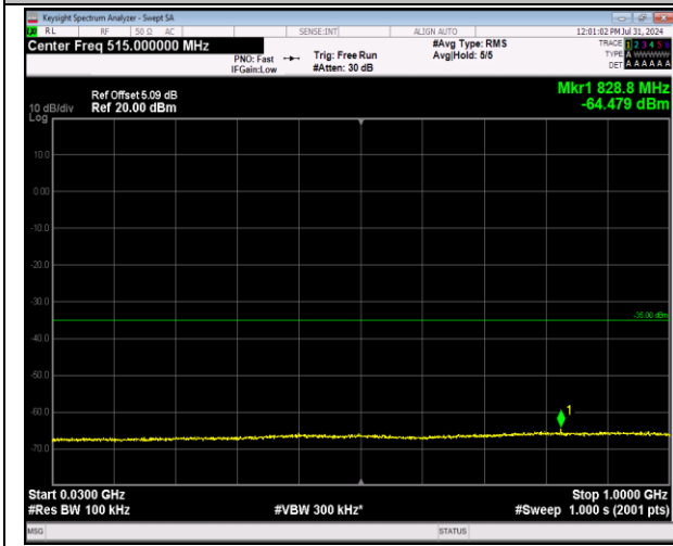
7-7-10MHz-20MHz-64QAM-64QAM-20805-20949-1RB#4 49-0RB#0-30~1000MHz-PASS
