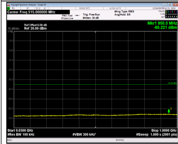
7-7-10MHz-20MHz-64QAM-64QAM-21206-21350-1RB#4 49-0RB#0-30~1000MHz-PASS
