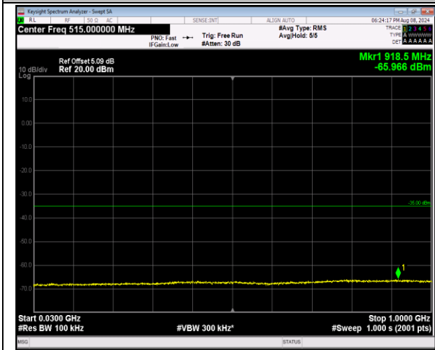
7-7-10MHz-20MHz-16QAM-16QAM-21206-21350-1RB#0-0-1RB#99-30~1000MHz-PASS
