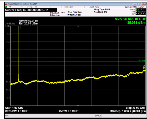
7-7-10MHz-20MHz-64QAM-64QAM-20805-20949-1RB#4 9-0RB#0-1000~27000MHz-PASS
