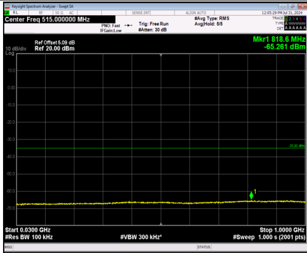
7-7-10MHz-20MHz-64QAM-64QAM-21206-21350-1RB# 0-0RB#0-30~1000MHz-PASS
