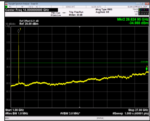
7-7-20MHz-10MHz-64QAM-64QAM-20850-20994-1RB#0-1RB#49-1000~27000MHz-PASS
