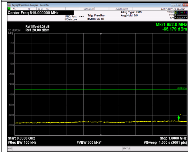
7-7-10MHz-20MHz-64QAM-64QAM-21206-21350-50RB #0-100RB#0-30~1000MHz-PASS
