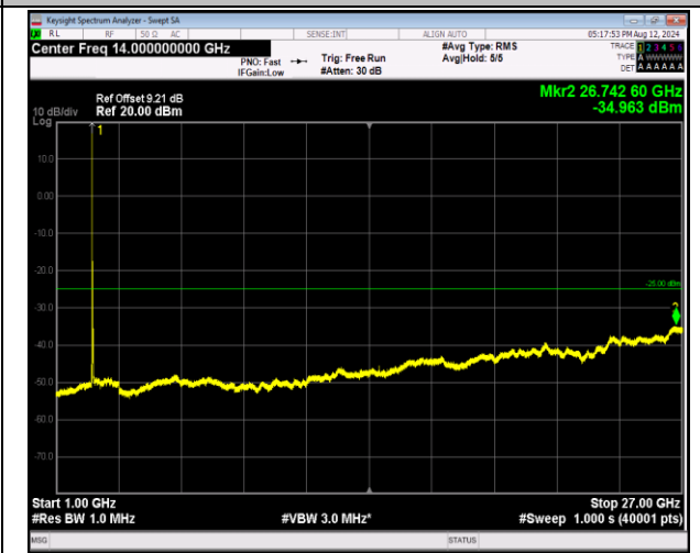
7-7-20MHz-10MHz-16QAM-16QAM-20850-20994-1RB#0-0-0RB#0-1000~27000MHz-PASS
