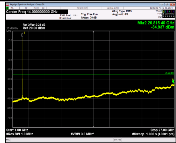
7-7-10MHz-20MHz-64QAM-64QAM-21206-21350-1RB#0 -1RB#99-1000~27000MHz-PASS
