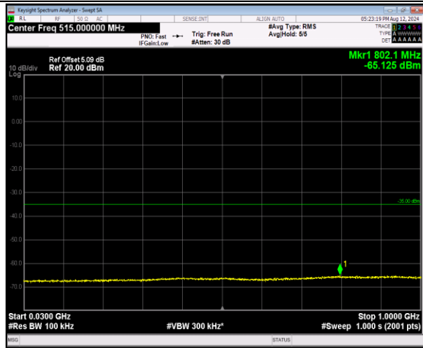
7-7-20MHz-10MHz-QPSK-QPSK-21051-21195-1RB#99-0 ORB#0-30~1000MHz-PASS
