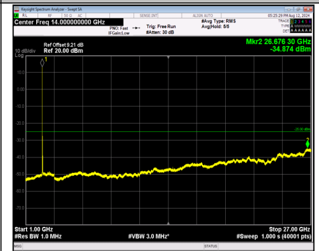
7-7-20MHz-10MHz-16QAM-16QAM-21051-21195-1RB#0-0-1RB#49-1000~27000MHz-PASS
