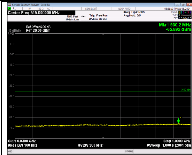
7-7-10MHz-20MHz-QPSK-QPSK-21206-21350-1RB#0-0 RB#0-30~1000MHz-PASS
