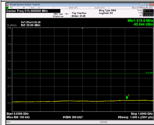
7-7-10MHz-20MHz-16QAM-16QAM-20805-20949-1RB#0-0-0RB#0-30~1000MHz-PASS
