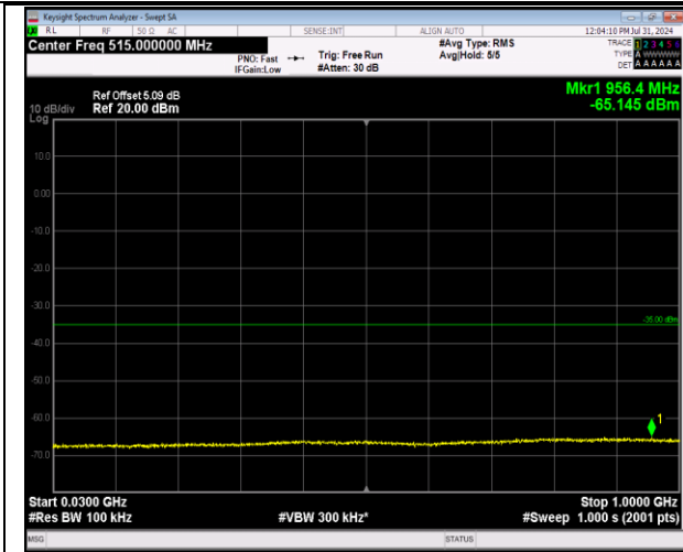
7-7-10MHz-20MHz-64QAM-64QAM-21006-21150-1RB#0-1RB#99-30~1000MHz-PASS
