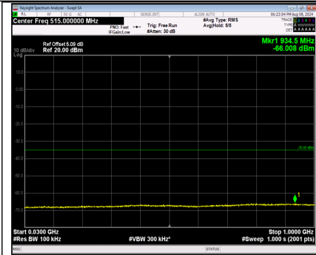
7-7-10MHz-20MHz-16QAM-16QAM-21206-21350-1RB# 49-0RB#0-30~1000MHz-PASS
