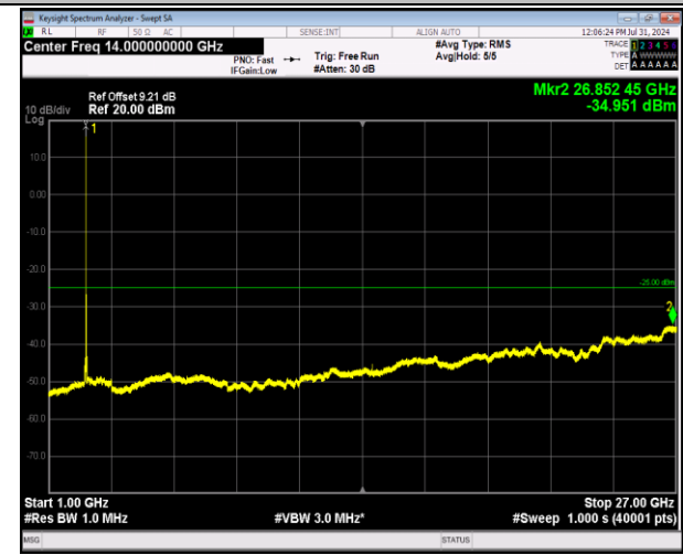
7-7-10MHz-20MHz-64QAM-64QAM-21206-21350-1RB#4 9-0RB#0-1000~27000MHz-PASS
