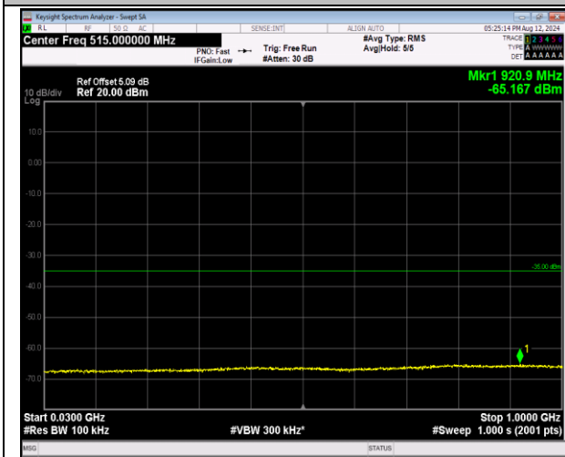
7-7-20MHz-10MHz-16QAM-16QAM-21051-21195-1RB#0-0-1RB#49-30~1000MHz-PASS
