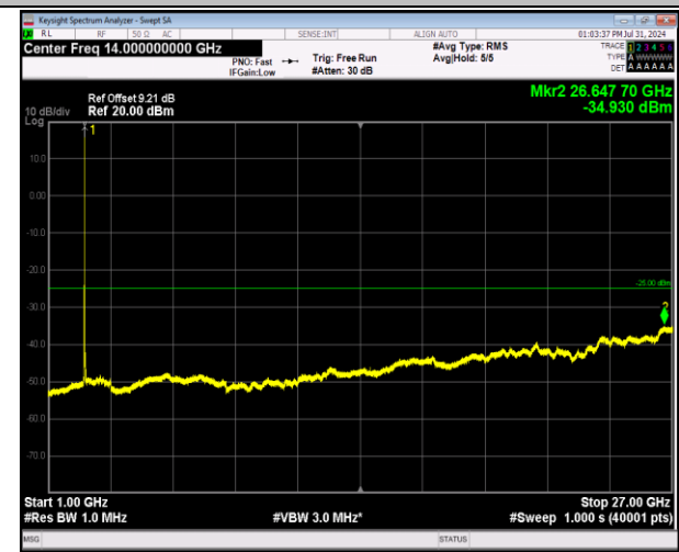
7-7-20MHz-10MHz-64QAM-64QAM-20850-20994-1RB#99-0RB#0-1000~27000MHz-PASS
