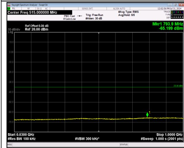
7-7-10MHz-20MHz-64QAM-64QAM-21006-21150-1RB#4 0-0RB#0-30~1000MHz-PASS
