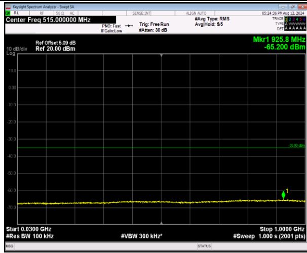
7-7-20MHz-10MHz-QPSK-QPSK-21051-21195-1RB#0-1 RB#49-30~1000MHz-PASS
