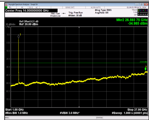
7-7-20MHz-10MHz-64QAM-64QAM-20850-20994-100RB#0-50RB#0-1000~27000MHz-PASS
