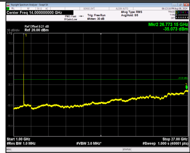
7-7-10MHz-20MHz-16QAM-16QAM-20805-20949-1RB#4 9-0RB#0-1000~27000MHz-PASS
