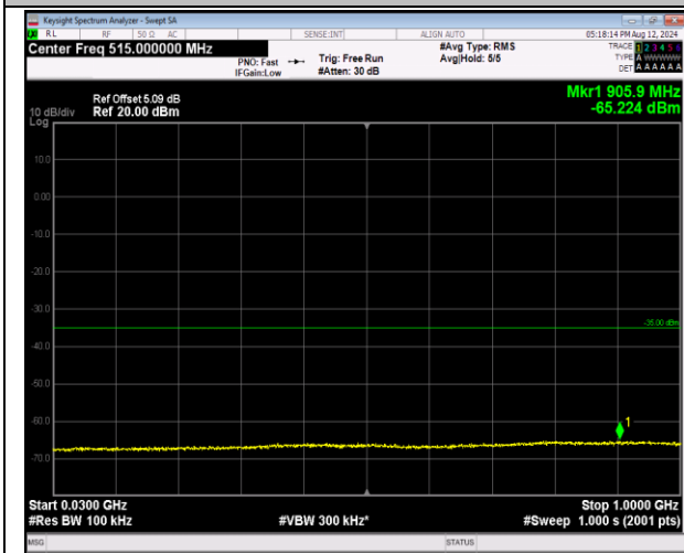
7-7-20MHz-10MHz-QPSK-QPSK-20850-20994-1RB#99-0 ORB#0-30~1000MHz-PASS
