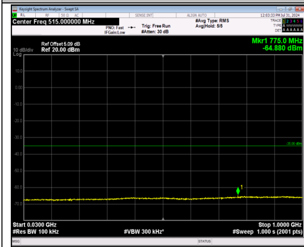
7-7-10MHz-20MHz-64QAM-64QAM-21006-21150-1RB#0-49-0RB#0-30~1000MHz-PASS
