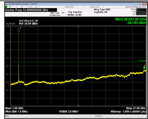
7-7-10MHz-20MHz-16QAM-16QAM-21206-21350-1RB#0-0-1RB#99-1000~27000MHz-PASS
