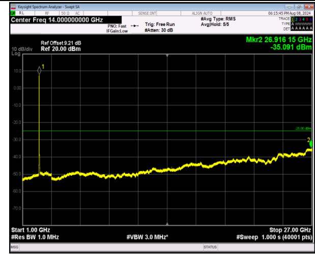
7-7-10MHz-20MHz-16QAM-16QAM-20805-20949-50RB# 0-100RB#0-1000~27000MHz-PASS
