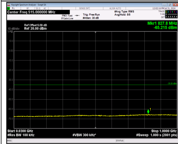
7-7-10MHz-20MHz-64QAM-64QAM-20805-20949-50RB #0-100RB#0-30~1000MHz-PASS
