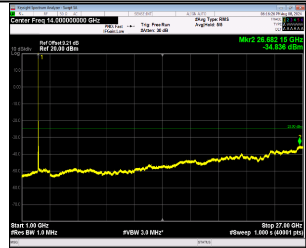
7-7-10MHz-20MHz-QPSK-QPSK-21006-21150-1RB#0-0 RB#0-1000~27000MHz-PASS
