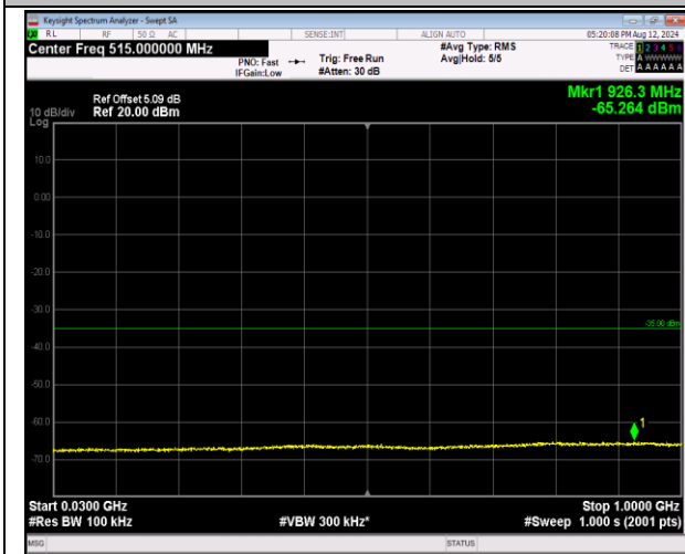
7-7-20MHz-10MHz-16QAM-16QAM-20850-20994-1RB#0-0-1RB#49-30~1000MHz-PASS
