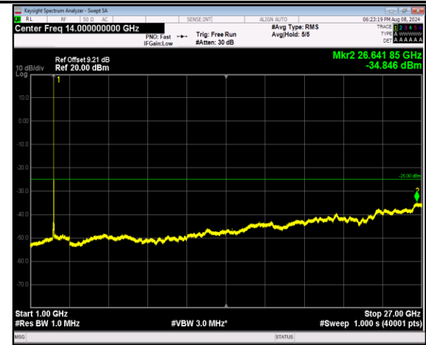
7-7-10MHz-20MHz-16QAM-16QAM-21206-21350-1RB#4 9-0RB#0-1000~27000MHz-PASS
