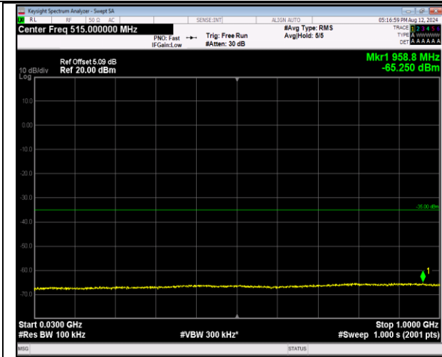
7-7-20MHz-10MHz-QPSK-QPSK-20850-20994-1RB#0-0 RB#0-30~1000MHz-PASS
