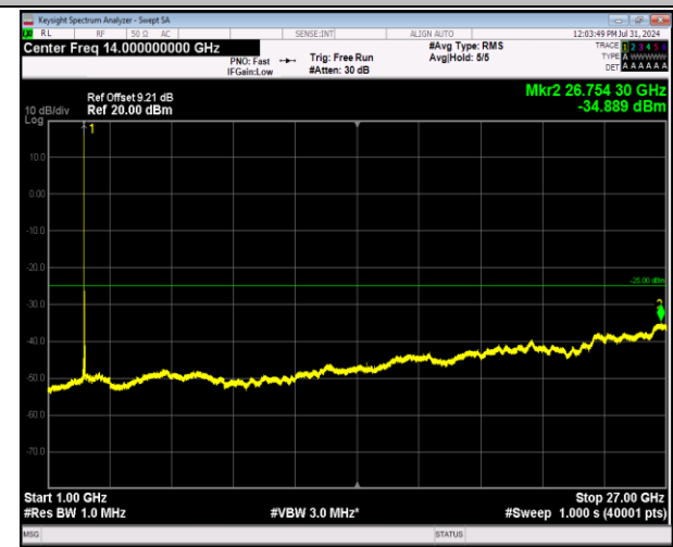
7-7-10MHz-20MHz-64QAM-64QAM-21006-21150-1RB#0-49-0RB#0-1000~27000MHz-PASS
