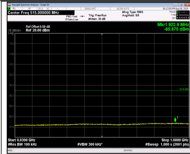
7-7-10MHz-20MHz-16QAM-16QAM-20805-20949-1RB# 49-0RB#0-30~1000MHz-PASS
