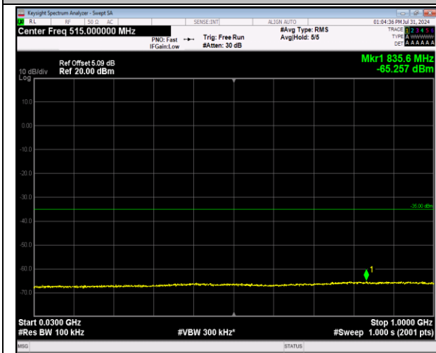
7-7-20MHz-10MHz-64QAM-64QAM-20850-20994-100RB#0-50RB#0-30~1000MHz-PASS
