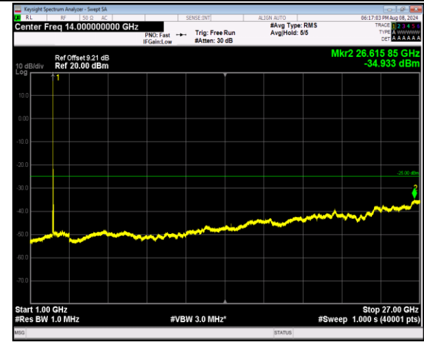
7-7-10MHz-20MHz-16QAM-16QAM-21006-21150-1RB#0-0RB#0-1000~27000MHz-PASS
