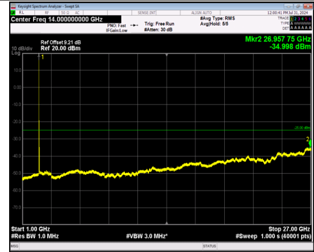
7-7-10MHz-20MHz-64QAM-64QAM-20805-20949-1RB#0 -0RB#0-1000~27000MHz-PASS
