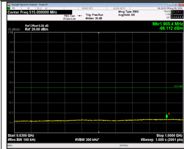
7-7-10MHz-20MHz-16QAM-16QAM-21006-21150-1RB#4 49-0RB#0-30~1000MHz-PASS
