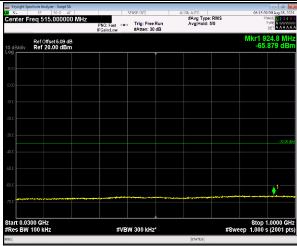
7-7-10MHz-20MHz-16QAM-16QAM-20805-20949-50RB #0-100RB#0-30~1000MHz-PASS
