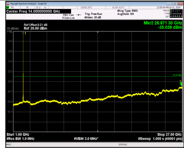
7-7-10MHz-20MHz-64QAM-64QAM-21206-21350-1RB#0 -0RB#0-1000~27000MHz-PASS
