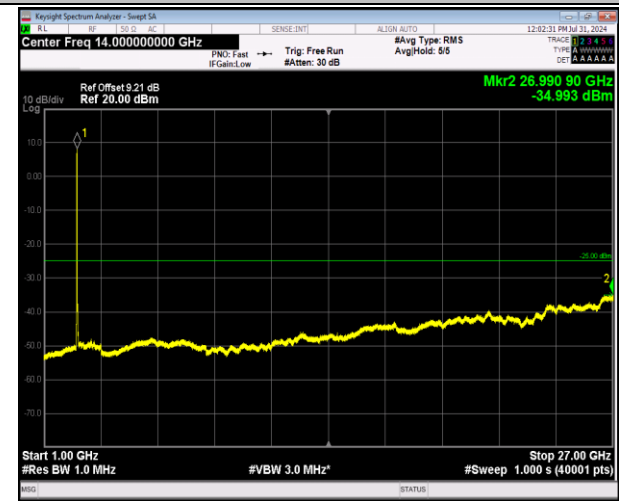
7-7-10MHz-20MHz-64QAM-64QAM-20805-20949-50RB# 0-100RB#0-1000~27000MHz-PASS
