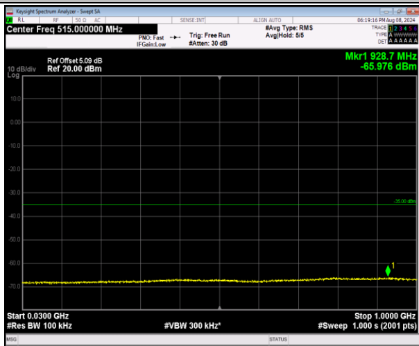
7-7-10MHz-20MHz-16QAM-16QAM-21006-21150-1RB#0-0-1RB#99-30~1000MHz-PASS
