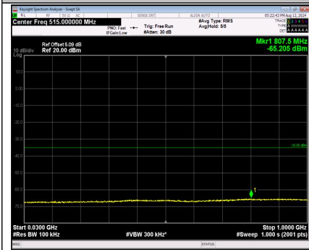
7-7-20MHz-10MHz-16QAM-16QAM-21051-21195-1RB#0-0-0RB#0-30~1000MHz-PASS
