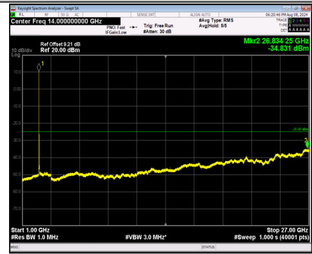
7-7-10MHz-20MHz-16QAM-16QAM-21006-21150-50RB# 0-100RB#0-1000~27000MHz-PASS
