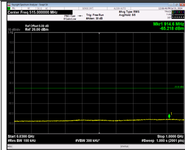
7-7-10MHz-20MHz-64QAM-64QAM-21206-21350-1RB# 0-1RB#99-30~1000MHz-PASS
