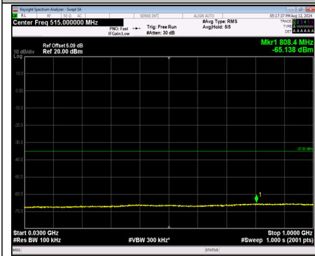
7-7-20MHz-10MHz-16QAM-16QAM-20850-20994-1RB#0-0-0RB#0-30~1000MHz-PASS
