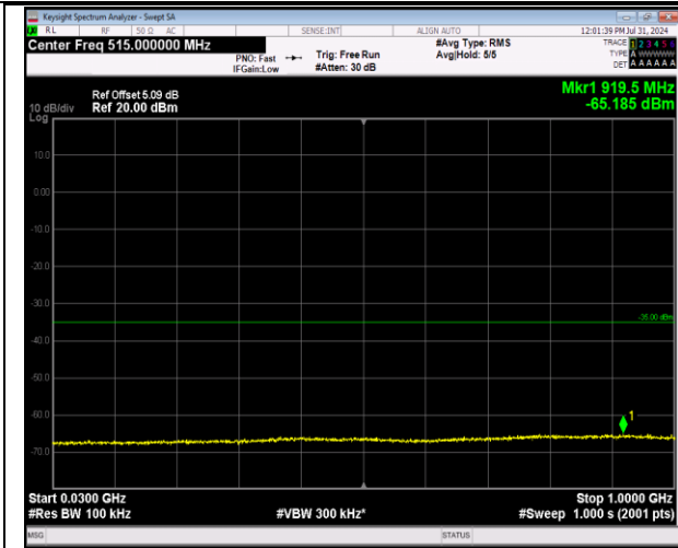
7-7-10MHz-20MHz-64QAM-64QAM-20805-20949-1RB# 0-1RB#99-30~1000MHz-PASS
