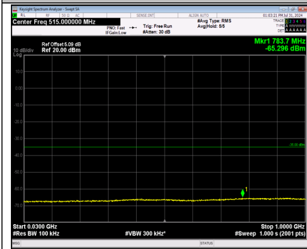
7-7-20MHz-10MHz-64QAM-64QAM-20850-20994-1RB#99-0RB#0-30~1000MHz-PASS
