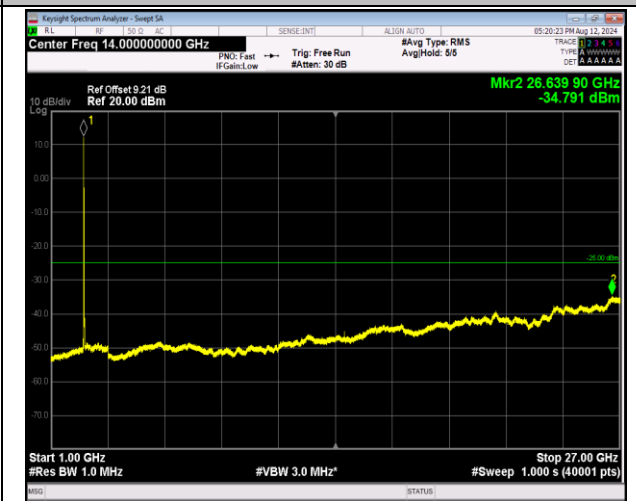
7-7-20MHz-10MHz-16QAM-16QAM-20850-20994-1RB#0-0-1RB#49-1000~27000MHz-PASS
