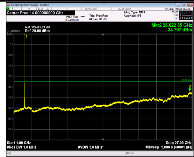
7-7-10MHz-20MHz-16QAM-16QAM-21006-21150-1RB#4 9-0RB#0-1000~27000MHz-PASS
