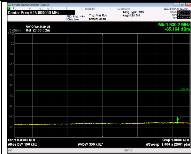
7-7-20MHz-10MHz-64QAM-64QAM-20850-20994-1RB#0-1RB#49-30~1000MHz-PASS
