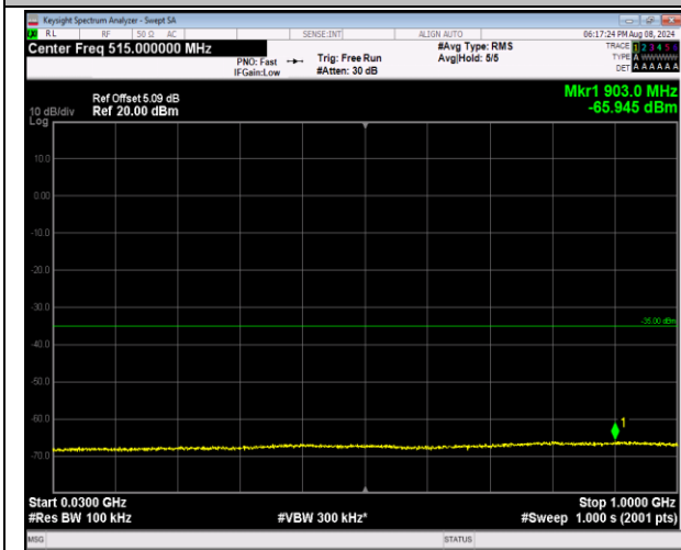
7-7-10MHz-20MHz-QPSK-QPSK-21006-21150-1RB#49-0 ORB#0-30~1000MHz-PASS
