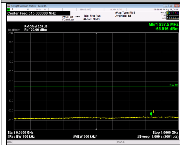
7-7-10MHz-20MHz-16QAM-16QAM-21206-21350-1RB#0-0-0RB#0-30~1000MHz-PASS
