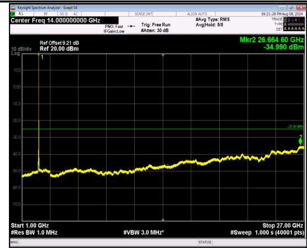
7-7-10MHz-20MHz-QPSK-QPSK-21206-21350-1RB#0-0 RB#0-1000~27000MHz-PASS
