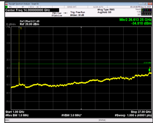
7-7-20MHz-10MHz-16QAM-16QAM-20850-20994-1RB#9 9-0RB#0-1000~27000MHz-PASS
