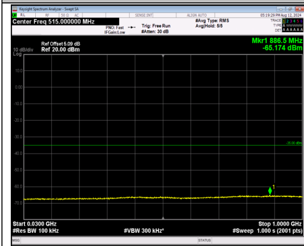
7-7-20MHz-10MHz-QPSK-QPSK-20850-20994-1RB#0-1 RB#49-30~1000MHz-PASS
