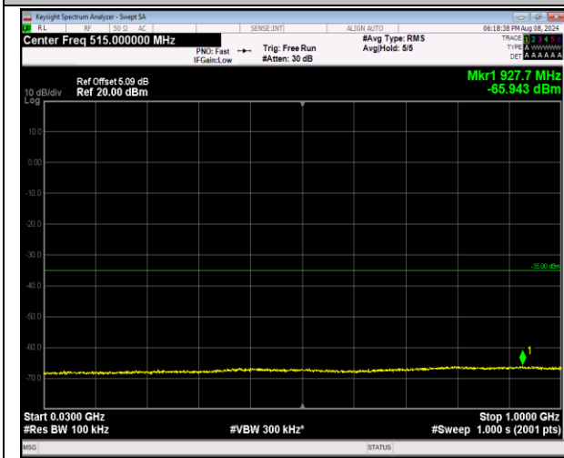
7-7-10MHz-20MHz-QPSK-QPSK-21006-21150-1RB#0-1 RB#99-30~1000MHz-PASS
