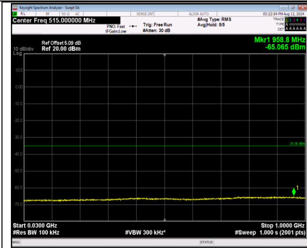
7-7-20MHz-10MHz-QPSK-QPSK-21051-21195-1RB#0-0 RB#0-30~1000MHz-PASS
