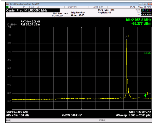
5-5-10MHz-10MHz-16QAM-16QAM-20476-20575-1RB#0-0-1RB#49-30~1000MHz-PASS
