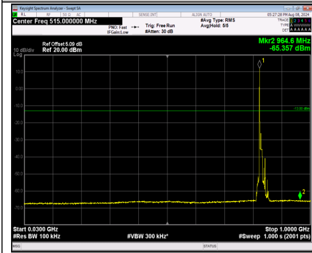
5-5-10MHz-10MHz-16QAM-16QAM-20476-20575-1RB#0-0RB#0-30~1000MHz-PASS
