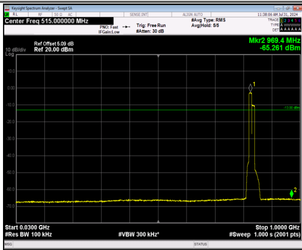
5-5-10MHz-10MHz-64QAM-64QAM-20450-20549-50RB#0-50RB#0-30~1000MHz-PASS
