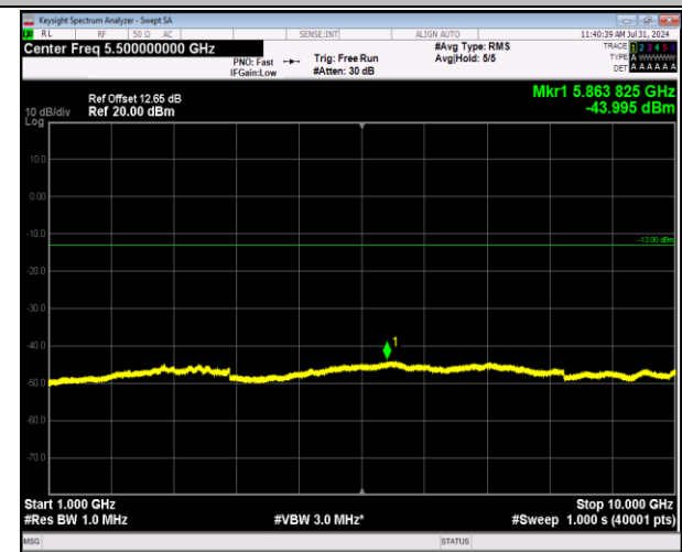
5-5-10MHz-10MHz-64QAM-64QAM-20476-20575-50RB# 0-50RB#0-1000~10000MHz-PASS
