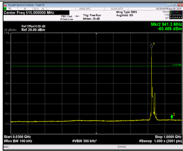
5-5-10MHz-10MHz-QPSK-QPSK-20476-20575-1RB#0-1 RB#49-30~1000MHz-PASS
