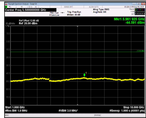
5-5-10MHz-10MHz-QPSK-QPSK-20476-20575-1RB#49-0 RB#0-1000~10000MHz-PASS
