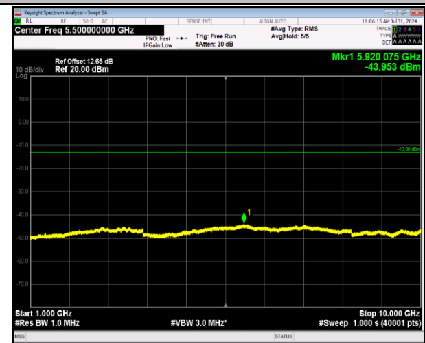
5-5-5MHz-3MHz-64QAM-64QAM-20595-20634-1RB#0-0RB#0-1000~10000MHz-PASS
