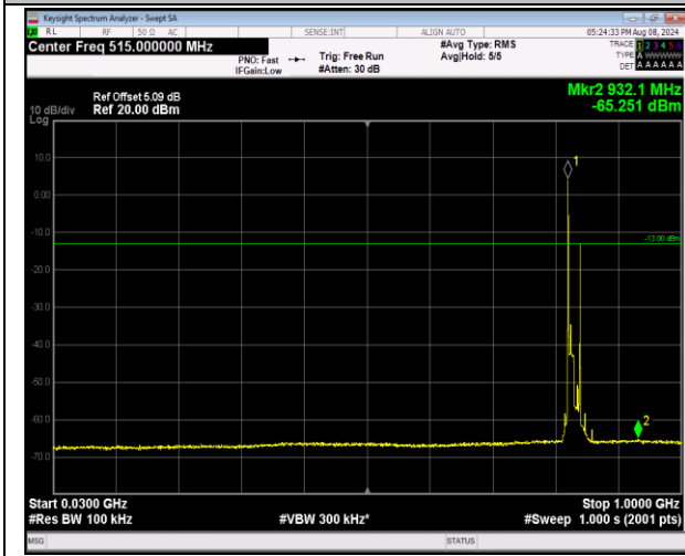
5-5-10MHz-10MHz-QPSK-QPSK-20450-20549-1RB#0-1 RB#49-30~1000MHz-PASS
