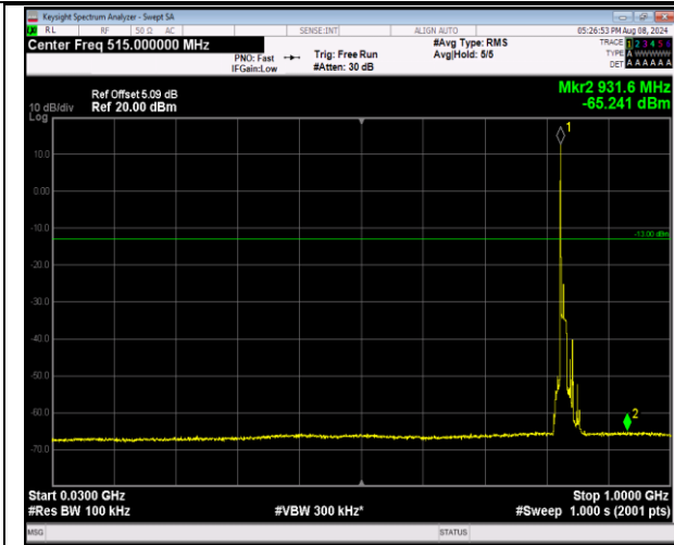
5-5-10MHz-10MHz-QPSK-QPSK-20476-20575-1RB#0-0 RB#0-30~1000MHz-PASS
