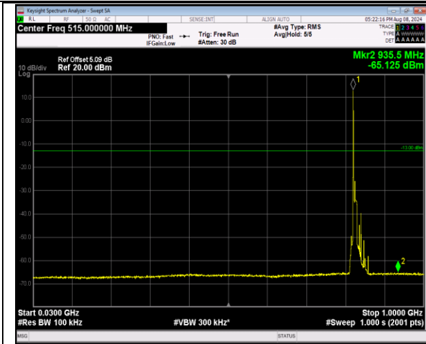
5-5-10MHz-10MHz-QPSK-QPSK-20450-20549-1RB#0-0 RB#0-30~1000MHz-PASS
