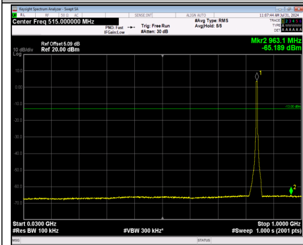
5-5-5MHz-3MHz-64QAM-64QAM-20595-20634-25RB#0- 15RB#0-30~1000MHz-PASS
