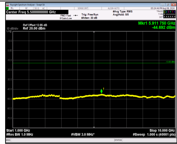
5-5-10MHz-10MHz-QPSK-QPSK-20450-20549-1RB#0-1 RB#49-1000~10000MHz-PASS
