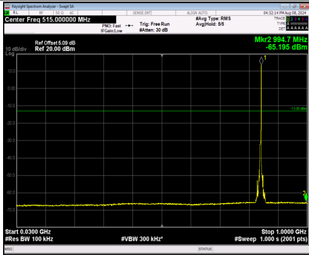
5-5-5MHz-3MHz-QPSK-QPSK-20595-20634-1RB#24-0R B#0-30~1000MHz-PASS
