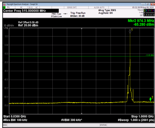
5-5-10MHz-10MHz-QPSK-QPSK-20501-20600-1RB#49-0 ORB#0-30~1000MHz-PASS
