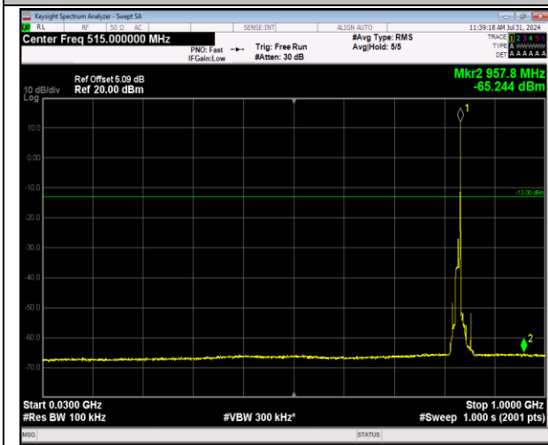
5-5-10MHz-10MHz-64QAM-64QAM-20476-20575-1RB#4 49-0RB#0-30~1000MHz-PASS
