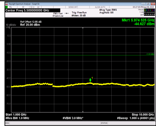
5-5-10MHz-10MHz-QPSK-QPSK-20476-20575-1RB#0-0 RB#0-1000~10000MHz-PASS
