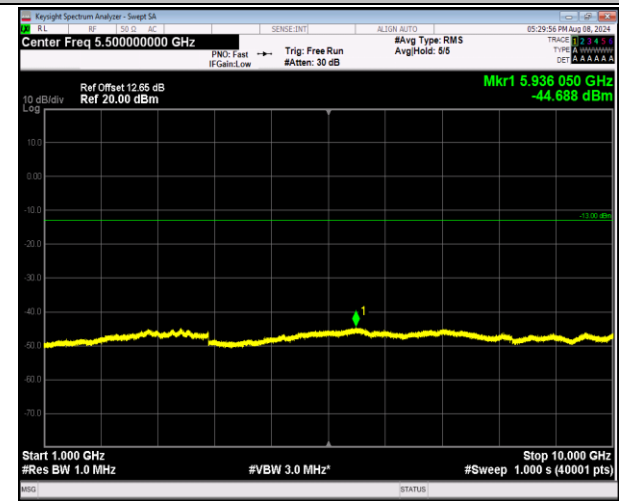
5-5-10MHz-10MHz-16QAM-16QAM-20476-20575-1RB#0-1RB#49-1000~10000MHz-PASS
