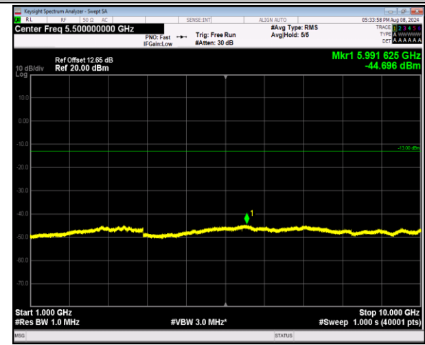
5-5-10MHz-10MHz-QPSK-QPSK-20501-20600-1RB#0-1 RB#49-1000~10000MHz-PASS
