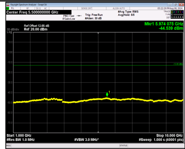
5-5-10MHz-10MHz-QPSK-QPSK-20450-20549-1RB#0-0 RB#0-1000~10000MHz-PASS
