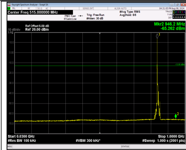
5-5-5MHz-3MHz-QPSK-QPSK-20595-20634-1RB#0-0R B#0-30~1000MHz-PASS
