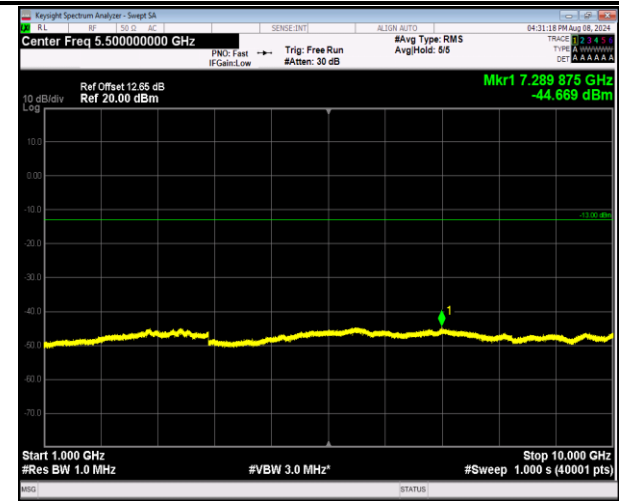
5-5-5MHz-3MHz-QPSK-QPSK-20595-20634-1RB#0-0RB #0-1000~10000MHz-PASS
