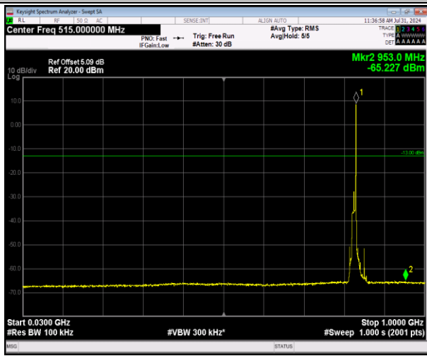
5-5-10MHz-10MHz-64QAM-64QAM-20450-20549-1RB#49-0RB#0-30~1000MHz-PASS
