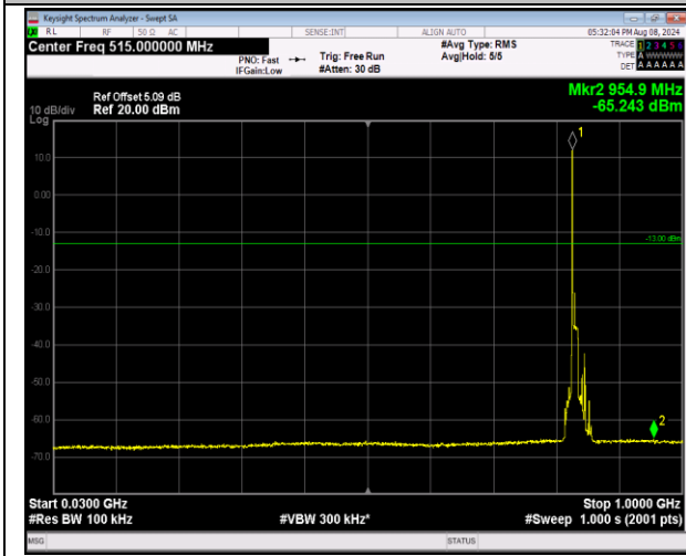
5-5-10MHz-10MHz-16QAM-16QAM-20501-20600-1RB#0-0RB#0-30~1000MHz-PASS
