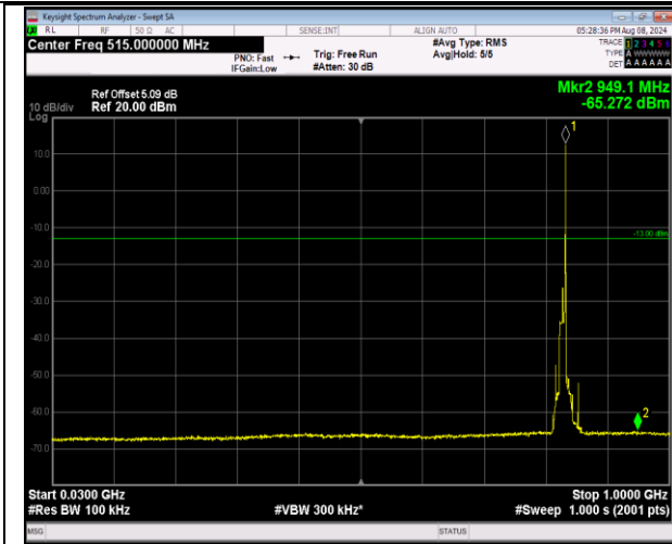
5-5-10MHz-10MHz-16QAM-16QAM-20476-20575-1RB# 49-0RB#0-30~1000MHz-PASS
