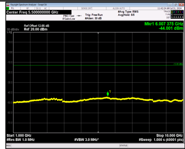
5-5-10MHz-10MHz-64QAM-64QAM-20501-20600-1RB#0 -1RB#49-1000~10000MHz-PASS
