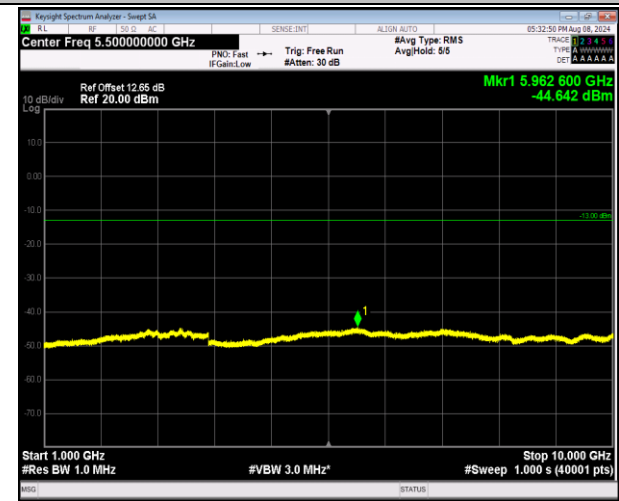
5-5-10MHz-10MHz-QPSK-QPSK-20501-20600-1RB#49-0 RB#0-1000~10000MHz-PASS
