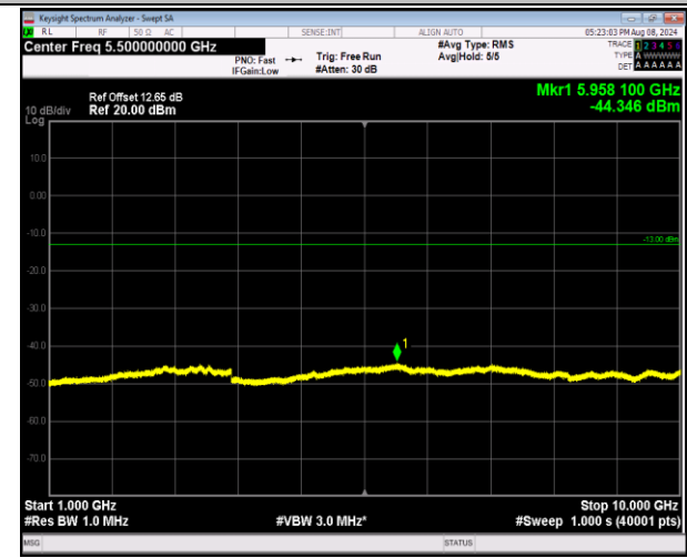
5-5-10MHz-10MHz-16QAM-16QAM-20450-20549-1RB#0-0RB#0-1000~10000MHz-PASS
