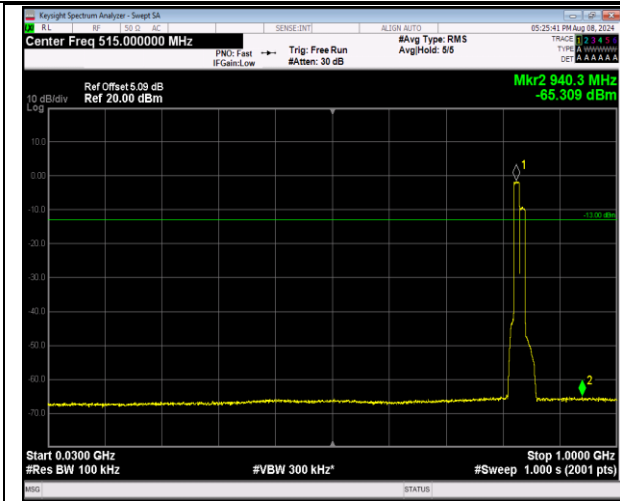
5-5-10MHz-10MHz-QPSK-QPSK-20450-20549-50RB#0-50RB#0-30~1000MHz-PASS
