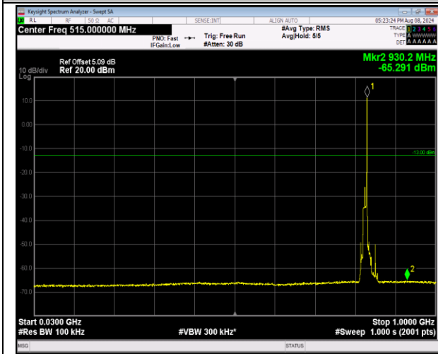
5-5-10MHz-10MHz-QPSK-QPSK-20450-20549-1RB#49-0 ORB#0-30~1000MHz-PASS
