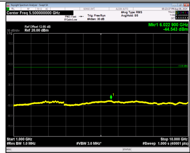
5-5-10MHz-10MHz-QPSK-QPSK-20450-20549-1RB#49-0 RB#0-1000~10000MHz-PASS
