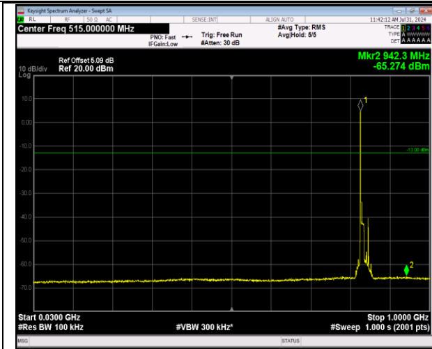
5-5-10MHz-10MHz-64QAM-64QAM-20501-20600-1RB# 0-1RB#49-30~1000MHz-PASS
