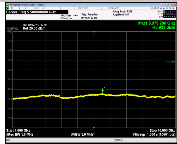
5-5-10MHz-10MHz-64QAM-64QAM-20450-20549-1RB#4-9-0RB#0-1000~10000MHz-PASS
