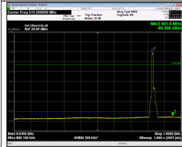
5-5-10MHz-10MHz-64QAM-64QAM-20501-20600-50RB #0-50RB#0-30~1000MHz-PASS
