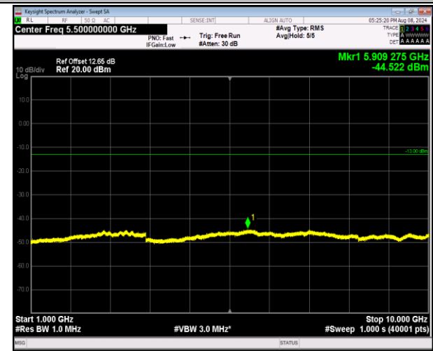
5-5-10MHz-10MHz-16QAM-16QAM-20450-20549-1RB#0-1RB#49-1000~10000MHz-PASS
