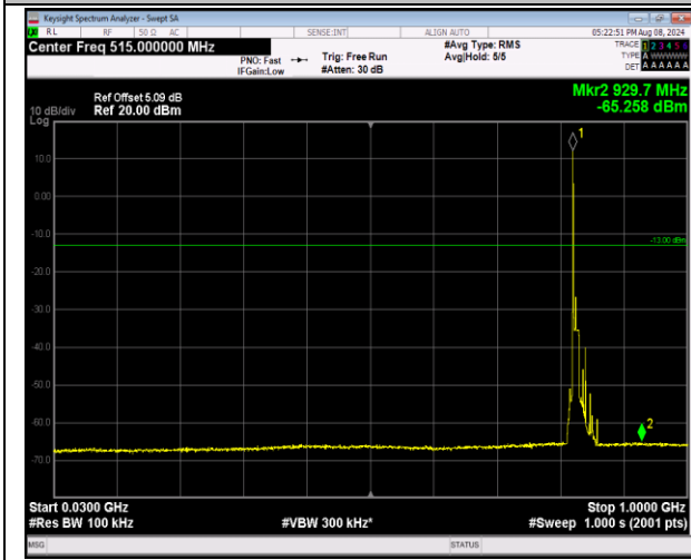
5-5-10MHz-10MHz-16QAM-16QAM-20450-20549-1RB#0-0RB#0-30~1000MHz-PASS
