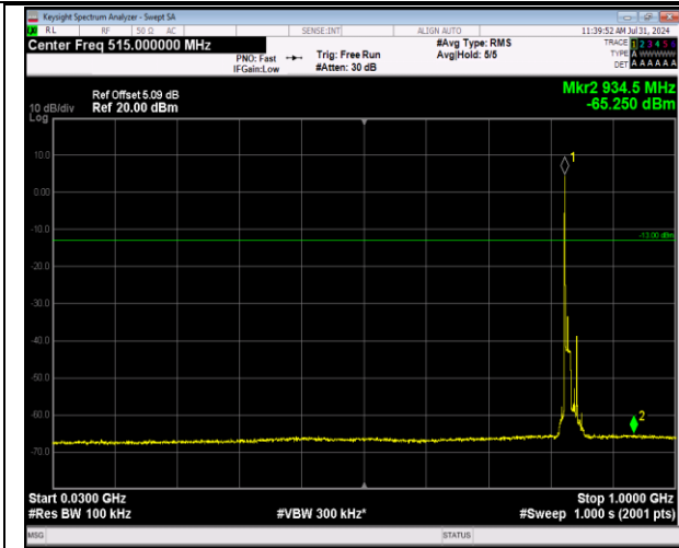
5-5-10MHz-10MHz-64QAM-64QAM-20476-20575-1RB# 0-1RB#49-30~1000MHz-PASS
