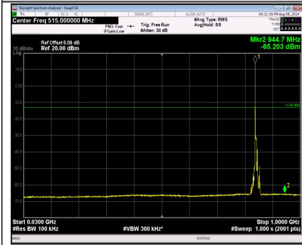
5-5-5MHz-3MHz-16QAM-16QAM-20595-20634-1RB#0-0 RB#0-30~1000MHz-PASS
