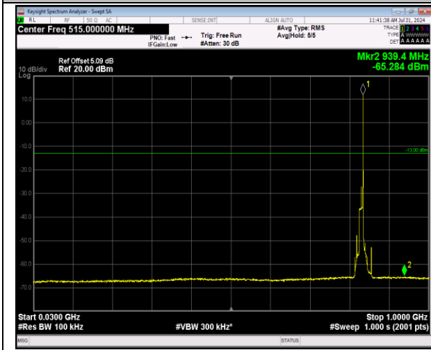
5-5-10MHz-10MHz-64QAM-64QAM-20501-20600-1RB#4 49-0RB#0-30~1000MHz-PASS
