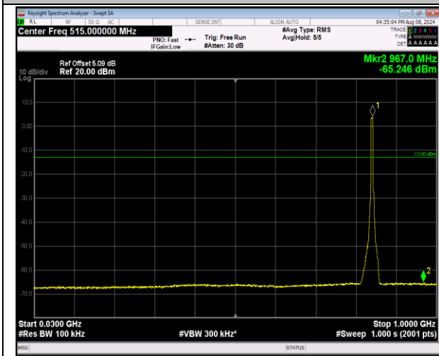
5-5-5MHz-3MHz-16QAM-16QAM-20595-20634-25RB#0-15RB#0-30~1000MHz-PASS
