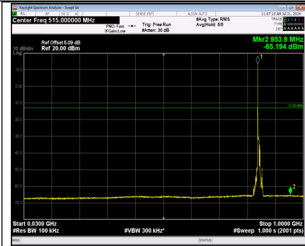
5-5-5MHz-3MHz-64QAM-64QAM-20595-20634-1RB#0-1 RB#15-30~1000MHz-PASS
