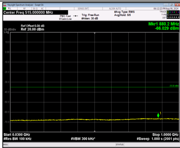
7-7-10MHz-20MHz-QPSK-QPSK-20805-20949-1RB#49-0 ORB#0-30~1000MHz-PASS
