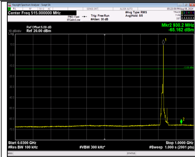
5-5-10MHz-10MHz-16QAM-16QAM-20450-20549-1RB# 49-0RB#0-30~1000MHz-PASS
