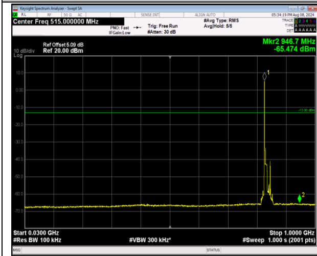
5-5-10MHz-10MHz-16QAM-16QAM-20501-20600-1RB#0-0-1RB#49-30~1000MHz-PASS
