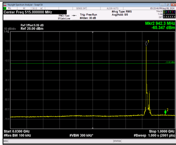
5-5-10MHz-10MHz-QPSK-QPSK-20501-20600-1RB#0-1 RB#49-30~1000MHz-PASS
