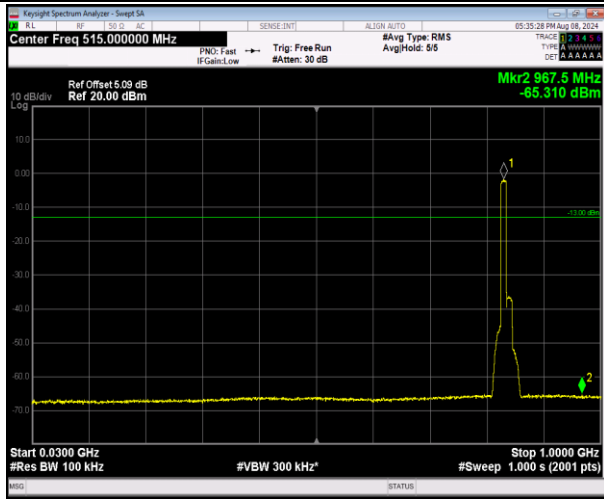
5-5-10MHz-10MHz-16QAM-16QAM-20501-20600-50RB #0-50RB#0-30~1000MHz-PASS
