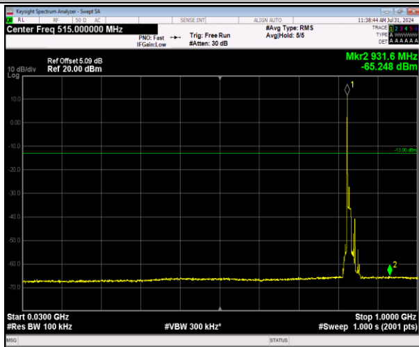
5-5-10MHz-10MHz-64QAM-64QAM-20476-20575-1RB# 0-0RB#0-30~1000MHz-PASS
