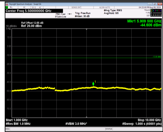
5-5-5MHz-3MHz-16QAM-16QAM-20595-20634-1RB#24-ORB#0-1000~10000MHz-PASS
