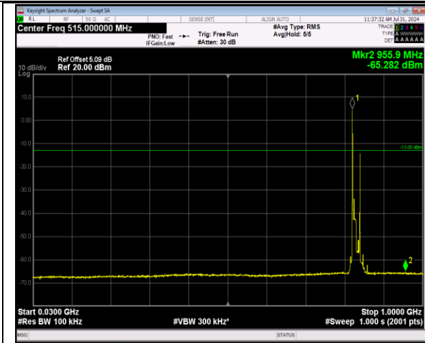
5-5-10MHz-10MHz-64QAM-64QAM-20450-20549-1RB#0-1RB#49-30~1000MHz-PASS
