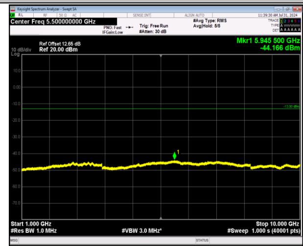
5-5-10MHz-10MHz-64QAM-64QAM-20476-20575-1RB#4 9-0RB#0-1000~10000MHz-PASS
