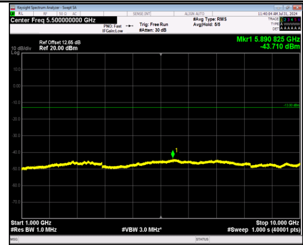
5-5-10MHz-10MHz-64QAM-64QAM-20476-20575-1RB#0 -1RB#49-1000~10000MHz-PASS
