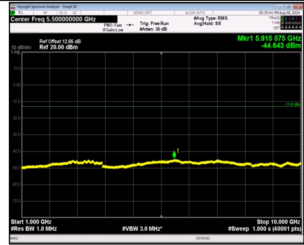
5-5-10MHz-10MHz-16QAM-16QAM-20501-20600-50RB# 0-50RB#0-1000~10000MHz-PASS
