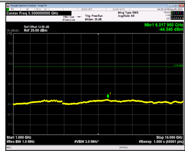
5-5-5MHz-3MHz-16QAM-16QAM-20595-20634-25RB#0-15RB#0-1000~10000MHz-PASS
