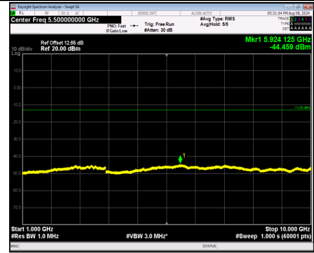
5-5-10MHz-10MHz-16QAM-16QAM-20476-20575-50RB# 0-50RB#0-1000~10000MHz-PASS
