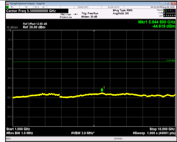
5-5-5MHz-3MHz-QPSK-QPSK-20595-20634-1RB#24-0R B#0-1000~10000MHz-PASS
