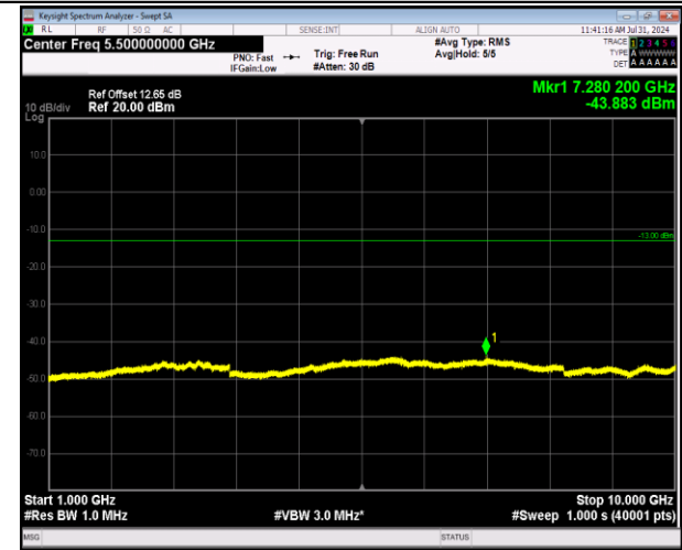
5-5-10MHz-10MHz-64QAM-64QAM-20501-20600-1RB#0 -0RB#0-1000~10000MHz-PASS
