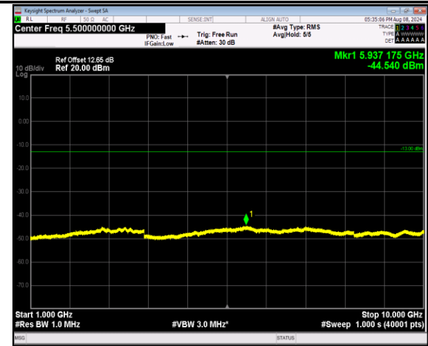
5-5-10MHz-10MHz-QPSK-QPSK-20501-20600-50RB#0-5ORB#0-1000~10000MHz-PASS
