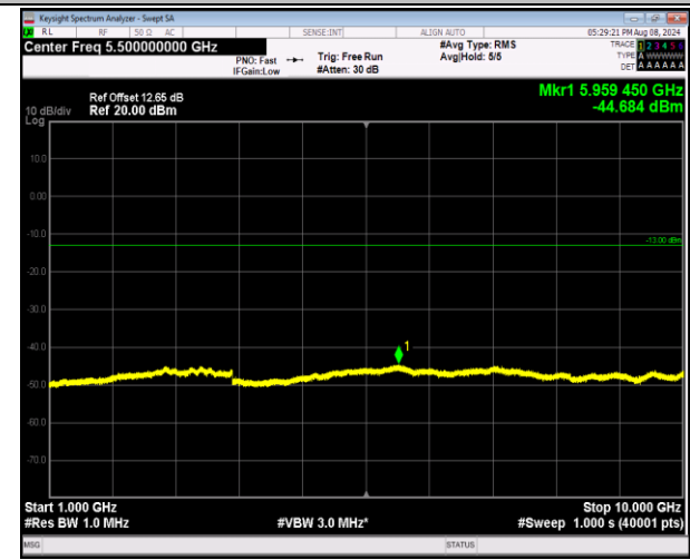
5-5-10MHz-10MHz-QPSK-QPSK-20476-20575-1RB#0-1 RB#49-1000~10000MHz-PASS
