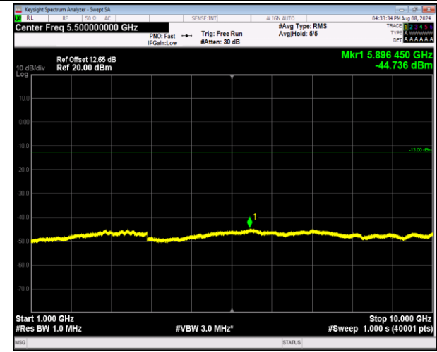
5-5-5MHz-3MHz-QPSK-QPSK-20595-20634-1RB#0-1RB #15-1000~10000MHz-PASS
