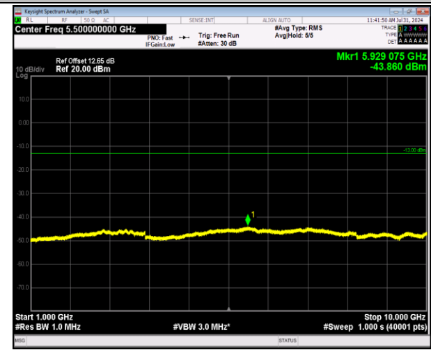
5-5-10MHz-10MHz-64QAM-64QAM-20501-20600-1RB#4 9-0RB#0-1000~10000MHz-PASS
