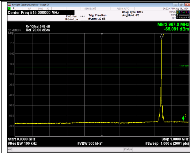
5-5-5MHz-3MHz-16QAM-16QAM-20595-20634-1RB#24-ORB#0-30~1000MHz-PASS
