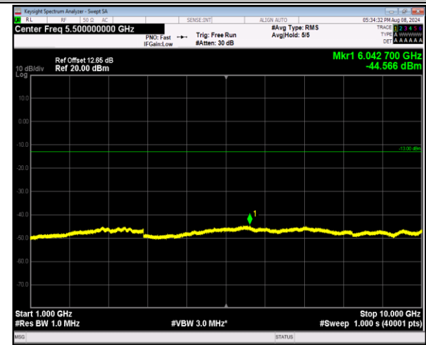
5-5-10MHz-10MHz-16QAM-16QAM-20501-20600-1RB#0-1RB#49-1000~10000MHz-PASS
