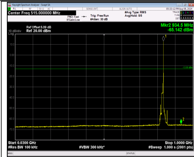
5-5-10MHz-10MHz-16QAM-16QAM-20501-20600-1RB# 49-0RB#0-30~1000MHz-PASS
