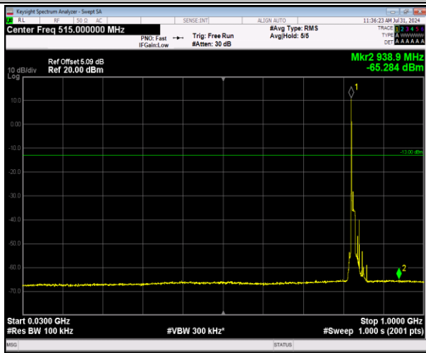
5-5-10MHz-10MHz-64QAM-64QAM-20450-20549-1RB# 0-0RB#0-30~1000MHz-PASS
