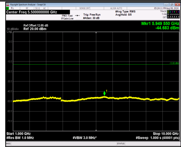
5-5-10MHz-10MHz-16QAM-16QAM-20450-20549-1RB#4 9-0RB#0-1000~10000MHz-PASS
