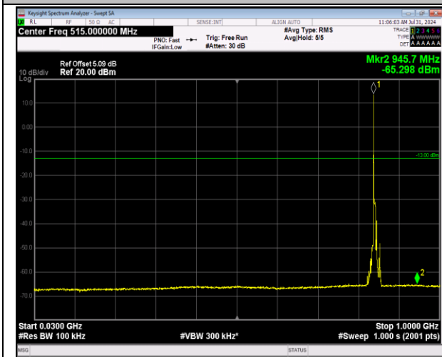
5-5-5MHz-3MHz-64QAM-64QAM-20595-20634-1RB#0-0RB#0-30~1000MHz-PASS
