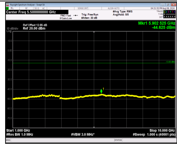
5-5-5MHz-3MHz-16QAM-16QAM-20595-20634-1RB#0-0 RB#0-1000~10000MHz-PASS
