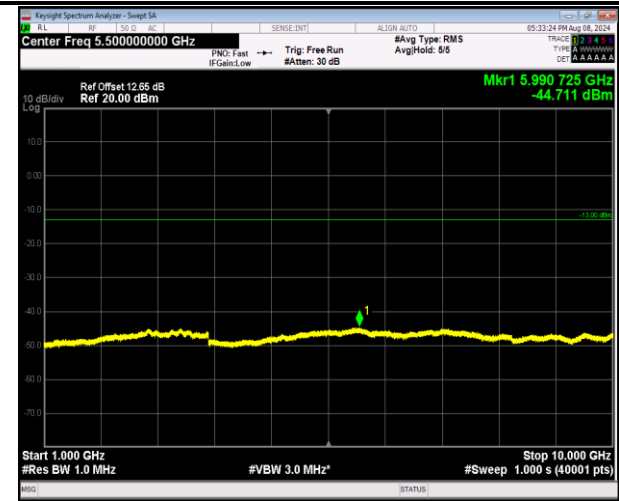
5-5-10MHz-10MHz-16QAM-16QAM-20501-20600-1RB#4 9-0RB#0-1000~10000MHz-PASS
