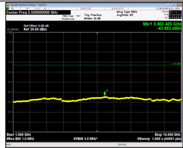
5-5-10MHz-10MHz-64QAM-64QAM-20450-20549-50RB#0-50RB#0-1000~10000MHz-PASS
