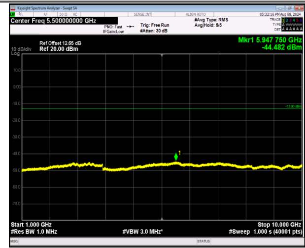
5-5-10MHz-10MHz-16QAM-16QAM-20501-20600-1RB#0-0RB#0-1000~10000MHz-PASS
