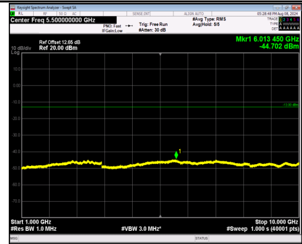
5-5-10MHz-10MHz-16QAM-16QAM-20476-20575-1RB#4 9-0RB#0-1000~10000MHz-PASS
