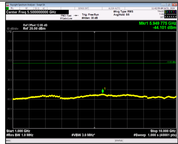
5-5-10MHz-10MHz-64QAM-64QAM-20501-20600-50RB# 0-50RB#0-1000~10000MHz-PASS
