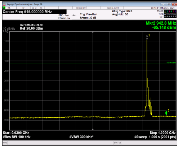
5-5-10MHz-10MHz-64QAM-64QAM-20501-20600-1RB# 0-0RB#0-30~1000MHz-PASS
