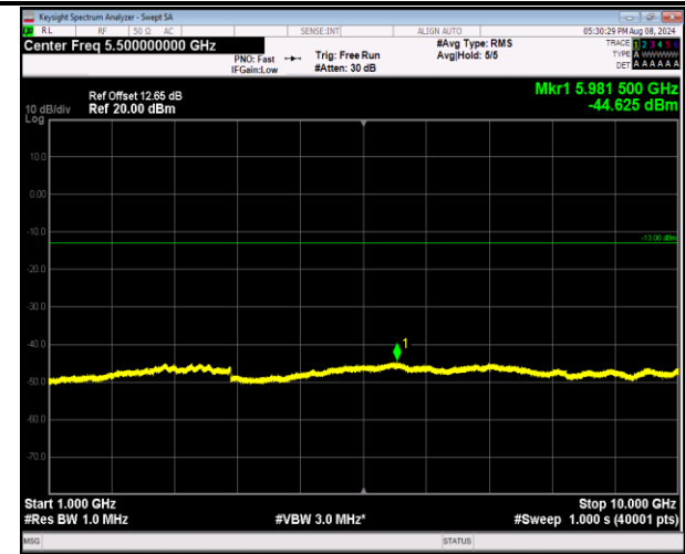
5-5-10MHz-10MHz-QPSK-QPSK-20476-20575-50RB#0-5ORB#0-1000~10000MHz-PASS
