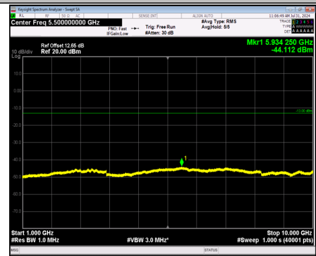
5-5-5MHz-3MHz-64QAM-64QAM-20595-20634-1RB#24- ORB#0-1000~10000MHz-PASS
