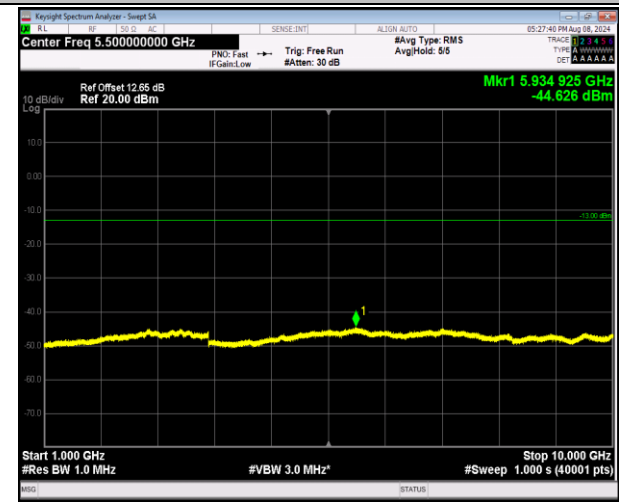
5-5-10MHz-10MHz-16QAM-16QAM-20476-20575-1RB#0-0RB#0-1000~10000MHz-PASS
