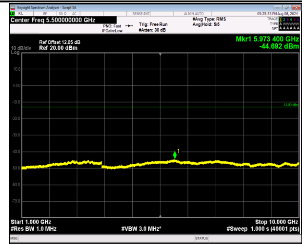
5-5-10MHz-10MHz-QPSK-QPSK-20450-20549-50RB#0-50RB#0-1000~10000MHz-PASS
