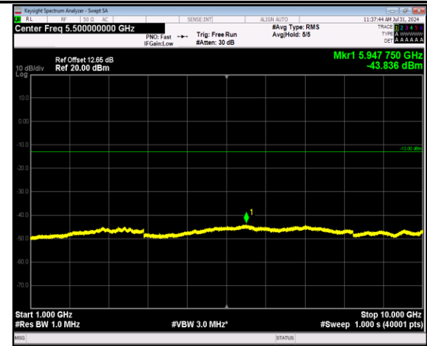
5-5-10MHz-10MHz-64QAM-64QAM-20450-20549-1RB#0-1RB#49-1000~10000MHz-PASS
