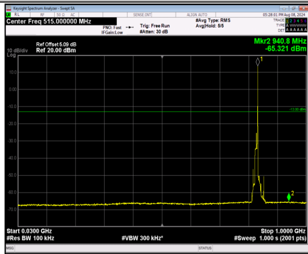
5-5-10MHz-10MHz-QPSK-QPSK-20476-20575-1RB#49-0 ORB#0-30~1000MHz-PASS
