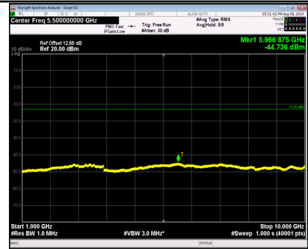
5-5-10MHz-10MHz-QPSK-QPSK-20501-20600-1RB#0-0 RB#0-1000~10000MHz-PASS
