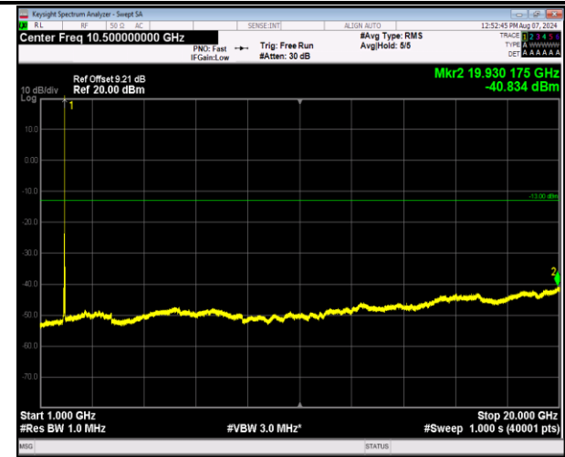
2-2-5MHz-20MHz-16QAM-16QAM-18983-19100-1RB#24 -0RB#0-1000~20000MHz-PASS
