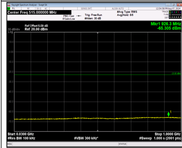
2-2-5MHz-20MHz-16QAM-16QAM-18983-19100-25RB# 0-100RB#0-30~1000MHz-PASS
