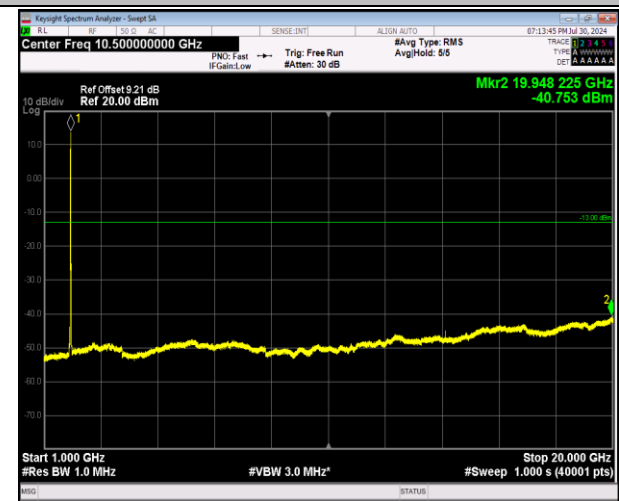
2-2-5MHz-20MHz-64QAM-64QAM-18983-19100-25RB#0-100RB#0-1000~20000MHz-PASS
