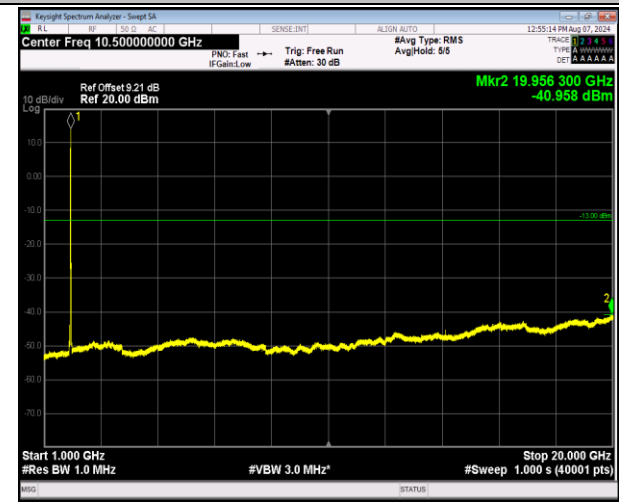
2-2-5MHz-20MHz-16QAM-16QAM-18983-19100-25RB#0 -100RB#0-1000~20000MHz-PASS
