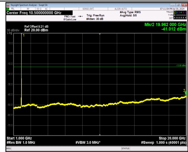
2-2-5MHz-20MHz-64QAM-64QAM-18983-19100-1RB#0- 0RB#0-1000~20000MHz-PASS
