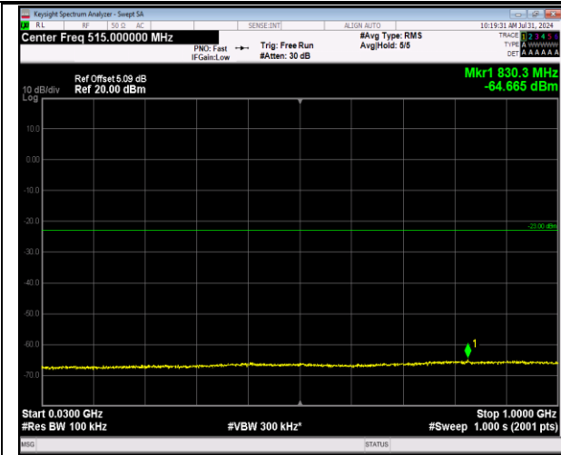
2-2-20MHz-20MHz-64QAM-64QAM-18902-19100-1RB#0-1RB#99-30~1000MHz-PASS
