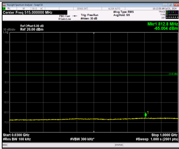
2-2-20MHz-20MHz-64QAM-64QAM-18700-18898-1RB#99-0RB#0-30~1000MHz-PASS
