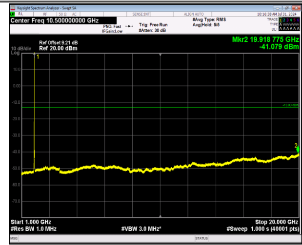
2-2-20MHz-20MHz-64QAM-64QAM-18801-18999-1RB#9 9-0RB#0-1000~20000MHz-PASS
