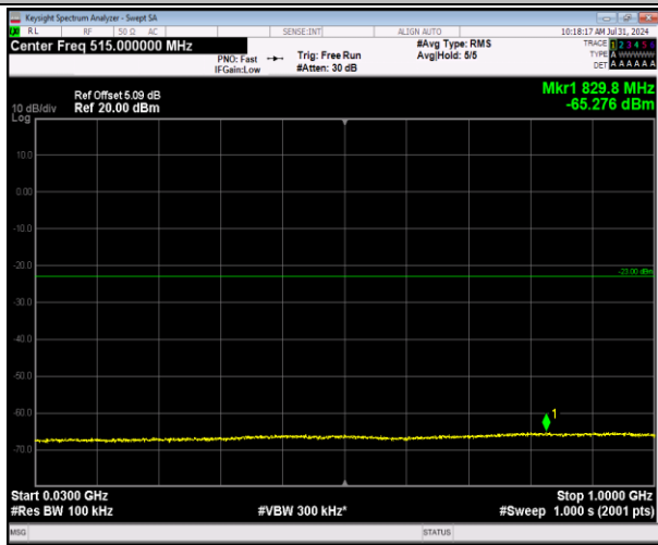
2-2-20MHz-20MHz-64QAM-64QAM-18902-19100-1RB# 0-0RB#0-30~1000MHz-PASS
