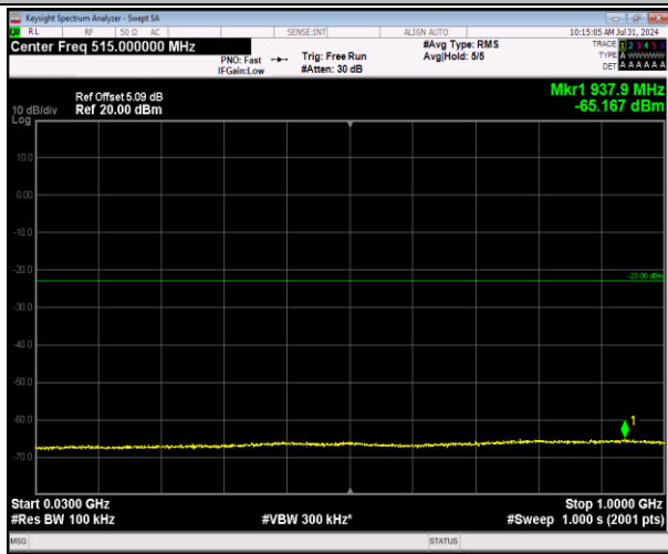
2-2-20MHz-20MHz-64QAM-64QAM-18700-18898-100RB#0-100RB#0-30~1000MHz-PASS
