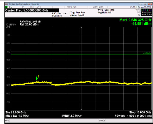
5-5-3MHz-5MHz-QPSK-QPSK-20416-20455-1RB#0-1RB #24-1000~10000MHz-PASS
