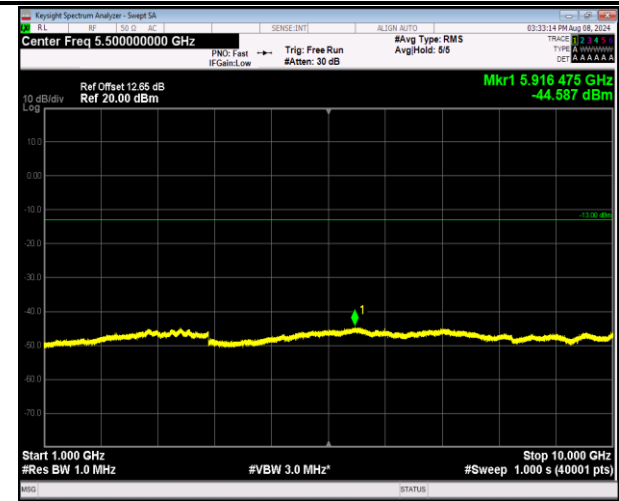
5-5-3MHz-5MHz-16QAM-16QAM-20416-20455-1RB#14-ORB#0-1000~10000MHz-PASS
