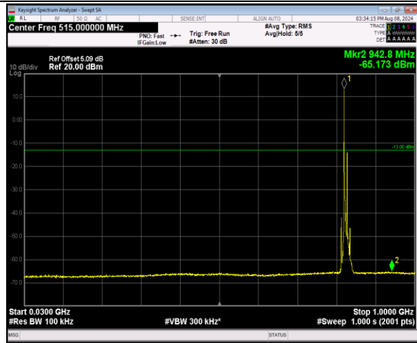
5-5-3MHz-5MHz-16QAM-16QAM-20416-20455-1RB#0-1 RB#24-30~1000MHz-PASS
