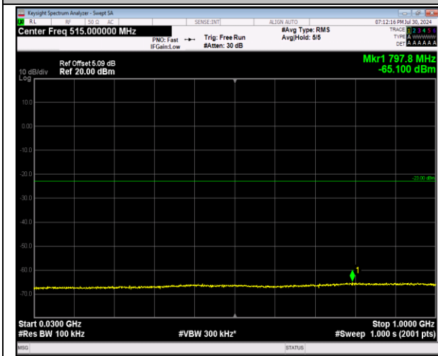
2-2-5MHz-20MHz-64QAM-64QAM-18983-19100-1RB#2-4-0RB#0-30~1000MHz-PASS
