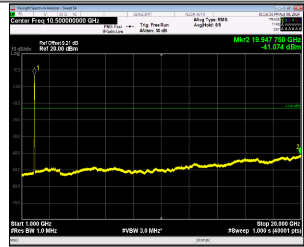
2-2-20MHz-20MHz-16QAM-16QAM-18700-18898-100RB #0-100RB#0-1000~20000MHz-PASS
