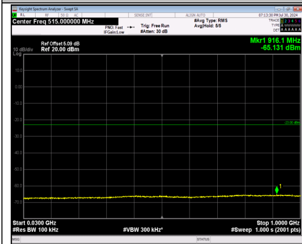
2-2-5MHz-20MHz-64QAM-64QAM-18983-19100-25RB#0-100RB#0-30~1000MHz-PASS
