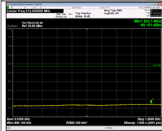
2-2-5MHz-20MHz-64QAM-64QAM-18983-19100-1RB#0- 0RB#0-30~1000MHz-PASS
