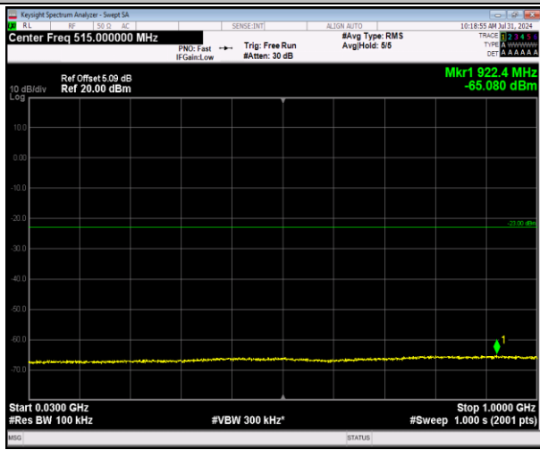
2-2-20MHz-20MHz-64QAM-64QAM-18902-19100-1RB#99-0RB#0-30~1000MHz-PASS
