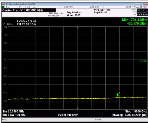
2-2-20MHz-20MHz-16QAM-16QAM-18902-19100-100R B#0-100RB#0-30~1000MHz-PASS
