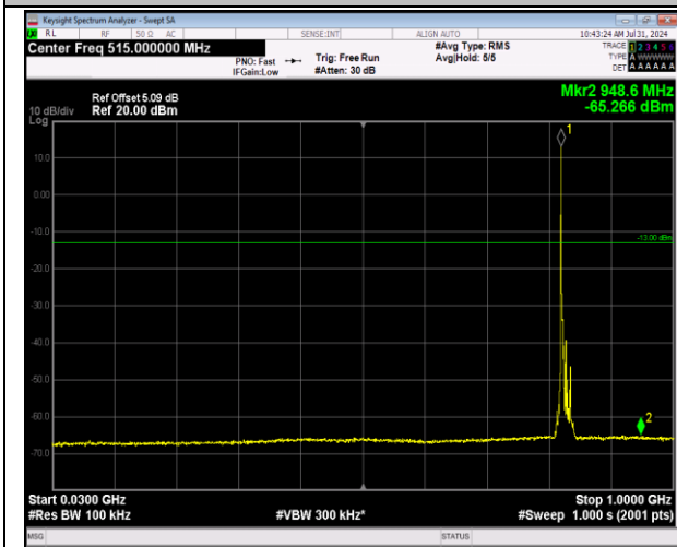
5-5-3MHz-5MHz-64QAM-64QAM-20416-20455-1RB#0-0RB#0-30~1000MHz-PASS
