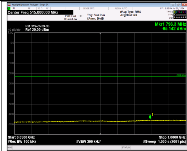
2-2-5MHz-20MHz-64QAM-64QAM-18983-19100-1RB#0-1RB#99-30~1000MHz-PASS
