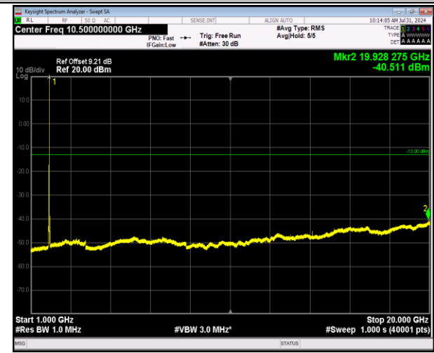
2-2-20MHz-20MHz-64QAM-64QAM-18700-18898-1RB#9-0RB#0-1000~20000MHz-PASS
