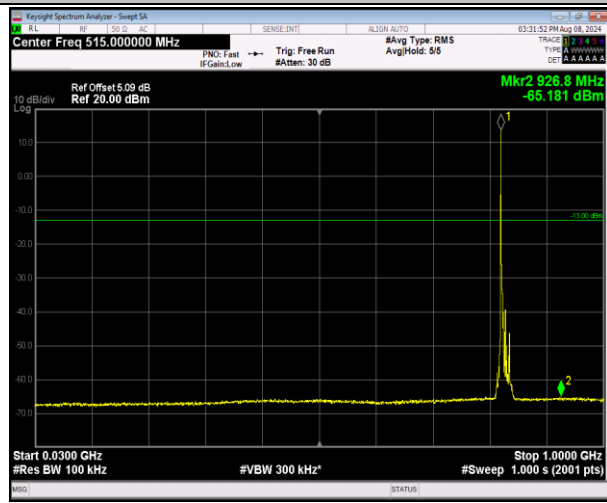
5-5-3MHz-5MHz-16QAM-16QAM-20416-20455-1RB#0-0 RB#0-30~1000MHz-PASS
