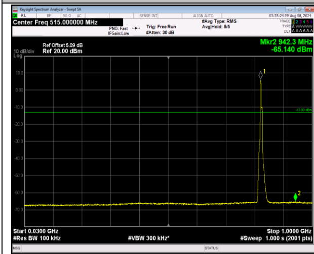
5-5-3MHz-5MHz-16QAM-16QAM-20416-20455-15RB#0-25RB#0-30~1000MHz-PASS
