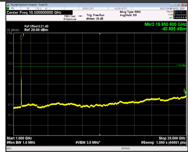
2-2-20MHz-20MHz-64QAM-64QAM-18801-18999-1RB#0 -1RB#99-1000~20000MHz-PASS
