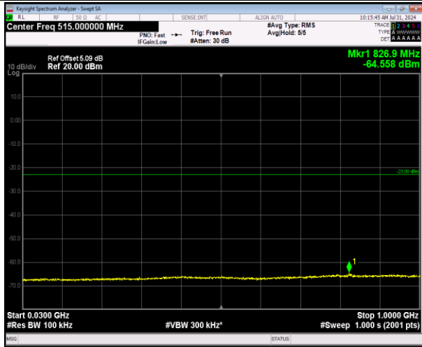
2-2-20MHz-20MHz-64QAM-64QAM-18801-18999-1RB#0-0RB#0-30~1000MHz-PASS
