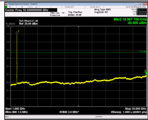
2-2-20MHz-20MHz-16QAM-16QAM-18902-19100-100RB #0-100RB#0-1000~20000MHz-PASS
