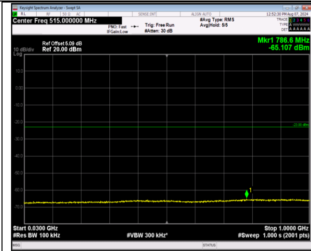
2-2-5MHz-20MHz-16QAM-16QAM-18983-19100-1RB#2 4-0RB#0-30~1000MHz-PASS
