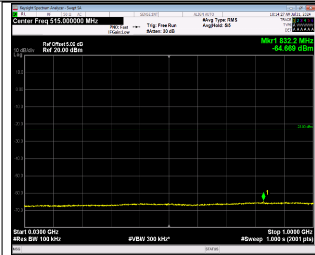
2-2-20MHz-20MHz-64QAM-64QAM-18700-18898-1RB#0-1RB#99-30~1000MHz-PASS
