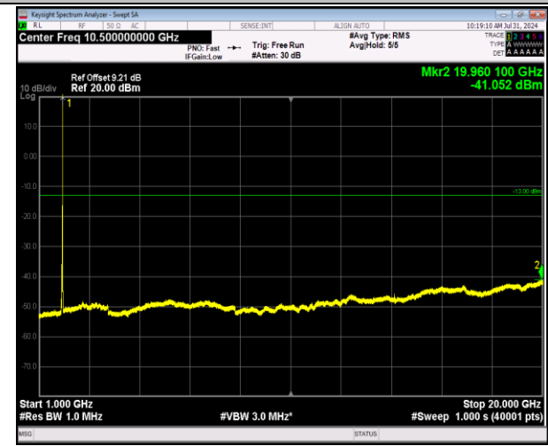
2-2-20MHz-20MHz-64QAM-64QAM-18902-19100-1RB#9-0RB#0-1000~20000MHz-PASS
