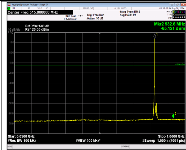
5-5-3MHz-5MHz-16QAM-16QAM-20416-20455-1RB#14-ORB#0-30~1000MHz-PASS
