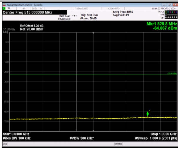
2-2-20MHz-20MHz-64QAM-64QAM-18801-18999-1RB#99-0RB#0-30~1000MHz-PASS
