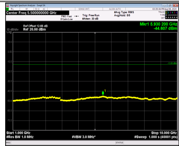
5-5-3MHz-5MHz-16QAM-16QAM-20416-20455-15RB#0-25RB#0-1000~10000MHz-PASS
