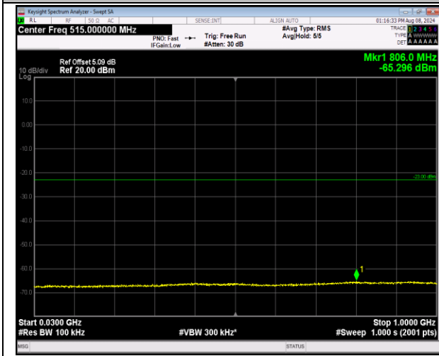
2-2-20MHz-20MHz-16QAM-16QAM-18700-18898-100R B#0-100RB#0-30~1000MHz-PASS
