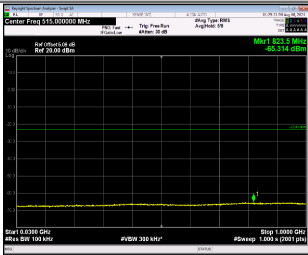
2-2-20MHz-20MHz-16QAM-16QAM-18902-19100-1RB# 0-1RB#99-30~1000MHz-PASS
