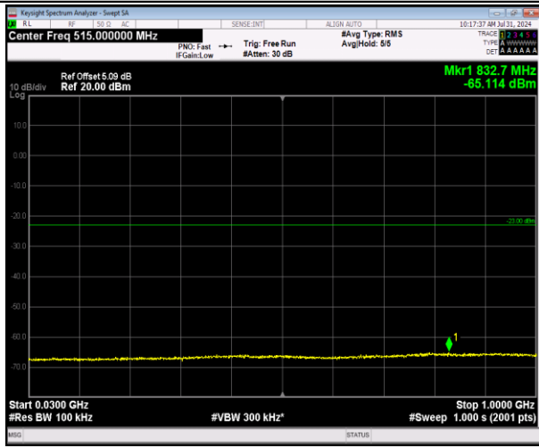
2-2-20MHz-20MHz-64QAM-64QAM-18801-18999-100R B#0-100RB#0-30~1000MHz-PASS
