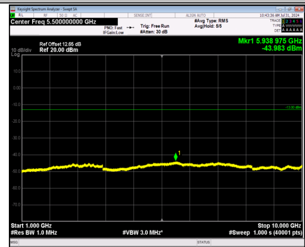
5-5-3MHz-5MHz-64QAM-64QAM-20416-20455-1RB#0-0RB#0-1000~10000MHz-PASS
