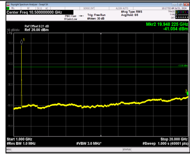
2-2-20MHz-20MHz-64QAM-64QAM-18801-18999-100RB #0-100RB#0-1000~20000MHz-PASS
