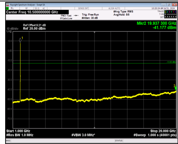
2-2-20MHz-20MHz-64QAM-64QAM-18902-19100-100RB#0-100RB#0-1000~20000MHz-PASS
