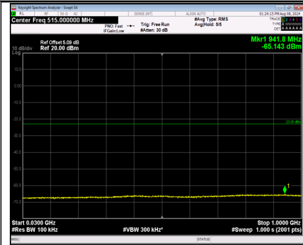
2-2-20MHz-20MHz-16QAM-16QAM-18902-19100-1RB# 99-0RB#0-30~1000MHz-PASS
