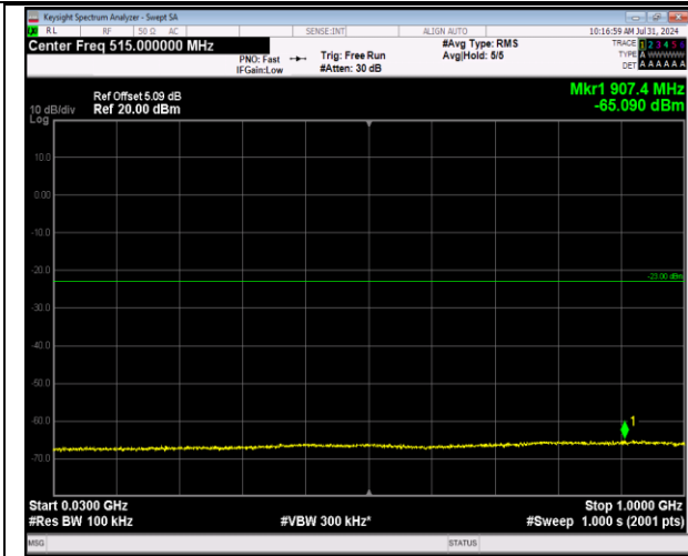
2-2-20MHz-20MHz-64QAM-64QAM-18801-18999-1RB# 0-1RB#99-30~1000MHz-PASS
