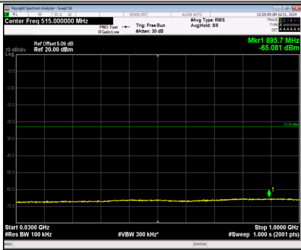
2-2-20MHz-20MHz-64QAM-64QAM-18902-19100-100RB#0-100RB#0-30~1000MHz-PASS
