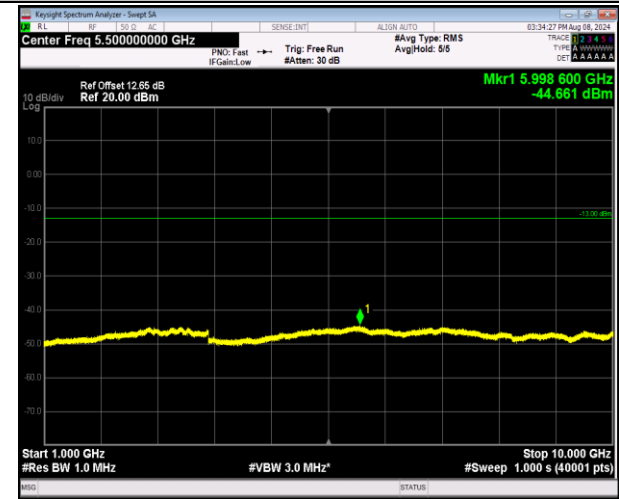
5-5-3MHz-5MHz-16QAM-16QAM-20416-20455-1RB#0-1 RB#24-1000~10000MHz-PASS
