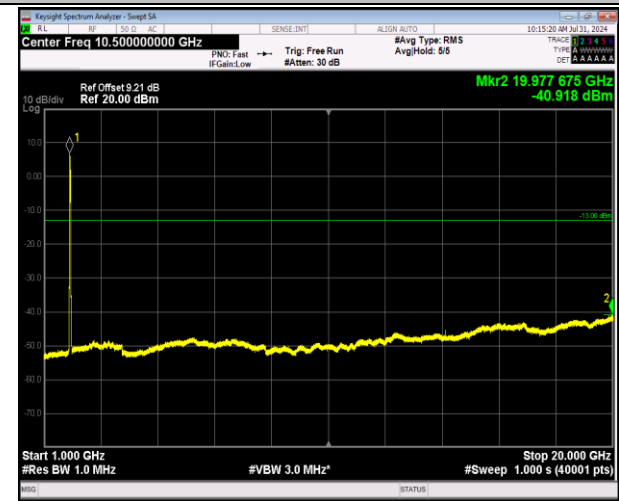
2-2-20MHz-20MHz-64QAM-64QAM-18700-18898-100RB#0-100RB#0-1000~20000MHz-PASS
