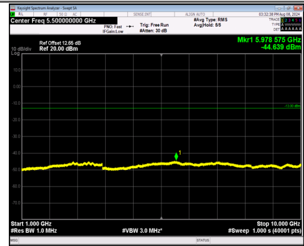
5-5-3MHz-5MHz-QPSK-QPSK-20416-20455-1RB#14-0R B#0-1000~10000MHz-PASS
