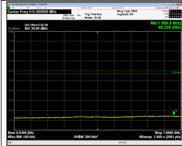
2-2-20MHz-20MHz-64QAM-64QAM-18700-18898-1RB# 0-0RB#0-30~1000MHz-PASS
