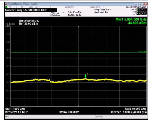
5-5-3MHz-5MHz-16QAM-16QAM-20416-20455-1RB#0-0 RB#0-1000~10000MHz-PASS
