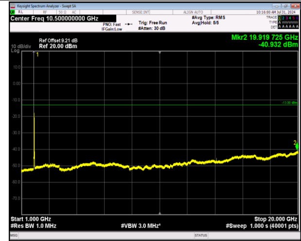
2-2-20MHz-20MHz-64QAM-64QAM-18801-18999-1RB#0-0RB#0-1000~20000MHz-PASS
