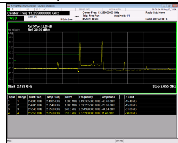
41-41-5MHz-20MHz-QPSK@QPSK-QPSK@QPSK-4027 3-40390-1RB#0@25RB#0-1RB#99@100RB#0-PASS
