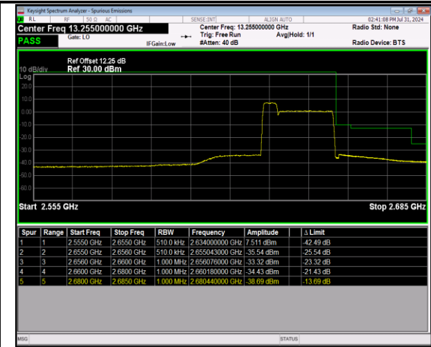
41-41-5MHz-20MHz-64QAM@64QAM-64QAM@64QAM-41023-41140-25RB#0 @25RB#0-100RB#0 @100RB#0-PA SS
