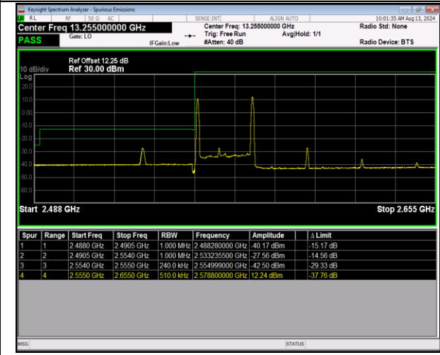
41-41-20MHz-5MHz-QPSK@QPSK-QPSK@QPSK-4034 0-40475-1RB#0 @100RB#0-1RB#24 @25RB#0-PASS
