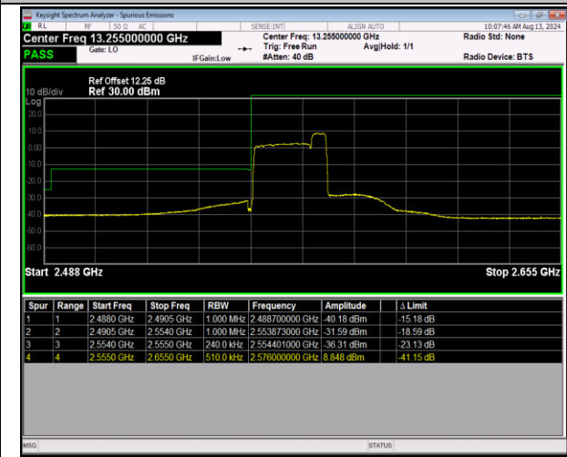
41-41-20MHz-5MHz-QPSK@QPSK-QPSK@QPSK-4034 0-40475-100RB#0 @100RB#0-25RB#0 @25RB#0-PASS
