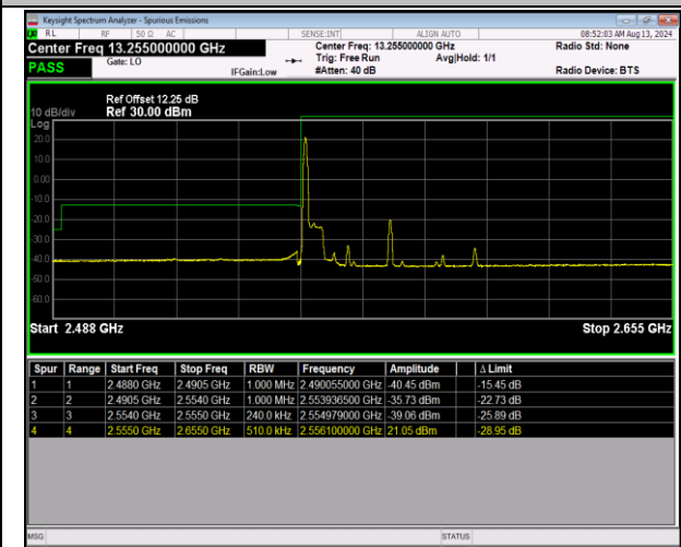
41-41-5MHz-20MHz-16QAM@16QAM-16QAM@16QAM-40273-40390-1RB#0@25RB#0-0RB#0@100RB#0-PASS
