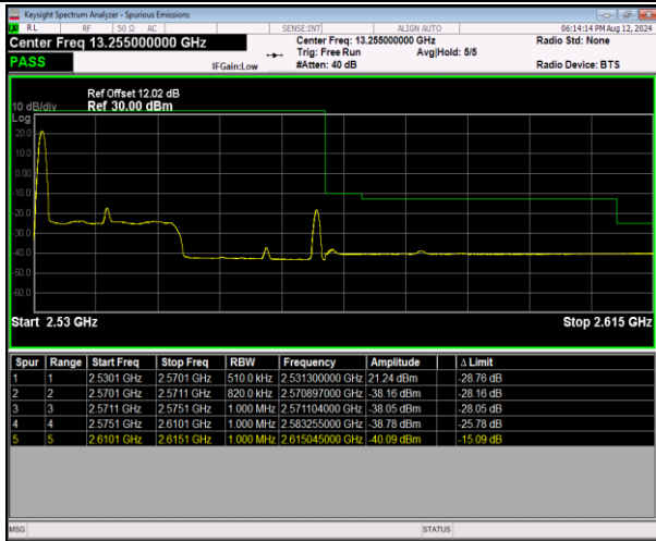
7-7-20MHz-20MHz-16QAM@16QAM-16QAM@16QAM-21152-21350-1RB#0@100RB#0-0RB#0@100RB#0-PASS
