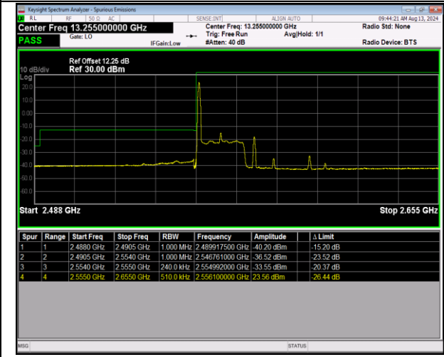
41-41-20MHz-5MHz-QPSK@QPSK-QPSK@QPSK-4034 0-40475-1RB#0 @100RB#0-0RB#0 @25RB#0-PASS
