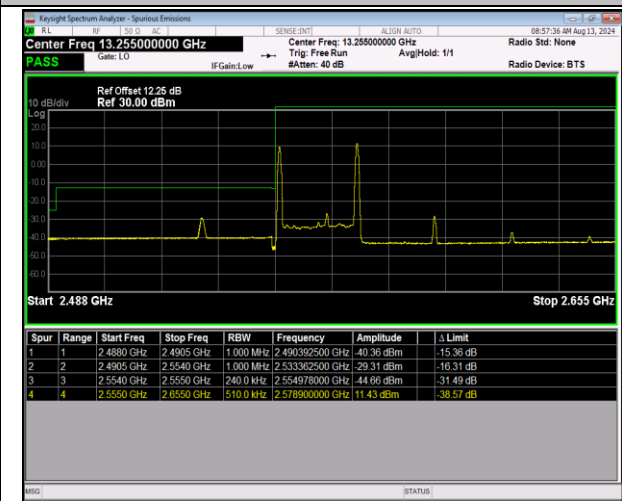
41-41-5MHz-20MHz-16QAM@16QAM-16QAM@16QAM-40273-40390-1RB#0@25RB#0-1RB#99@100RB#0-PASS
