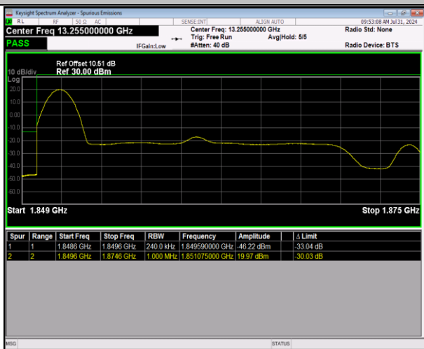
2-2-20MHz-5MHz-64QAM@64QAM-64QAM@64QAM-18 700-18817-1RB#0@100RB#0-0RB#0@25RB#0-PASS
