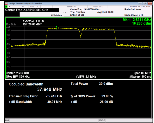
41-41-20MHz-20MHz-64QAM-64QAM-40942-41140-100RB RB#0-100RB#0-PASS
