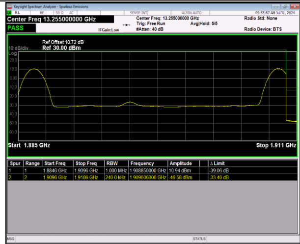
2-2-20MHz-5MHz-64QAM@64QAM-64QAM@64QAM-19 050-19167-1RB#0@100RB#0-1RB#24@25RB#0-PASS
