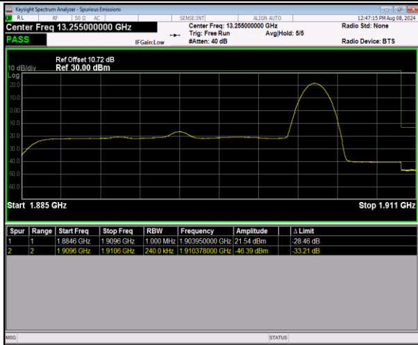
2-2-20MHz-5MHz-16QAM@16QAM-16QAM@16QAM-19 050-19167-1RB#99@100RB#0-0RB#0@25RB#0-PASS
