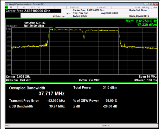
41-41-20MHz-20MHz-QPSK-QPSK-40942-41140-100RB B#0-100RB#0-PASS
