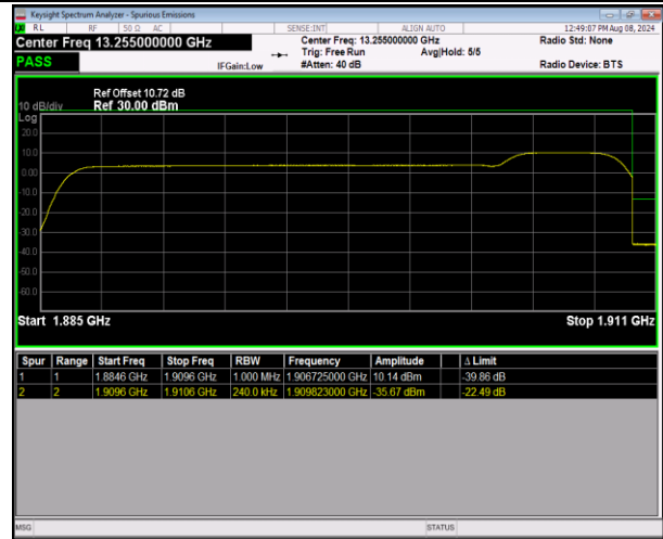
2-2-20MHz-5MHz-16QAM@16QAM-16QAM@16QAM-19 050-19167-100RB#0@100RB#0-25RB#0@25RB#0-PASS S
