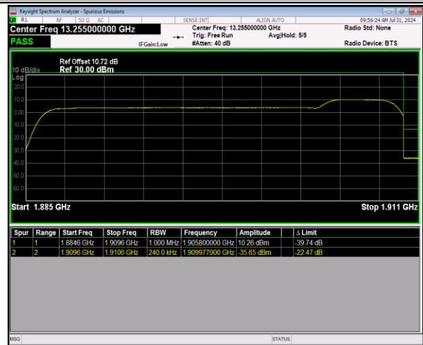
2-2-20MHz-5MHz-64QAM@64QAM-64QAM@64QAM-19
