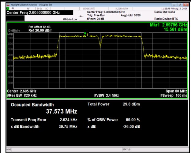
41-41-20MHz-20MHz-16QAM-16QAM-40641-40839-100RB RB#0-100RB#0-PASS
