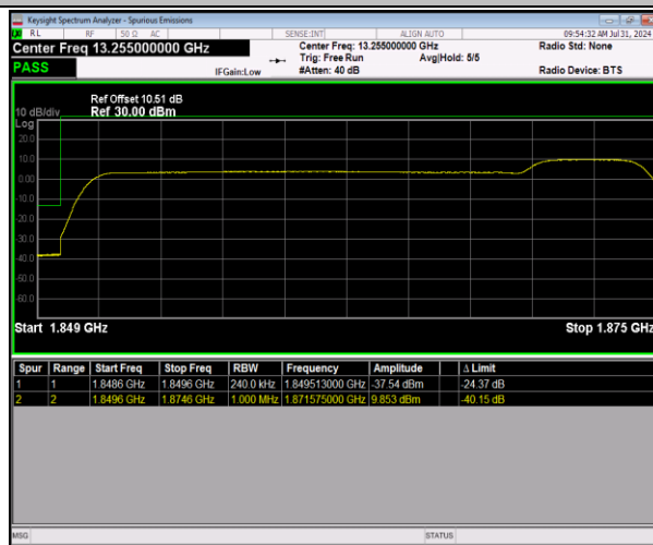
2-2-20MHz-5MHz-64QAM@64QAM-64QAM@64QAM-18
