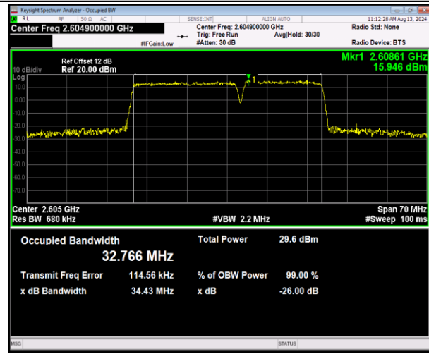
41-41-20MHz-15MHz-16QAM-16QAM-40666-40837-100RB#0-75RB#0-PASS
