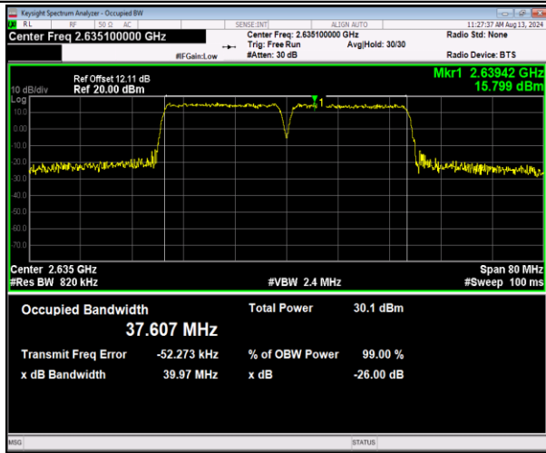
41-41-20MHz-20MHz-16QAM-16QAM-40942-41140-100RB RB#0-100RB#0-PASS
