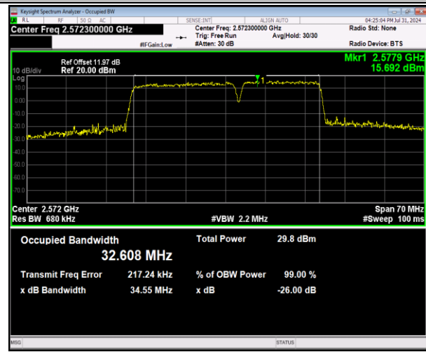
41-41-20MHz-15MHz-64QAM-64QAM-40340-40511-100RB#0-75RB#0-PASS
