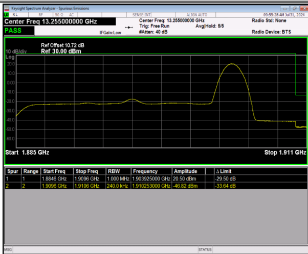
2-2-20MHz-5MHz-64QAM@64QAM-64QAM@64QAM-19
