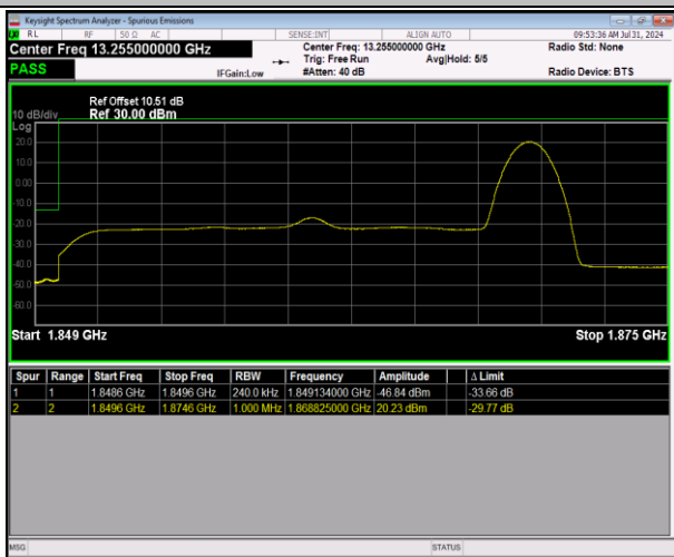
2-2-20MHz-5MHz-64QAM@64QAM-64QAM@64QAM-18
