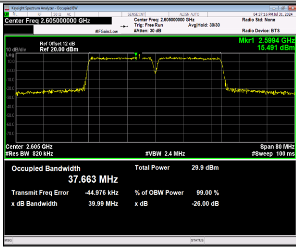
41-41-20MHz-20MHz-64QAM-64QAM-40641-40839-100RB RB#0-100RB#0-PASS
