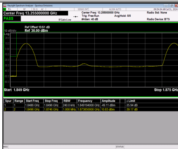
2-2-20MHz-5MHz-64QAM@64QAM-64QAM@64QAM-18 700-18817-1RB#0@100RB#0-1RB#24@25RB#0-PASS
