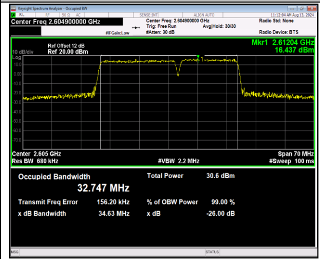
41-41-20MHz-15MHz-QPSK-QPSK-40666-40837-100RB#0-75RB#0-PASS
