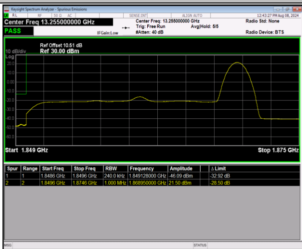
2-2-20MHz-5MHz-16QAM@16QAM-16QAM@16QAM-18 700-18817-1RB#99@100RB#0-0RB#0@25RB#0-PASS
