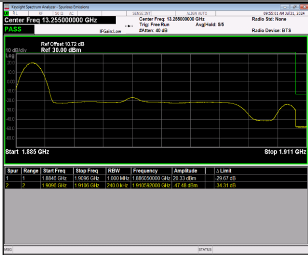
2-2-20MHz-5MHz-64QAM@64QAM-64QAM@64QAM-19 050-19167-1RB#0@100RB#0-0RB#0@25RB#0-PASS
