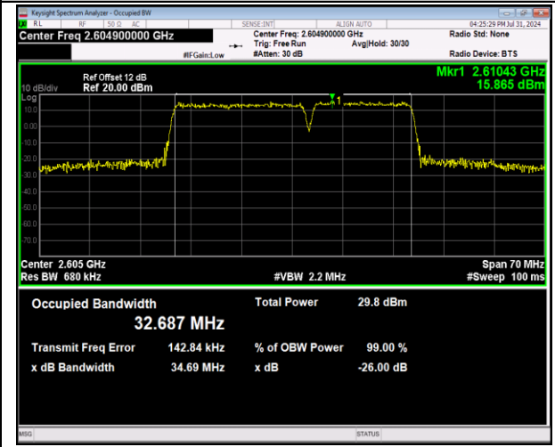
41-41-20MHz-15MHz-64QAM-64QAM-40666-40837-100RB#0-75RB#0-PASS
