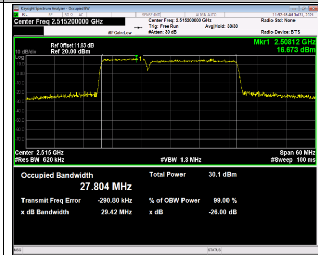
7-7-10MHz-20MHz-64QAM-64QAM-20805-20949-50RB #0-100RB#0-PASS
