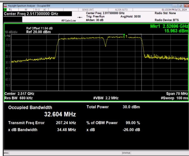
7-7-20MHz-15MHz-64QAM-64QAM-20850-21021-100RB#0-75RB#0-PASS
