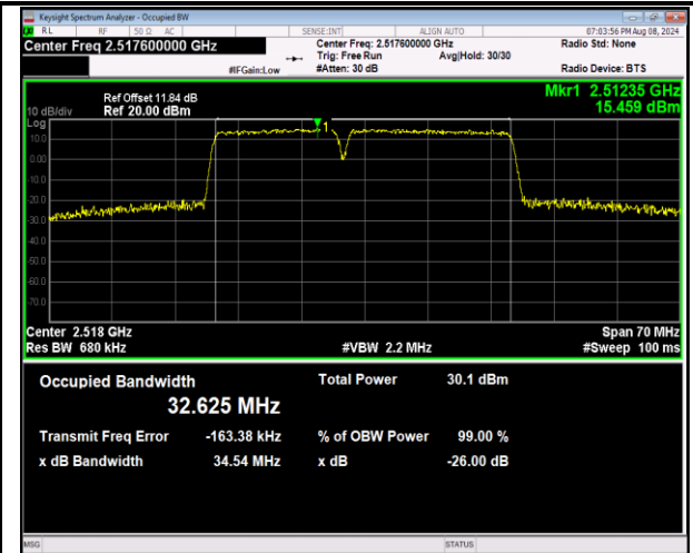
7-7-15MHz-20MHz-16QAM-16QAM-20828-20999-75RB#0-100RB#0-PASS
