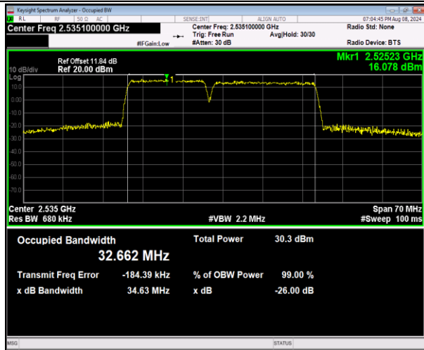
7-7-15MHz-20MHz-16QAM-16QAM-21003-21174-75RB#0-100RB#0-PASS
