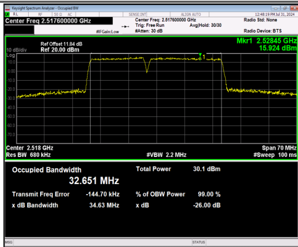
7-7-15MHz-20MHz-64QAM-64QAM-20828-20999-75RB#0-100RB#0-PASS
