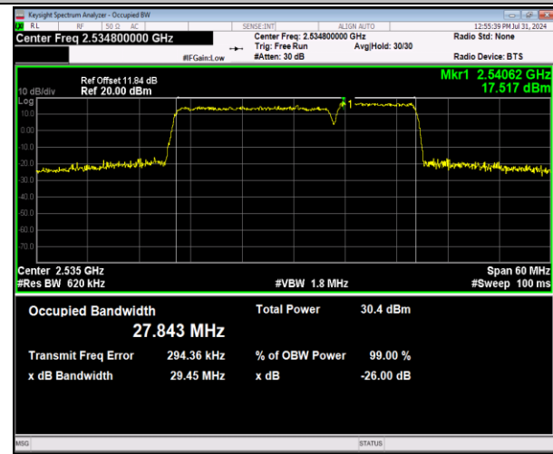
7-7-20MHz-10MHz-64QAM-64QAM-21051-21195-100RB#0-50RB#0-PASS
