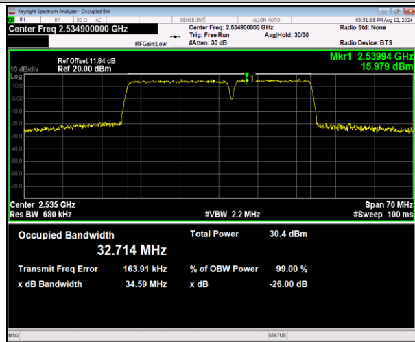
7-7-20MHz-15MHz-16QAM-16QAM-21026-21197-100RB#0-75RB#0-PASS
