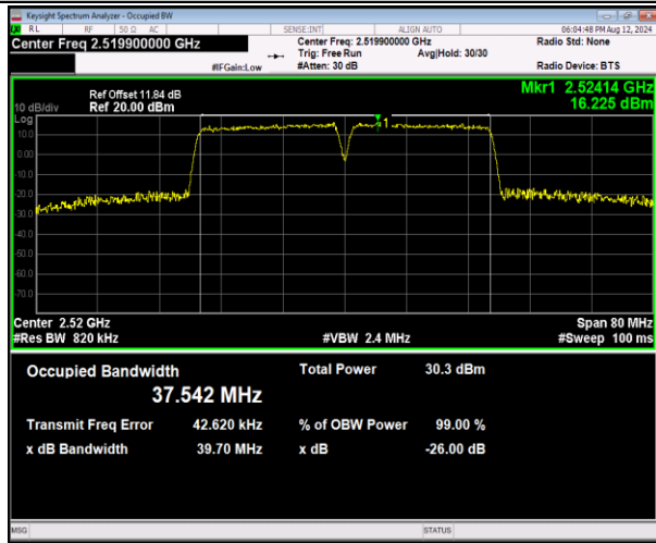
7-7-20MHz-20MHz-16QAM-16QAM-20850-21048-100RB#0-100RB#0-PASS
