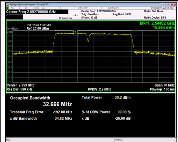
7-7-15MHz-20MHz-16QAM-16QAM-21179-21350-75RB#0-100RB#0-PASS
