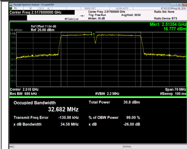
7-7-15MHz-20MHz-QPSK-QPSK-20828-20999-75RB#0-1 00RB#0-PASS
