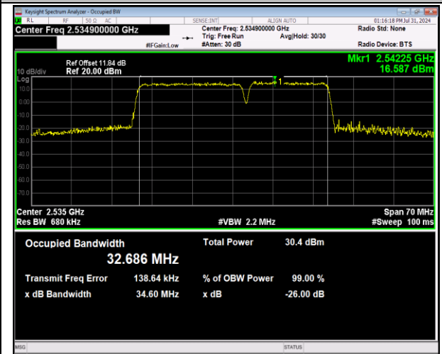
7-7-20MHz-15MHz-64QAM-64QAM-21026-21197-100RB#0-75RB#0-PASS
