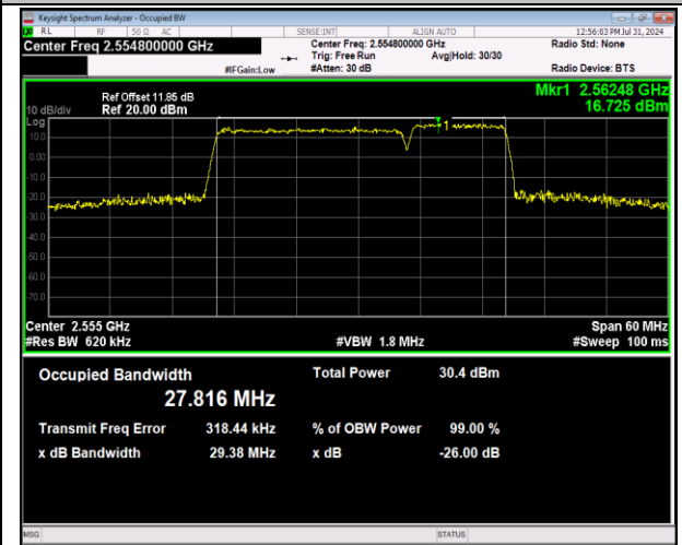
7-7-20MHz-10MHz-64QAM-64QAM-21251-21395-100RB#0-50RB#0-PASS
