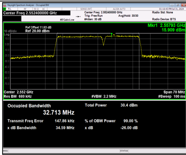
7-7-20MHz-15MHz-64QAM-64QAM-21201-21372-100RB#0-75RB#0-PASS
