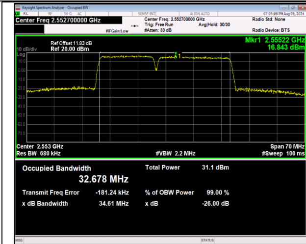
7-7-15MHz-20MHz-QPSK-QPSK-21179-21350-75RB#0-1 00RB#0-PASS
