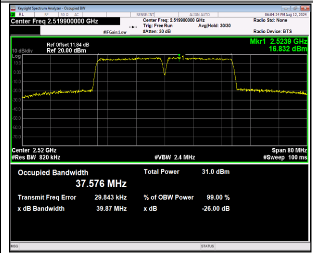
7-7-20MHz-20MHz-QPSK-QPSK-20850-21048-100RB#0-100RB#0-PASS
