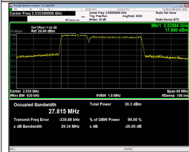
7-7-10MHz-20MHz-64QAM-64QAM-21006-21150-50RB# 0-100RB#0-PASS
