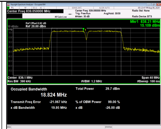
5-5-10MHz-10MHz-16QAM-16QAM-20501-20600-50RB #0-50RB#0-PASS
