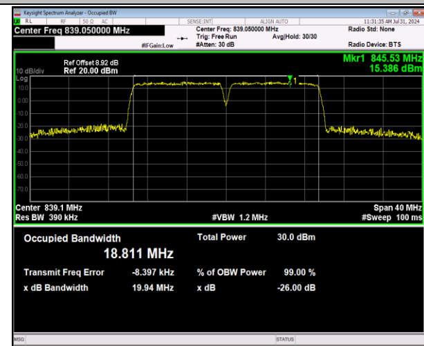
5-5-10MHz-10MHz-64QAM-64QAM-20501-20600-50RB# 0-50RB#0-PASS
