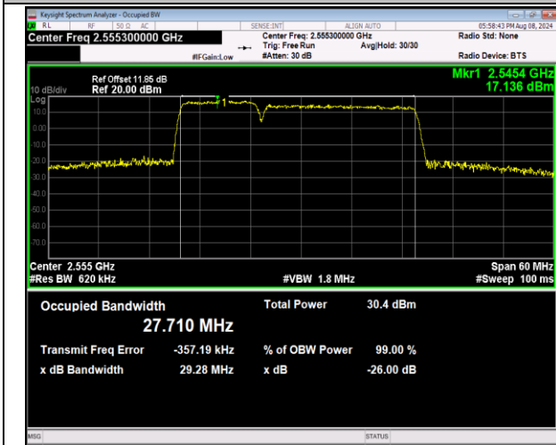
7-7-10MHz-20MHz-16QAM-16QAM-21206-21350-50RB# 0-100RB#0-PASS
