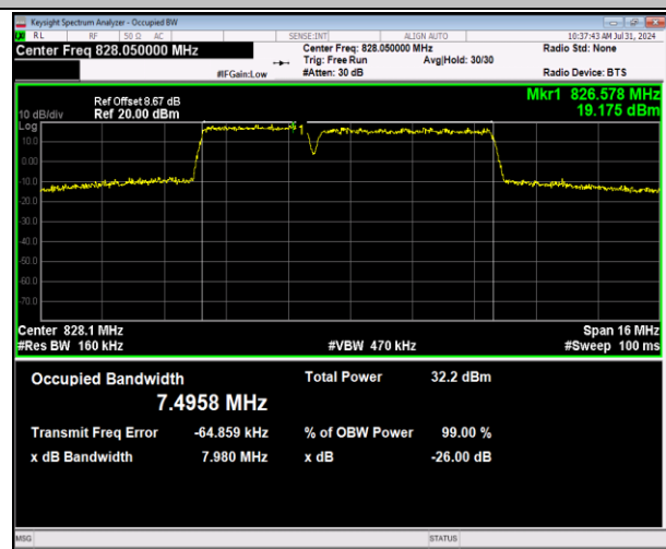
5-5-3MHz-5MHz-64QAM-64QAM-20416-20455-15RB#0-25RB#0-PASS
