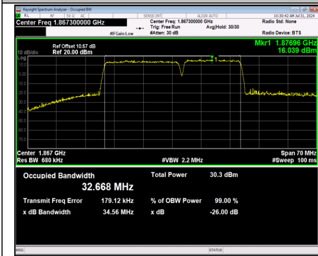
2-2-20MHz-15MHz-64QAM-64QAM-18700-18871-100RB#0-75RB#0-PASS
