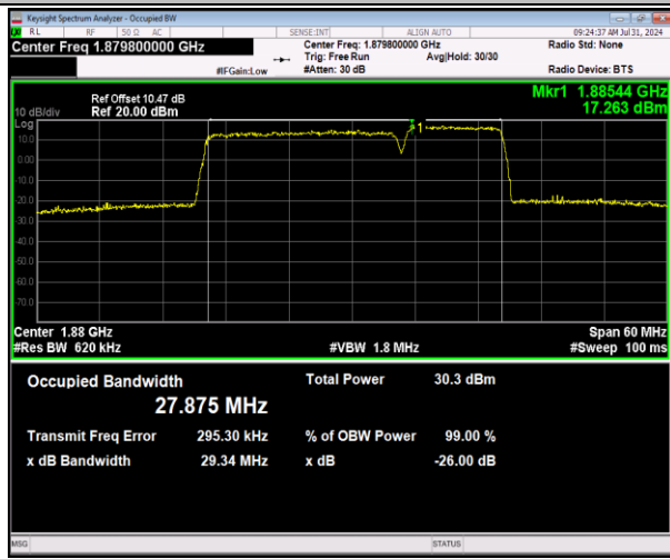
2-2-20MHz-10MHz-64QAM-64QAM-18851-18995-100RB#0-50RB#0-PASS
