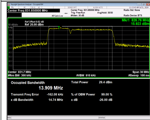
5-5-5MHz-10MHz-64QAM-64QAM-20428-20500-25RB#0-50RB#0-PASS
