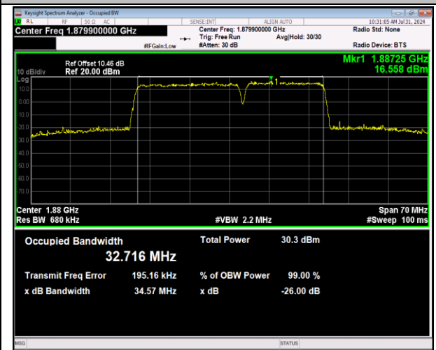
2-2-20MHz-15MHz-64QAM-64QAM-18826-18997-100RB#0-75RB#0-PASS
