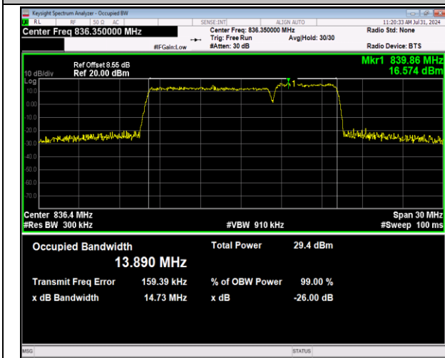
5-5-10MHz-5MHz-64QAM-64QAM-20500-20572-50RB#0-25RB#0-PASS
