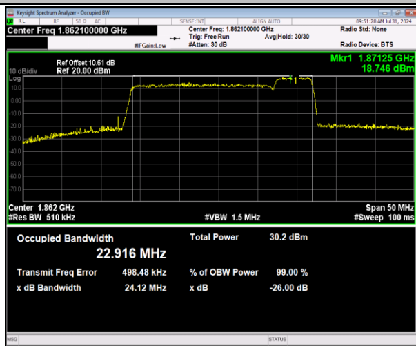
2-2-20MHz-5MHz-64QAM-64QAM-18700-18817-100RB#0-0-25RB#0-PASS
