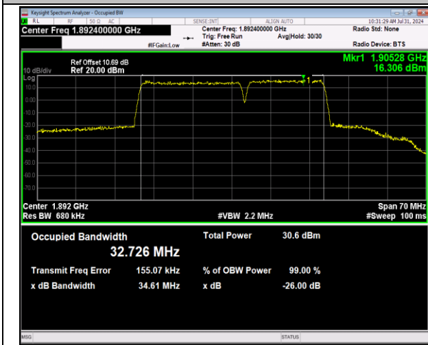
2-2-20MHz-15MHz-64QAM-64QAM-18951-19122-100RB#0-75RB#0-PASS
