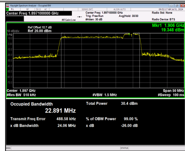
2-2-20MHz-5MHz-64QAM-64QAM-19050-19167-100RB# 0-25RB#0-PASS
