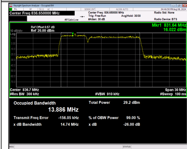
5-5-5MHz-10MHz-16QAM-16QAM-20478-20550-25RB#0-50RB#0-PASS
