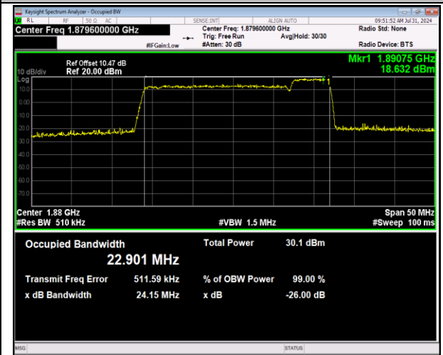
2-2-20MHz-5MHz-64QAM-64QAM-18875-18992-100RB#0-25RB#0-PASS
