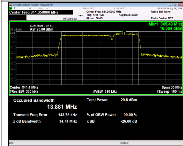
5-5-10MHz-5MHz-16QAM-16QAM-20550-20622-50RB#0-25RB#0-PASS
