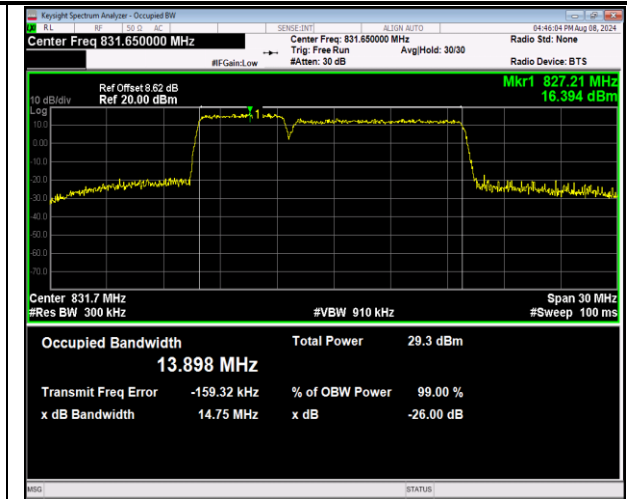
5-5-5MHz-10MHz-16QAM-16QAM-20428-20500-25RB#0-50RB#0-PASS
