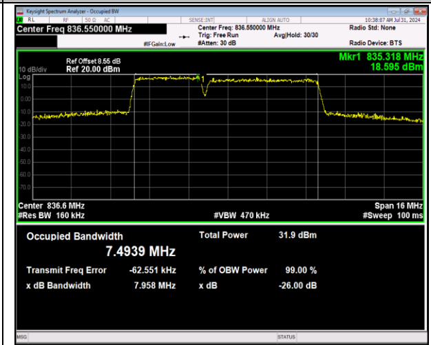
5-5-3MHz-5MHz-64QAM-64QAM-20501-20540-15RB#0-25RB#0-PASS
