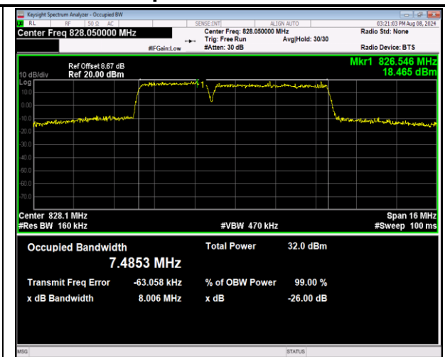
5-5-3MHz-5MHz-16QAM-16QAM-20416-20455-15RB#0-25RB#0-PASS
