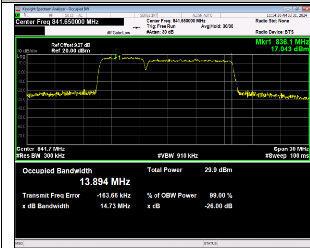
5-5-5MHz-10MHz-64QAM-64QAM-20528-20600-25RB#0-50RB#0-PASS
