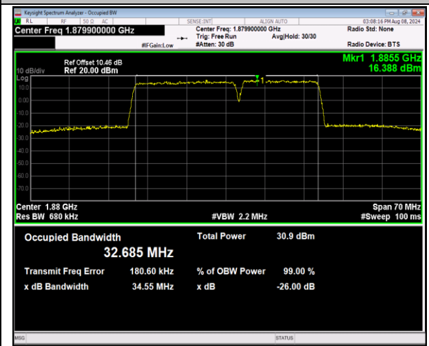
2-2-20MHz-15MHz-QPSK-QPSK-18826-18997-100RB#0-75RB#0-PASS
