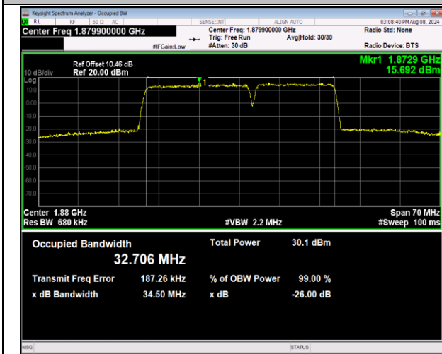
2-2-20MHz-15MHz-16QAM-16QAM-18826-18997-100RB#0-75RB#0-PASS
