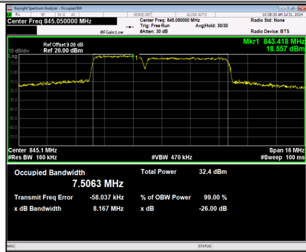
5-5-3MHz-5MHz-64QAM-64QAM-20586-20625-15RB#0-2 5RB#0-PASS
