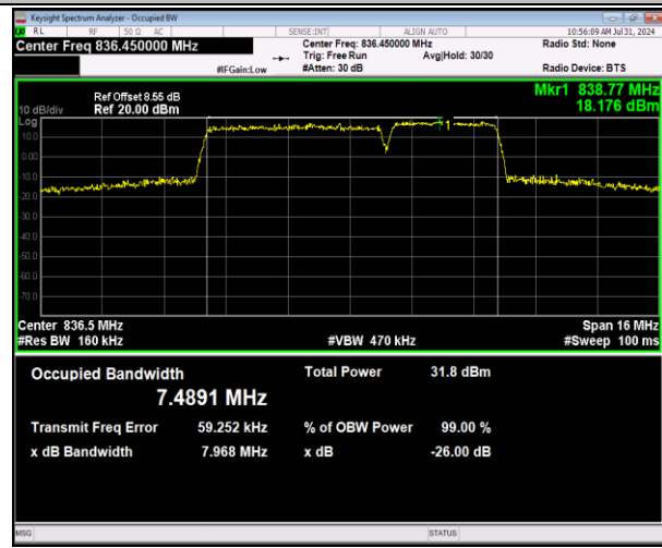
5-5-5MHz-3MHz-64QAM-64QAM-20510-20549-25RB#0-15 5RB#0-PASS
