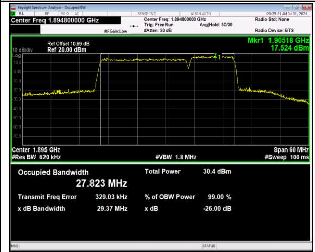
2-2-20MHz-10MHz-64QAM-64QAM-19001-19145-100RB#0-50RB#0-PASS
