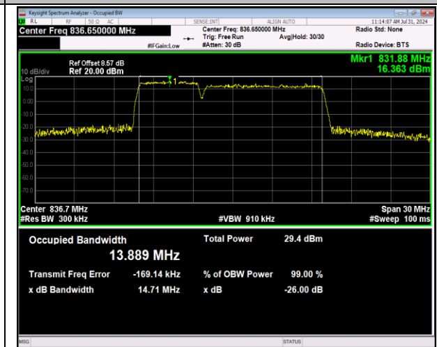
5-5-5MHz-10MHz-64QAM-64QAM-20478-20550-25RB#0-50RB#0-PASS
