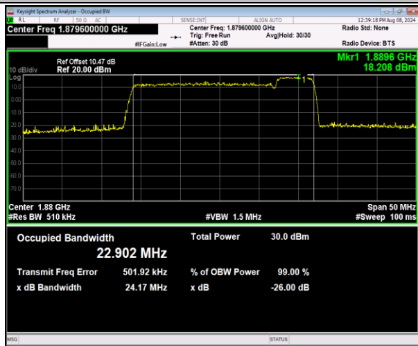
2-2-20MHz-5MHz-16QAM-16QAM-18875-18992-100RB#0-0-25RB#0-PASS
