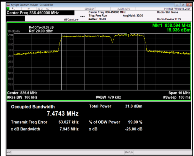
5-5-5MHz-3MHz-16QAM-16QAM-20510-20549-25RB#0-15 -15RB#0-PASS
