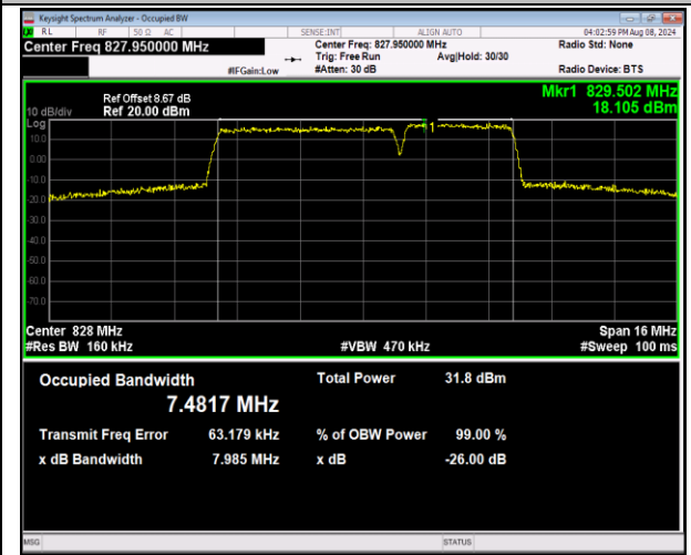
5-5-5MHz-3MHz-QPSK-QPSK-20425-20464-25RB#0-15 RB#0-PASS
