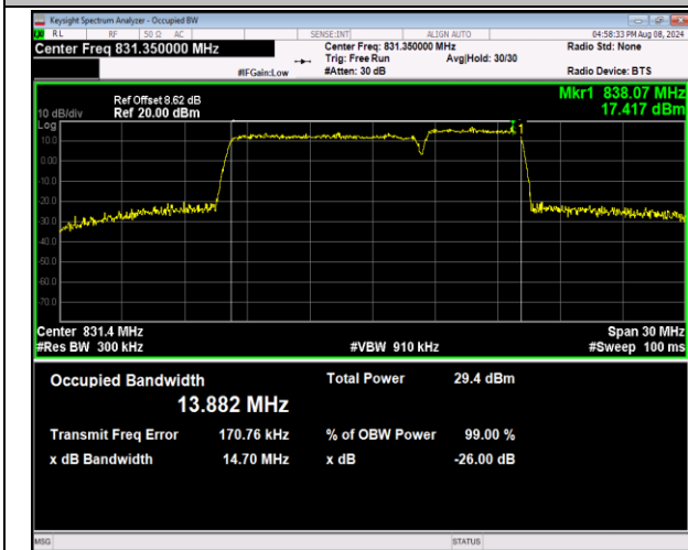
5-5-10MHz-5MHz-16QAM-16QAM-20450-20522-50RB#0-25RB#0-PASS
